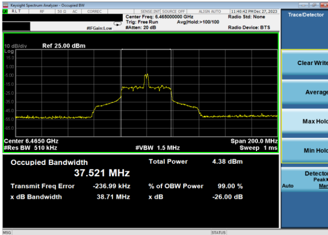
Plot 7-26. 26dB & 99% Bandwidth Plot Antenna 5T (80MHz 802.11ax RU26 (UNII Band 6) – Ch. 103)
