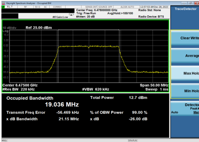
Plot 7-20. 26dB & 99% Bandwidth Plot Antenna 5T (20MHz 802.11ax RU242 (UNII Band 6) – Ch. 105)
