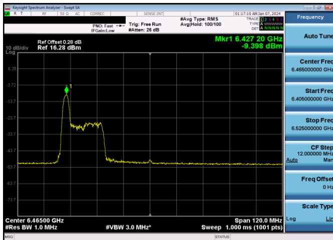
Plot 7-658. LPI Power Spectral Density Plot SDM Primary Antenna 3b (80MHz 802.11ax RU26 (UNII Band 6) – Ch. 103)
