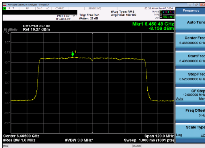
Plot 7-664. LPI Power Spectral Density Plot SDM Primary Antenna 3b (80MHz 802.11ax RU996 (UNII Band 6) – Ch. 103)
