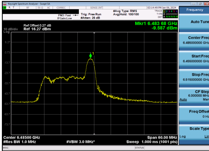
Plot 7-651. LPI Power Spectral Density Plot SDM Primary Antenna 5T (40MHz 802.11ax RU26 (UNII Band 6) – Ch. 107)
