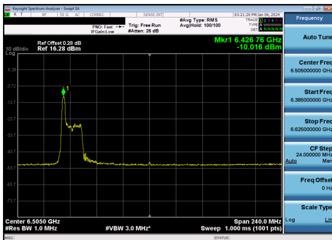
Plot 7-665. LPI Power Spectral Density Plot SDM Primary Antenna 5T (160MHz 802.11ax RU26 (UNII Band 6) – Ch. 111)
