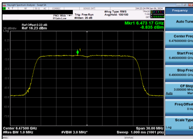
Plot 7-647. LPI Power Spectral Density Plot SDM Primary Antenna 5T (20MHz 802.11ax RU242 (UNII Band 6) - Ch. 105)
