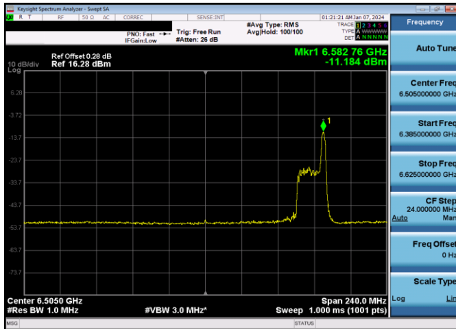
Plot 7-670. LPI Power Spectral Density Plot SDM Primary Antenna 3b (160MHz 802.11ax RU26 (UNII Band 6) – Ch. 111)
