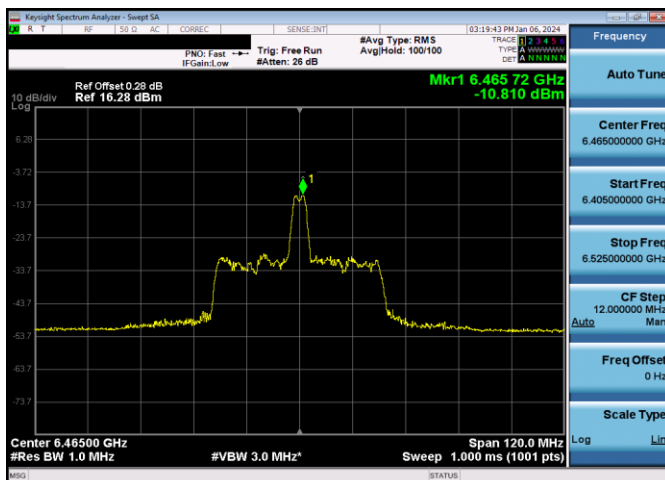
Plot 7-659. LPI Power Spectral Density Plot SDM Primary Antenna 5T (80MHz 802.11ax RU26 (UNII Band 6) – Ch. 103)
