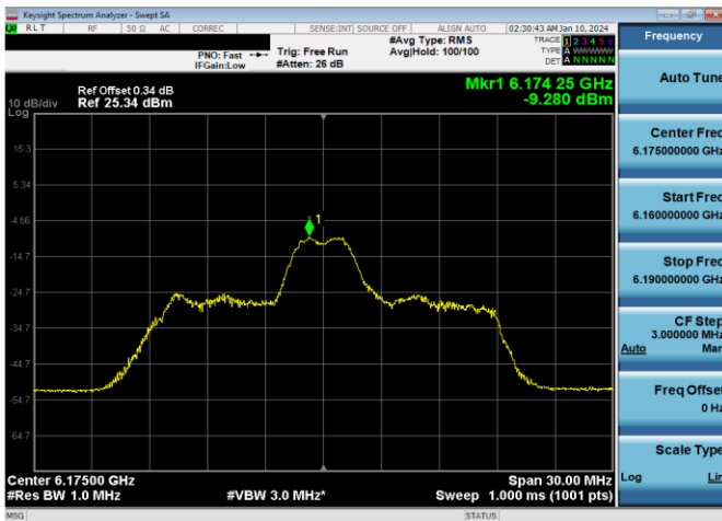
Plot 7-611. LPI Power Spectral Density Plot SDM Primary Antenna 5T (20MHz 802.11ax RU26 (UNII Band 5) – Ch. 45)
