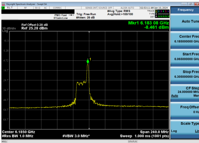
Plot 7-635. LPI Power Spectral Density Plot SDM Primary Antenna 5T (160MHz 802.11ax RU26 (UNII Band 5) – Ch. 47)
