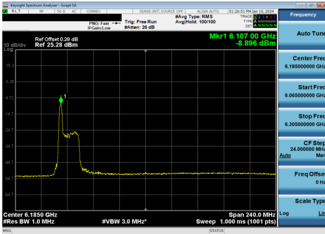
Plot 7-634. LPI Power Spectral Density Plot SDM Primary Antenna 3b (160MHz 802.11ax RU26 (UNII Band 5) – Ch. 47)
