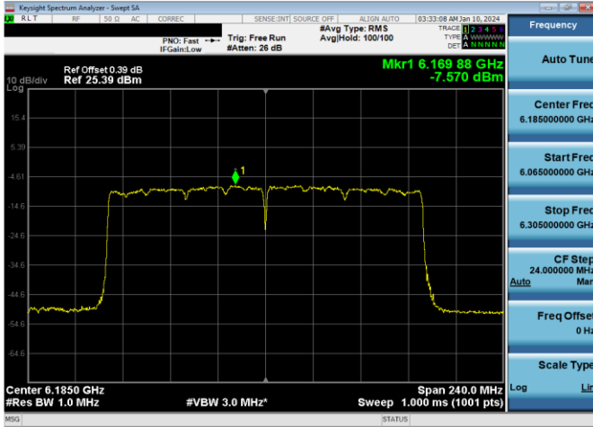
Plot 7-639. LPI Power Spectral Density Plot SDM Primary Antenna 5T (160MHz 802.11ax RU996x2 (UNII Band 5) – Ch. 47)
