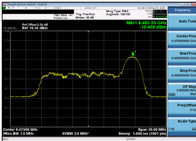
Plot 7-646. LPI Power Spectral Density Plot SDM Primary Antenna 3b (20MHz 802.11ax RU26 (UNII Band 6) - Ch. 105)
