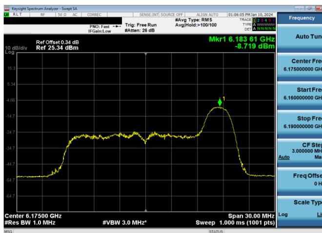
Plot 7-614. LPI Power Spectral Density Plot SDM Primary Antenna 3b (20MHz 802.11ax RU26 (UNII Band 5) – Ch. 45)
