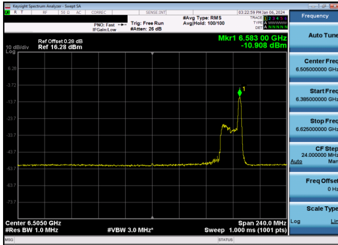
Plot 7-669. LPI Power Spectral Density Plot SDM Primary Antenna 5T (160MHz 802.11ax RU26 (UNII Band 6) – Ch. 111)
