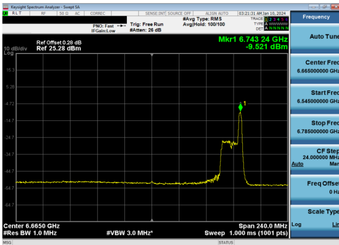
Plot 7-701. LPI Power Spectral Density Plot SDM Primary Antenna 5T (160MHz 802.11ax RU26 (UNII Band 7) – Ch. 143)
