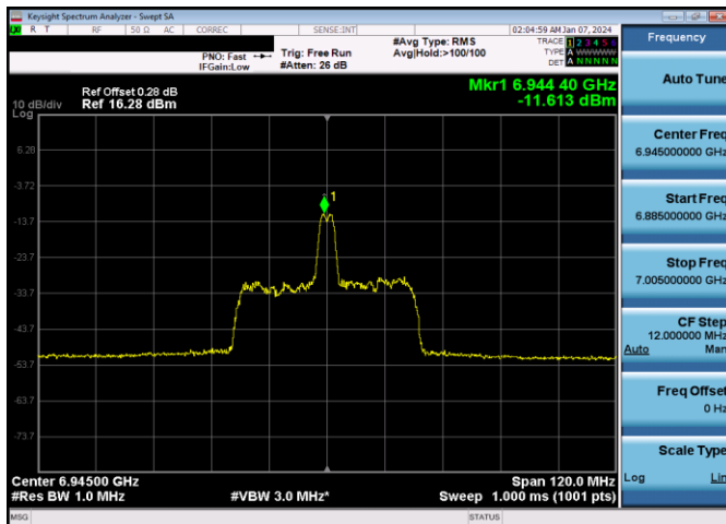
Plot 7-724. LPI Power Spectral Density Plot SDM Primary Antenna 3b (80MHz 802.11ax RU26 (UNII Band 8) – Ch. 199)
