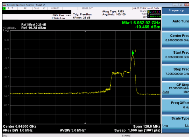
Plot 7-725. LPI Power Spectral Density Plot SDM Primary Antenna 5T (80MHz 802.11ax RU26 (UNII Band 8) – Ch. 199)
