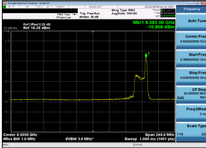
Plot 7-797. LPI Power Spectral Density Plot SDM Diversity Antenna 5T (160MHz 802.11ax RU26 (UNII Band 6) – Ch. 111)
