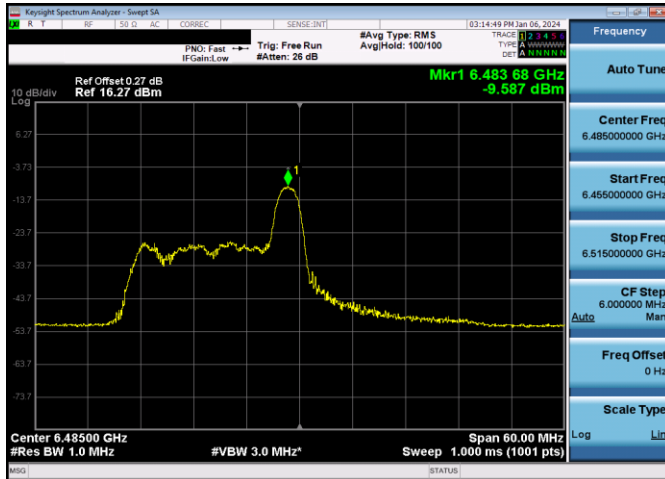
Plot 7-779. LPI Power Spectral Density Plot SDM Diversity Antenna 5T (40MHz 802.11ax RU26 (UNII Band 6) – Ch. 107)
