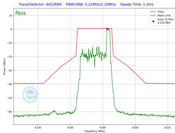
Plot 7-899. SP In-Band Emission Plot Antenna 3b (20MHz 802.11ax RU26 (UNII Band 5) – Ch. 45)
