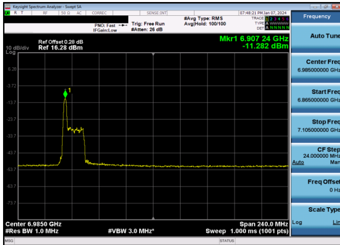
Plot 7-858. LPI Power Spectral Density Plot SDM Diversity Antenna 1b (160MHz 802.11ax RU26 (UNII Band 8) – Ch. 207)
