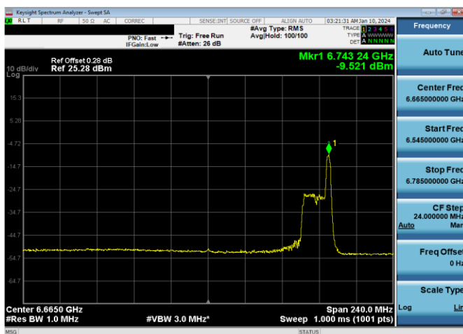
Plot 7-829. LPI Power Spectral Density Plot SDM Diversity Antenna 5T (160MHz 802.11ax RU26 (UNII Band 7) – Ch. 143)
