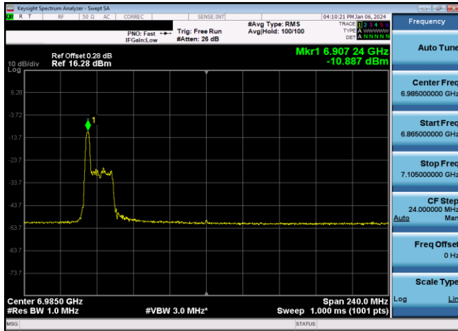
Plot 7-857. LPI Power Spectral Density Plot SDM Diversity Antenna 5T (160MHz 802.11ax RU26 (UNII Band 8) – Ch. 207)
