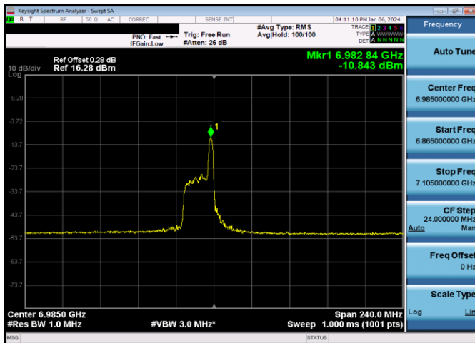
Plot 7-859. LPI Power Spectral Density Plot SDM Diversity Antenna 5T (160MHz 802.11ax RU26 (UNII Band 8) – Ch. 207)
