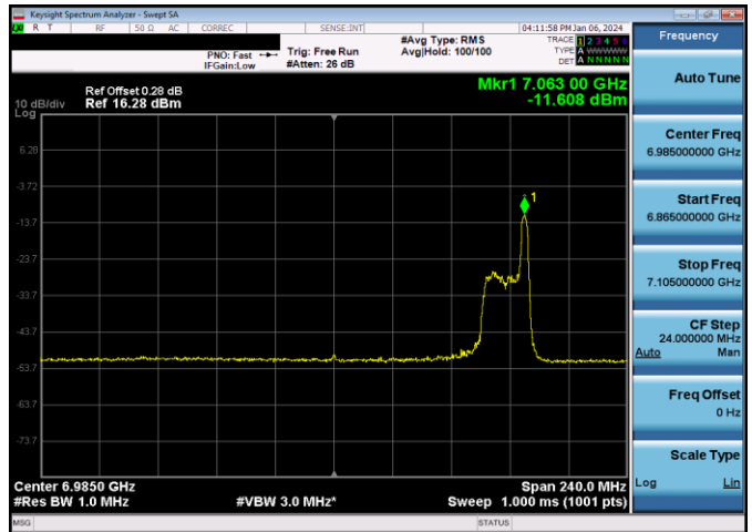
Plot 7-861. LPI Power Spectral Density Plot SDM Diversity Antenna 5T (160MHz 802.11ax RU26 (UNII Band 8) – Ch. 207)
