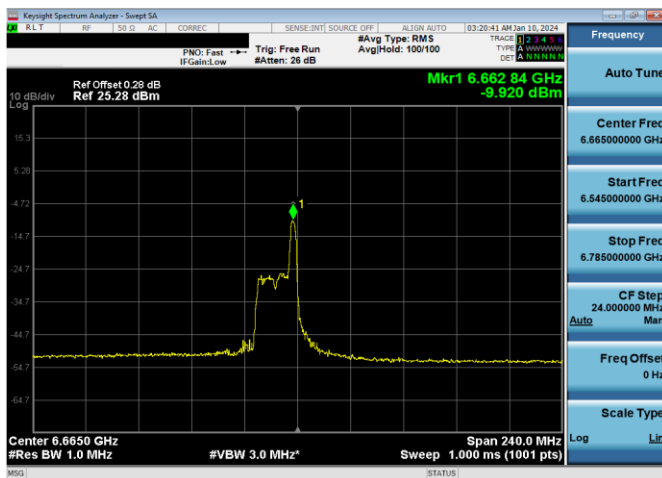
Plot 7-827. LPI Power Spectral Density Plot SDM Diversity Antenna 5T (160MHz 802.11ax RU26 (UNII Band 7) – Ch. 143)
