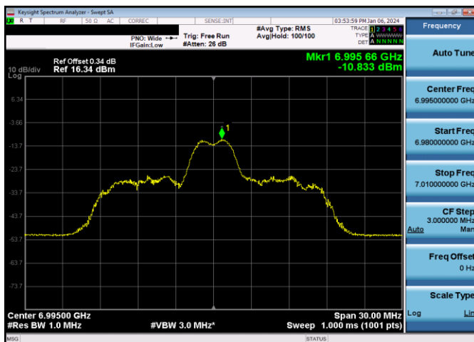
Plot 7-835. LPI Power Spectral Density Plot SDM Diversity Antenna 5T (20MHz 802.11ax RU26 (UNII Band 8) – Ch. 209)
