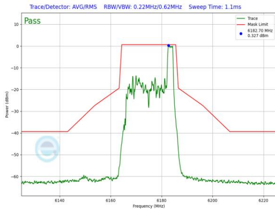
Plot 7-867. SP In-Band Emission Plot Antenna 5T (20MHz 802.11ax RU26 (UNII Band 5) – Ch. 45)
