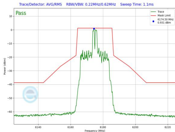
Plot 7-1027. SP In-Band Emission Plot CDD Diversity Antenna 5T (20MHz 802.11ax RU26 (UNII Band 5) – Ch. 45)
