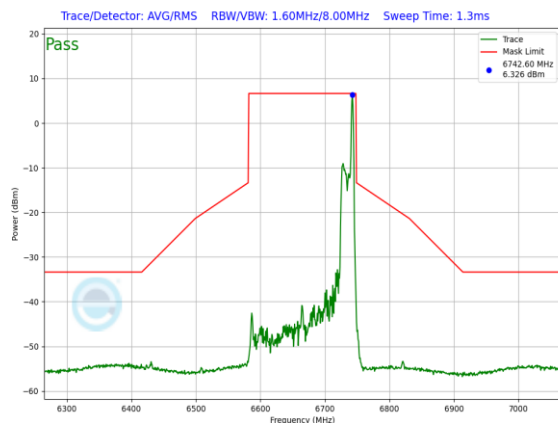
Plot 7-927. SP In-Band Emission Plot Antenna 3b (160MHz 802.11ax RU26 (UNII Band 7) – Ch. 143)
