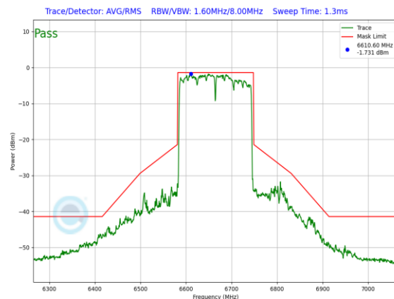
Plot 7-928. SP In-Band Emission Plot Antenna 3b (160MHz 802.11ax RU996x2 (UNII Band 7) – Ch. 143)
