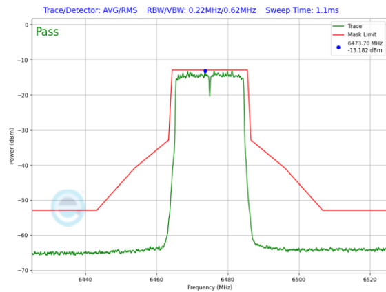
Plot 7-1108. LPI In-Band Emission Plot Antenna 5T (20MHz 802.11ax RU242 (UNII Band 6) – Ch. 105)
