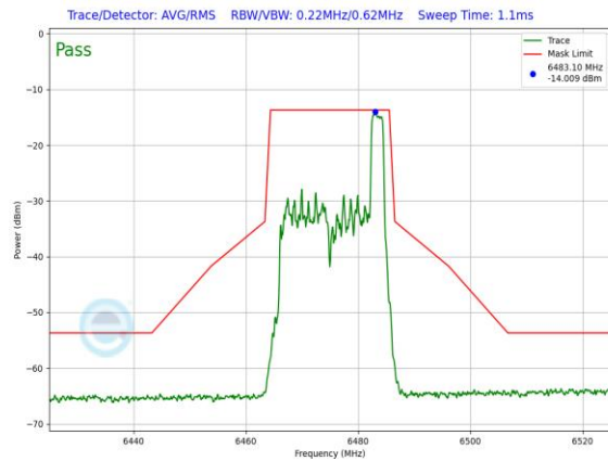
Plot 7-1107. LPI In-Band Emission Plot Antenna 5T (20MHz 802.11ax RU26 (UNII Band 6) – Ch. 105)
