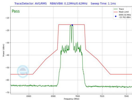
Plot 7-1138. LPI In-Band Emission Plot Antenna 5T (20MHz 802.11ax RU26 (UNII Band 8) – Ch. 209)
