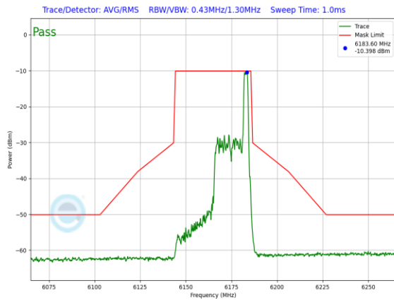
Plot 7-1095. LPI In-Band Emission Plot Antenna 5T (40MHz 802.11ax RU26 (UNII Band 5) – Ch. 43)
