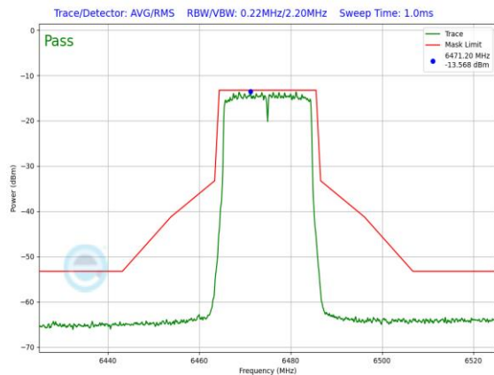
Plot 7-1236. LPI In-Band Emission Plot Antenna 1b (20MHz 802.11ax RU242 (UNII Band 6) – Ch. 105)
