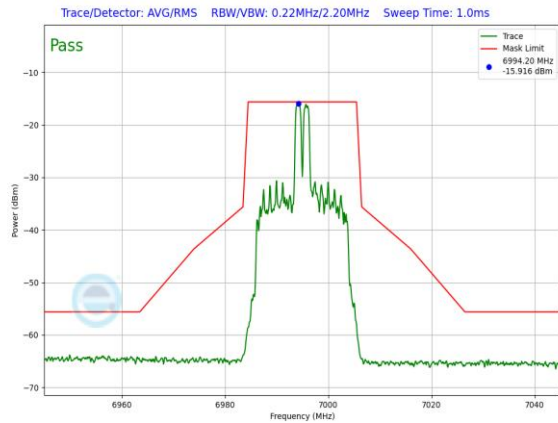
Plot 7-1202. LPI In-Band Emission Plot Antenna 3b (20MHz 802.11ax RU26 (UNII Band 8) – Ch. 209)
