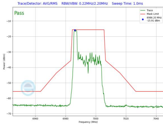
Plot 7-1201. LPI In-Band Emission Plot Antenna 3b (20MHz 802.11ax RU26 (UNII Band 8) – Ch. 209)
