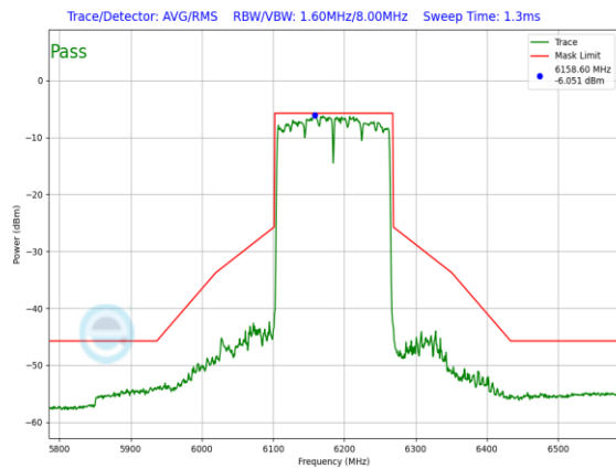
Plot 7-1440. LPI In-Band Emission Plot SDM Diversity Antenna 1b (160MHz 802.11ax RU996x2 (UNII Band 5) – Ch. 47)
