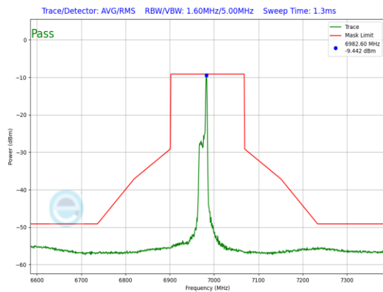
Plot 7-1403. LPI In-Band Emission Plot SDM Primary Antenna 5T (160MHz 802.11ax RU26 (UNII Band 8) – Ch. 207)
