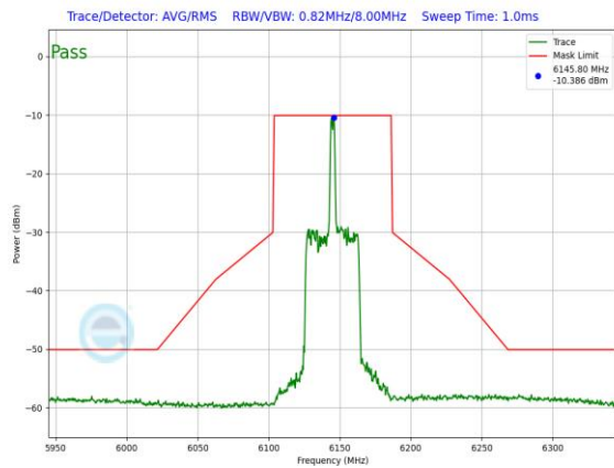
Plot 7-1428. LPI In-Band Emission Plot SDM Diversity Antenna 1b (80MHz 802.11ax RU26 (UNII Band 5) – Ch. 39)
