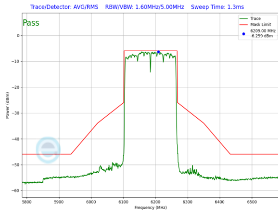
Plot 7-1439. LPI In-Band Emission Plot SDM Diversity Antenna 5T (160MHz 802.11ax RU996x2 (UNII Band 5) – Ch. 47)
