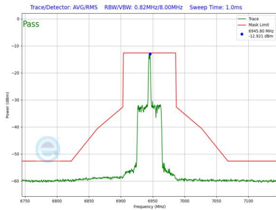
Plot 7-1396. LPI In-Band Emission Plot SDM Primary Antenna 3b (80MHz 802.11ax RU26 (UNII Band 8) – Ch. 199)
