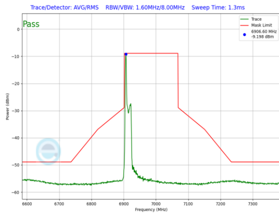
Plot 7-1402. LPI In-Band Emission Plot SDM Primary Antenna 3b (160MHz 802.11ax RU26 (UNII Band 8) – Ch. 207)
