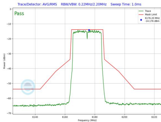
Plot 7-1416. LPI In-Band Emission Plot SDM Diversity Antenna 1b (20MHz) 802.11ax RU242 (UNII Band 5) – Ch. 45)
