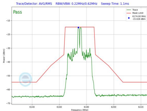
Plot 7-1411. LPI In-Band Emission Plot SDM Diversity Antenna 5T (20MHz 802.11ax RU26 (UNII Band 5) – Ch. 45)
