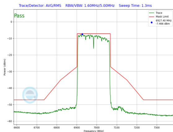
Plot 7-1407. LPI In-Band Emission Plot SDM Primary Antenna 5T (160MHz 802.11ax RU996x2 (UNII Band 8) – Ch. 207)
