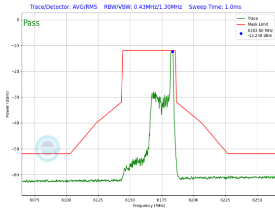
Plot 7-1421. LPI In-Band Emission Plot SDM Diversity Antenna 5T (40MHz 802.11ax RU26 (UNII Band 5) – Ch. 43)
