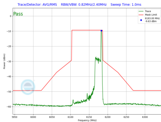
Plot 7-1429. LPI In-Band Emission Plot SDM Diversity Antenna 5T (80MHz 802.11ax RU26 (UNII Band 5) – Ch. 39)
