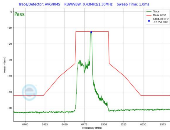
Plot 7-1323. LPI In-Band Emission Plot SDM Primary Antenna 5T (40MHz 802.11ax RU26 (UNII Band 6) – Ch. 107)
