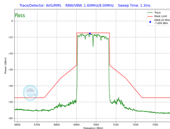
Plot 7-1408. LPI In-Band Emission Plot SDM Primary Antenna 3b (160MHz 802.11ax RU996x2 (UNII Band 8) – Ch. 207)
