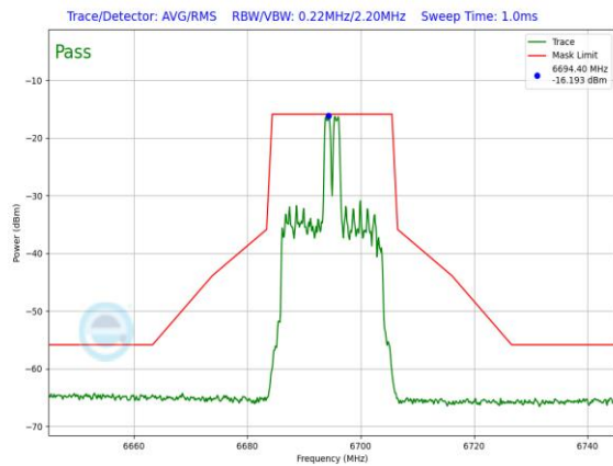
Plot 7-1348. LPI In-Band Emission Plot SDM Primary Antenna 3b (20MHz 802.11ax RU26 (UNII Band 7) – Ch. 149)
