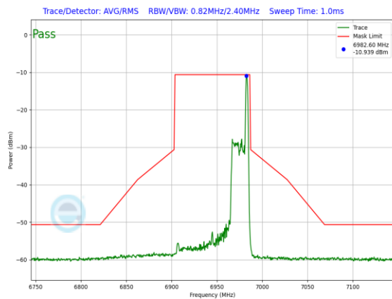
Plot 7-1397. LPI In-Band Emission Plot SDM Primary Antenna 5T (80MHz 802.11ax RU26 (UNII Band 8) – Ch. 199)
