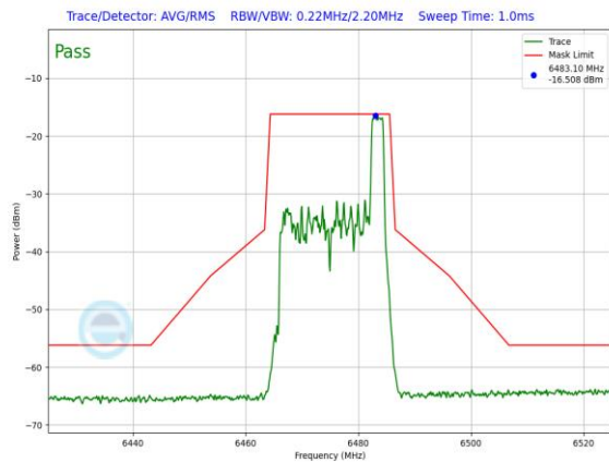
Plot 7-1446. LPI In-Band Emission Plot SDM Diversity Antenna 1b (20MHz 802.11ax RU26 (UNII Band 6) – Ch. 105)
