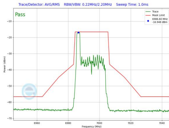
Plot 7-1378. LPI In-Band Emission Plot SDM Primary Antenna 3b (20MHz 802.11ax RU26 (UNII Band 8) – Ch. 209)
