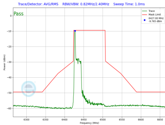
Plot 7-1329. LPI In-Band Emission Plot SDM Primary Antenna 5T (80MHz 802.11ax RU26 (UNII Band 6) – Ch. 103)
