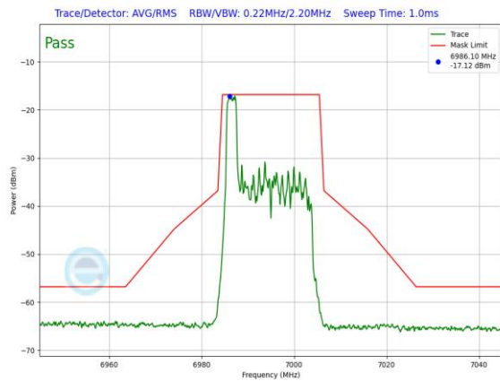
Plot 7-1506. LPI In-Band Emission Plot SDM Diversity Antenna 1b (20MHz 802.11ax RU26 (UNII Band 8) – Ch. 209)
