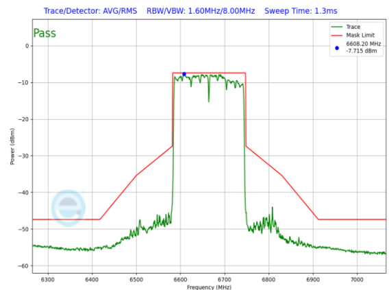
Plot 7-1504. LPI In-Band Emission Plot SDM Diversity Antenna 1b (160MHz 802.11ax RU996x2 (UNII Band 7) – Ch. 143)
