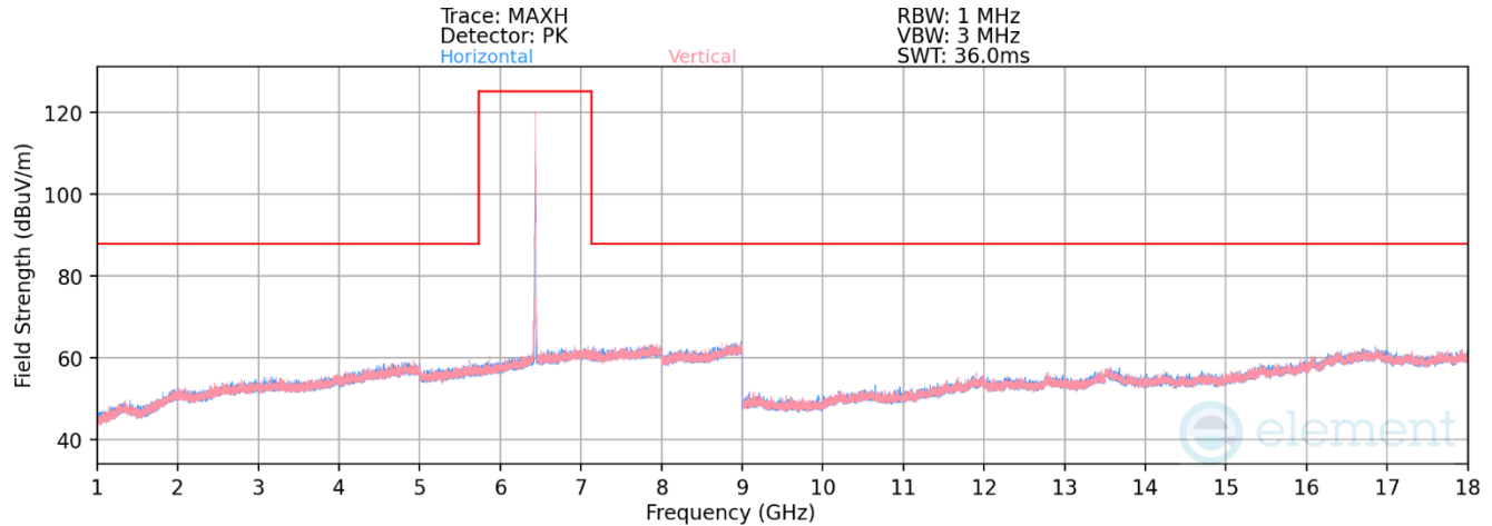
Plot 7-1576. Radiated Spurious Emissions above 1GHz Antenna 5T (802.11ax – Ch. 97 – RU26)
