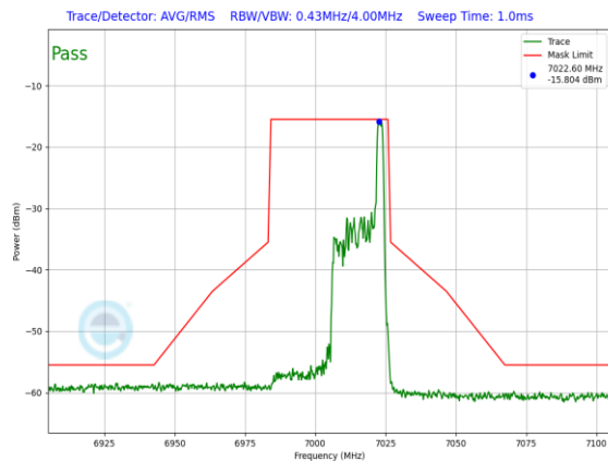
Plot 7-1518. LPI In-Band Emission Plot SDM Diversity Antenna 1b (40MHz 802.11ax RU26 (UNII Band 8) – Ch. 211)
