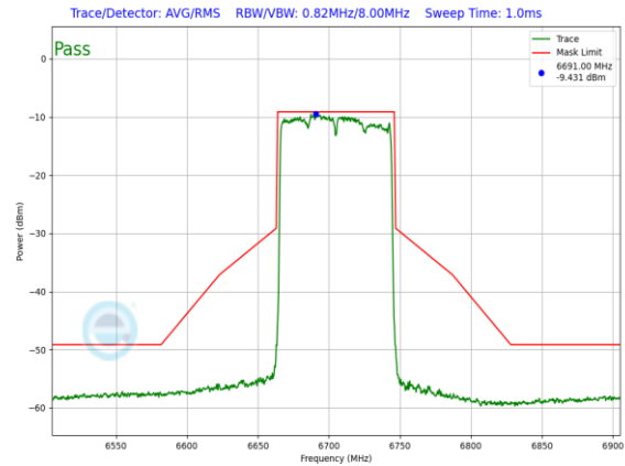
Plot 7-1496. LPI In-Band Emission Plot SDM Diversity Antenna 1b (80MHz 802.11ax RU996 (UNII Band 7) – Ch. 151)
