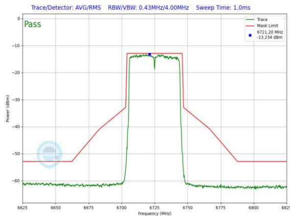
Plot 7-1488. LPI In-Band Emission Plot SDM Diversity Antenna 1b (40MHz 802.11ax RU484 (UNII Band 7) – Ch. 155)
