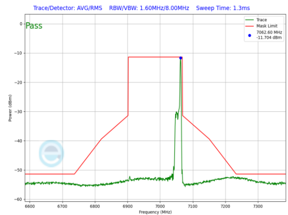
Plot 7-1534. LPI In-Band Emission Plot SDM Diversity Antenna 1b (160MHz 802.11ax RU26 (UNII Band 8) – Ch. 207)
