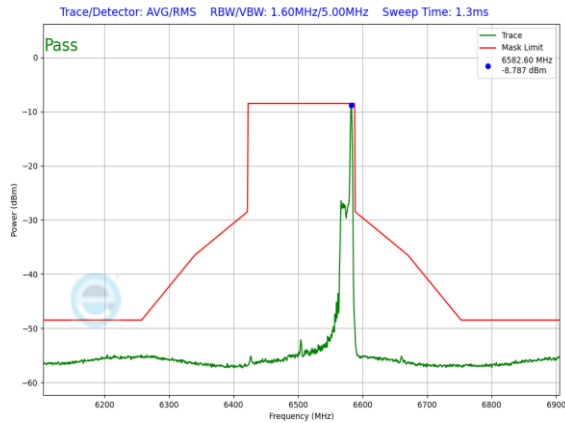
Plot 7-1469. LPI In-Band Emission Plot SDM Diversity Antenna 5T (160MHz 802.11ax RU26 (UNII Band 6) – Ch. 111)
