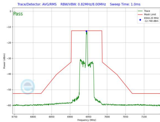
Plot 7-1524. LPI In-Band Emission Plot SDM Diversity Antenna 1b (80MHz 802.11ax RU26 (UNII Band 8) – Ch. 199)
