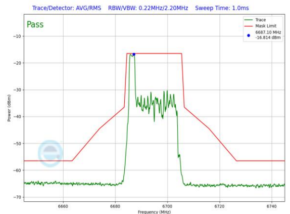
Plot 7-1474. LPI In-Band Emission Plot SDM Diversity Antenna 1b (20MHz 802.11ax RU26 (UNII Band 7) – Ch. 149)
