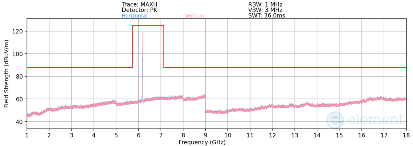
Plot 7-1574. Radiated Spurious Emissions above 1GHz Antenna 5T (802.11ax – Ch. 45 – RU26)
