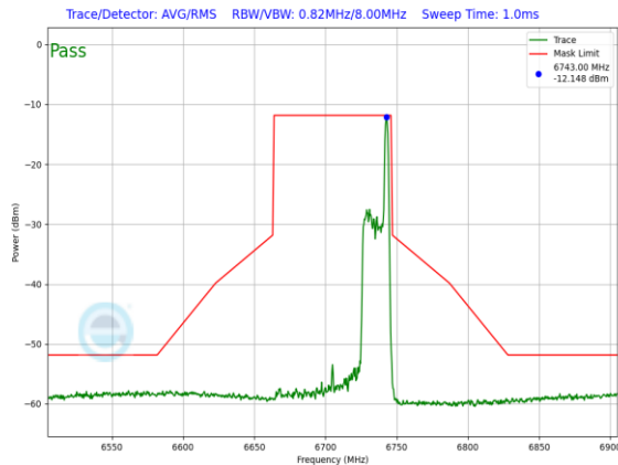
Plot 7-1494. LPI In-Band Emission Plot SDM Diversity Antenna 1b (80MHz 802.11ax RU26 (UNII Band 7) – Ch. 151)
