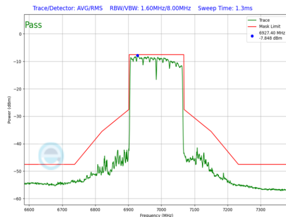
Plot 7-1536. LPI In-Band Emission Plot SDM Diversity Antenna 1b (160MHz 802.11ax RU996x2 (UNII Band 8) – Ch. 207)
