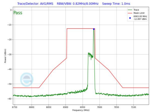
Plot 7-1526. LPI In-Band Emission Plot SDM Diversity Antenna 1b (80MHz 802.11ax RU26 (UNII Band 8) – Ch. 199)
