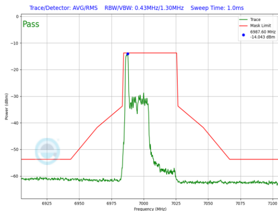
Plot 7-1513. LPI In-Band Emission Plot SDM Diversity Antenna 5T (40MHz 802.11ax RU26 (UNII Band 8) – Ch. 211)
