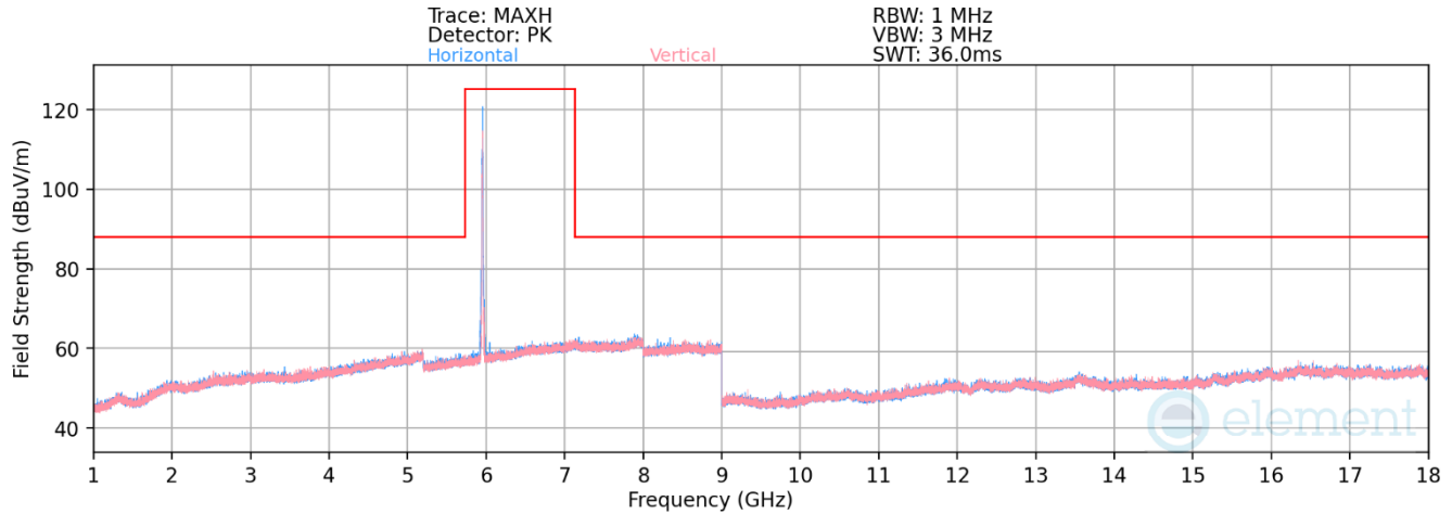
Plot 7-1573. Radiated Spurious Emissions above 1GHz Antenna 5T (802.11ax – Ch. 1 – RU26)
