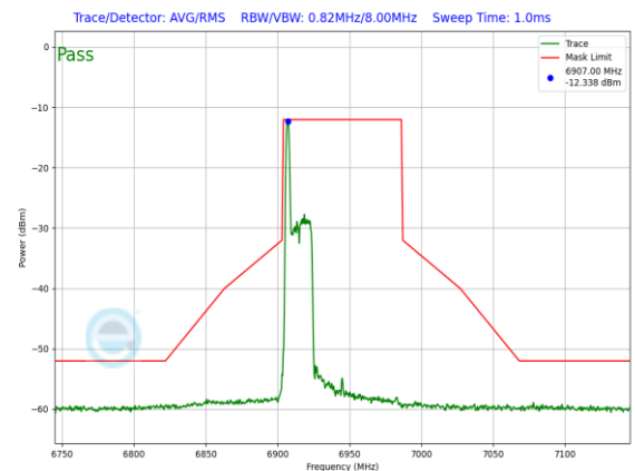
Plot 7-1522. LPI In-Band Emission Plot SDM Diversity Antenna 1b (80MHz 802.11ax RU26 (UNII Band 8) – Ch. 199)
