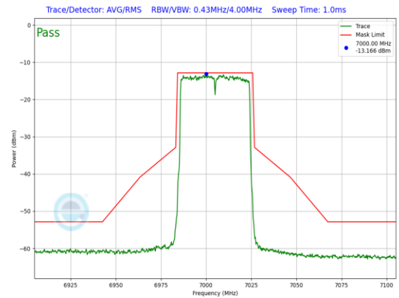
Plot 7-1520. LPI In-Band Emission Plot SDM Diversity Antenna 1b (40MHz 802.11ax RU484 (UNII Band 8) – Ch. 211)
