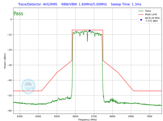
Plot 7-1503. LPI In-Band Emission Plot SDM Diversity Antenna 5T (160MHz 802.11ax RU996x2 (UNII Band 7) – Ch. 143)
