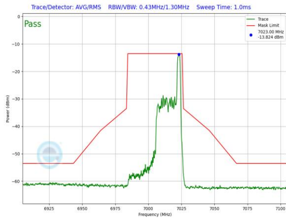
Plot 7-1517. LPI In-Band Emission Plot SDM Diversity Antenna 5T (40MHz 802.11ax RU26 (UNII Band 8) – Ch. 211)
