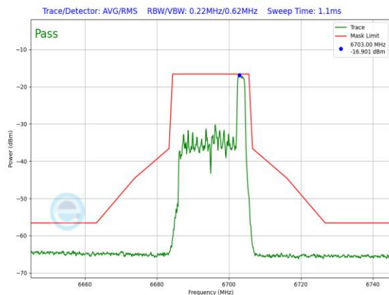
Plot 7-1477. LPI In-Band Emission Plot SDM Diversity Antenna 5T (20MHz 802.11ax RU26 (UNII Band 7) – Ch. 149)
