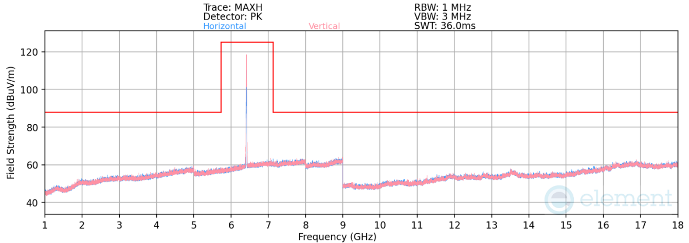
Plot 7-1575. Radiated Spurious Emissions above 1GHz Antenna 5T (802.11ax – Ch. 93 – RU26)
