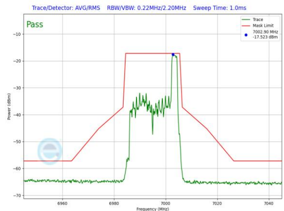
Plot 7-1510. LPI In-Band Emission Plot SDM Diversity Antenna 1b (20MHz 802.11ax RU26 (UNII Band 8) – Ch. 209)
