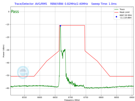
Plot 7-1489. LPI In-Band Emission Plot SDM Diversity Antenna 5T (80MHz 802.11ax RU26 (UNII Band 7) – Ch. 151)
