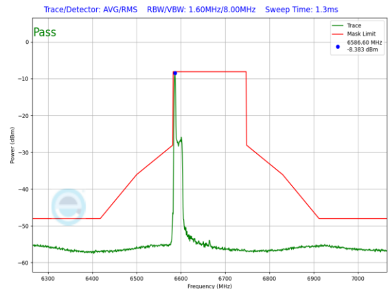
Plot 7-1498. LPI In-Band Emission Plot SDM Diversity Antenna 1b (160MHz 802.11ax RU26 (UNII Band 7) – Ch. 143)
