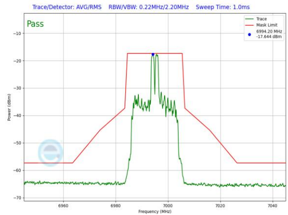
Plot 7-1508. LPI In-Band Emission Plot SDM Diversity Antenna 1b (20MHz 802.11ax RU26 (UNII Band 8) – Ch. 209)
