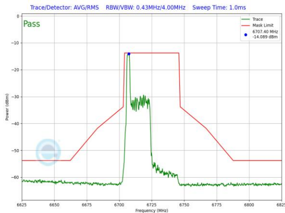
Plot 7-1482. LPI In-Band Emission Plot SDM Diversity Antenna 1b (40MHz 802.11ax RU26 (UNII Band 7) – Ch. 155)
