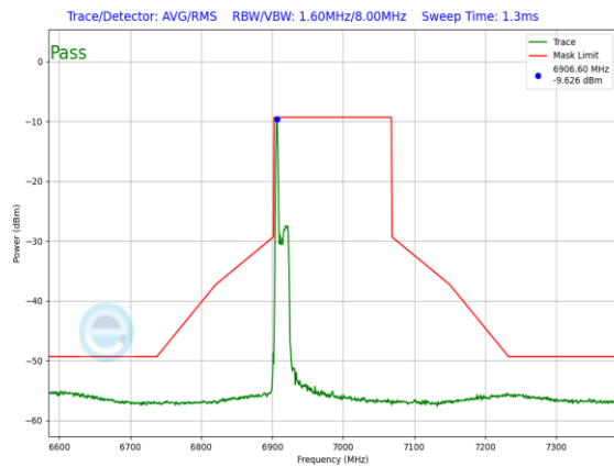
Plot 7-1530. LPI In-Band Emission Plot SDM Diversity Antenna 1b (160MHz 802.11ax RU26 (UNII Band 8) – Ch. 207)
