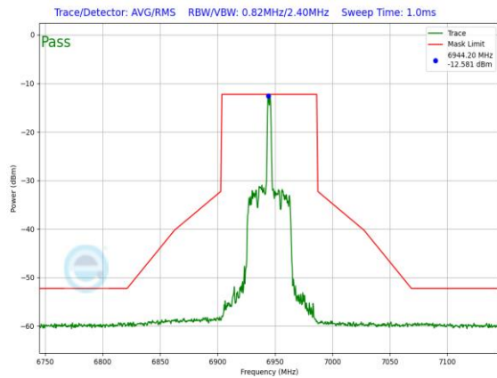
Plot 7-1523. LPI In-Band Emission Plot SDM Diversity Antenna 5T (80MHz 802.11ax RU26 (UNII Band 8) – Ch. 199)
