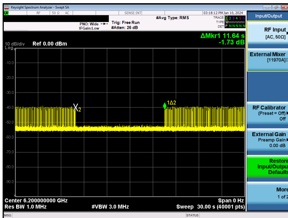
Plot 7-1555. Contention Based Protocol Timing Plot – UNII 5 – 160MHz Channel 47 – Mid
