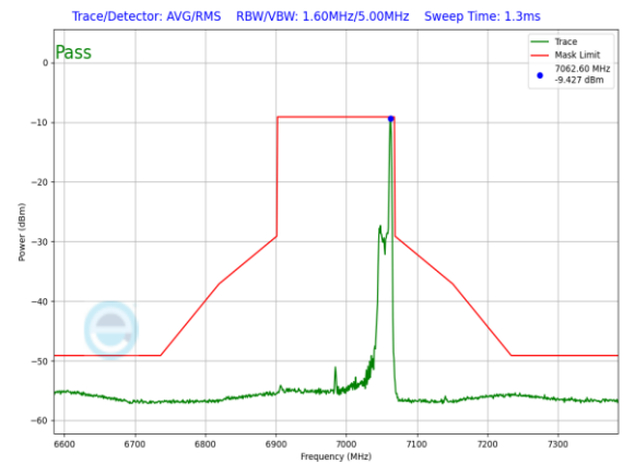
Plot 7-1533. LPI In-Band Emission Plot SDM Diversity Antenna 5T (160MHz 802.11ax RU26 (UNII Band 8) – Ch. 207)
