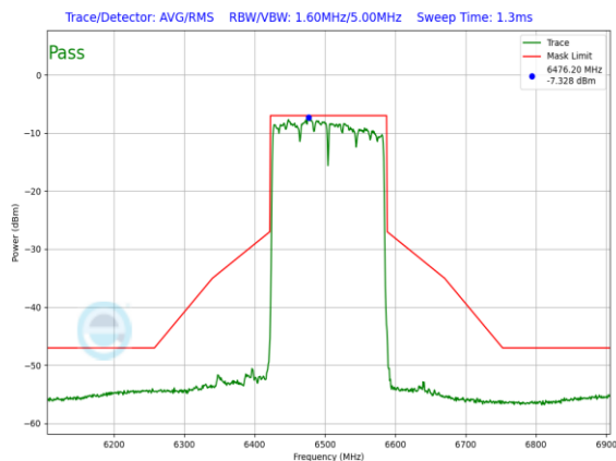
Plot 7-1471. LPI In-Band Emission Plot SDM Diversity Antenna 5T (160MHz 802.11ax RU996x2 (UNII Band 6) – Ch. 111)
