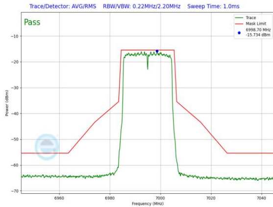
Plot 7-1512. LPI In-Band Emission Plot SDM Diversity Antenna 1b (20MHz 802.11ax RU242 (UNII Band 8) – Ch. 209)
