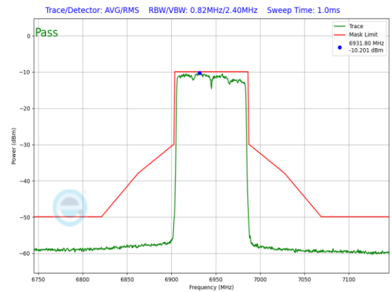
Plot 7-1527. LPI In-Band Emission Plot SDM Diversity Antenna 5T (80MHz 802.11ax RU996 (UNII Band 8) – Ch. 199)
