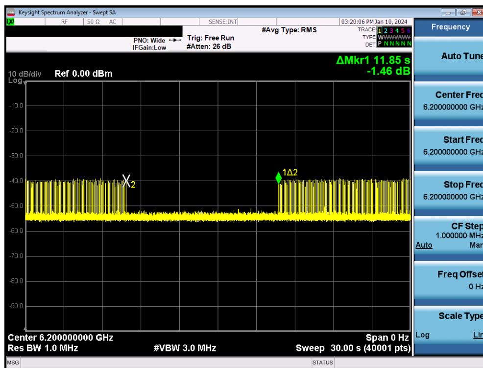
Plot 7-1554. Contention Based Protocol Timing Plot – UNII 5 – 160MHz Channel 47 – Low
