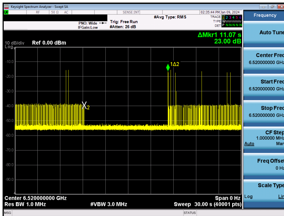
Plot 7-1559. Contention Based Protocol Timing Plot – UNII 6 – 160MHz Channel 111 – Mid
