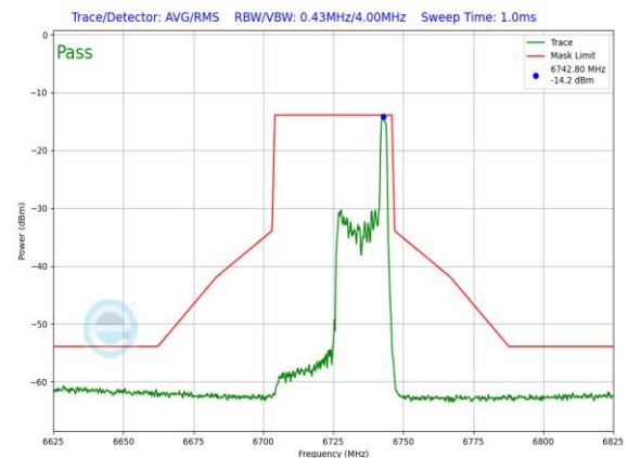
Plot 7-1486. LPI In-Band Emission Plot SDM Diversity Antenna 1b (40MHz 802.11ax RU26 (UNII Band 7) – Ch. 155)
