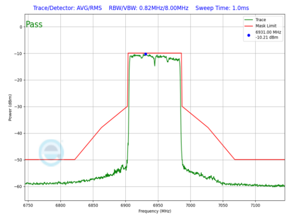
Plot 7-1528. LPI In-Band Emission Plot SDM Diversity Antenna 1b (80MHz 802.11ax RU996 (UNII Band 8) – Ch. 199)
