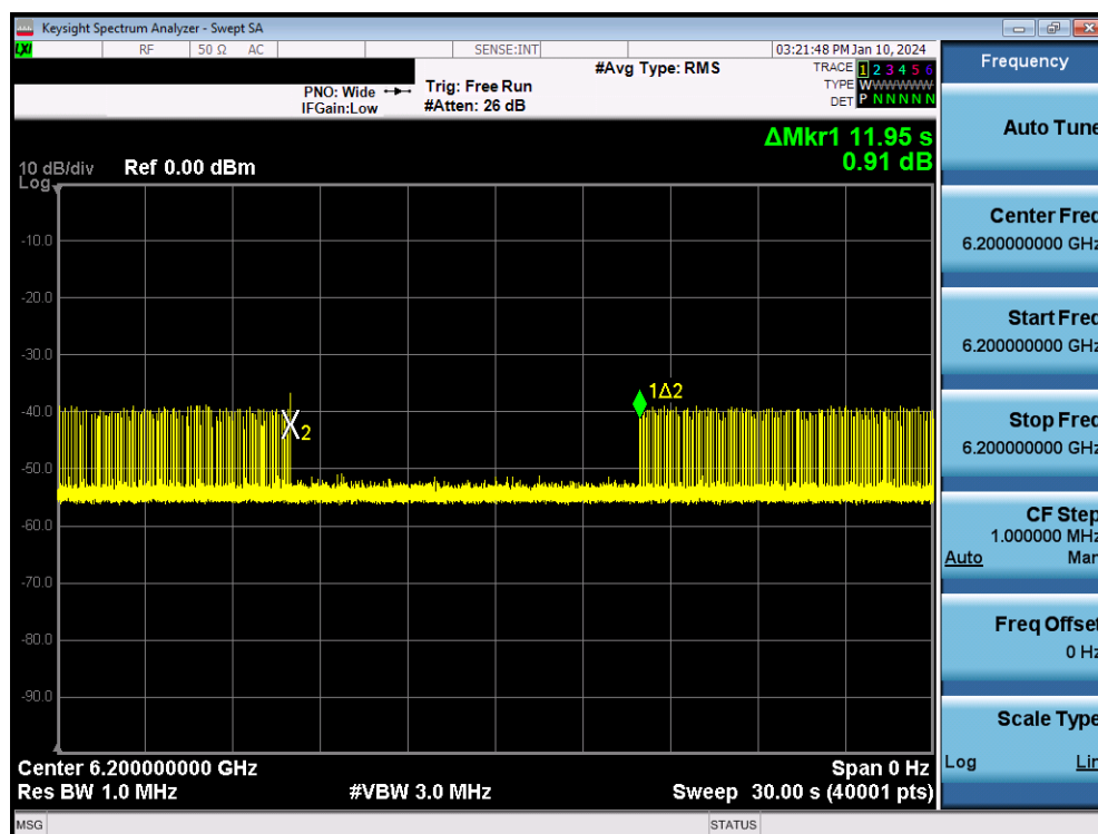
Plot 7-1556. Contention Based Protocol Timing Plot – UNII 5 – 160MHz Channel 47 – High
