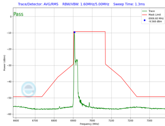
Plot 7-1529. LPI In-Band Emission Plot SDM Diversity Antenna 5T (160MHz 802.11ax RU26 (UNII Band 8) – Ch. 207)
