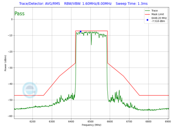
Plot 7-1472. LPI In-Band Emission Plot SDM Diversity Antenna 1b (160MHz 802.11ax RU996x2 (UNII Band 6) – Ch. 111)
