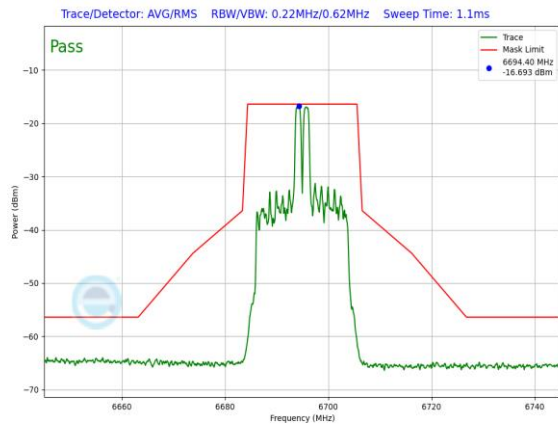
Plot 7-1475. LPI In-Band Emission Plot SDM Diversity Antenna 5T (20MHz 802.11ax RU26 (UNII Band 7) – Ch. 149)
