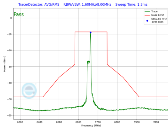
Plot 7-1500. LPI In-Band Emission Plot SDM Diversity Antenna 1b (160MHz 802.11ax RU26 (UNII Band 7) – Ch. 143)
