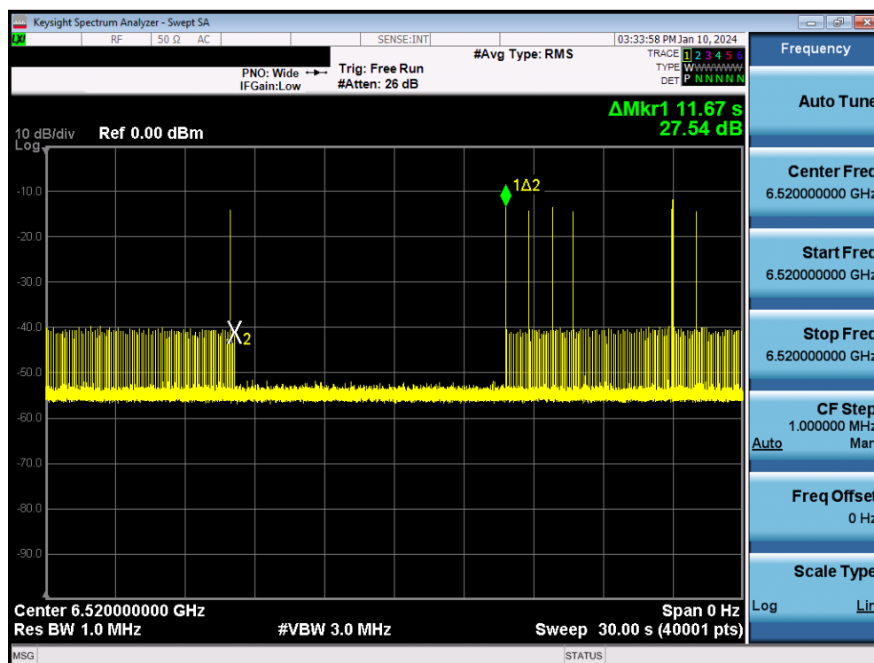
Plot 7-1560. Contention Based Protocol Timing Plot – UNII 6 – 160MHz Channel 111 – High
