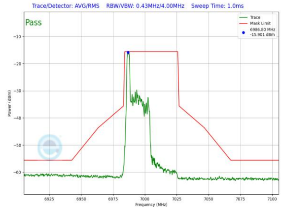
Plot 7-1514. LPI In-Band Emission Plot SDM Diversity Antenna 1b (40MHz 802.11ax RU26 (UNII Band 8) – Ch. 211)
