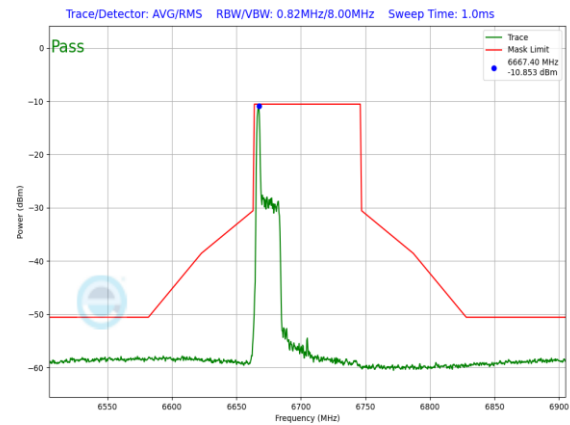
Plot 7-1490. LPI In-Band Emission Plot SDM Diversity Antenna 1b (80MHz 802.11ax RU26 (UNII Band 7) – Ch. 151)
