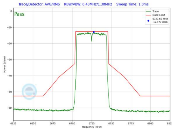
Plot 7-1487. LPI In-Band Emission Plot SDM Diversity Antenna 5T (40MHz 802.11ax RU484 (UNII Band 7) – Ch. 155)
