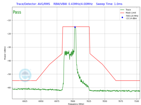
Plot 7-1516. LPI In-Band Emission Plot SDM Diversity Antenna 1b (40MHz 802.11ax RU26 (UNII Band 8) – Ch. 211)
