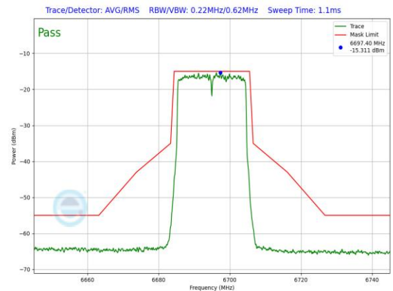
Plot 7-1479. LPI In-Band Emission Plot SDM Diversity Antenna 5T (20MHz 802.11ax RU242 (UNII Band 7) – Ch. 149)
