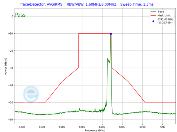
Plot 7-1502. LPI In-Band Emission Plot SDM Diversity Antenna 1b (160MHz 802.11ax RU26 (UNII Band 7) – Ch. 143)
