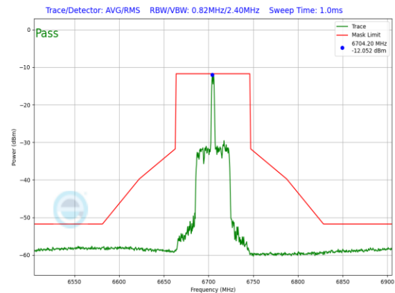
Plot 7-1491. LPI In-Band Emission Plot SDM Diversity Antenna 5T (80MHz 802.11ax RU26 (UNII Band 7) – Ch. 151)
