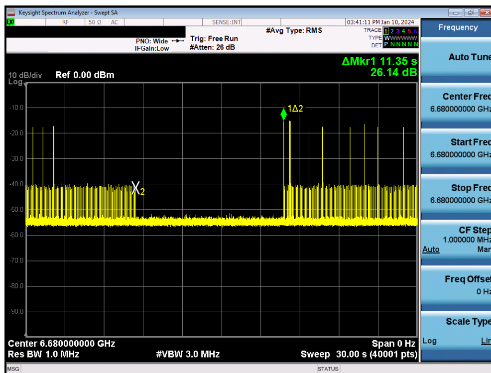
Plot 7-1562. Contention Based Protocol Timing Plot – UNII 7 – 160MHz Channel 143 – Low
