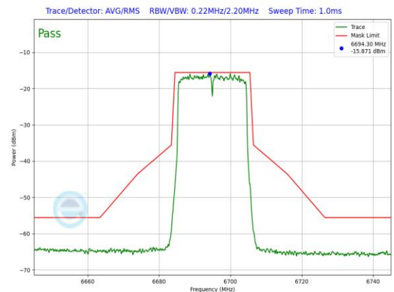
Plot 7-1480. LPI In-Band Emission Plot SDM Diversity Antenna 1b (20MHz 802.11ax RU242 (UNII Band 7) – Ch. 149)
