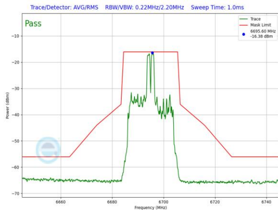
Plot 7-1476. LPI In-Band Emission Plot SDM Diversity Antenna 1b (20MHz 802.11ax RU26 (UNII Band 7) – Ch. 149)
