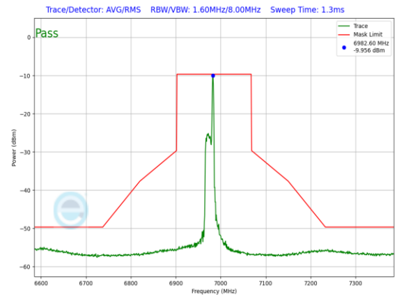
Plot 7-1532. LPI In-Band Emission Plot SDM Diversity Antenna 1b (160MHz 802.11ax RU26 (UNII Band 8) – Ch. 207)
