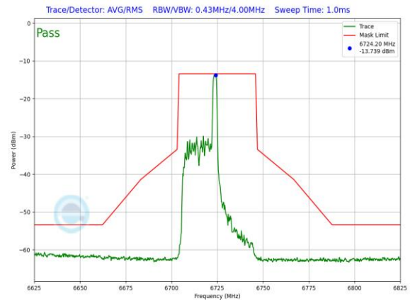
Plot 7-1484. LPI In-Band Emission Plot SDM Diversity Antenna 1b (40MHz 802.11ax RU26 (UNII Band 7) – Ch. 155)
