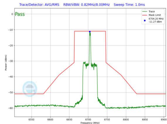
Plot 7-1492. LPI In-Band Emission Plot SDM Diversity Antenna 1b (80MHz 802.11ax RU26 (UNII Band 7) – Ch. 151)
