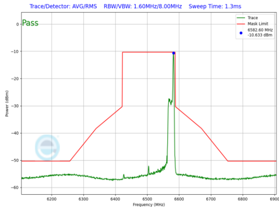
Plot 7-1470. LPI In-Band Emission Plot SDM Diversity Antenna 1b (160MHz 802.11ax RU26 (UNII Band 6) – Ch. 111)
