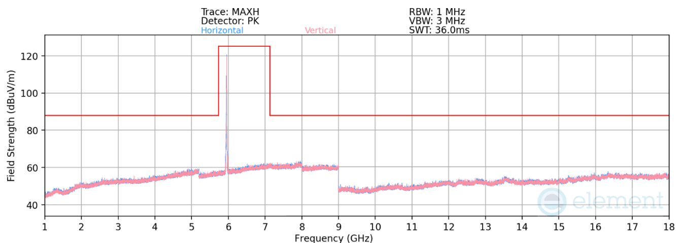
Plot 7-1621. Radiated Spurious Emissions above 1GHz Antenna 1b (802.11ax – Ch. 1 – RU26)
