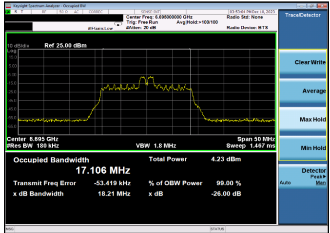
Plot 7-98. 26dB & 99% Bandwidth Plot Antenna 3b (20MHz 802.11ax RU26 (UNII Band 7) – Ch. 149)
