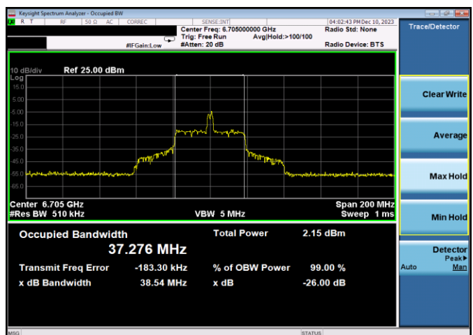
Plot 7-106. 26dB & 99% Bandwidth Plot Antenna 3b (80MHz 802.11ax RU26 (UNII Band 7) – Ch. 151)
