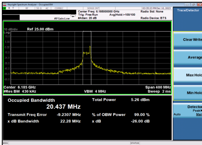
Plot 7-78. 26dB & 99% Bandwidth Plot Antenna 3b (160MHz 802.11ax RU26 (UNII Band 5) - Ch. 47)
