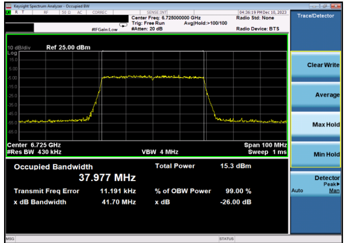
Plot 7-104. 26dB & 99% Bandwidth Plot Antenna 3b (40MHz 802.11ax RU484 (UNII Band 7) – Ch. 155)
