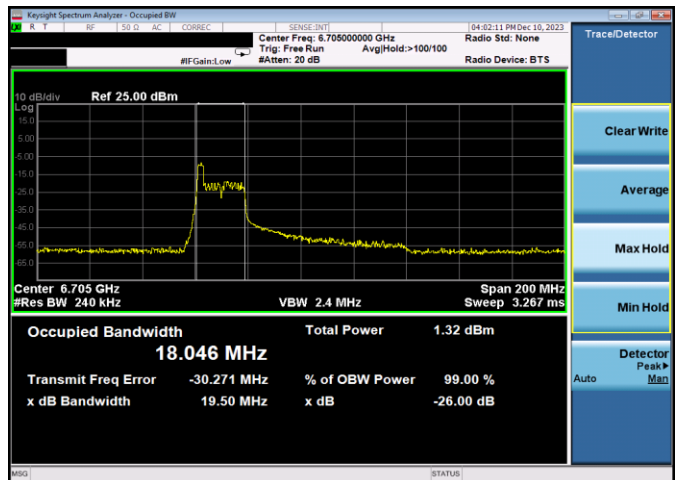
Plot 7-105. 26dB & 99% Bandwidth Plot Antenna 3b (80MHz 802.11ax RU26 (UNII Band 7) – Ch. 151)
