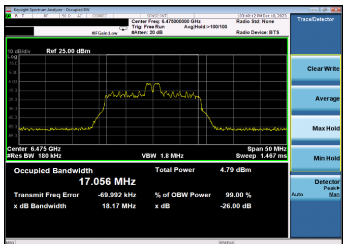
Plot 7-82. 26dB & 99% Bandwidth Plot Antenna 3b (20MHz 802.11ax RU26 (UNII Band 6) - Ch. 105)
