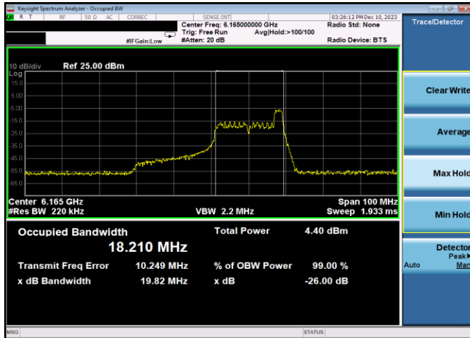
Plot 7-71. 26dB & 99% Bandwidth Plot Antenna 3b (40MHz 802.11ax RU26 (UNII Band 5) – Ch. 43)
