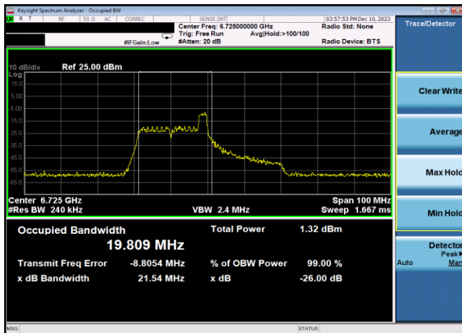
Plot 7-102. 26dB & 99% Bandwidth Plot Antenna 3b (40MHz 802.11ax RU26 (UNII Band 7) – Ch. 155)
