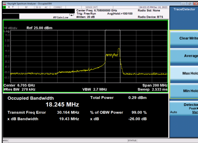
Plot 7-107. 26dB & 99% Bandwidth Plot Antenna 3b (80MHz 802.11ax RU26 (UNII Band 7) – Ch. 151)
