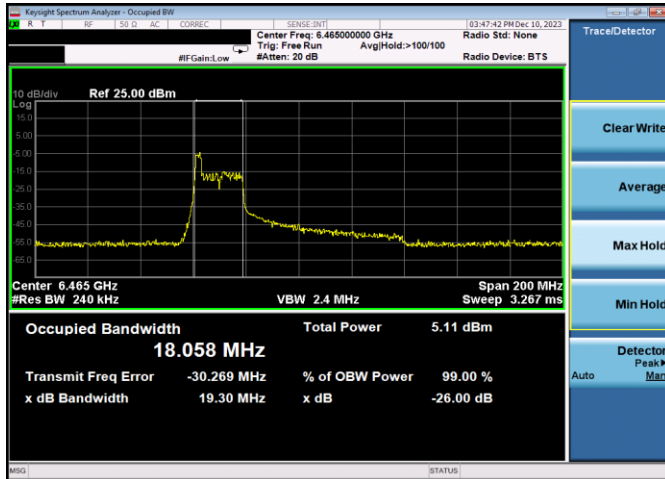
Plot 7-89. 26dB & 99% Bandwidth Plot Antenna 3b (80MHz 802.11ax RU26 (UNII Band 6) – Ch. 103)
