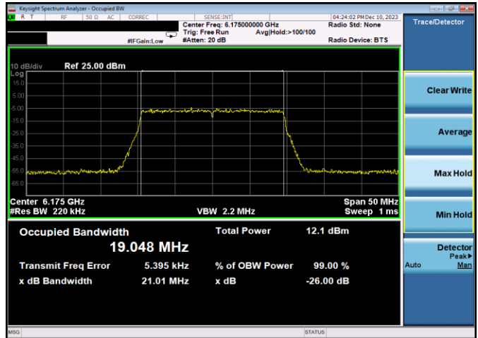
Plot 7-68. 26dB & 99% Bandwidth Plot Antenna 3b (20MHz 802.11ax RU242 (UNII Band 5) – Ch. 45)
