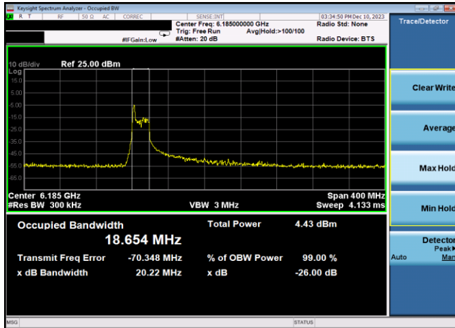
Plot 7-77. 26dB & 99% Bandwidth Plot Antenna 3b (160MHz 802.11ax RU26 (UNII Band 5) - Ch. 47)
