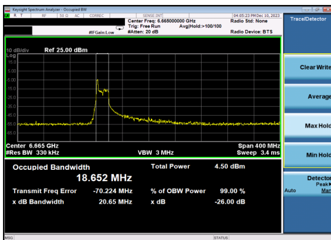
Plot 7-109. 26dB & 99% Bandwidth Plot Antenna 3b (160MHz 802.11ax RU26 (UNII Band 7) – Ch. 143)
