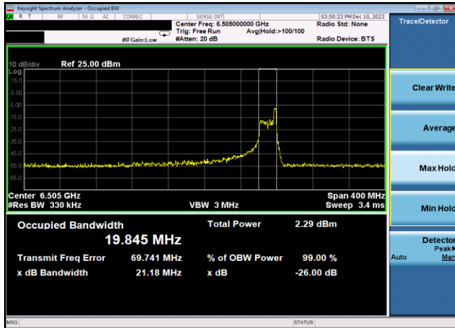
Plot 7-95. 26dB & 99% Bandwidth Plot Antenna 3b (160MHz 802.11ax RU26 (UNII Band 6) – Ch. 111)
