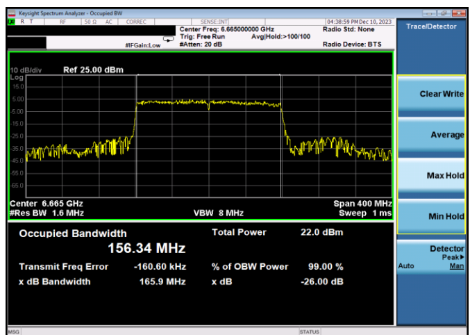
Plot 7-112. 26dB & 99% Bandwidth Plot Antenna 3b (160MHz 802.11ax RU484 (UNII Band 7) – Ch. 143)
