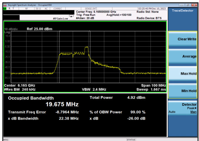
Plot 7-70. 26dB & 99% Bandwidth Plot Antenna 3b (40MHz 802.11ax RU26 (UNII Band 5) – Ch. 43)
