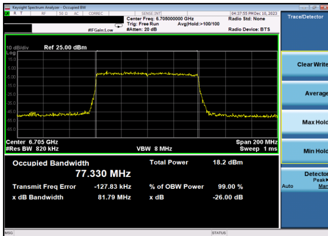
Plot 7-108. 26dB & 99% Bandwidth Plot Antenna 3b (80MHz 802.11ax RU996 (UNII Band 7) – Ch. 151)
