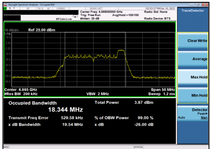
Plot 7-99. 26dB & 99% Bandwidth Plot Antenna 3b (20MHz 802.11ax RU26 (UNII Band 7) – Ch. 149)
