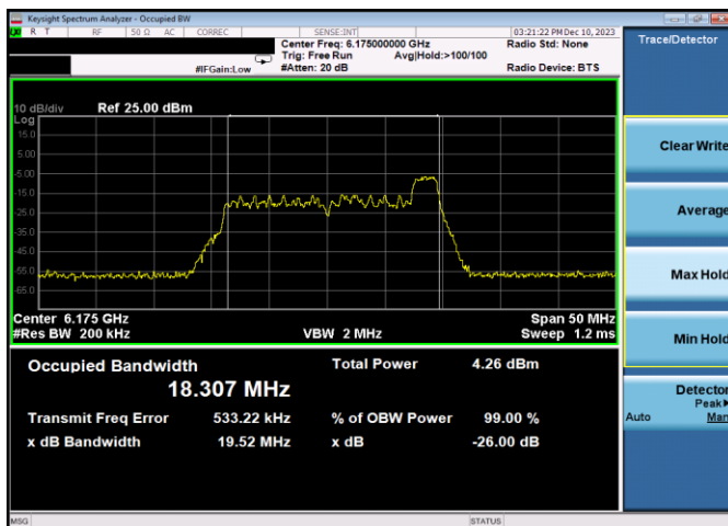
Plot 7-67. 26dB & 99% Bandwidth Plot Antenna 3b (20MHz 802.11ax RU26 (UNII Band 5) – Ch. 45)
