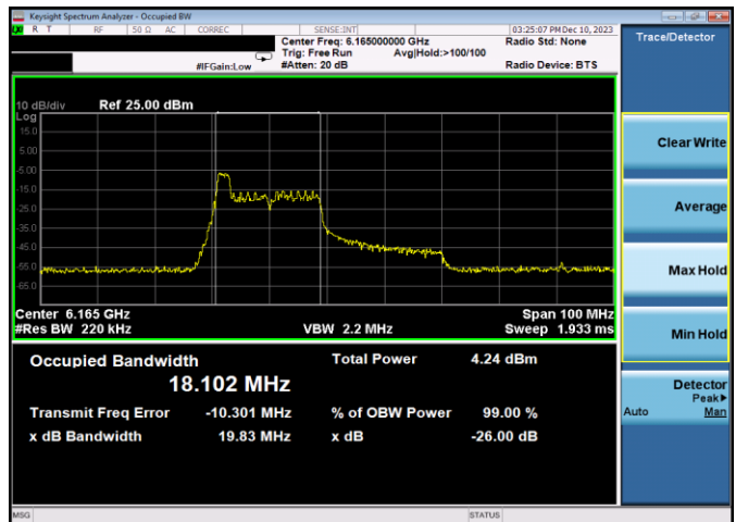
Plot 7-69. 26dB & 99% Bandwidth Plot Antenna 3b (40MHz 802.11ax RU26 (UNII Band 5) – Ch. 43)
