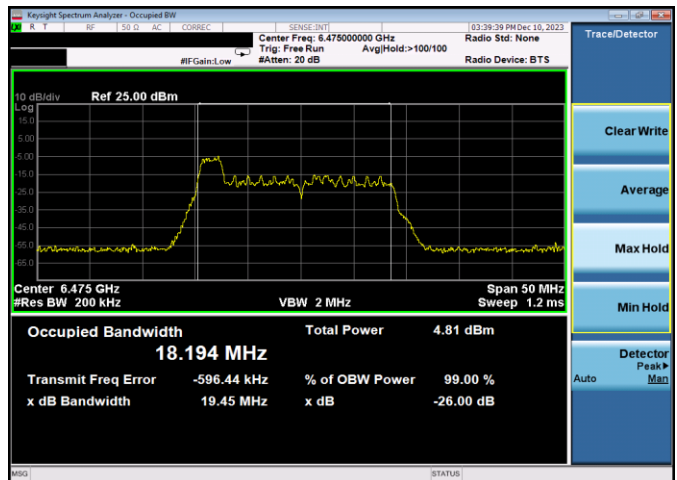
Plot 7-81. 26dB & 99% Bandwidth Plot Antenna 3b (20MHz 802.11ax RU26 (UNII Band 6) - Ch. 105)
