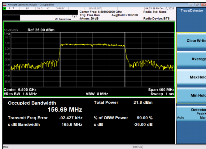
Plot 7-96. 26dB & 99% Bandwidth Plot Antenna 3b (160MHz 802.11ax RU996x2 (UNII Band 6) – Ch. 111)
