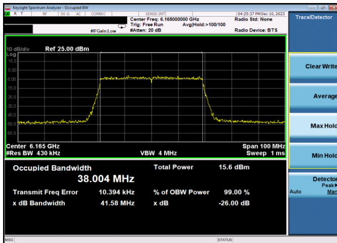
Plot 7-72. 26dB & 99% Bandwidth Plot Antenna 3b (40MHz 802.11ax RU484 (UNII Band 5) – Ch. 43)
