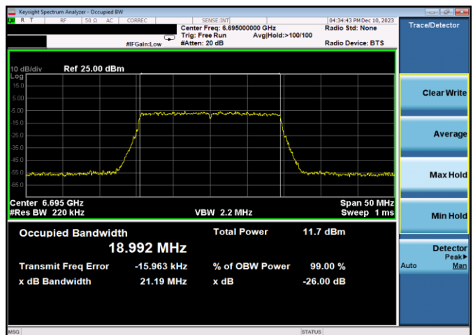
Plot 7-100. 26dB & 99% Bandwidth Plot Antenna 3b (20MHz 802.11ax RU242 (UNII Band 7) – Ch. 149)
