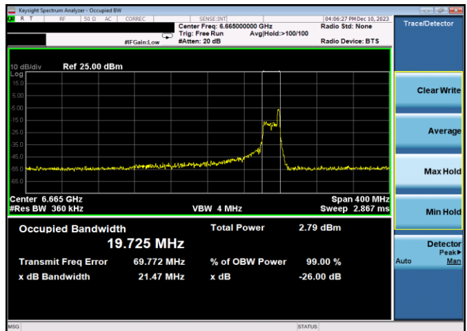
Plot 7-111. 26dB & 99% Bandwidth Plot Antenna 3b (160MHz 802.11ax RU26 (UNII Band 7) – Ch. 143)
