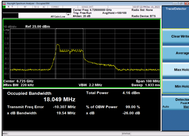
Plot 7-101. 26dB & 99% Bandwidth Plot Antenna 3b (40MHz 802.11ax RU26 (UNII Band 7) – Ch. 155)
