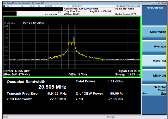
Plot 7-110. 26dB & 99% Bandwidth Plot Antenna 3b (160MHz 802.11ax RU26 (UNII Band 7) – Ch. 143)
