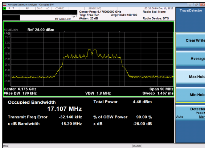
Plot 7-66. 26dB & 99% Bandwidth Plot Antenna 3b (20MHz 802.11ax RU26 (UNII Band 5) – Ch. 45)
