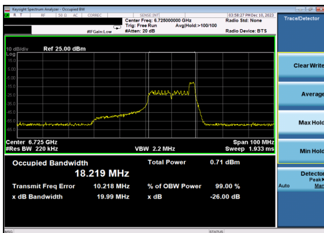
Plot 7-103. 26dB & 99% Bandwidth Plot Antenna 3b (40MHz 802.11ax RU26 (UNII Band 7) – Ch. 155)
