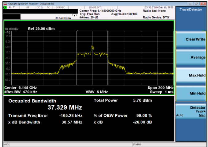
Plot 7-74. 26dB & 99% Bandwidth Plot Antenna 3b (80MHz 802.11ax RU26 (UNII Band 5) – Ch. 39)
