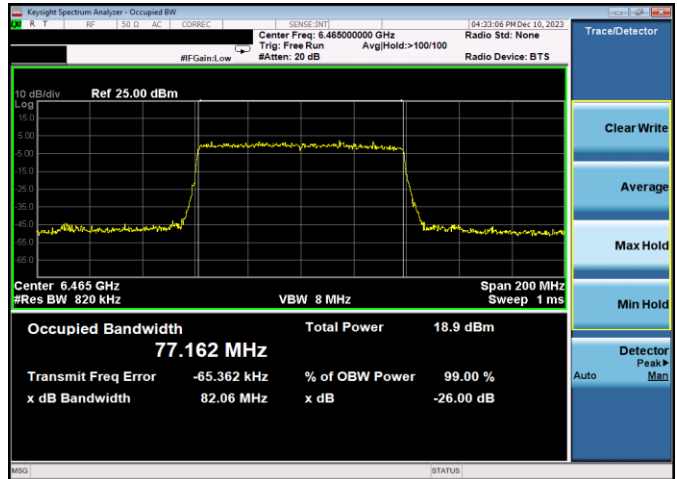
Plot 7-92. 26dB & 99% Bandwidth Plot Antenna 3b (80MHz 802.11ax RU96 (UNII Band 6) – Ch. 103)
