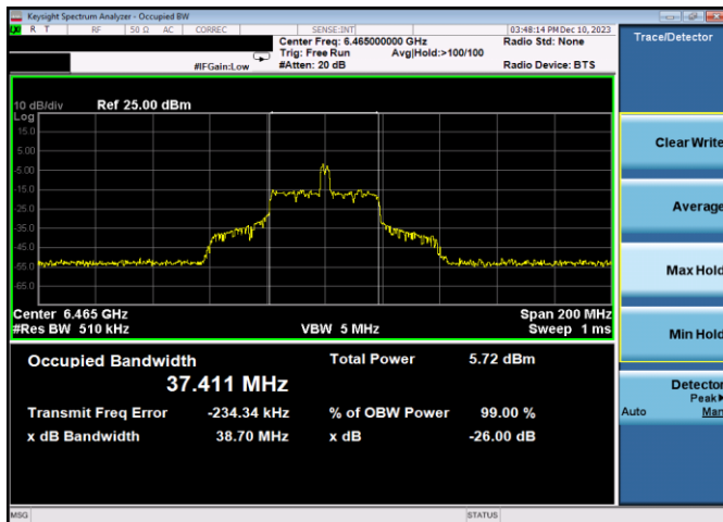
Plot 7-90. 26dB & 99% Bandwidth Plot Antenna 3b (80MHz 802.11ax RU26 (UNII Band 6) – Ch. 103)
