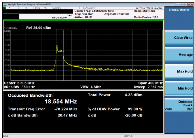
Plot 7-93. 26dB & 99% Bandwidth Plot Antenna 3b (160MHz 802.11ax RU26 (UNII Band 6) – Ch. 111)
