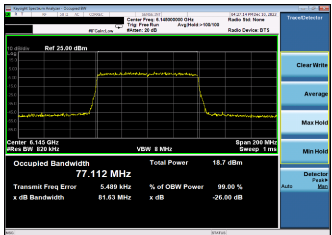
Plot 7-76. 26dB & 99% Bandwidth Plot Antenna 3b (80MHz 802.11ax RU996 (UNII Band 5) – Ch. 39)
