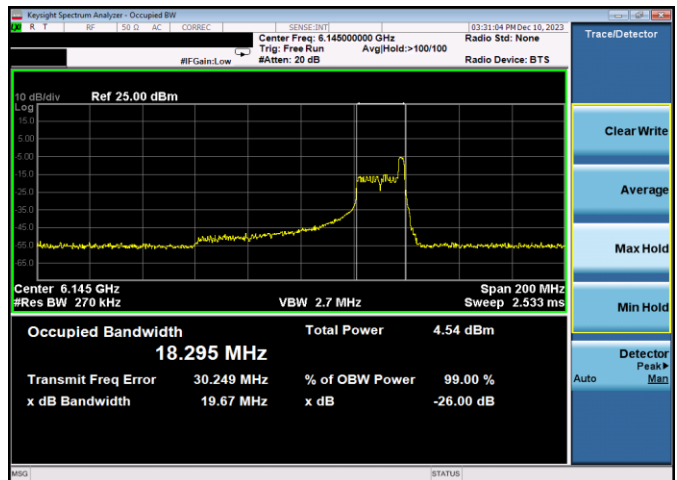
Plot 7-75. 26dB & 99% Bandwidth Plot Antenna 3b (80MHz 802.11ax RU26 (UNII Band 5) – Ch. 39)
