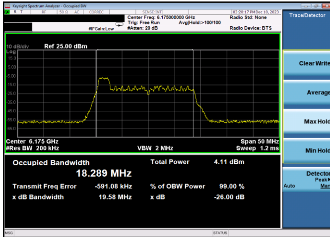
Plot 7-65. 26dB & 99% Bandwidth Plot Antenna 3b (20MHz 802.11ax RU26 (UNII Band 5) – Ch. 45)
