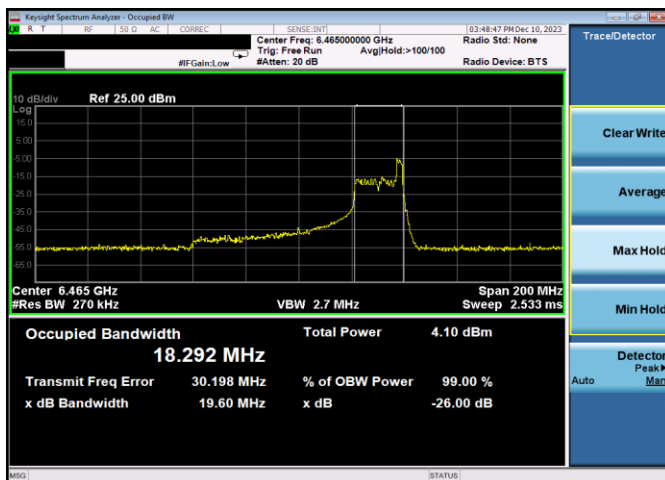
Plot 7-91. 26dB & 99% Bandwidth Plot Antenna 3b (80MHz 802.11ax RU26 (UNII Band 6) – Ch. 103)
