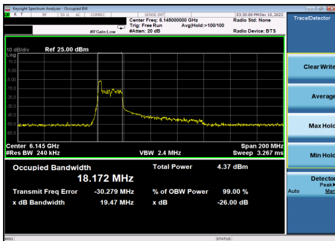
Plot 7-73. 26dB & 99% Bandwidth Plot Antenna 3b (80MHz 802.11ax RU26 (UNII Band 5) – Ch. 39)
