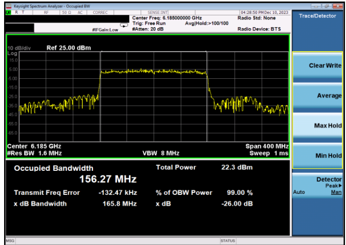
Plot 7-80. 26dB & 99% Bandwidth Plot Antenna 3b (160MHz 802.11ax RU996x2 (UNII Band 5) - Ch. 47)
