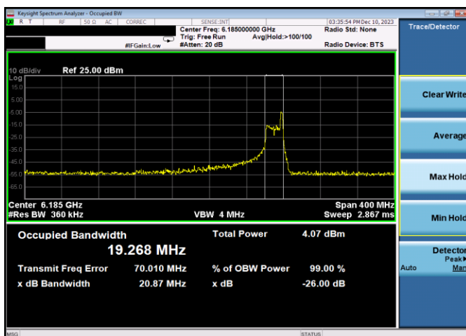
Plot 7-79. 26dB & 99% Bandwidth Plot Antenna 3b (160MHz 802.11ax RU26 (UNII Band 5) - Ch. 47)
