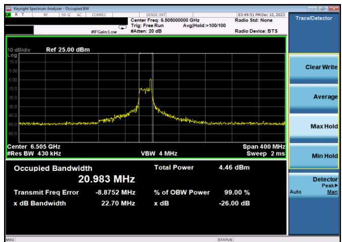
Plot 7-94. 26dB & 99% Bandwidth Plot Antenna 3b (160MHz 802.11ax RU26 (UNII Band 6) – Ch. 111)
