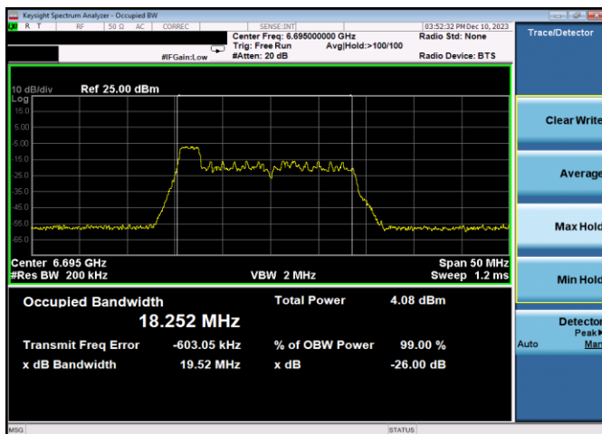
Plot 7-97. 26dB & 99% Bandwidth Plot Antenna 3b (20MHz 802.11ax RU26 (UNII Band 7) – Ch. 149)
