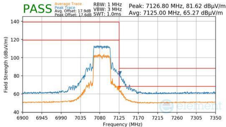
Plot 7-1778. SDM Primary Radiated Upper Band Edge (Peak & Average – UNII Band 8 – RU484)
