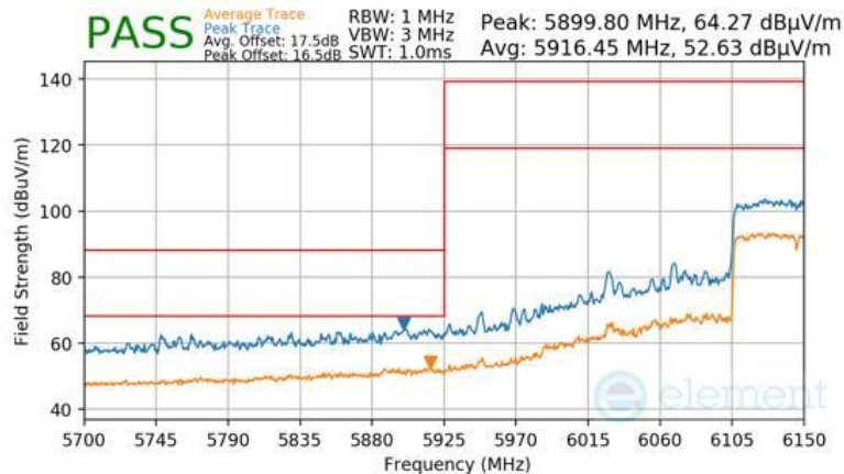
Plot 7-1747. Antenna 3b Radiated Lower Band Edge (Peak & Average – UNII Band 5 – RU996x2)
