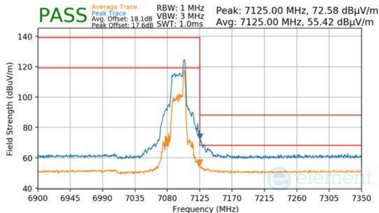
Plot 7-1710. Antenna 5T Radiated Upper Band Edge (Peak/Average – UNII Band 8 – RU26)
