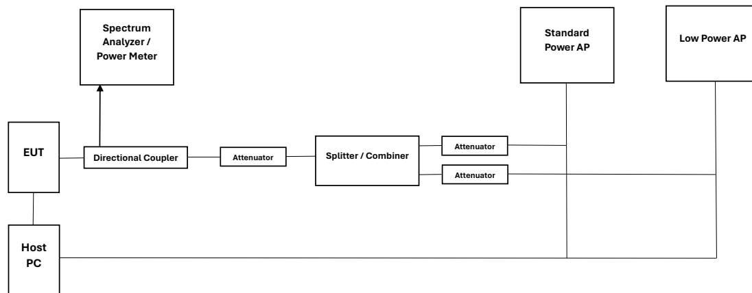
Figure 7-9. Test Instrument & Measurement Setup
