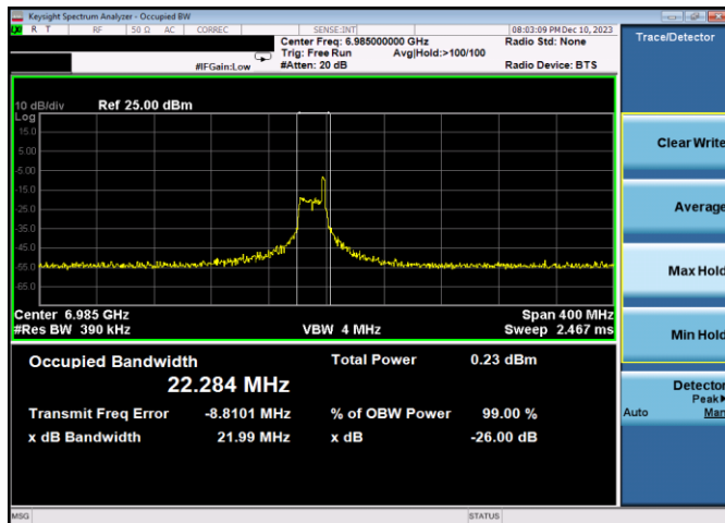
Plot 7-190. 26dB & 99% Bandwidth Plot Antenna 1b (160MHz 802.11ax RU26 (UNII Band 8) – Ch. 207)
