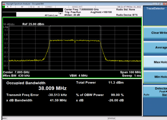
Plot 7-184. 26dB & 99% Bandwidth Plot Antenna 1b (40MHz 802.11ax RU484 (UNII Band 8) – Ch. 211)
