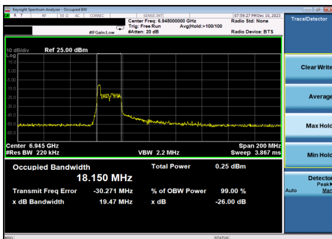
Plot 7-185. 26dB & 99% Bandwidth Plot Antenna 1b (80MHz 802.11ax RU26 (UNII Band 8) – Ch. 199)
