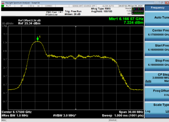
Plot 7-290. SP Power Spectral Density Plot CDD Primary Antenna 3b (20MHz 802.11ax RU26 (UNII Band 5) – Ch. 45)
