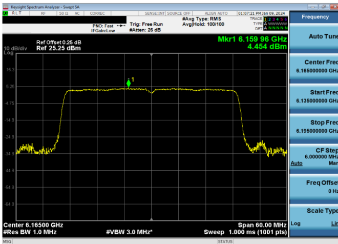
Plot 7-303. SP Power Spectral Density Plot CDD Primary Antenna 5T (40MHz 802.11ax RU484 (UNII Band 5) – Ch. 43)
