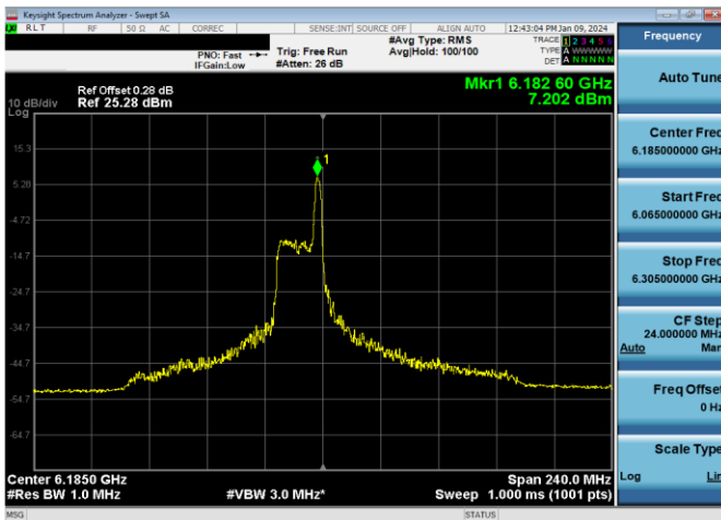
Plot 7-315. SP Power Spectral Density Plot CDD Primary Antenna 5T (160MHz 802.11ax RU26 (UNII Band 5) – Ch. 47)
