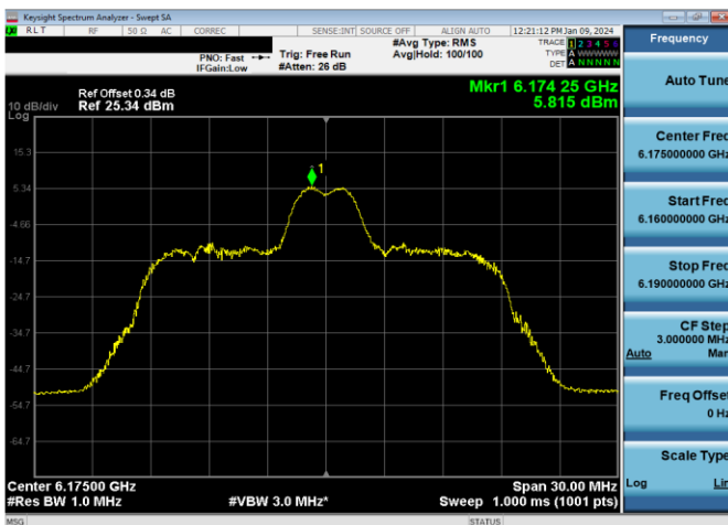
Plot 7-291. SP Power Spectral Density Plot CDD Primary Antenna 5T (20MHz 802.11ax RU26 (UNII Band 5) – Ch. 45)
