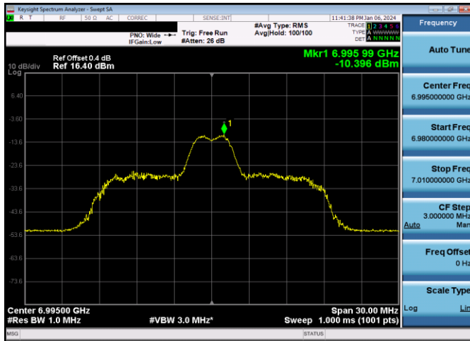
Plot 7-530. LPI Power Spectral Density Plot Antenna 3b (20MHz 802.11ax RU26 (UNII Band 8) – Ch. 209)
