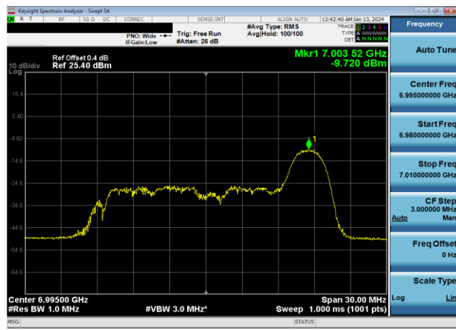
Plot 7-531. LPI Power Spectral Density Plot Antenna 3b (20MHz 802.11ax RU26 (UNII Band 8) – Ch. 209)
