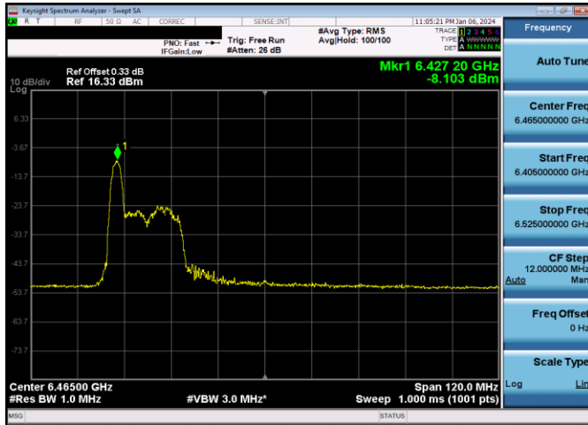
Plot 7-505. LPI Power Spectral Density Plot Antenna 3b (80MHz 802.11ax RU26 (UNII Band 6) – Ch. 103)
