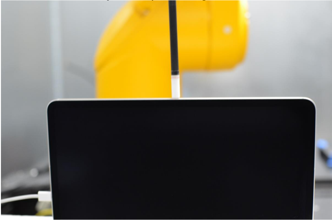
Near Field Power Density Test Setup 23: Left Edge at 2mm – Antenna 1b/3b/5T
