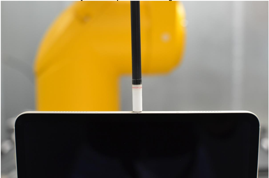
Near Field Power Density Test Setup 20: Bottom Edge at 2mm – Antenna 1b/3b/5T
