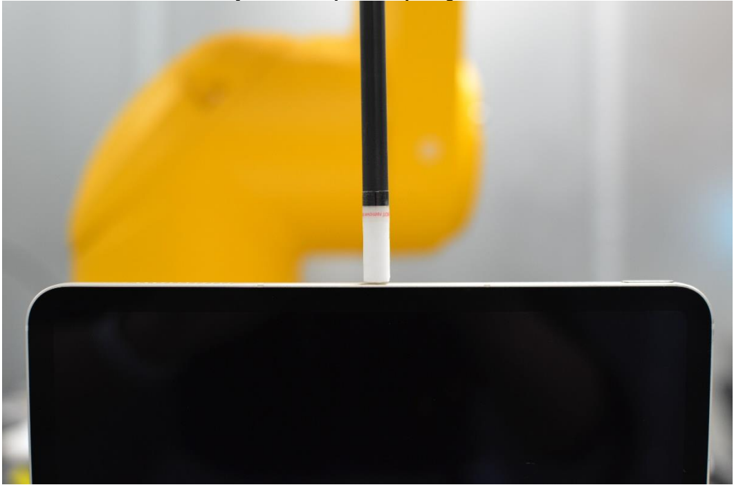
Near Field Power Density Test Setup 19: Top Edge at 2mm – Antenna 1b/3b/5T
