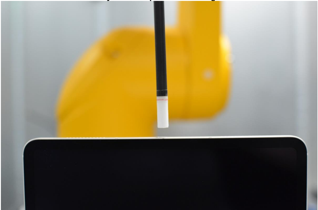
Near Field Power Density Test Setup 21: Bottom Edge at 9mm – Antenna 1b
