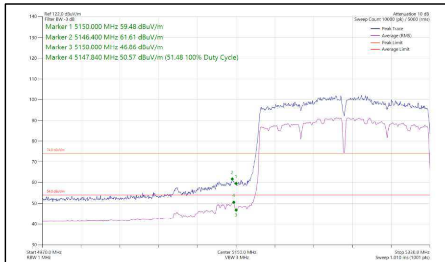
Figure 151 - 802.11ac, VHT160, SDM, Core 0-1 - 5250 MHz, Band Edge Frequency 5150 MHz
