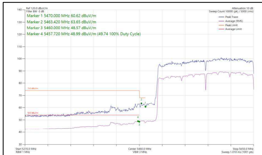
Figure 140 - 802.11ax, HE160, SU, SISO, Core 1 - 5570 MHz, Band Edge Frequency 5460 MHz
