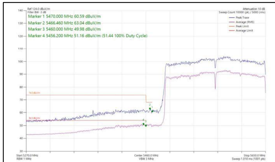
Figure 149 - 802.11ax, HE160, SU, CDD, Core 0-1 - 5570 MHz, Band Edge Frequency 5460 MHz
