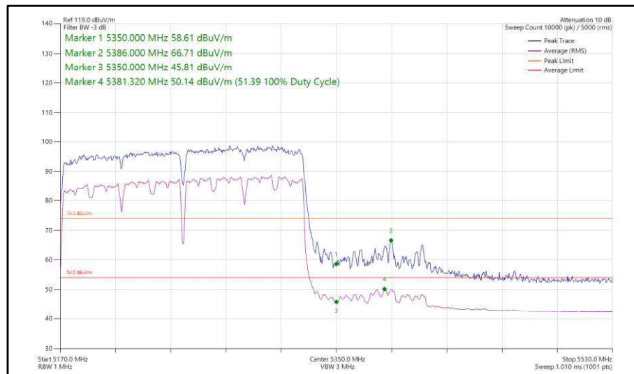
Figure 154 - 802.11ac, VHT160, SDM, Core 0-1 - 5250 MHz, Band Edge Frequency 5350 MHz
