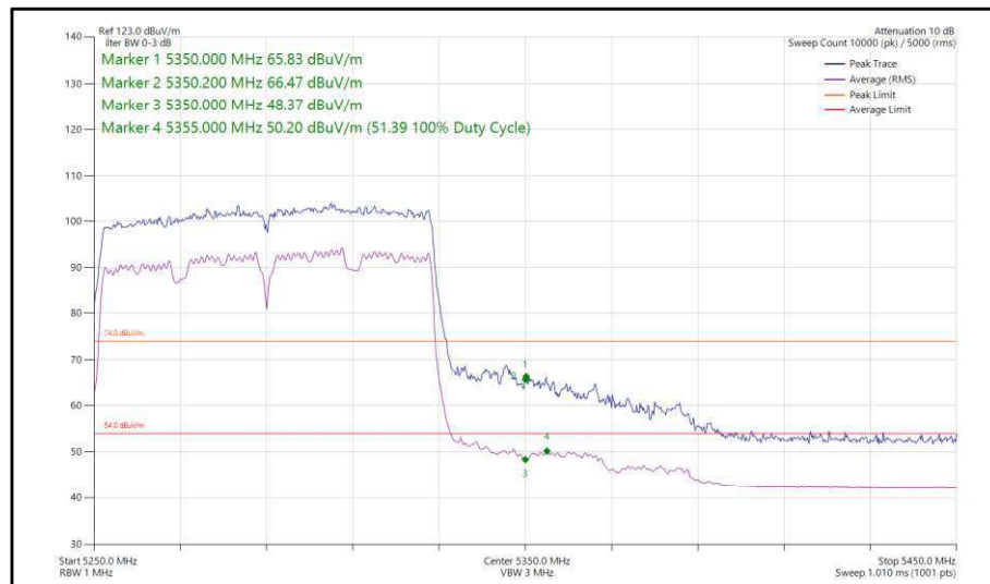
Figure 115 - 802.11ac, VHT80, SDM, Core 0-1 - 5290 MHz, Band Edge Frequency 5350 MHz
