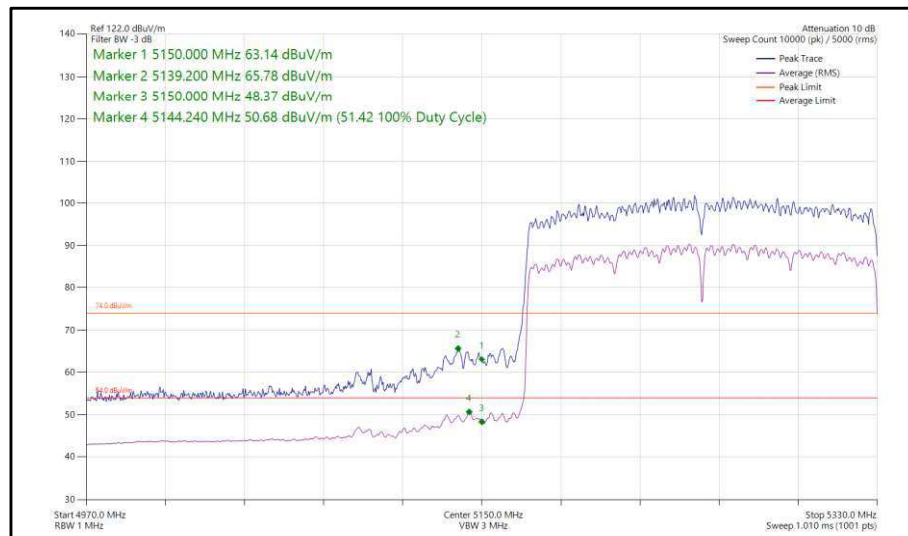
Figure 143 - 802.11ax, HE160, SU, CDD, Core 0-1 - 5250 MHz, Band Edge Frequency 5150 MHz
