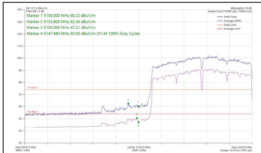
Figure 133 - 802.11ac, VHT160, SISO, Core 1 - 5250 MHz, Band Edge Frequency 5150 MHz
