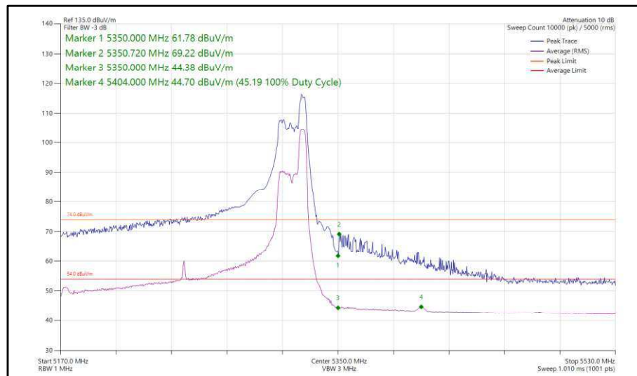
Figure 129 - 802.11ax, HE160, RU 52-52, SISO, Core 0 - 5250 MHz, Band Edge Frequency 5350 MHz
