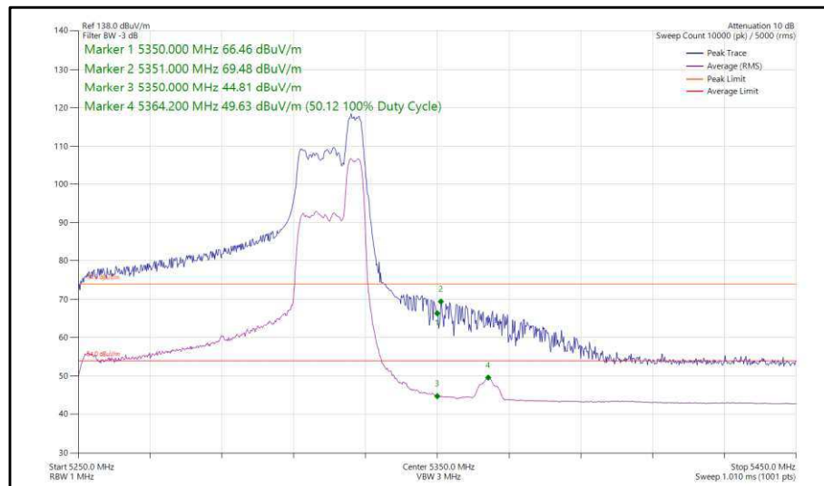
Figure 117 - 802.11ax, HE80, RU 52-52, SDM, Core 0-1 - 5290 MHz, Band Edge Frequency 5350 MHz
