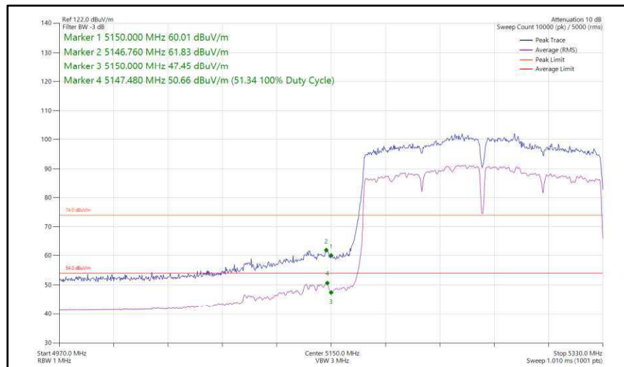
Figure 142 - 802.11ac, VHT160, CDD, Core 0-1 - 5250 MHz, Band Edge Frequency 5150 MHz
