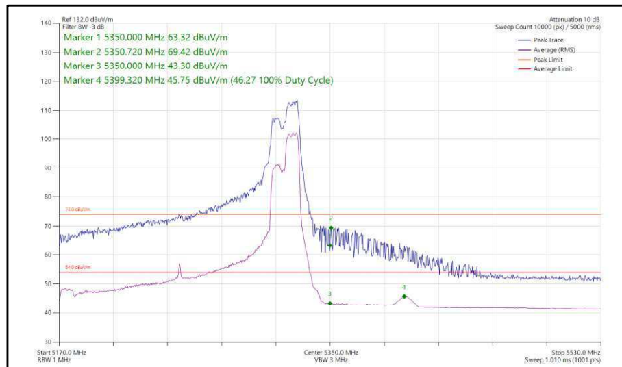
Figure 156 - 802.11ax, HE160, RU 106-60, SDM, Core 0-1 - 5250 MHz, Band Edge Frequency 5350 MHz
