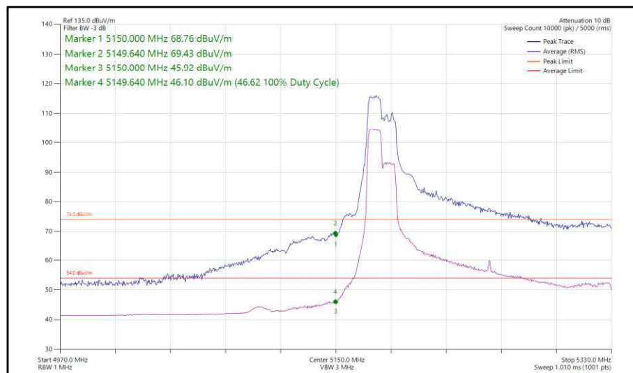
Figure 126 - 802.11ax, HE160, RU 106-53, SISO, Core 0 - 5250 MHz, Band Edge Frequency 5150 MHz
