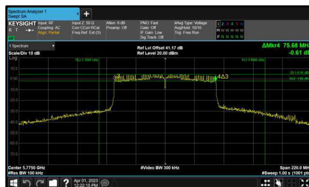
Figure 167 - 802.11ac VHT80 Maximum 6 dB EBW
