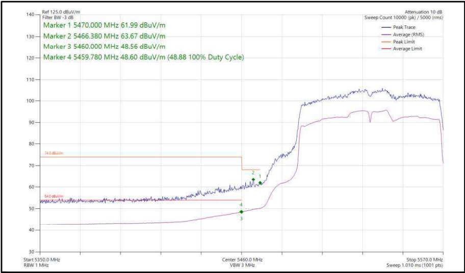
Figure 123 - 802.11ac, VHT80, TxBF, Core 0-1 - 5530 MHz, Band Edge Frequency 5460 MHz
