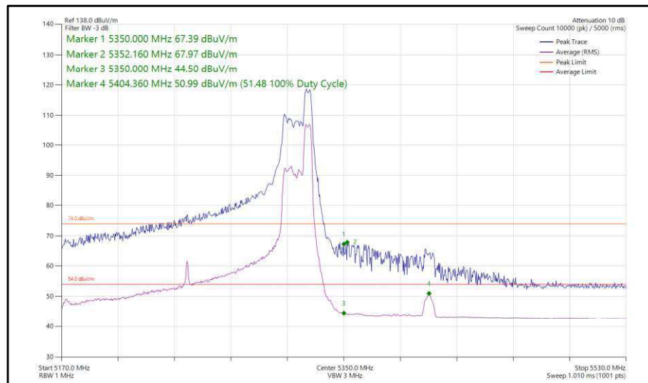
Figure 147 - 802.11ax, HE160, RU 52-52, CDD, Core 0-1 - 5250 MHz, Band Edge Frequency 5350 MHz
