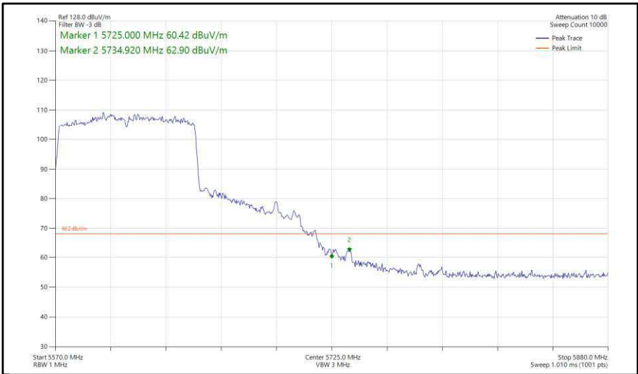
Figure 453 - 802.11ac, VHT80, SISO, Core 1 - 5610 MHz, Band Edge Frequency 5725 MHz
