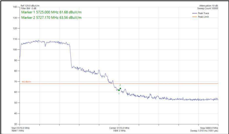
Figure 468 - 802.11ac, VHT80, CDD, Core 0-1 - 5610 MHz, Band Edge Frequency 5725 MHz
