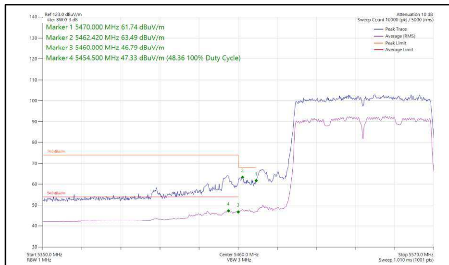
Figure 432 - 802.11ac, VHT80, SISO, Core 0 - 5530 MHz, Band Edge Frequency 5470 MHz
