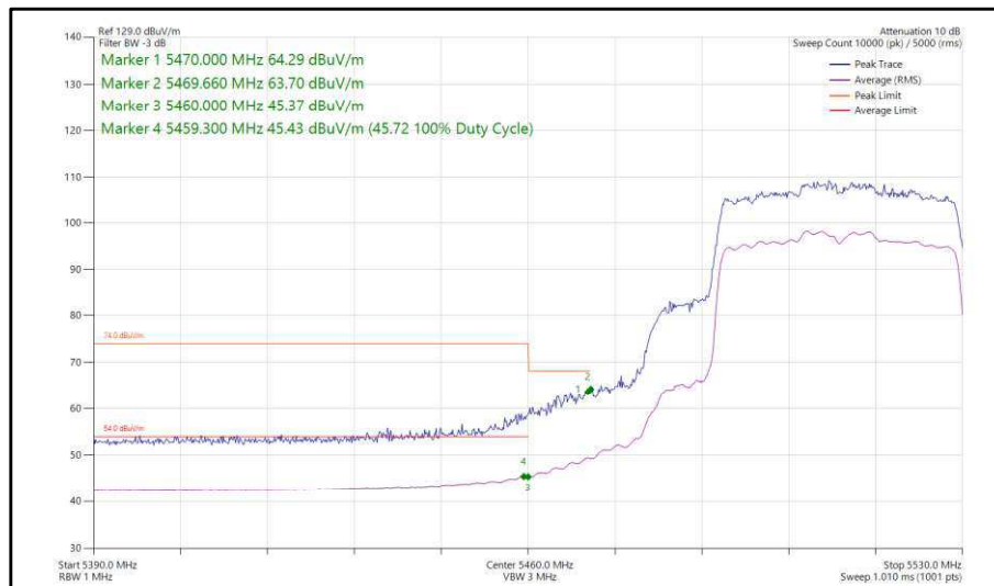
Figure 386 - 802.11ax, HE40, SU, CDD, Core 0-1 - 5510 MHz, Band Edge Frequency 5470 MHz
