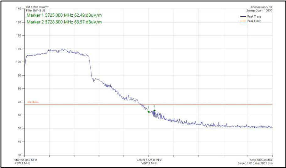
Figure 359 - 802.11ax, HE40, SU, SISO, Core 0 - 5670 MHz, Band Edge Frequency 5725 MHz
