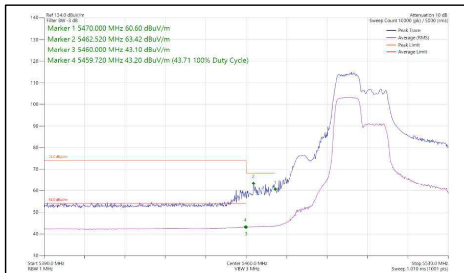
Figure 351 - 802.11ax, HE40, RU 106-53, SISO, Core 0 - 5510 MHz, Band Edge Frequency 5470 MHz
