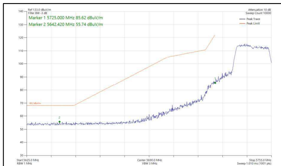
Figure 345 - 802.11n, HT20, TxBF, Core 0-1 - 5745 MHz, Band Edge Frequency 5725 MHz
