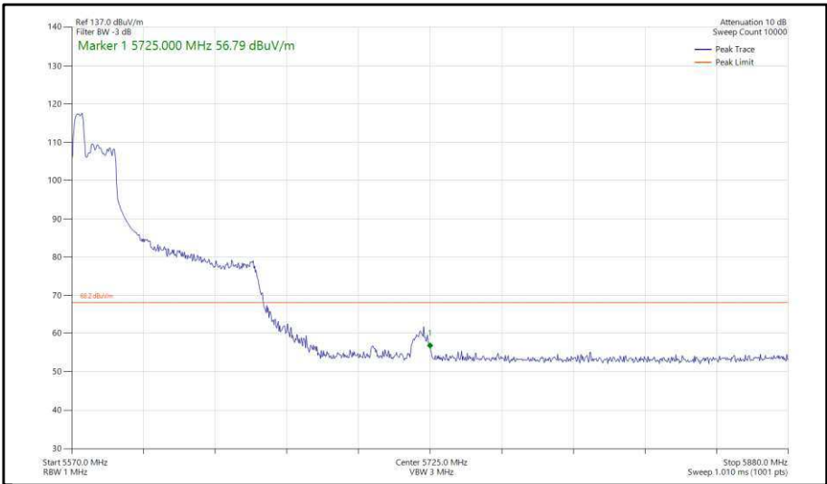
Figure 455 - 802.11ax, HE80, RU 52-37, SISO, Core 1 - 5610 MHz, Band Edge Frequency 5725 MHz
