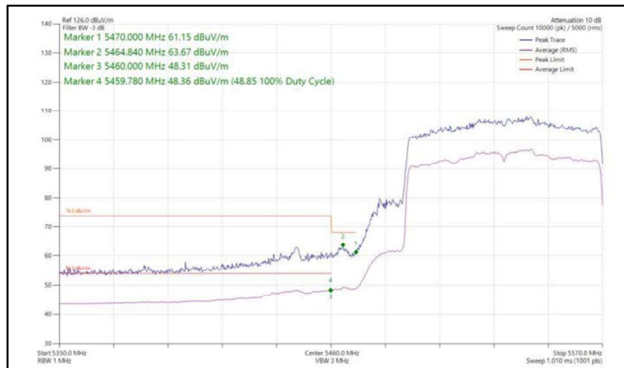
Figure 478 - 802.11ax, HE80, SU, SDM, Core 0-1 - 5530 MHz, Band Edge Frequency 5470 MHz
