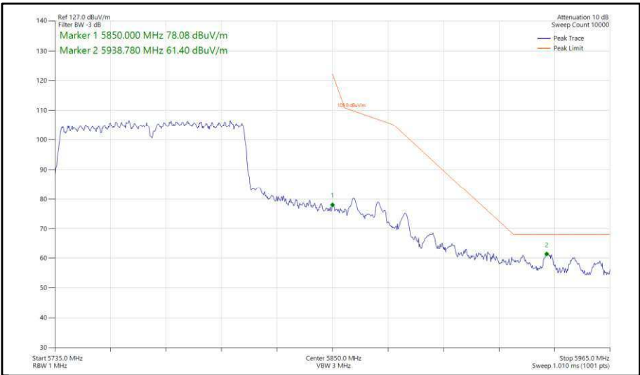
Figure 472 - 802.11ac, VHT80, CDD, Core 0-1 - 5775 MHz, Band Edge Frequency 5850 MHz
