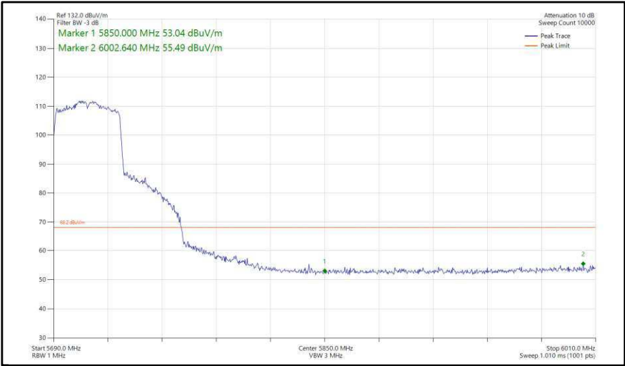
Figure 417 - 802.11ax, HE40, SU, SDM, Core 0-1 - 5710 MHz, Band Edge Frequency 5850 MHz
