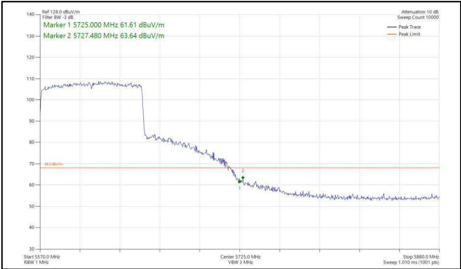
Figure 454 - 802.11ax, HE80, SU, SISO, Core 1 - 5610 MHz, Band Edge Frequency 5725 MHz
