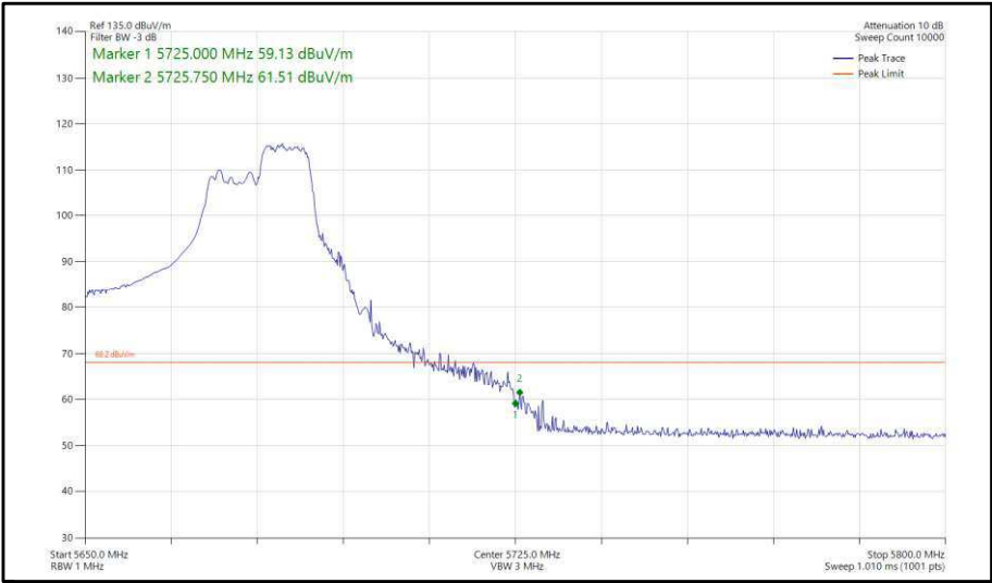
Figure 414 - 802.11ax, HE40, RU 106-56, SDM, Core 0-1 - 5670 MHz, Band Edge Frequency 5725 MHz
