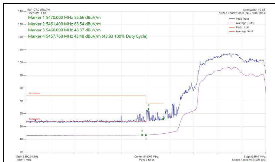
Figure 422 - 802.11ax, HE40, SU, TxBF, Core 0-1 - 5510 MHz, Band Edge Frequency 5470 MHz
