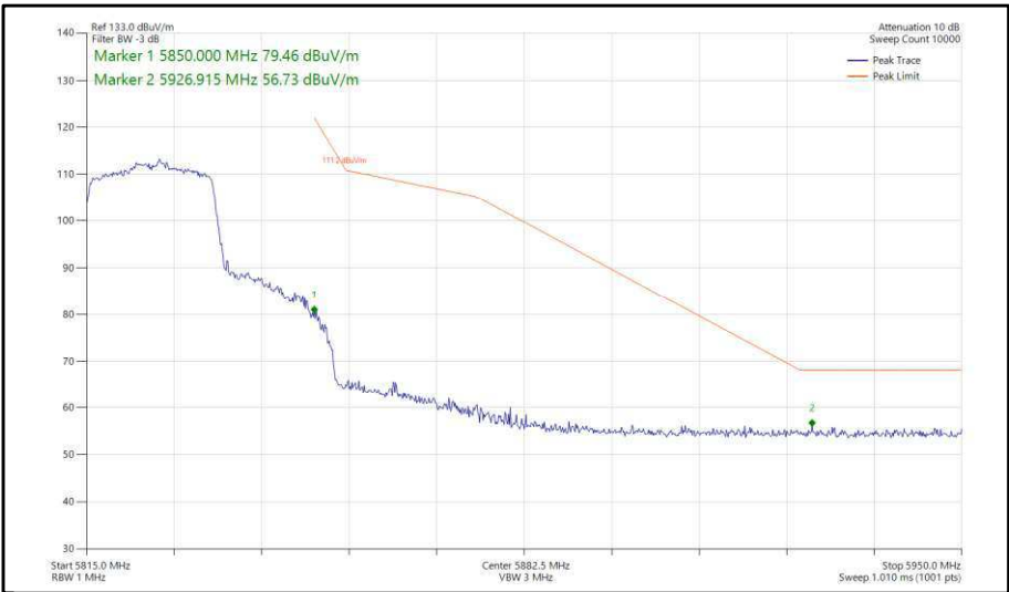
Figure 342 - 802.11ax, HE20, SU, SDM, Core 0-1 - 5825 MHz, Band Edge Frequency 5850 MHz
