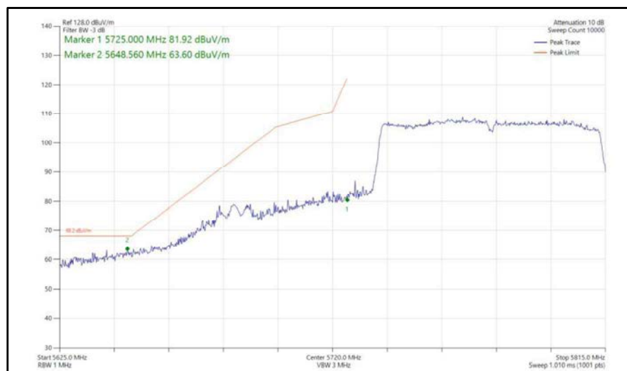
Figure 493 - 802.11ac, VHT80, TxBF, Core 0-1 - 5775 MHz, Band Edge Frequency 5725 MHz
