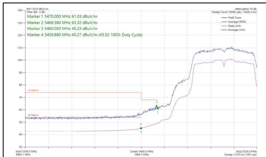
Figure 367 - 802.11n, HT40, SISO, Core 1 - 5510 MHz, Band Edge Frequency 5470 MHz
