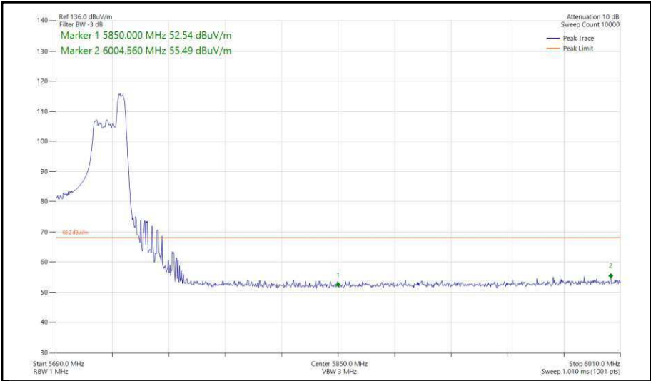
Figure 364 - 802.11ax, HE40, RU 52-44, SISO, Core 0 - 5710 MHz, Band Edge Frequency 5850 MHz
