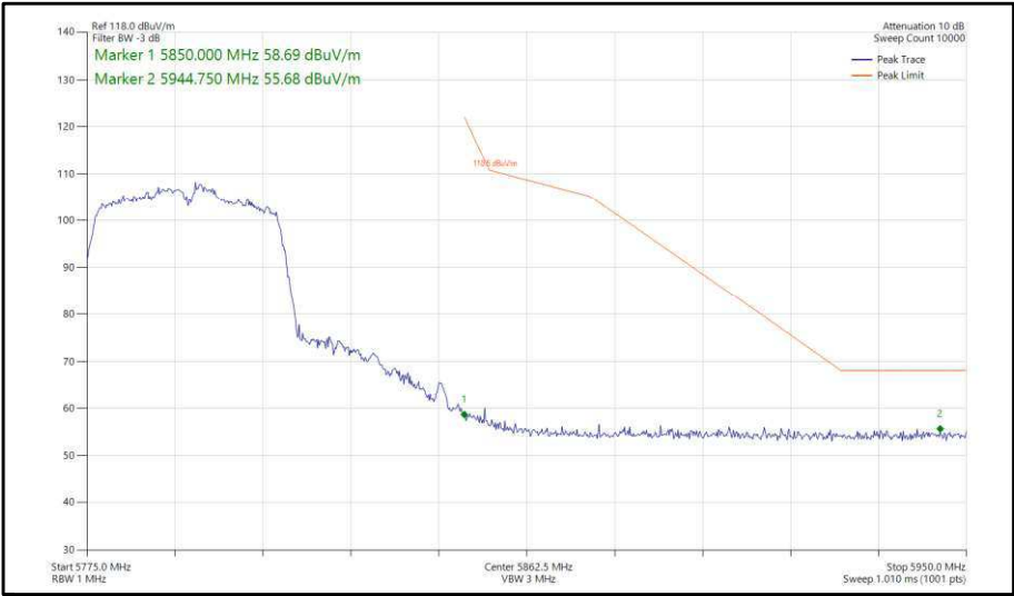
Figure 362 - 802.11n, HT40, SISO, Core 0 - 5795 MHz, Band Edge Frequency 5850 MHz
