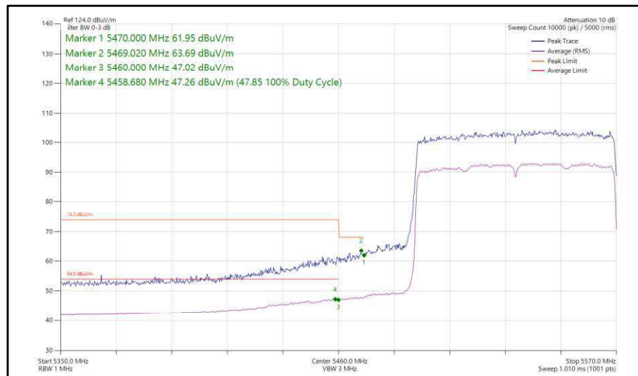
Figure 433 - 802.11ax, HE80, SU, SISO, Core 0 - 5530 MHz, Band Edge Frequency 5470 MHz
