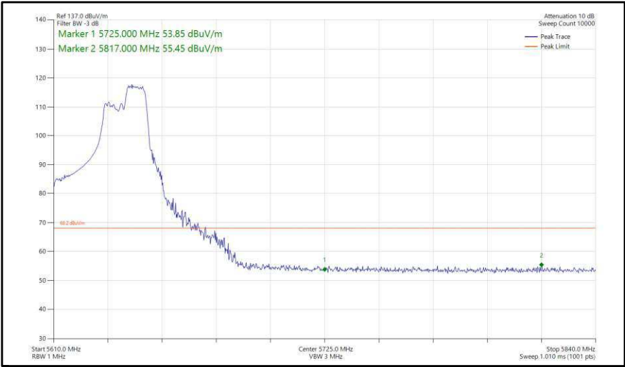
Figure 376 - 802.11ax, HE40, RU 106-56, SISO, Core 1 - 5630 MHz, Band Edge Frequency 5725 MHz
