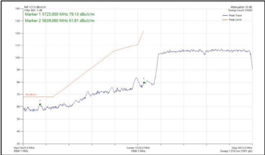
Figure 465 - 802.11ac, VHT80, CDD, Core 0-1 - 5775 MHz, Band Edge Frequency 5725 MHz
