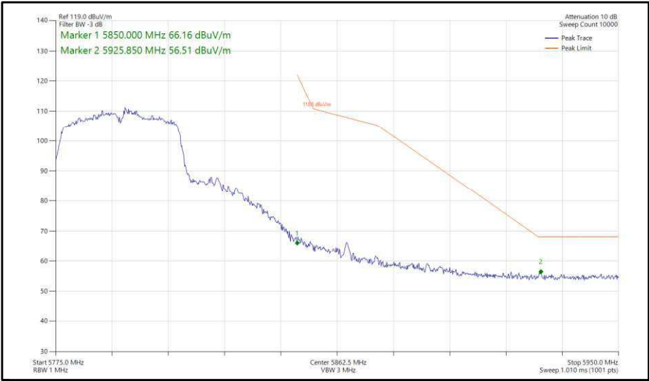
Figure 380 - 802.11n, HT40, SISO, Core 1 - 5795 MHz, Band Edge Frequency 5850 MHz
