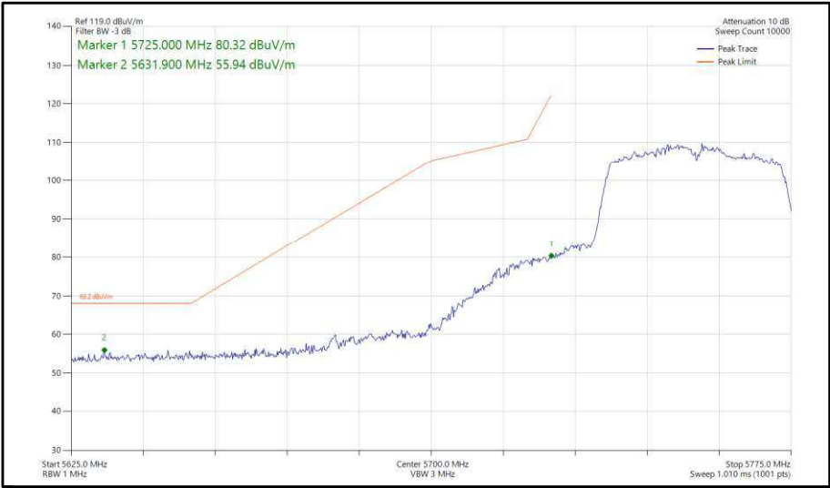
Figure 370 - 802.11n, HT40, SISO, Core 1 - 5755 MHz, Band Edge Frequency 5725 MHz
