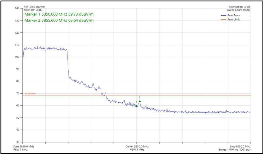
Figure 456 - 802.11ac, VHT80, SISO, Core 1 - 5690 MHz, Band Edge Frequency 5850 MHz
