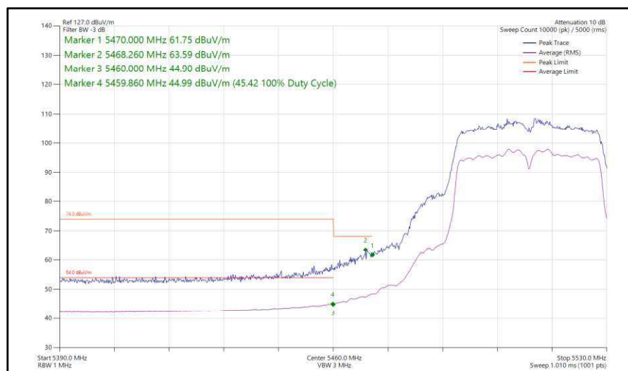
Figure 385 - 802.11n, HT40, CDD, Core 0-1 - 5510 MHz, Band Edge Frequency 5470 MHz
