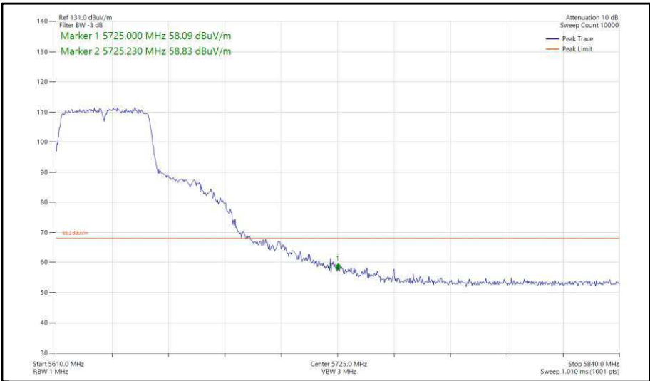
Figure 373 - 802.11n, HT40, SISO, Core 1 - 5630 MHz, Band Edge Frequency 5725 MHz
