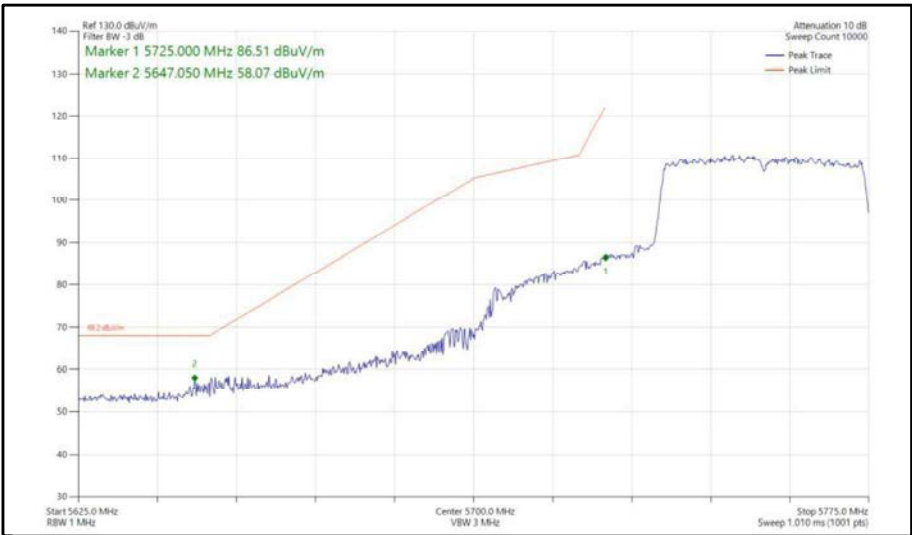
Figure 407 - 802.11ax, HE40, SU, SDM, Core 0-1 - 5755 MHz, Band Edge Frequency 5725 MHz
