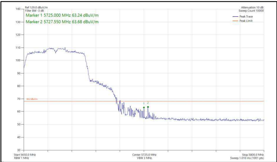
Figure 425 - 802.11n, HT40, TxBF, Core 0-1 - 5670 MHz, Band Edge Frequency 5725 MHz
