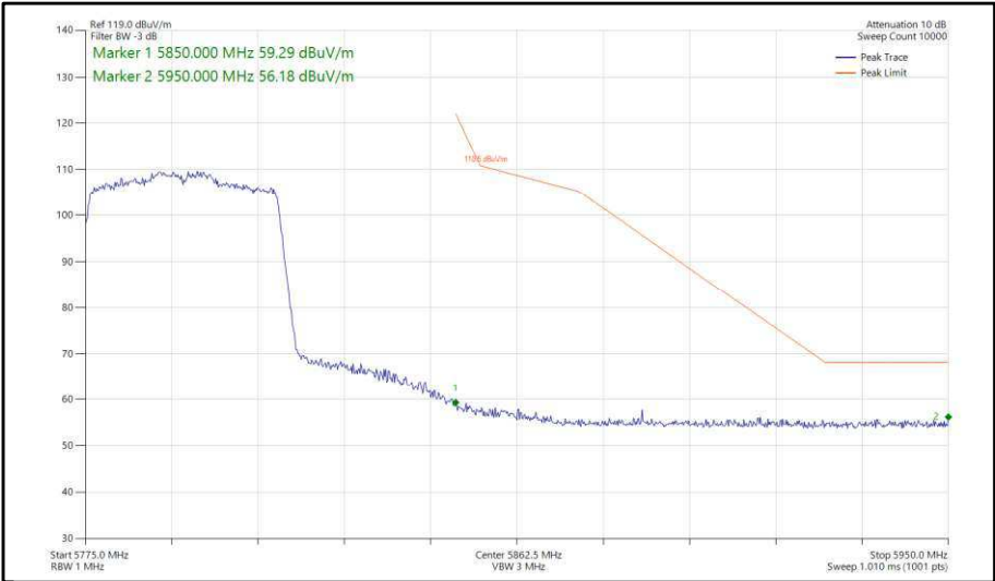
Figure 365 - 802.11ax, HE40, SU, SISO, Core 0 - 5795 MHz, Band Edge Frequency 5850 MHz
