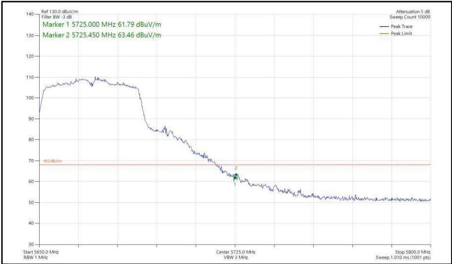
Figure 356 - 802.11n, HT40, SISO, Core 0 - 5670 MHz, Band Edge Frequency 5725 MHz
