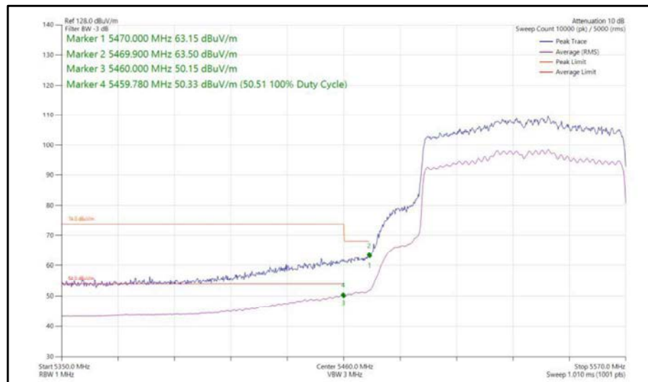
Figure 463 - 802.11ax, HE80, SU, CDD, Core 0-1 - 5530 MHz, Band Edge Frequency 5470 MHz
