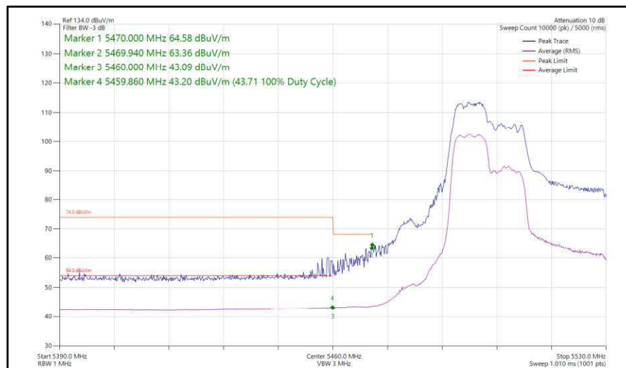
Figure 387 - 802.11ax, HE40, RU 106-53, CDD, Core 0-1 - 5510 MHz, Band Edge Frequency 5470 MHz
