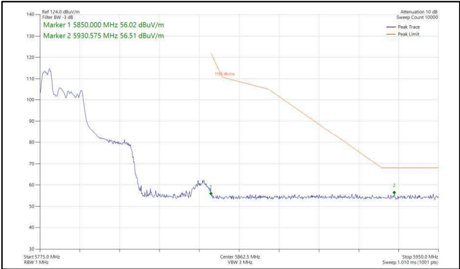
Figure 420 - 802.11ax, HE40, RU 52-37, SDM, Core 0-1 - 5795 MHz, Band Edge Frequency 5850 MHz
