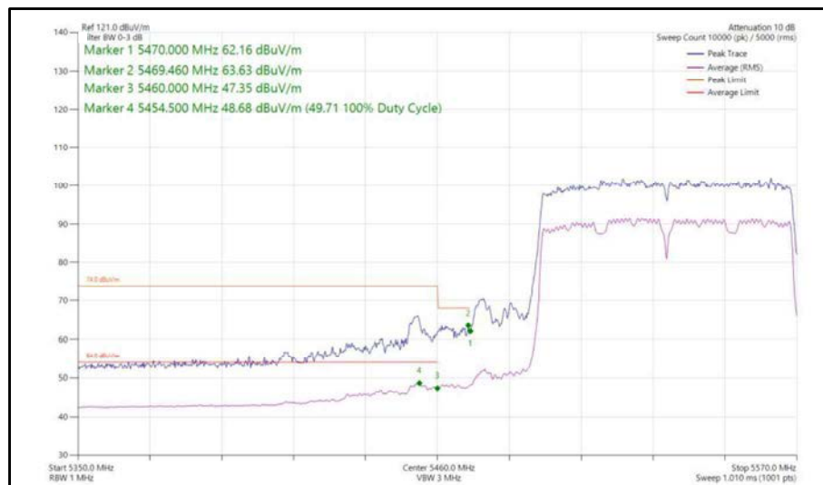
Figure 447 - 802.11ac, VHT80, SISO, Core 1 - 5530 MHz, Band Edge Frequency 5470 MHz
