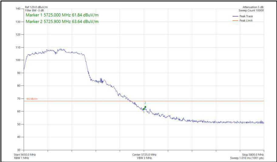
Figure 392 - 802.11n, HT40, CDD, Core 0-1 - 5670 MHz, Band Edge Frequency 5725 MHz
