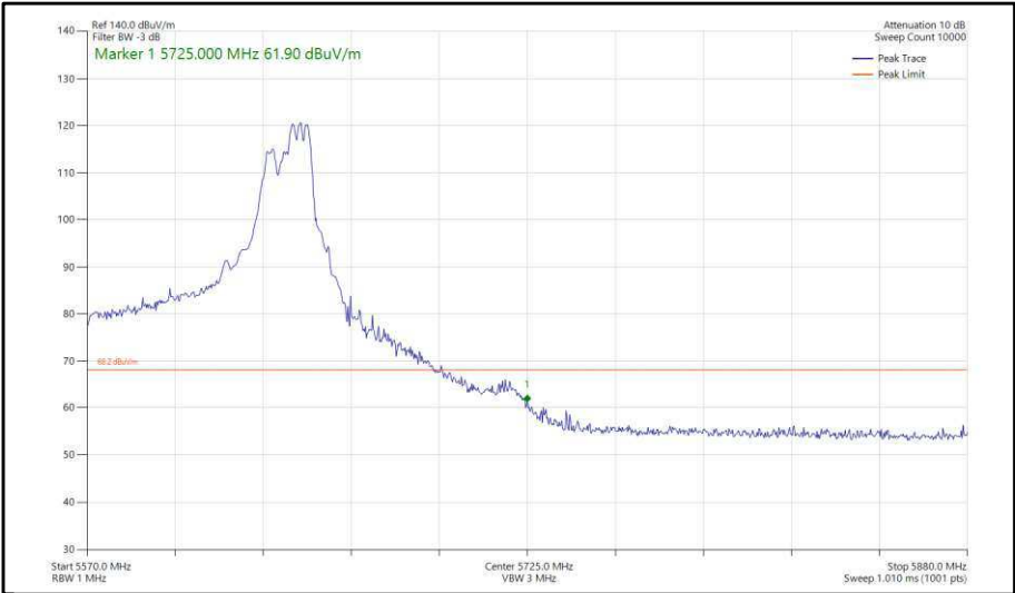
Figure 485 - 802.11ax, HE80, RU 106-60, SDM, Core 0-1 - 5610 MHz, Band Edge Frequency 5725 MHz
