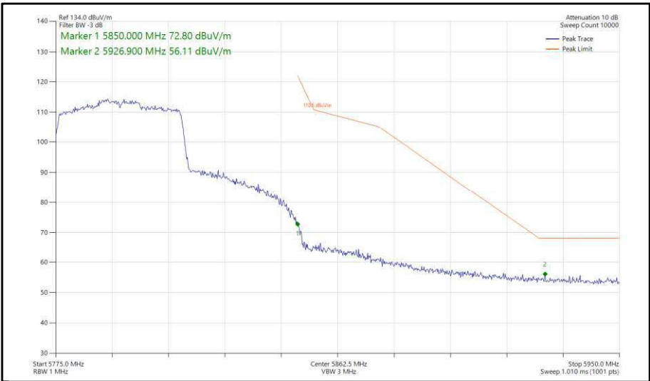
Figure 383 - 802.11ax, HE40, SU, SISO, Core 1 - 5795 MHz, Band Edge Frequency 5850 MHz
