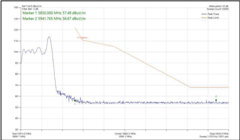
Figure 343 - 802.11ax, HE20, RU 26-8, SDM, Core 0-1 - 5825 MHz, Band Edge Frequency 5850 MHz
