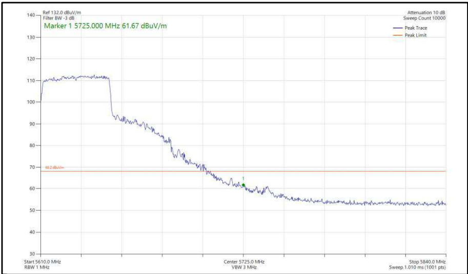
Figure 357 - 802.11ax, HE40, SU, SISO, Core 0 - 5630 MHz, Band Edge Frequency 5725 MHz
