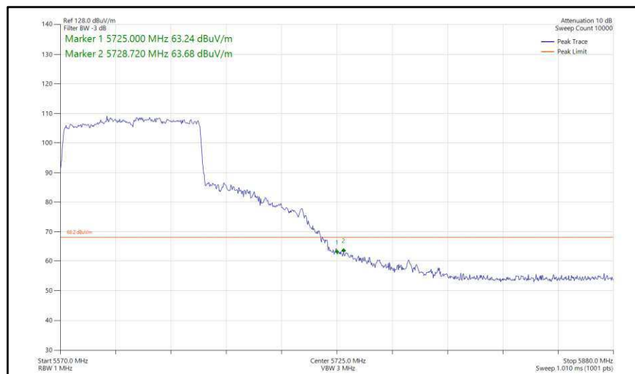
Figure 483 - 802.11ac, VHT80, SDM, Core 0-1 - 5610 MHz, Band Edge Frequency 5725 MHz
