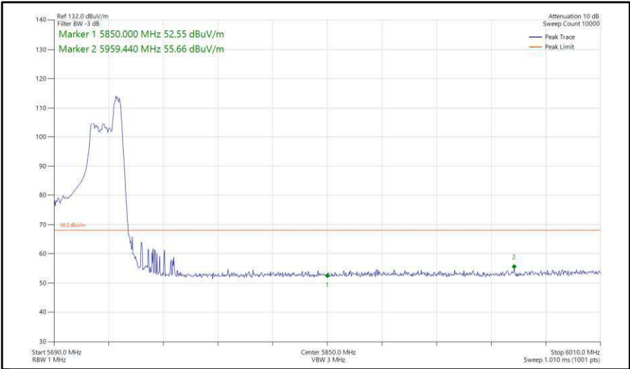
Figure 382 - 802.11ax, HE40, RU 52-44, SISO, Core 1 - 5710 MHz, Band Edge Frequency 5850 MHz
