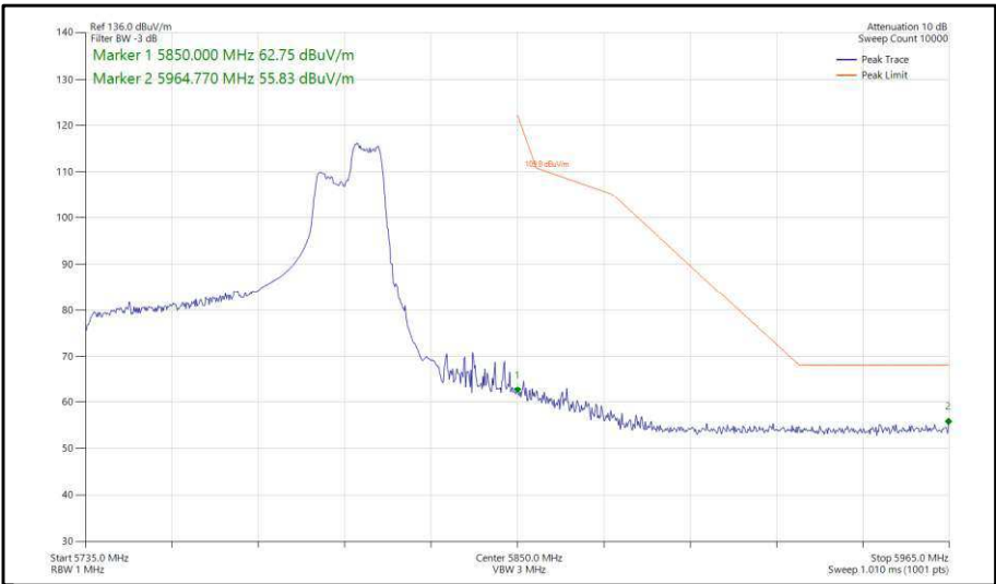
Figure 446 - 802.11ax, HE80, RU 106-60, SISO, Core 0 - 5775 MHz, Band Edge Frequency 5850 MHz
