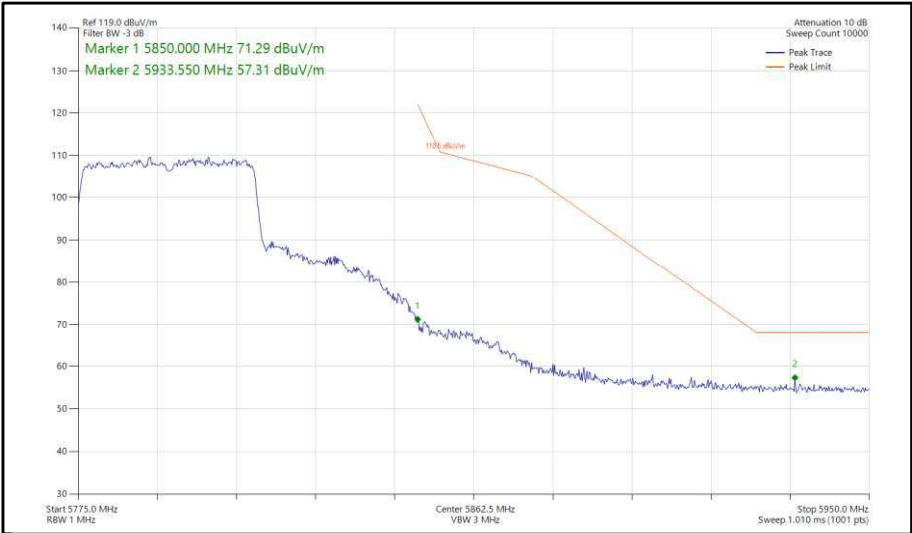
Figure 419 - 802.11ax, HE40, SU, SDM, Core 0-1 - 5795 MHz, Band Edge Frequency 5850 MHz
