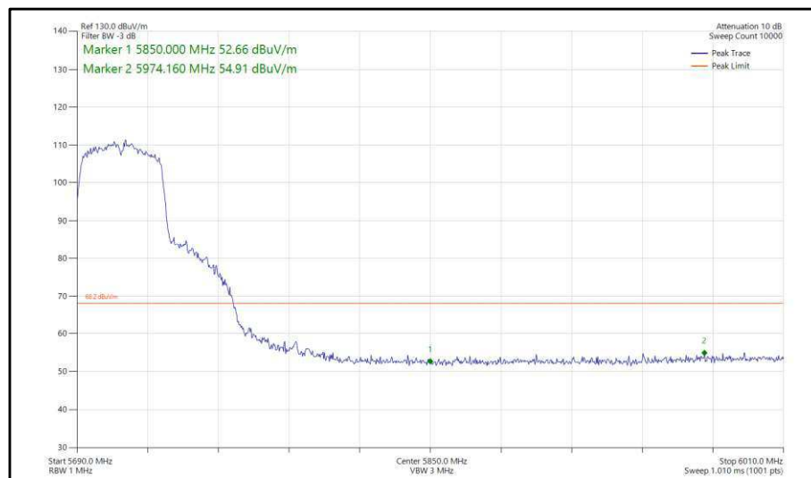
Figure 361 - 802.11n, HT40, SISO, Core 0 - 5710 MHz, Band Edge Frequency 5850 MHz
