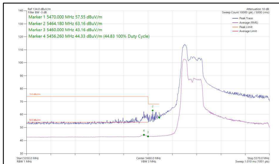
Figure 434 - 802.11ax, HE80, RU 52-37, SISO, Core 0 - 5530 MHz, Band Edge Frequency 5470 MHz
