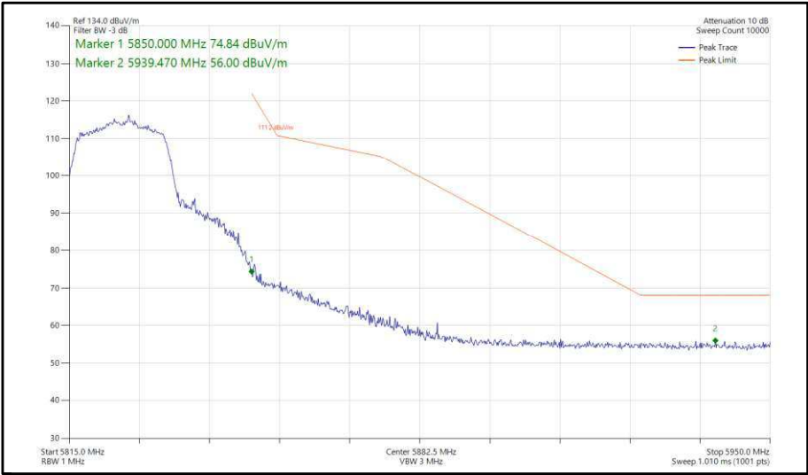
Figure 348 - 802.11n, HT20, TxBF, Core 0-1 - 5825 MHz, Band Edge Frequency 5850 MHz
