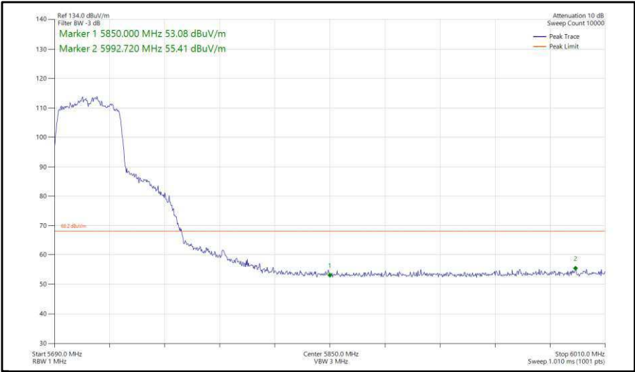
Figure 415 - 802.11n, HT40, SDM, Core 0-1 - 5710 MHz, Band Edge Frequency 5850 MHz
