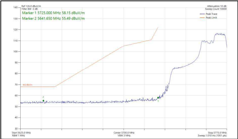
Figure 372 - 802.11ax, HE40, RU 106-56, SISO, Core 1 - 5755 MHz, Band Edge Frequency 5725 MHz
