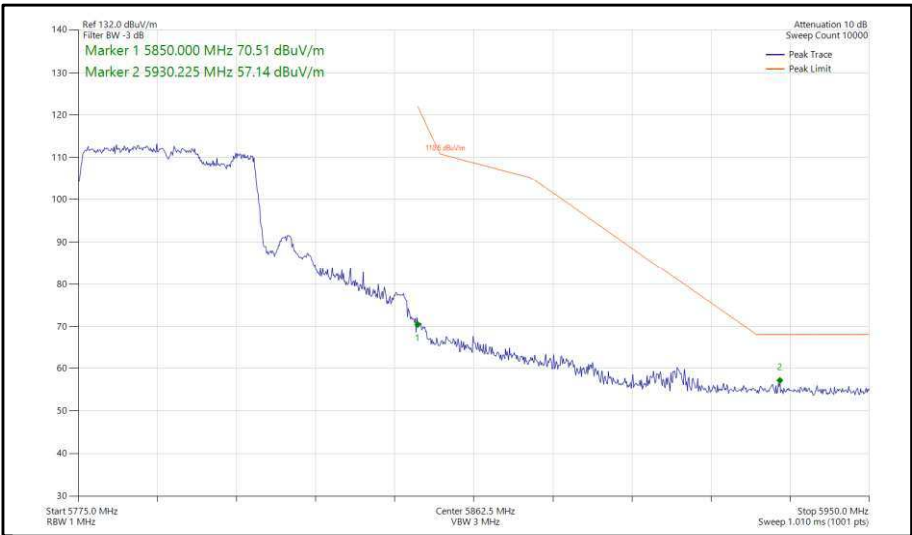
Figure 431 - 802.11ax, HE40, SU, TxBF, Core 0-1 - 5795 MHz, Band Edge Frequency 5850 MHz
