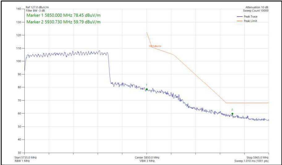
Figure 475 - 802.11ax, HE80, SU, CDD, Core 0-1 - 5775 MHz, Band Edge Frequency 5850 MHz
