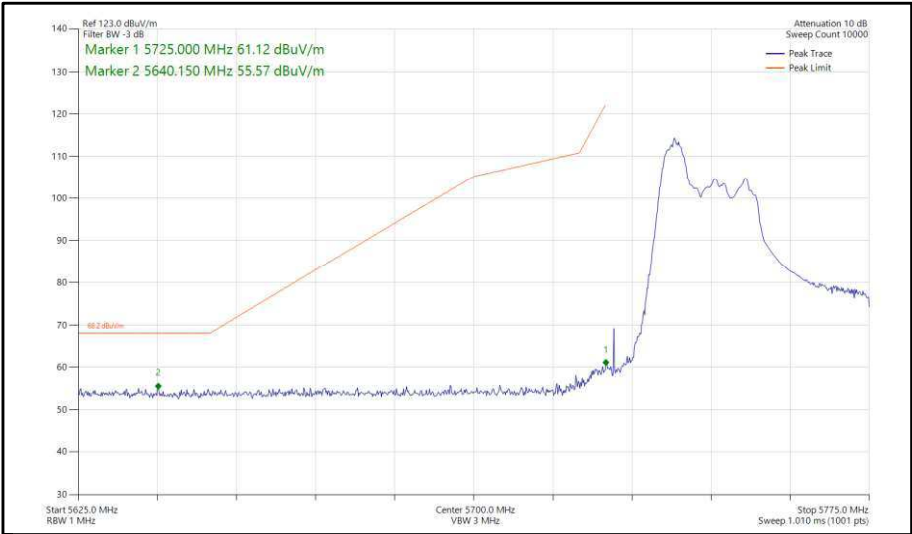
Figure 408 - 802.11ax, HE40, RU 52-37, SDM, Core 0-1 - 5755 MHz, Band Edge Frequency 5725 MHz
