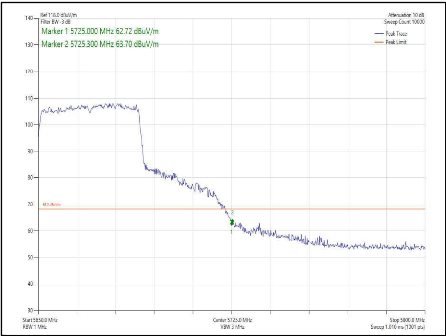
Figure 413 - 802.11ax, HE40, SU, SDM, Core 0-1 - 5670 MHz, Band Edge Frequency 5725 MHz
