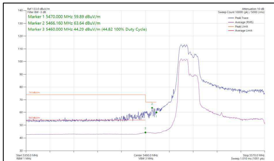
Figure 464 - 802.11ax, HE80, RU 106-53, CDD, Core 0-1 - 5530 MHz, Band Edge Frequency 5470 MHz
