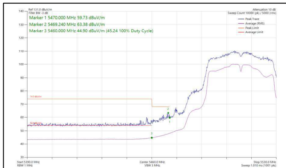
Figure 421 - 802.11n, HT40, TxBF, Core 0-1 - 5510 MHz, Band Edge Frequency 5470 MHz
