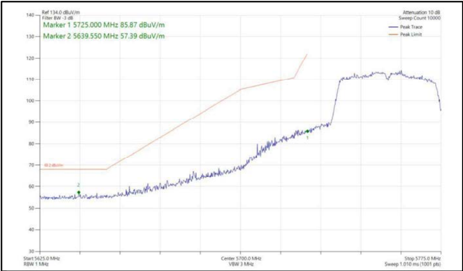
Figure 423 - 802.11n, HT40, TxBF, Core 0-1 - 5755 MHz, Band Edge Frequency 5725 MHz
