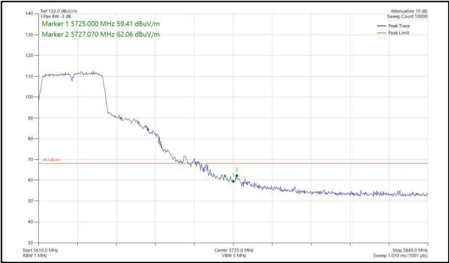
Figure 355 - 802.11n, HT40, SISO, Core 0 - 5630 MHz, Band Edge Frequency 5725 MHz
