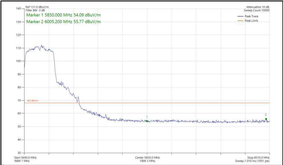
Figure 379 - 802.11n, HT40, SISO, Core 1 - 5710 MHz, Band Edge Frequency 5850 MHz
