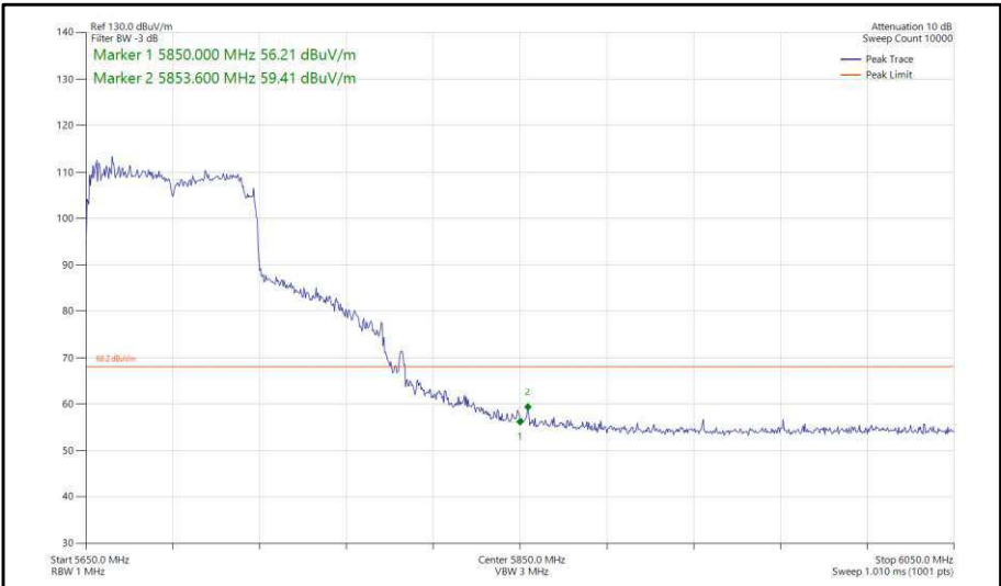
Figure 495 - 802.11ac, VHT80, TxBF, Core 0-1 - 5690 MHz, Band Edge Frequency 5850 MHz
