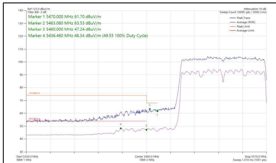
Figure 477 - 802.11ac, VHT80, SDM, Core 0-1 - 5530 MHz, Band Edge Frequency 5470 MHz
