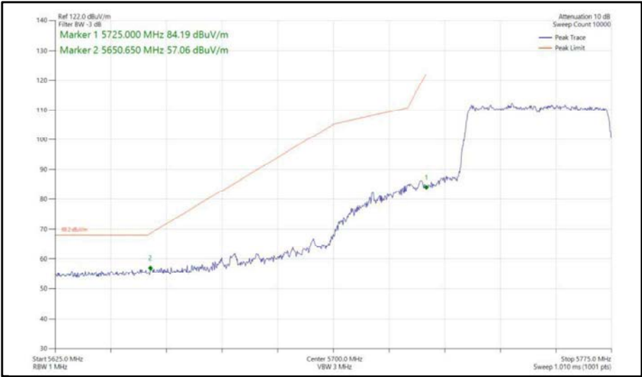
Figure 371 - 802.11ax, HE40, SU, SISO, Core 1 - 5755 MHz, Band Edge Frequency 5725 MHz
