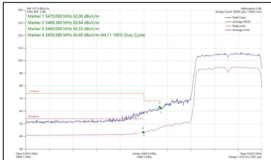
Figure 404 - 802.11ax, HE40, SU, SDM, Core 0-1 - 5510 MHz, Band Edge Frequency 5470 MHz
