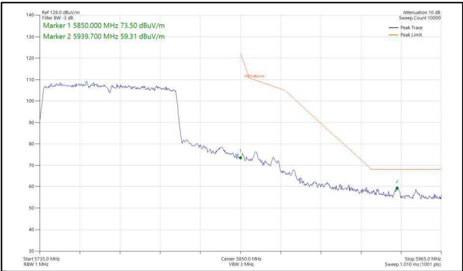
Figure 442 - 802.11ac, VHT80, SISO, Core 0 - 5775 MHz, Band Edge Frequency 5850 MHz
