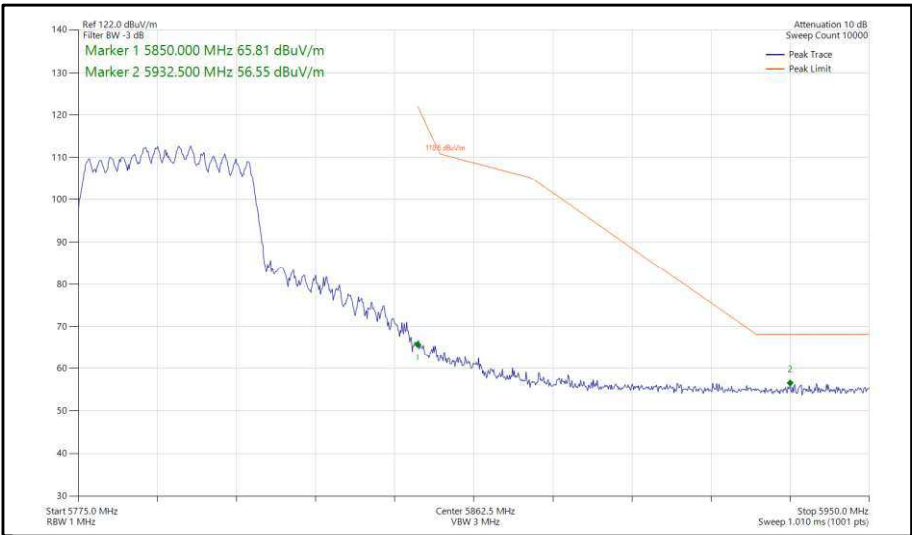
Figure 401 - 802.11ax, HE40, SU, CDD, Core 0-1 - 5795 MHz, Band Edge Frequency 5850 MHz
