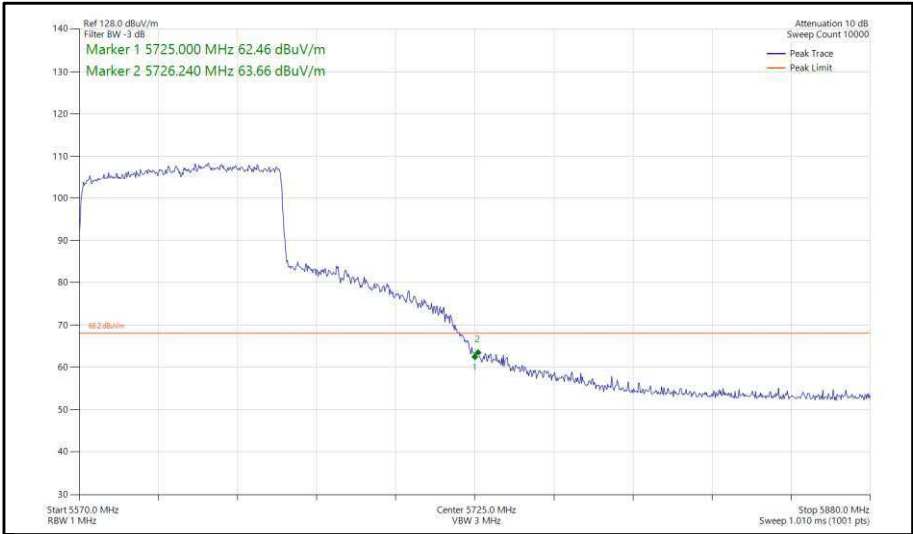
Figure 439 - 802.11ax, HE80, SU, SISO, Core 0 - 5610 MHz, Band Edge Frequency 5725 MHz
