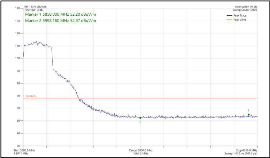
Figure 363 - 802.11ax, HE40, SU, SISO, Core 0 - 5710 MHz, Band Edge Frequency 5850 MHz
