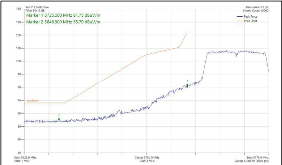
Figure 406 - 802.11n, HT40, SDM, Core 0-1 - 5755 MHz, Band Edge Frequency 5725 MHz
