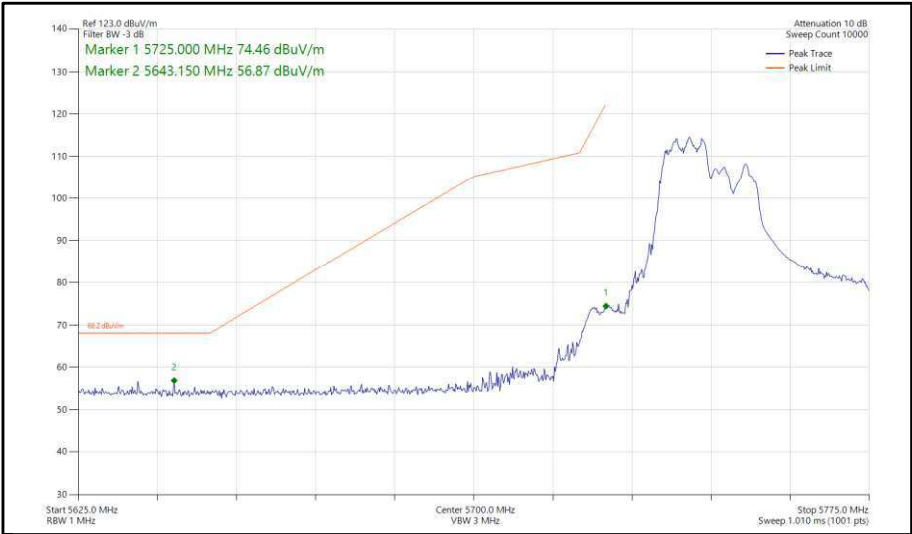
Figure 390 - 802.11ax, HE40, RU 106-53, CDD, Core 0-1 - 5755 MHz, Band Edge Frequency 5725 MHz
