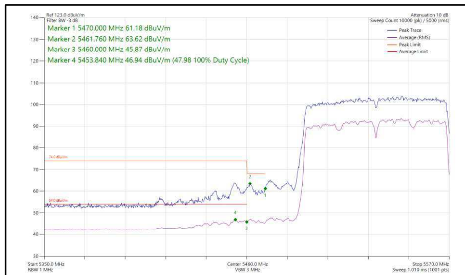
Figure 462 - 802.11ac, VHT80, CDD, Core 0-1 - 5530 MHz, Band Edge Frequency 5470 MHz
