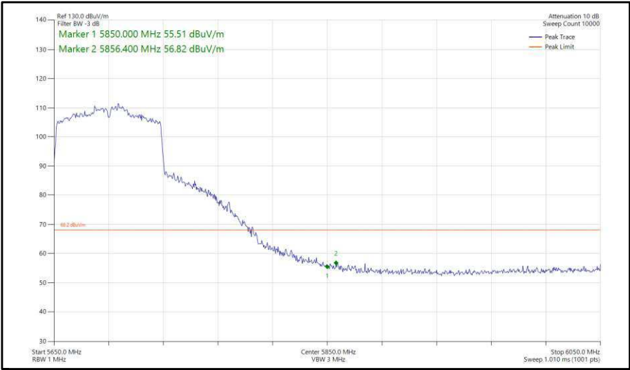
Figure 471 - 802.11ac, VHT80, CDD, Core 0-1 - 5690 MHz, Band Edge Frequency 5850 MHz
