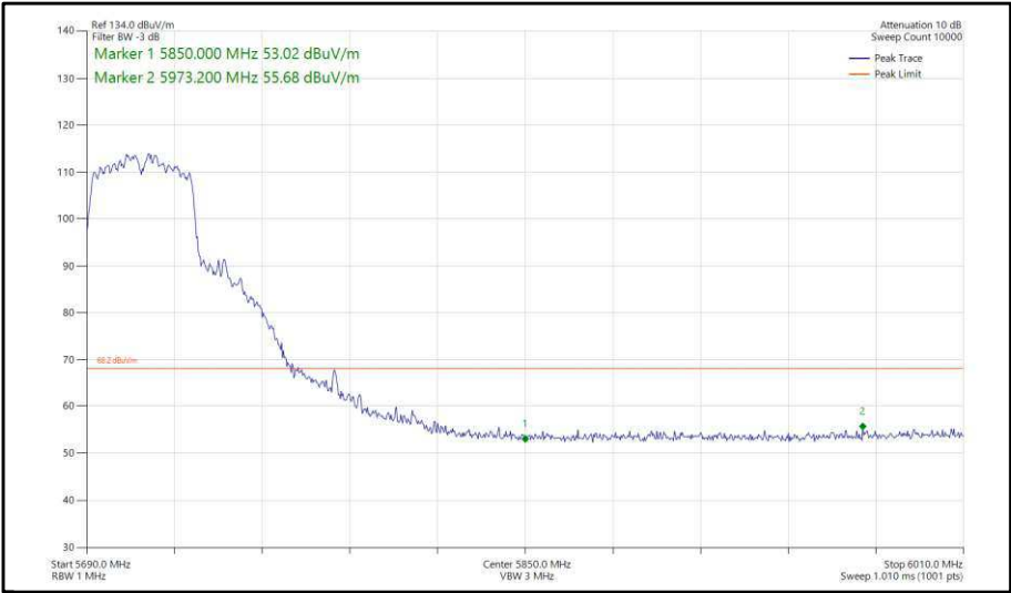
Figure 397 - 802.11n, HT40, CDD, Core 0-1 - 5710 MHz, Band Edge Frequency 5850 MHz
