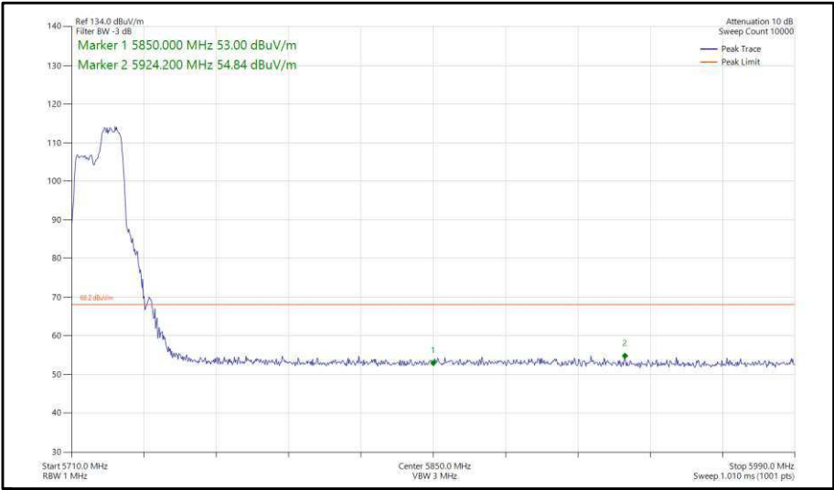
Figure 341 - 802.11ax, HE20, RU 106-54, SDM, Core 0-1 - 5720 MHz, Band Edge Frequency 5850 MHz
