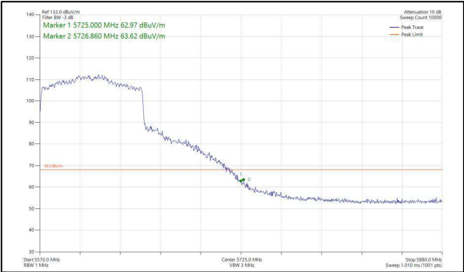
Figure 469 - 802.11ax, HE80, SU, CDD, Core 0-1 - 5610 MHz, Band Edge Frequency 5725 MHz
