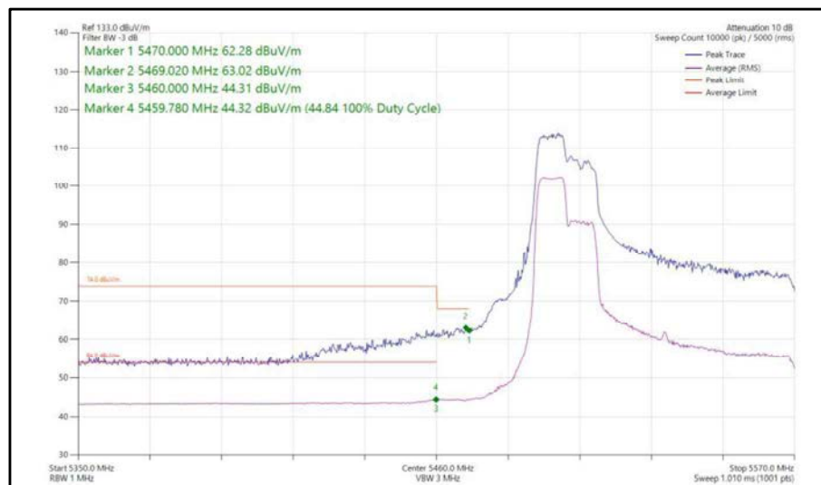
Figure 449 - 802.11ax, HE80, RU 106-53, SISO, Core 1 - 5530 MHz, Band Edge Frequency 5470 MHz
