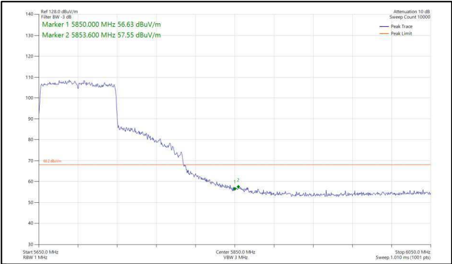
Figure 441 - 802.11ac, VHT80, SISO, Core 0 - 5690 MHz, Band Edge Frequency 5850 MHz
