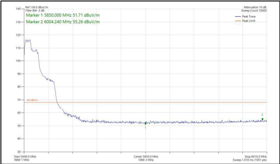
Figure 418 - 802.11ax, HE40, RU 106-53, SDM, Core 0-1 - 5710 MHz, Band Edge Frequency 5850 MHz
