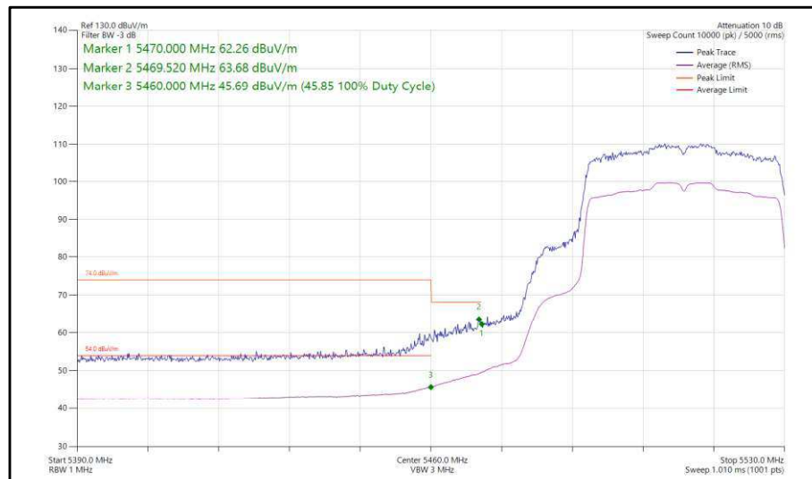
Figure 350 - 802.11ax, HE40, SU, SISO, Core 0 - 5510 MHz, Band Edge Frequency 5470 MHz
