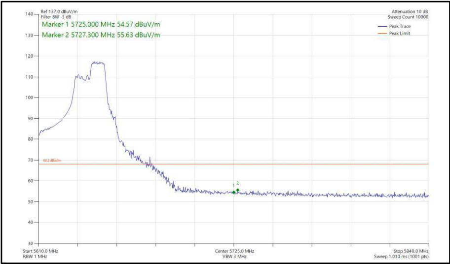
Figure 358 - 802.11ax, HE40, RU 106-56, SISO, Core 0 - 5630 MHz, Band Edge Frequency 5725 MHz
