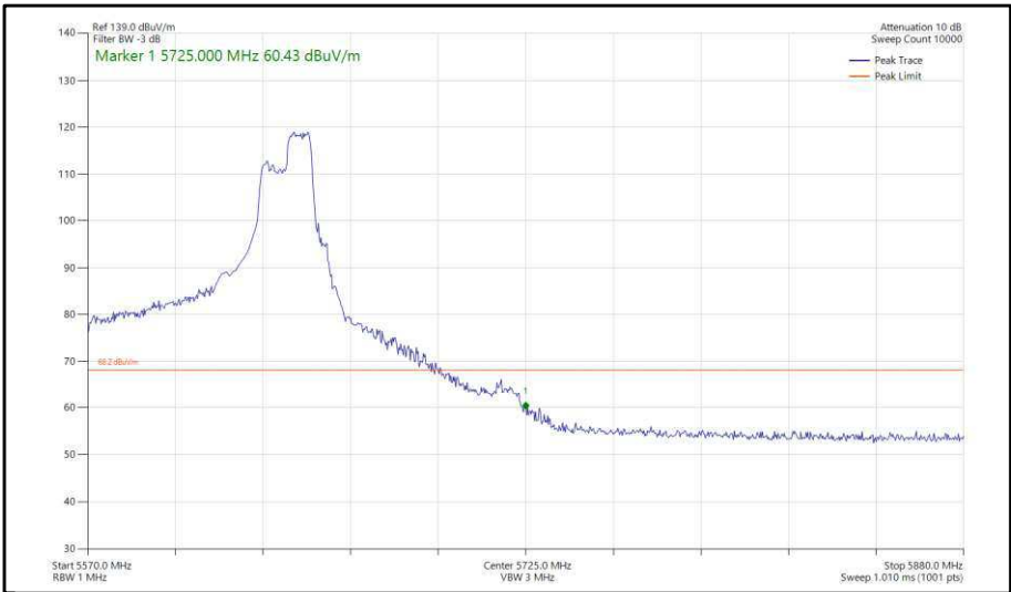
Figure 440 - 802.11ax, HE80, RU 106-60, SISO, Core 0 - 5610 MHz, Band Edge Frequency 5725 MHz
