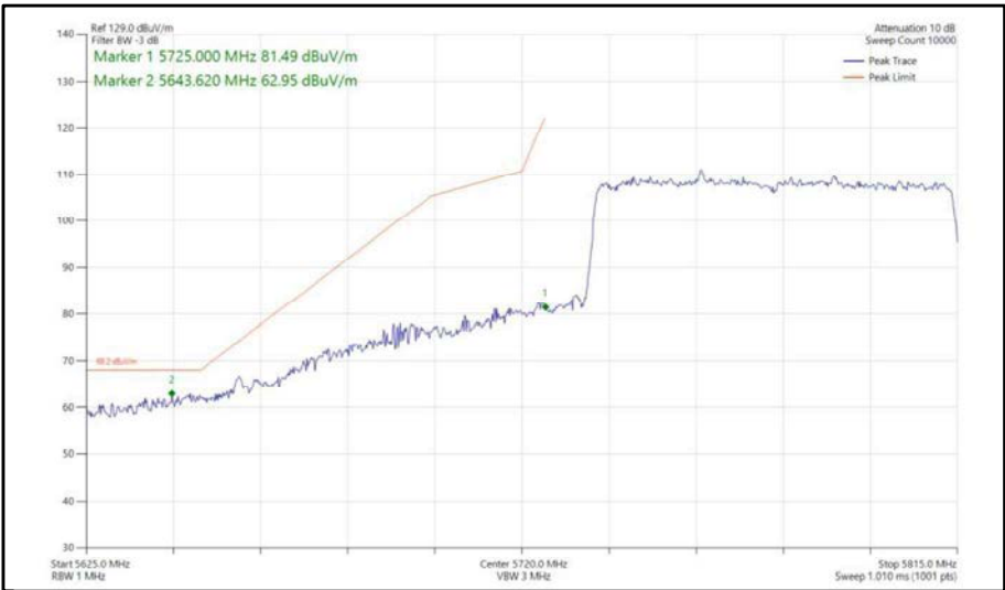
Figure 481 - 802.11ax, HE80, SU, SDM, Core 0-1 - 5775 MHz, Band Edge Frequency 5725 MHz
