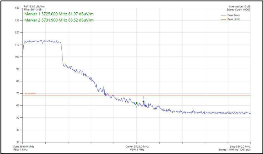
Figure 375 - 802.11ax, HE40, SU, SISO, Core 1 - 5630 MHz, Band Edge Frequency 5725 MHz
