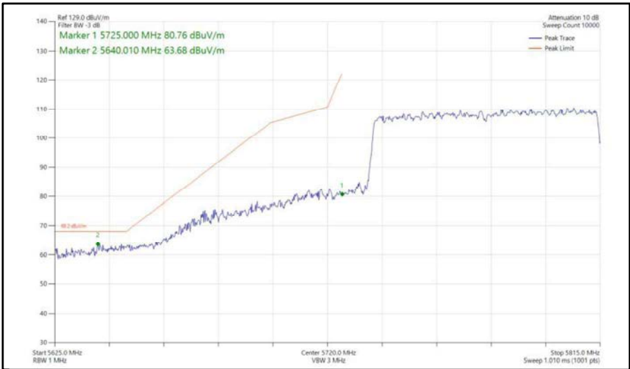
Figure 466 - 802.11ax, HE80, SU, CDD, Core 0-1 - 5775 MHz, Band Edge Frequency 5725 MHz
