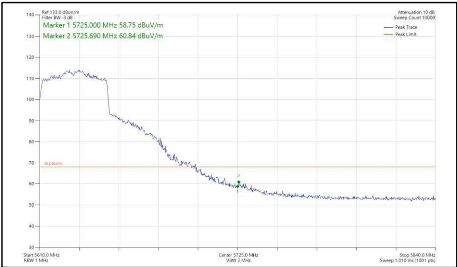
Figure 411 - 802.11ax, HE40, SU, SDM, Core 0-1 - 5630 MHz, Band Edge Frequency 5725 MHz
