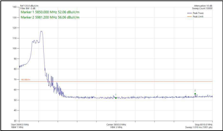
Figure 400 - 802.11ax, HE40, RU 52-44, CDD, Core 0-1 - 5710 MHz, Band Edge Frequency 5850 MHz
