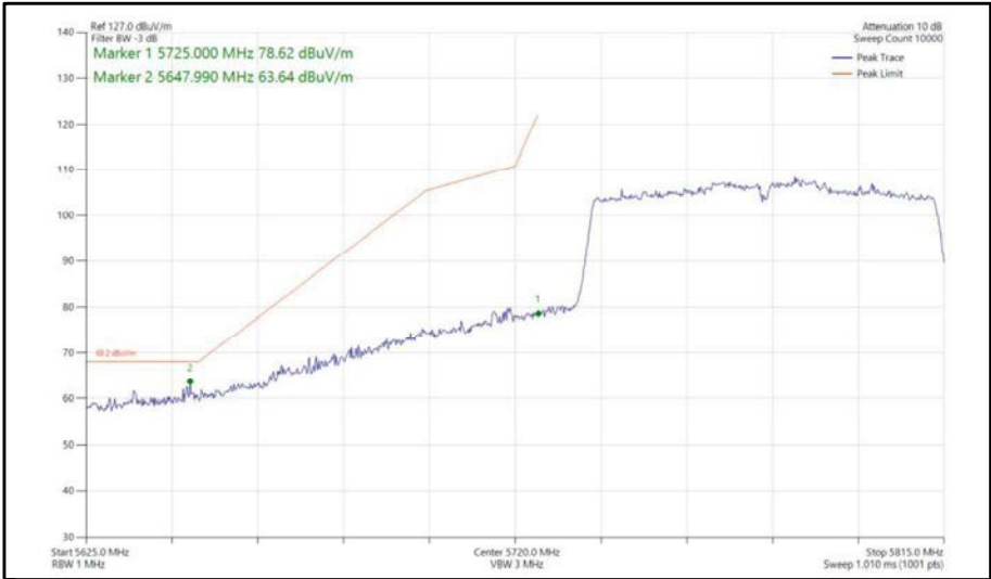
Figure 450 - 802.11ac, VHT80, SISO, Core 1 - 5775 MHz, Band Edge Frequency 5725 MHz
