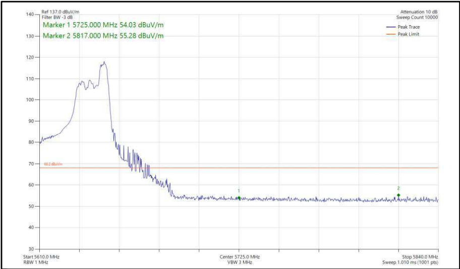
Figure 412 - 802.11ax, HE40, RU 52-44, SDM, Core 0-1 - 5630 MHz, Band Edge Frequency 5725 MHz
