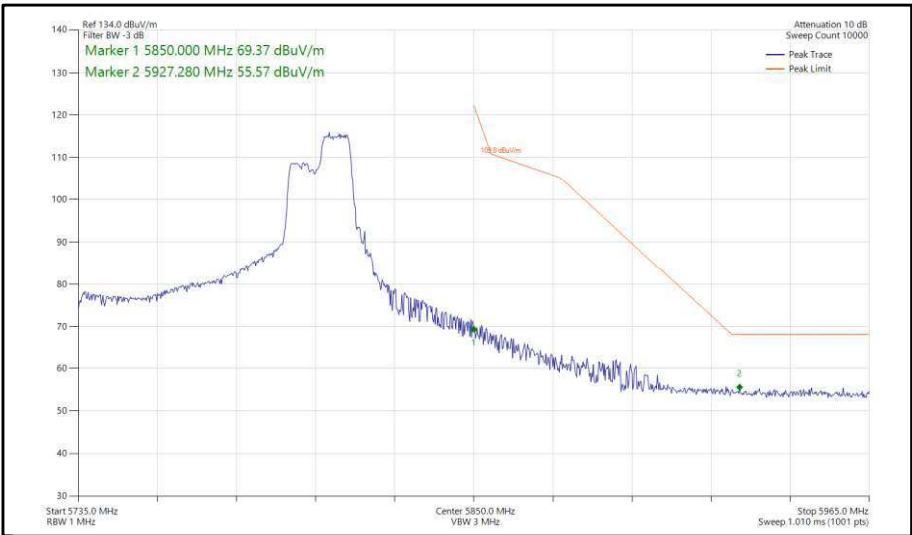
Figure 491 - 802.11ax, HE80, RU 106-60, SDM, Core 0-1 - 5775 MHz, Band Edge Frequency 5850 MHz
