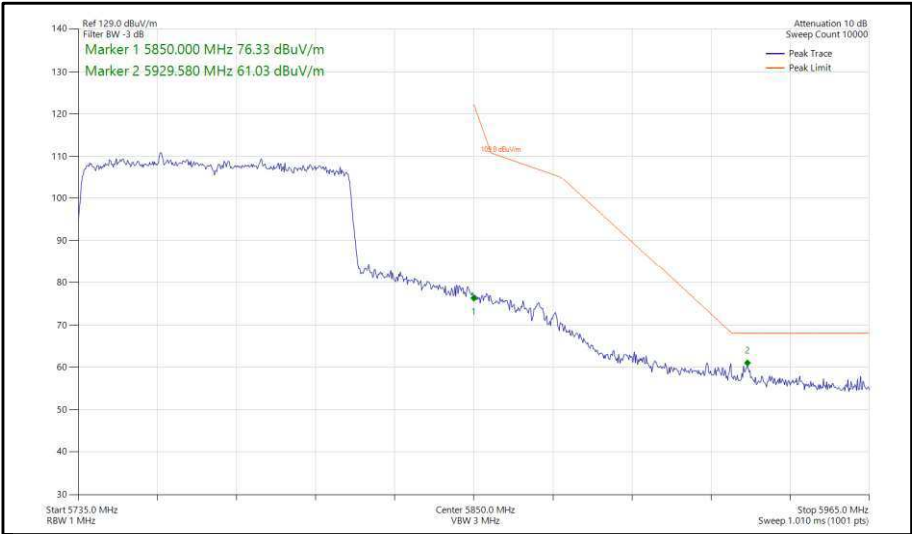
Figure 490 - 802.11ax, HE80, SU, SDM, Core 0-1 - 5775 MHz, Band Edge Frequency 5850 MHz
