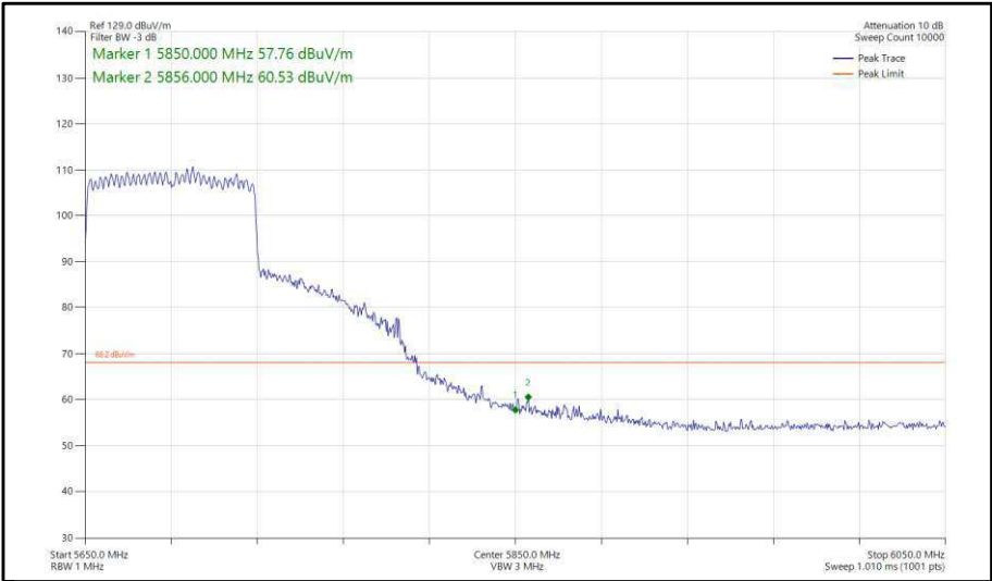
Figure 473 - 802.11ax, HE80, SU, CDD, Core 0-1 - 5690 MHz, Band Edge Frequency 5850 MHz
