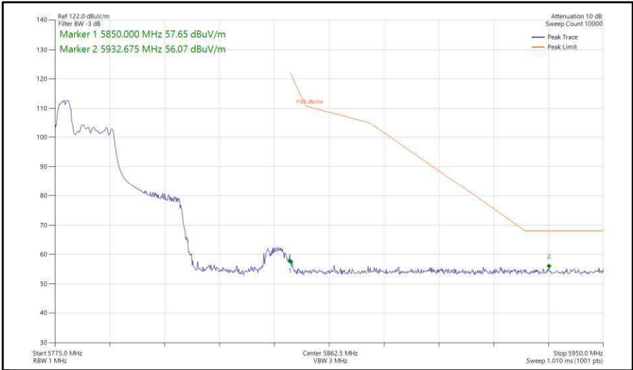
Figure 384 - 802.11ax, HE40, RU 52-37, SISO, Core 1 - 5795 MHz, Band Edge Frequency 5850 MHz
