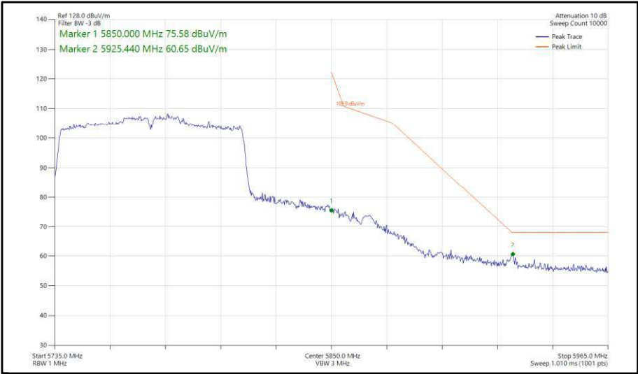
Figure 457 - 802.11ac, VHT80, SISO, Core 1 - 5775 MHz, Band Edge Frequency 5850 MHz
