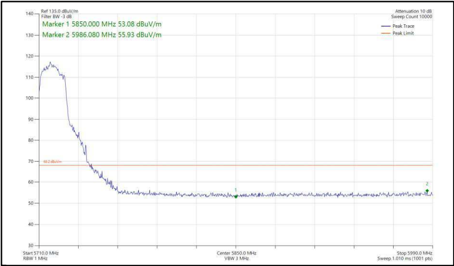
Figure 347 - 802.11n, HT20, TxBF, Core 0-1 - 5720 MHz, Band Edge Frequency 5850 MHz
