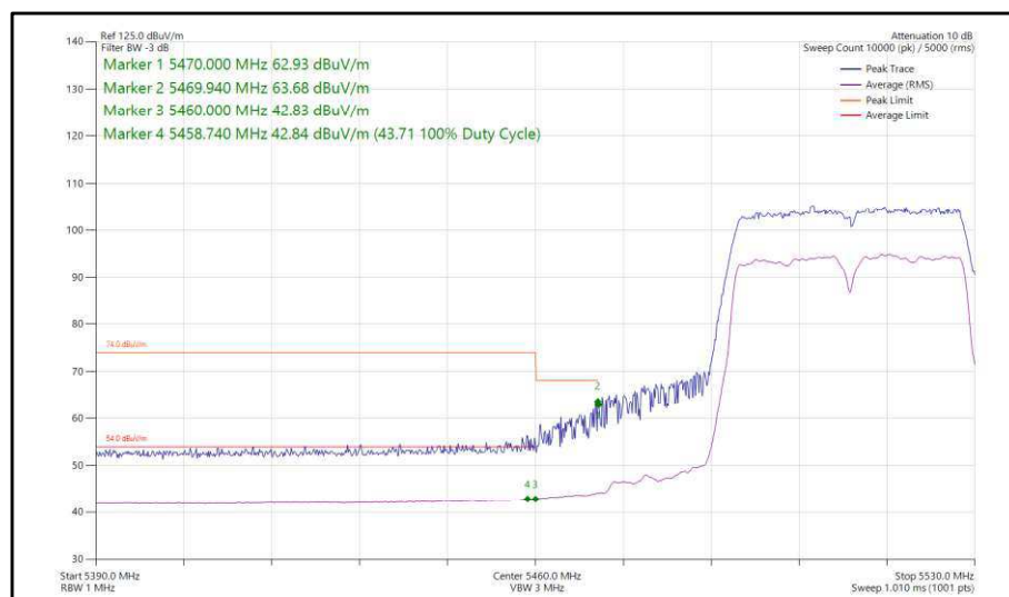
Figure 403 - 802.11n, HT40, SDM, Core 0-1 - 5510 MHz, Band Edge Frequency 5470 MHz
