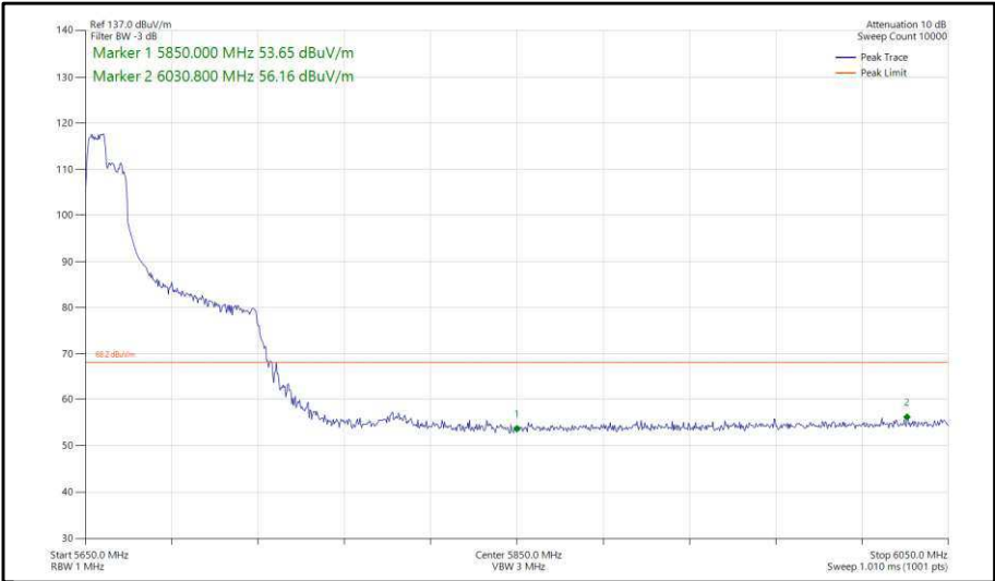
Figure 444 - 802.11ax, HE80, RU 106-53, SISO, Core 0 - 5690 MHz, Band Edge Frequency 5850 MHz
