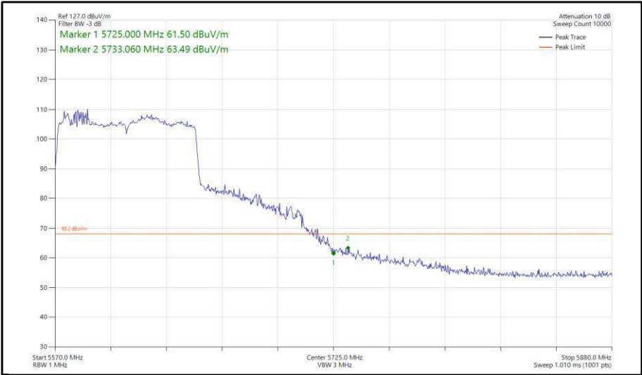
Figure 494 - 802.11ac, VHT80, TxBF, Core 0-1 - 5610 MHz, Band Edge Frequency 5725 MHz
