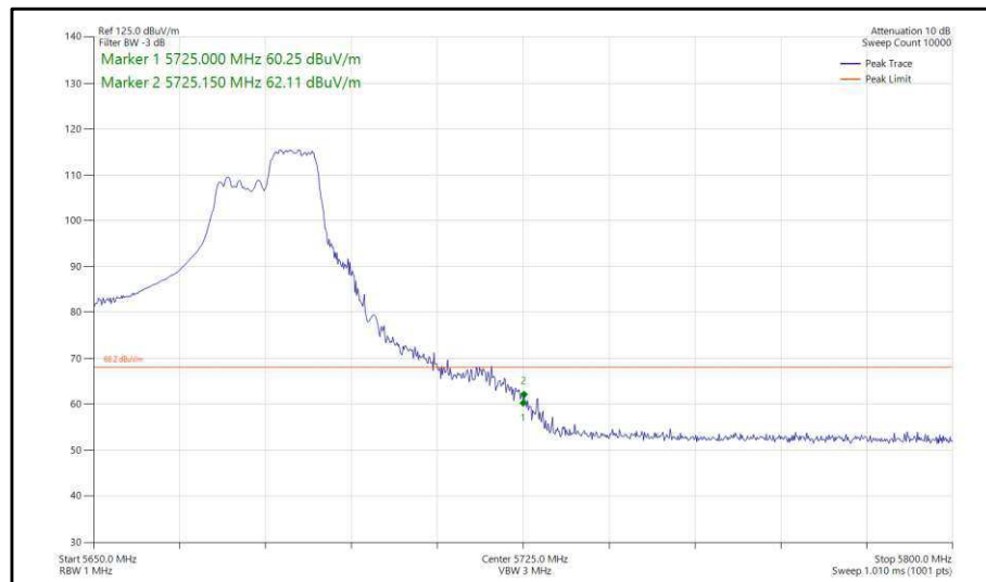
Figure 360 - 802.11ax, HE40, RU 106-56, SISO, Core 0 - 5670 MHz, Band Edge Frequency 5725 MHz
