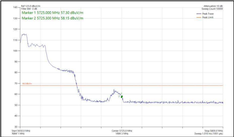
Figure 378 - 802.11ax, HE40, RU 52-37, SISO, Core 1 - 5670 MHz, Band Edge Frequency 5725 MHz
