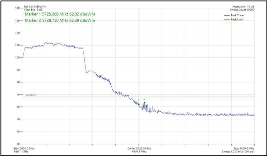
Figure 377 - 802.11ax, HE40, SU, SISO, Core 1 - 5670 MHz, Band Edge Frequency 5725 MHz
