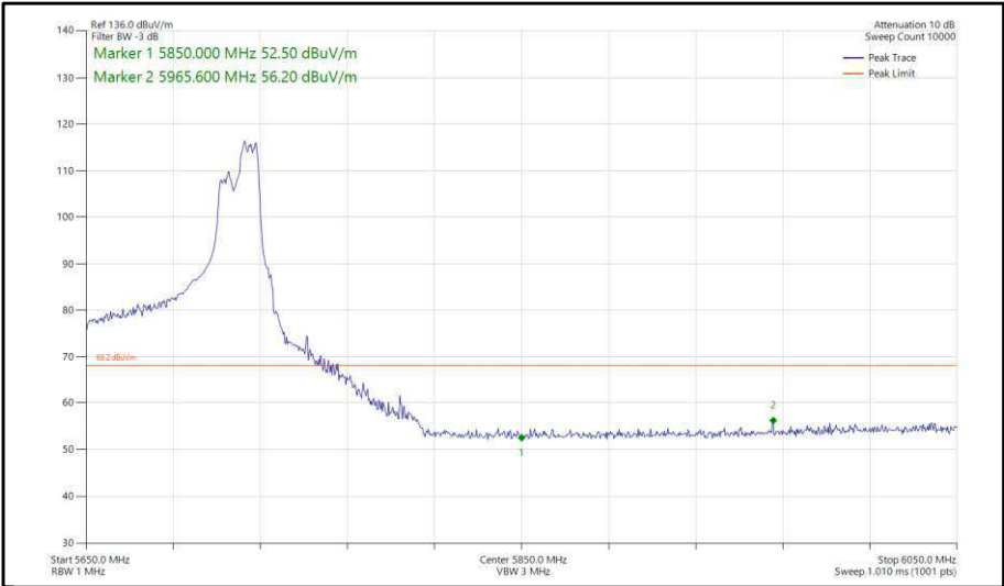
Figure 474 - 802.11ax, HE80, RU 106-60, CDD, Core 0-1 - 5690 MHz, Band Edge Frequency 5850 MHz
