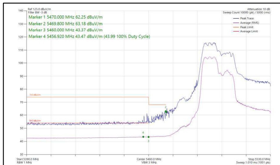
Figure 405 - 802.11ax, HE40, RU 106-53, SDM, Core 0-1 - 5510 MHz, Band Edge Frequency 5470 MHz
