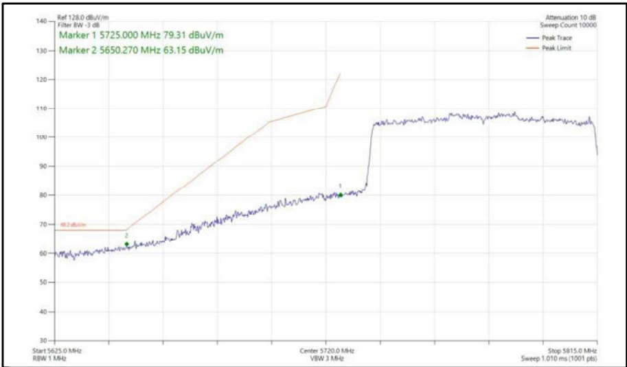
Figure 451 - 802.11ax, HE80, SU, SISO, Core 1 - 5775 MHz, Band Edge Frequency 5725 MHz
