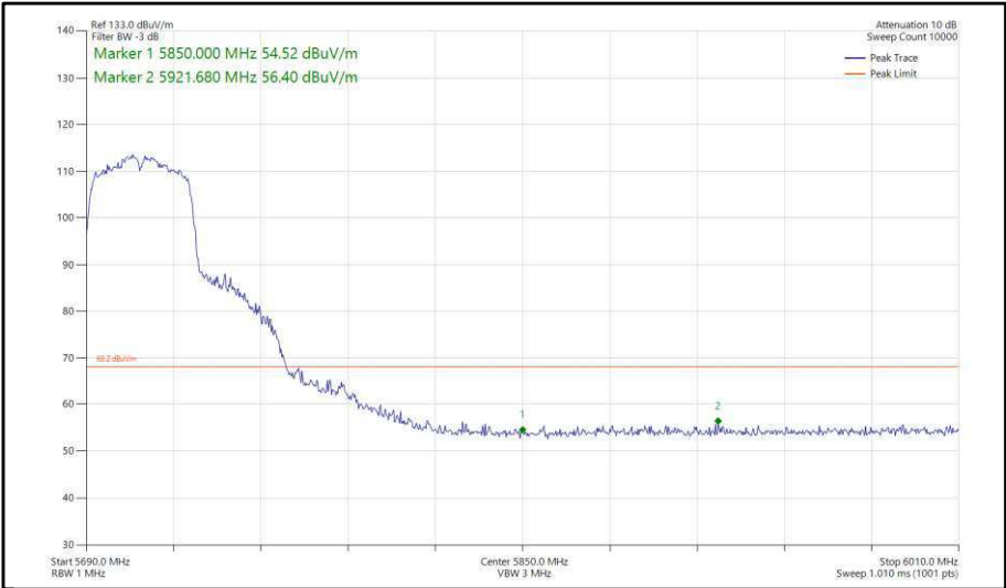
Figure 427 - 802.11n, HT40, TxBF, Core 0-1 - 5710 MHz, Band Edge Frequency 5850 MHz
