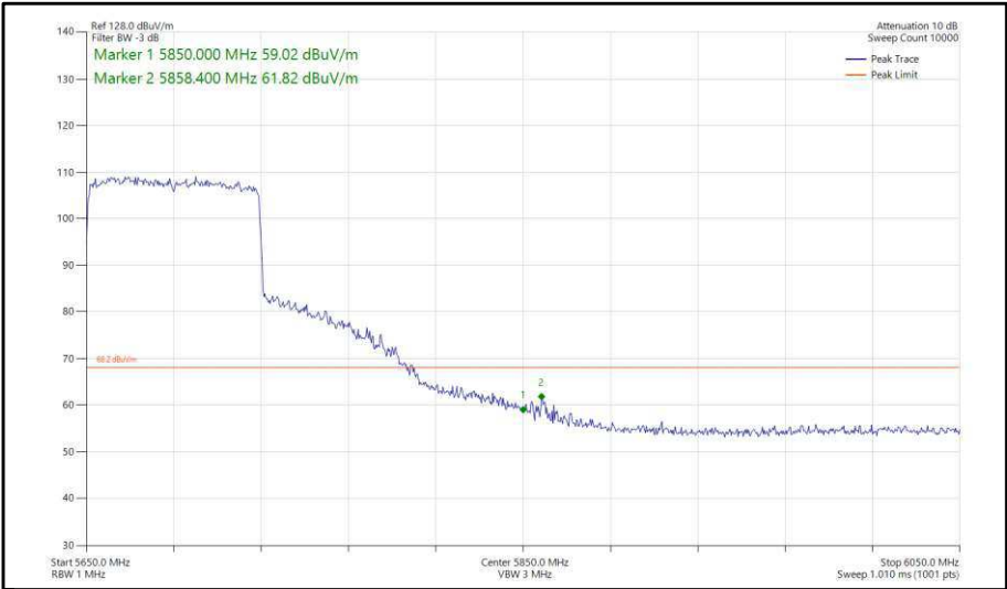
Figure 458 - 802.11ax, HE80, SU, SISO, Core 1 - 5690 MHz, Band Edge Frequency 5850 MHz
