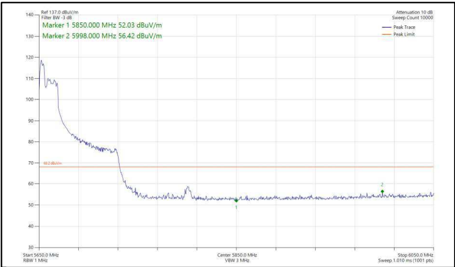
Figure 489 - 802.11ax, HE80, RU 52-37, SDM, Core 0-1 - 5690 MHz, Band Edge Frequency 5850 MHz
