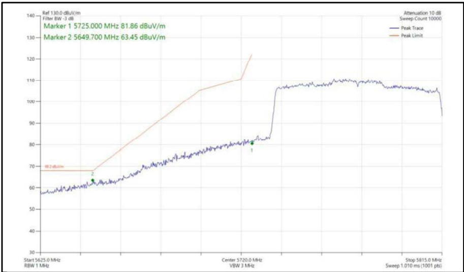
Figure 436 - 802.11ax, HE80, SU, SISO, Core 0 - 5775 MHz, Band Edge Frequency 5725 MHz
