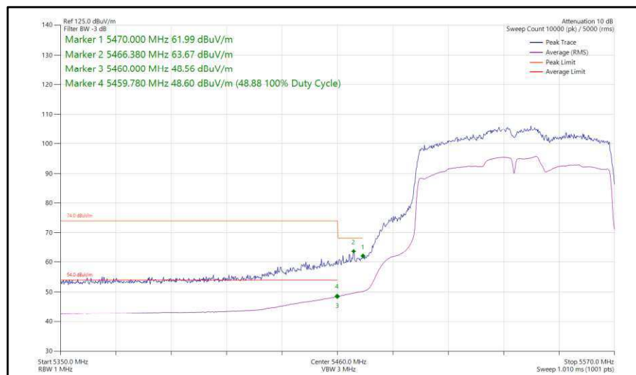
Figure 492 - 802.11ac, VHT80, TxBF, Core 0-1 - 5530 MHz, Band Edge Frequency 5470 MHz
