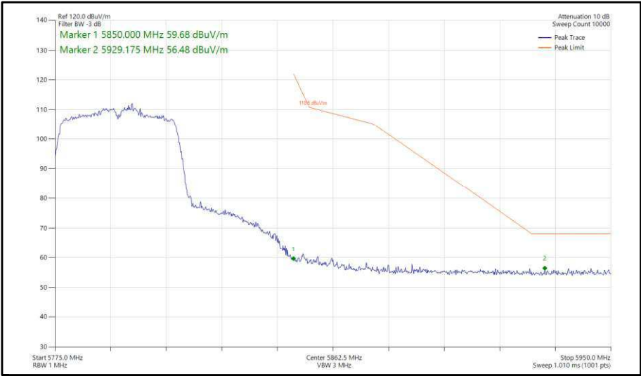
Figure 416 - 802.11n, HT40, SDM, Core 0-1 - 5795 MHz, Band Edge Frequency 5850 MHz
