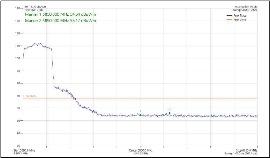
Figure 381 - 802.11ax, HE40, SU, SISO, Core 1 - 5710 MHz, Band Edge Frequency 5850 MHz
