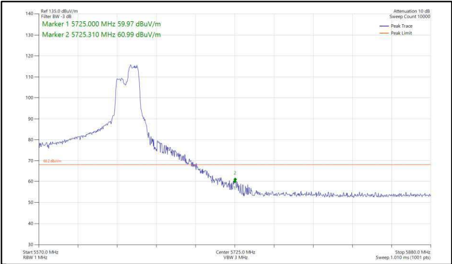
Figure 470 - 802.11ax, HE80, RU 106-60, CDD, Core 0-1 - 5610 MHz, Band Edge Frequency 5725 MHz
