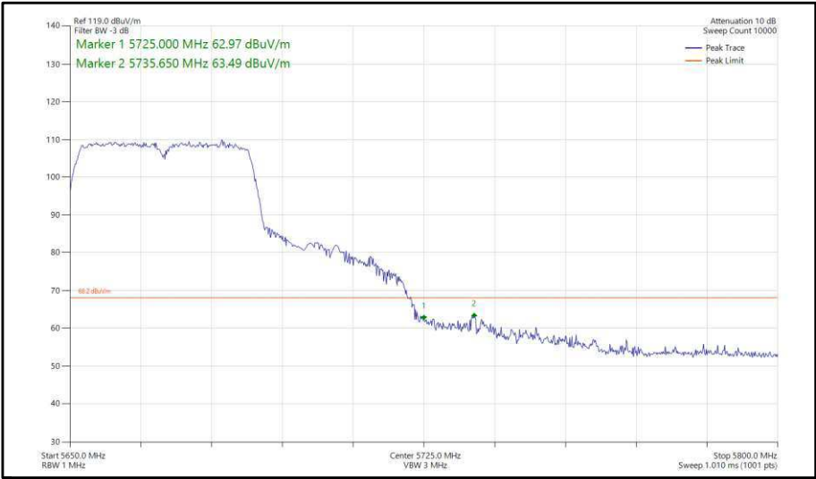
Figure 374 - 802.11n, HT40, SISO, Core 1 - 5670 MHz, Band Edge Frequency 5725 MHz
