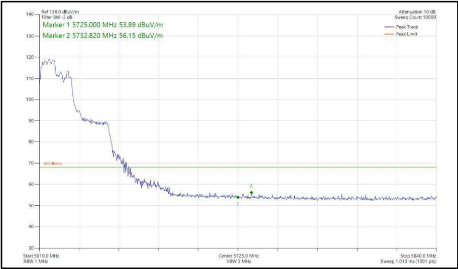
Figure 394 - 802.11ax, HE40, RU 106-53, CDD, Core 0-1 - 5630 MHz, Band Edge Frequency 5725 MHz
