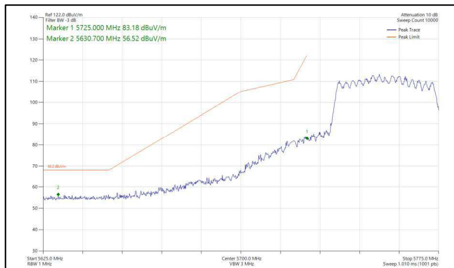
Figure 389 - 802.11ax, HE40, SU, CDD, Core 0-1 - 5755 MHz, Band Edge Frequency 5725 MHz
