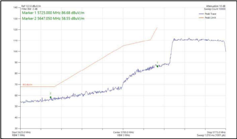
Figure 353 - 802.11ax, HE40, SU, SISO, Core 0 - 5755 MHz, Band Edge Frequency 5725 MHz
