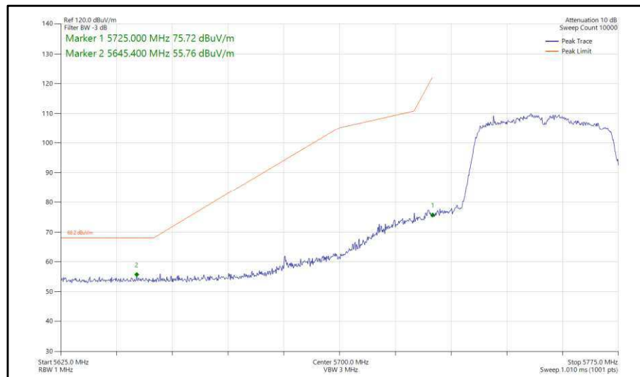
Figure 388 - 802.11n, HT40, CDD, Core 0-1 - 5755 MHz, Band Edge Frequency 5725 MHz
