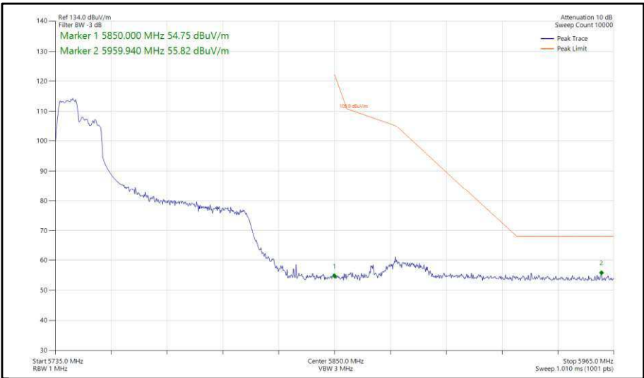
Figure 461 - 802.11ax, HE80, RU 106-53, SISO, Core 1 - 5775 MHz, Band Edge Frequency 5850 MHz
