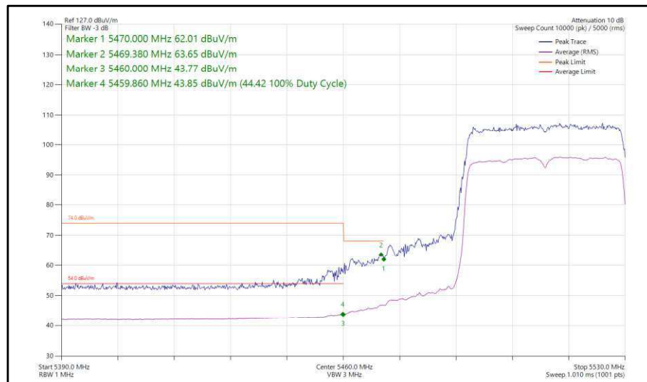
Figure 368 - 802.11ax, HE40, SU, SISO, Core 1 - 5510 MHz, Band Edge Frequency 5470 MHz
