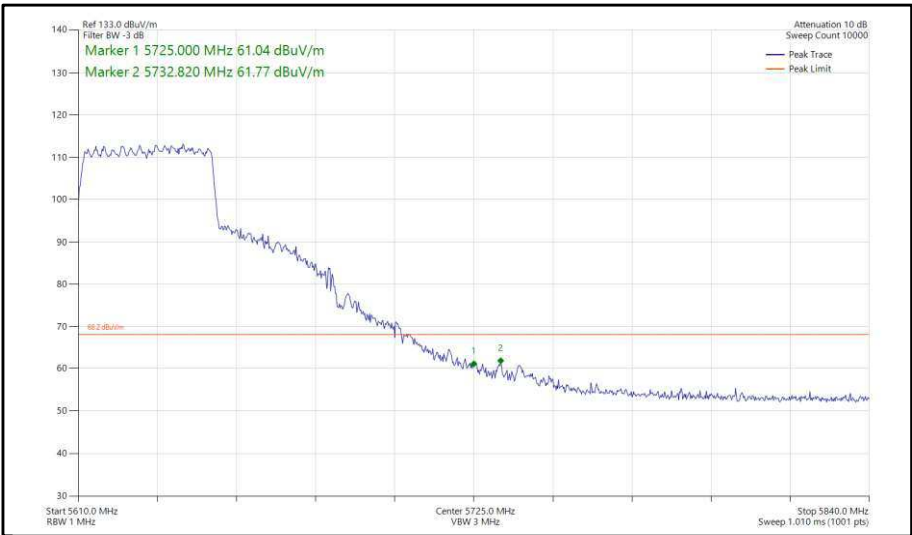
Figure 393 - 802.11ax, HE40, SU, CDD, Core 0-1 - 5630 MHz, Band Edge Frequency 5725 MHz
