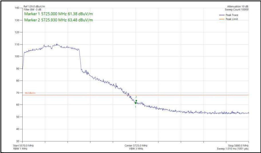
Figure 438 - 802.11ac, VHT80, SISO, Core 0 - 5610 MHz, Band Edge Frequency 5725 MHz
