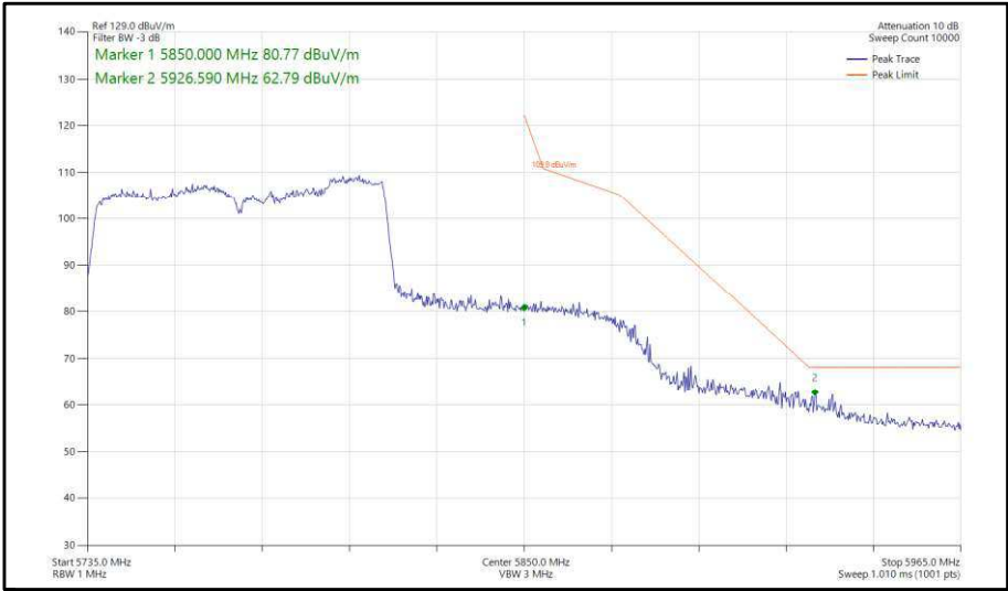
Figure 496 - 802.11ac, VHT80, TxBF, Core 0-1 - 5775 MHz, Band Edge Frequency 5850 MHz
