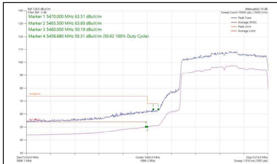
Figure 448 - 802.11ax, HE80, SU, SISO, Core 1 - 5530 MHz, Band Edge Frequency 5470 MHz
