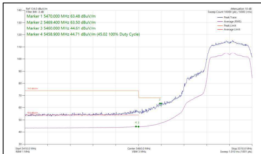
Figure 344 - 802.11n, HT20, TxBF, Core 0-1 - 5500 MHz, Band Edge Frequency 5470 MHz
