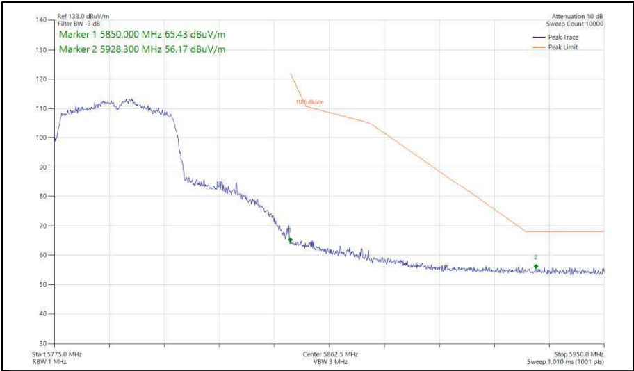
Figure 428 - 802.11n, HT40, TxBF, Core 0-1 - 5795 MHz, Band Edge Frequency 5850 MHz
