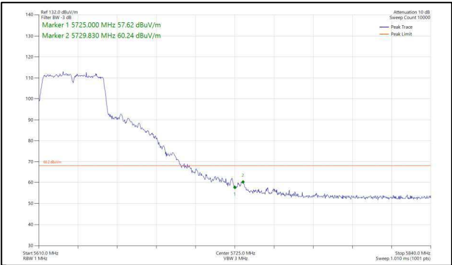
Figure 409 - 802.11n, HT40, SDM, Core 0-1 - 5630 MHz, Band Edge Frequency 5725 MHz
