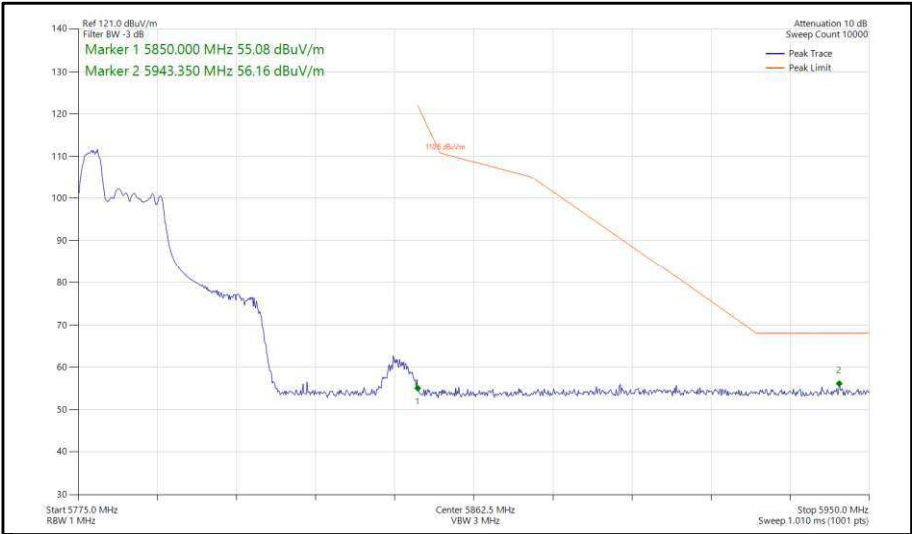
Figure 366 - 802.11ax, HE40, RU 52-37, SISO, Core 0 - 5795 MHz, Band Edge Frequency 5850 MHz
