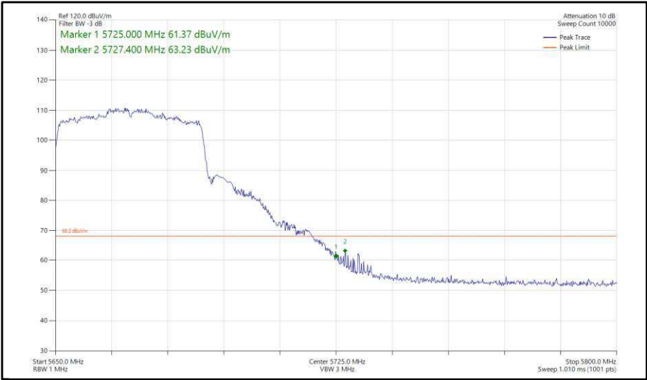
Figure 395 - 802.11ax, HE40, SU, CDD, Core 0-1 - 5670 MHz, Band Edge Frequency 5725 MHz
