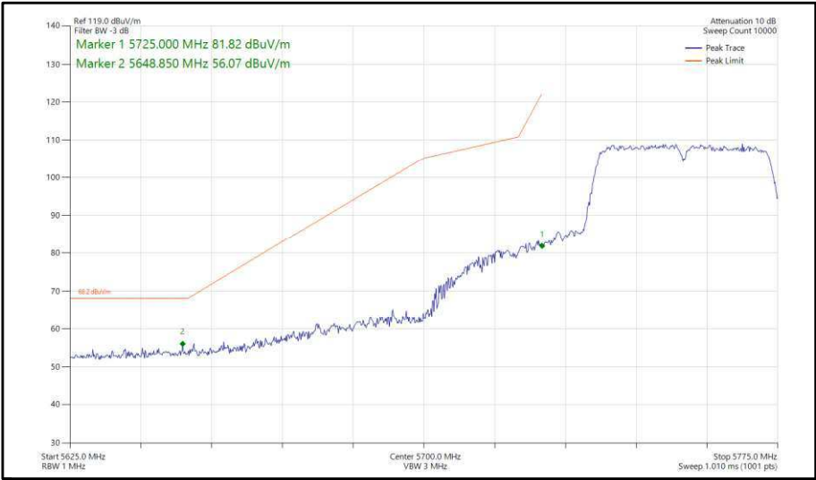
Figure 352 - 802.11n, HT40, SISO, Core 0 - 5755 MHz, Band Edge Frequency 5725 MHz
