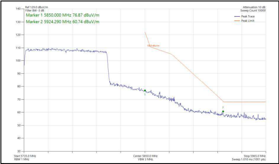
Figure 445 - 802.11ax, HE80, SU, SISO, Core 0 - 5775 MHz, Band Edge Frequency 5850 MHz
