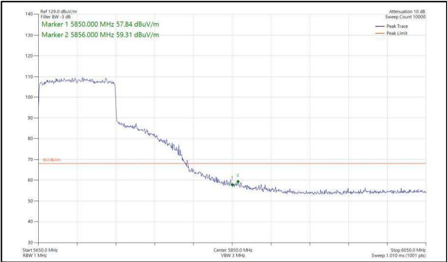
Figure 443 - 802.11ax, HE80, SU, SISO, Core 0 - 5690 MHz, Band Edge Frequency 5850 MHz
