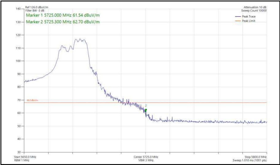
Figure 396 - 802.11ax, HE40, RU 106-56, CDD, Core 0-1 - 5670 MHz, Band Edge Frequency 5725 MHz
