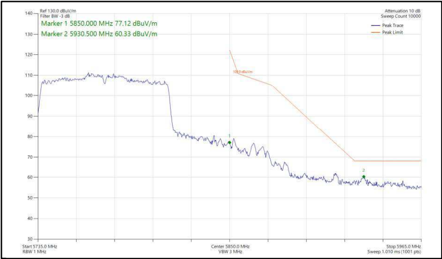
Figure 487 - 802.11ac, VHT80, SDM, Core 0-1 - 5775 MHz, Band Edge Frequency 5850 MHz
