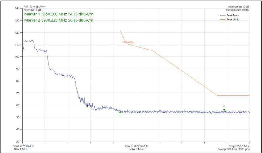
Figure 402 - 802.11ax, HE40, RU 106-53, CDD, Core 0-1 - 5795 MHz, Band Edge Frequency 5850 MHz
