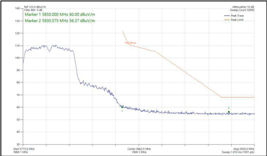
Figure 398 - 802.11n, HT40, CDD, Core 0-1 - 5795 MHz, Band Edge Frequency 5850 MHz
