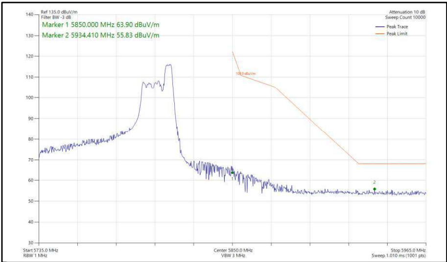
Figure 476 - 802.11ax, HE80, RU 52-52, CDD, Core 0-1 - 5775 MHz, Band Edge Frequency 5850 MHz
