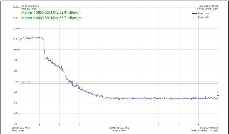
Figure 430 - 802.11ax, HE40, SU, TxBF, Core 0-1 - 5710 MHz, Band Edge Frequency 5850 MHz
