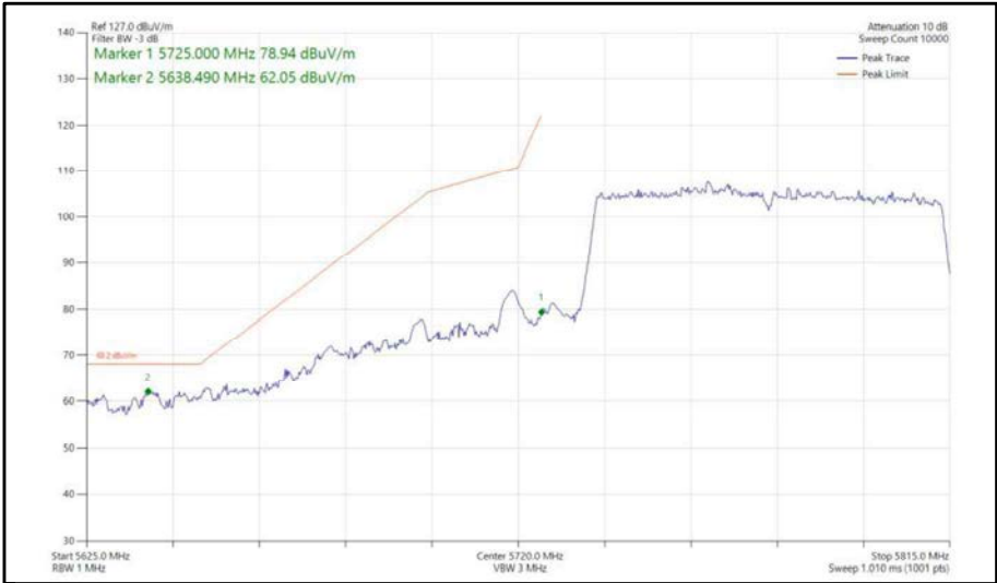
Figure 435 - 802.11ac, VHT80, SISO, Core 0 - 5775 MHz, Band Edge Frequency 5725 MHz
