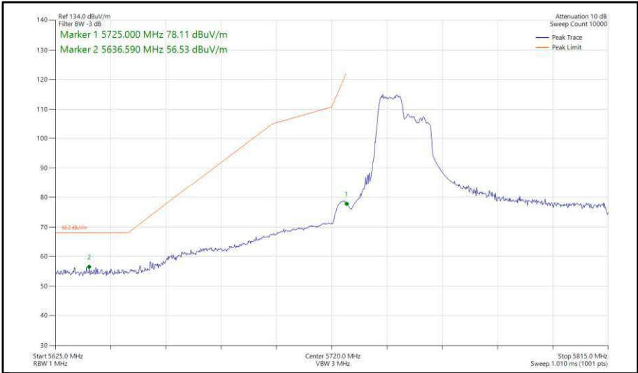
Figure 452 - 802.11ax, HE80, RU 106-53, SISO, Core 1 - 5775 MHz, Band Edge Frequency 5725 MHz
