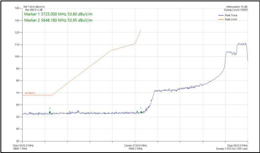
Figure 437 - 802.11ax, HE80, RU 106-60, SISO, Core 0 - 5775 MHz, Band Edge Frequency 5725 MHz
