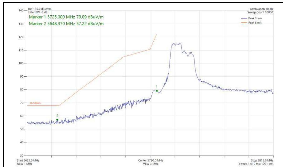
Figure 482 - 802.11ax, HE80, RU 106-53, SDM, Core 0-1 - 5775 MHz, Band Edge Frequency 5725 MHz
