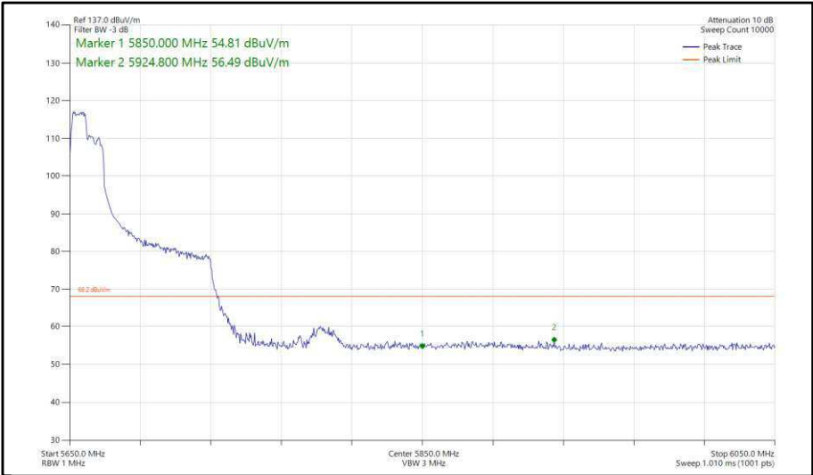
Figure 459 - 802.11ax, HE80, RU 106-53, SISO, Core 1 - 5690 MHz, Band Edge Frequency 5850 MHz
