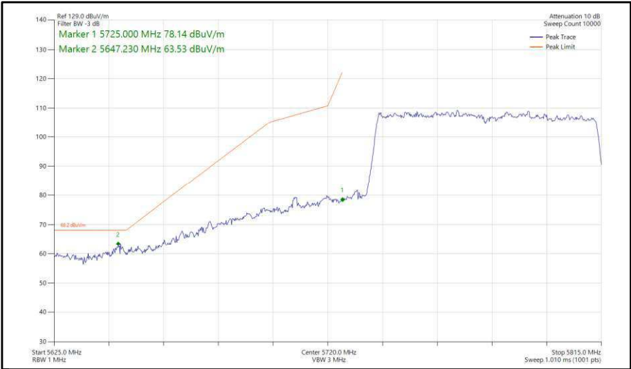
Figure 480 - 802.11ac, VHT80, SDM, Core 0-1 - 5775 MHz, Band Edge Frequency 5725 MHz
