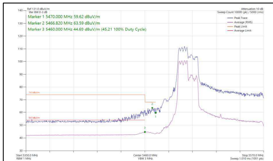
Figure 479 - 802.11ax, HE80, RU 106-53, SDM, Core 0-1 - 5530 MHz, Band Edge Frequency 5470 MHz
