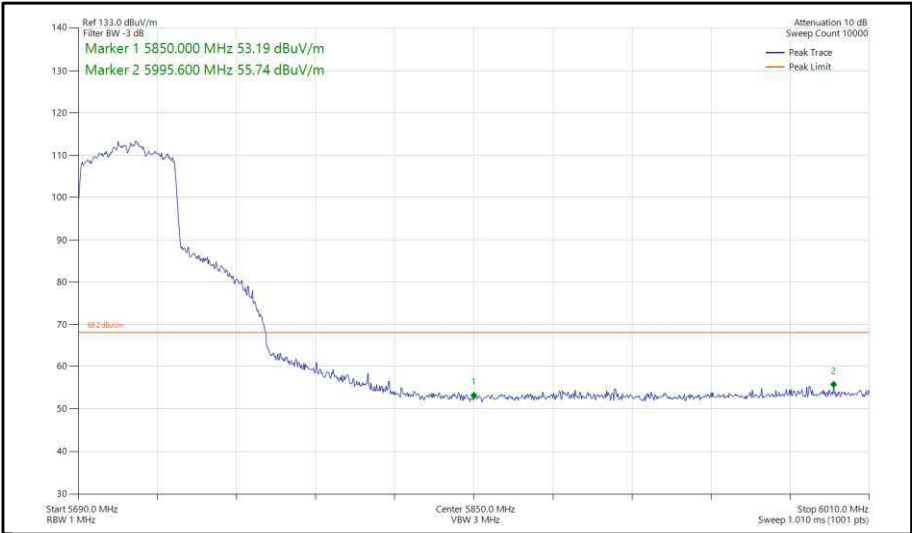
Figure 399 - 802.11ax, HE40, SU, CDD, Core 0-1 - 5710 MHz, Band Edge Frequency 5850 MHz
