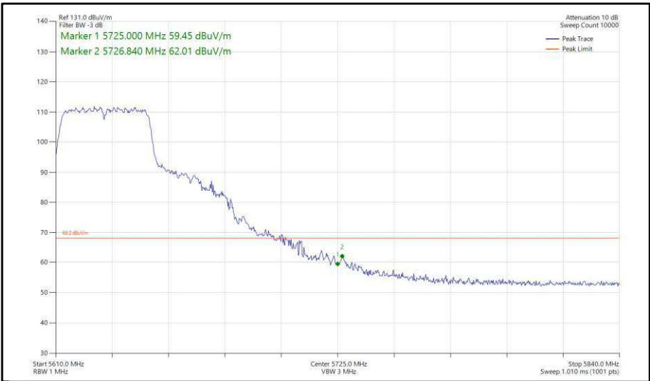
Figure 391 - 802.11n, HT40, CDD, Core 0-1 - 5630 MHz, Band Edge Frequency 5725 MHz
