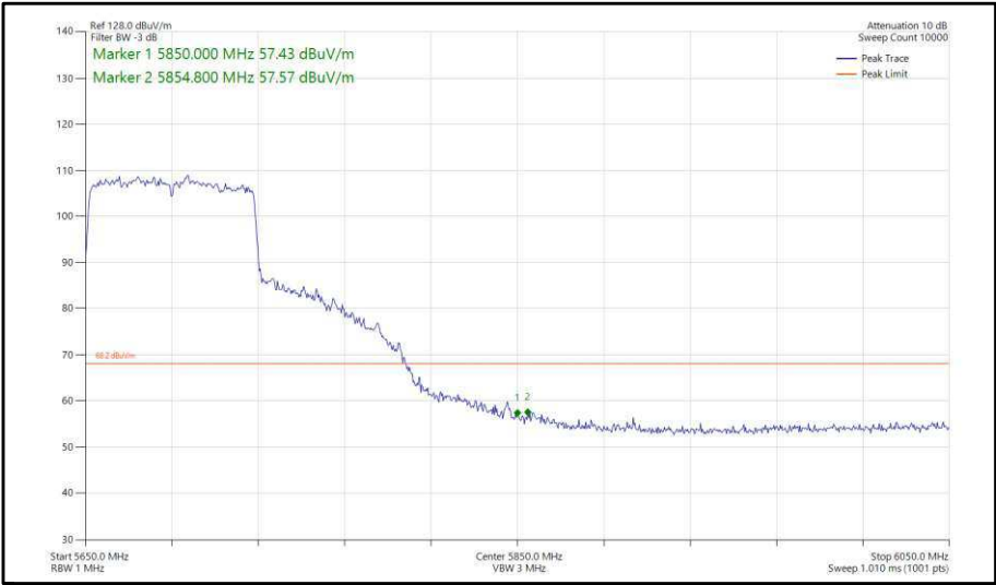
Figure 486 - 802.11ac, VHT80, SDM, Core 0-1 - 5690 MHz, Band Edge Frequency 5850 MHz
