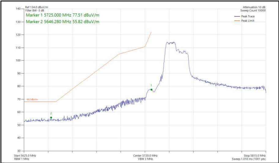
Figure 467 - 802.11ax, HE80, RU 106-53, CDD, Core 0-1 - 5775 MHz, Band Edge Frequency 5725 MHz
