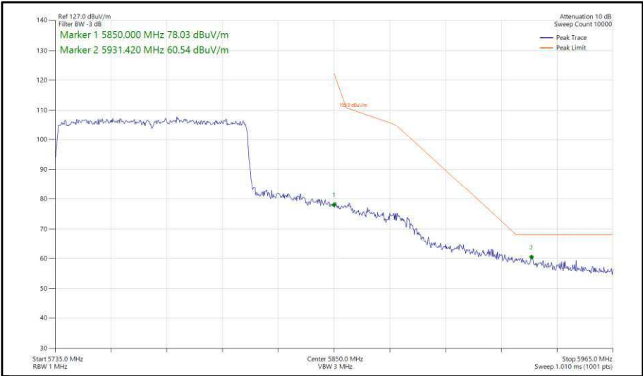
Figure 460 - 802.11ax, HE80, SU, SISO, Core 1 - 5775 MHz, Band Edge Frequency 5850 MHz
