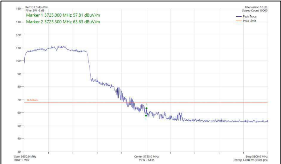
Figure 426 - 802.11ax, HE40, SU, TxBF, Core 0-1 - 5670 MHz, Band Edge Frequency 5725 MHz
