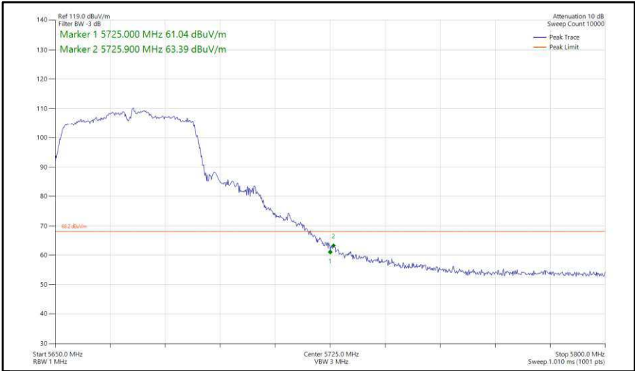
Figure 410 - 802.11n, HT40, SDM, Core 0-1 - 5670 MHz, Band Edge Frequency 5725 MHz
