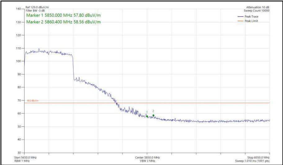
Figure 488 - 802.11ax, HE80, SU, SDM, Core 0-1 - 5690 MHz, Band Edge Frequency 5850 MHz
