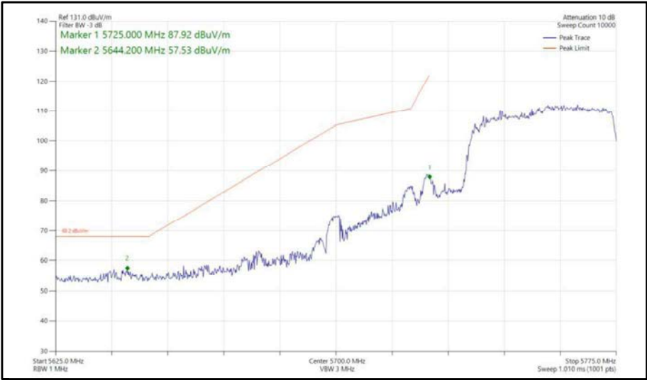
Figure 424 - 802.11ax, HE40, SU, TxBF, Core 0-1 - 5755 MHz, Band Edge Frequency 5725 MHz
