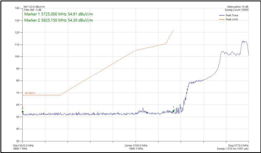
Figure 354 - 802.11ax, HE40, RU 52-44, SISO, Core 0 - 5755 MHz, Band Edge Frequency 5725 MHz
