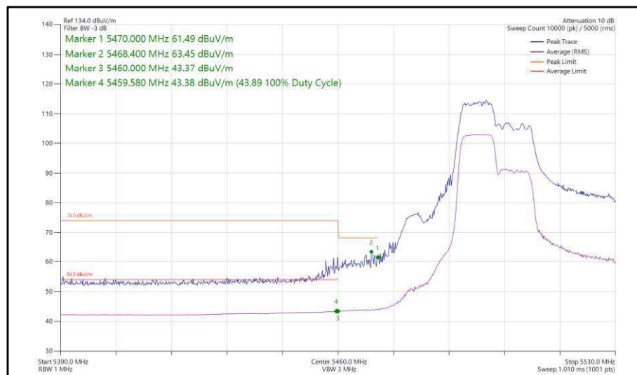
Figure 369 - 802.11ax, HE40, RU 106-53, SISO, Core 1 - 5510 MHz, Band Edge Frequency 5470 MHz
