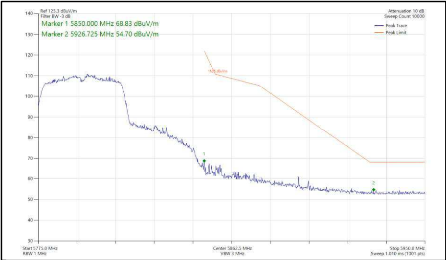
Figure 429 - 802.11ac, VHT40, TxBF, Core 0-1 - 5795 MHz, Band Edge Frequency 5850 MHz
