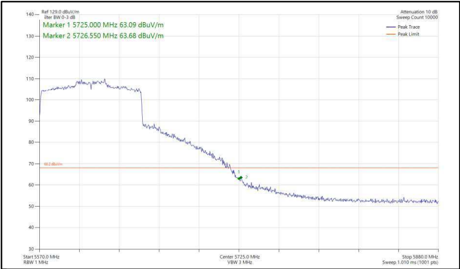
Figure 484 - 802.11ax, HE80, SU, SDM, Core 0-1 - 5610 MHz, Band Edge Frequency 5725 MHz
