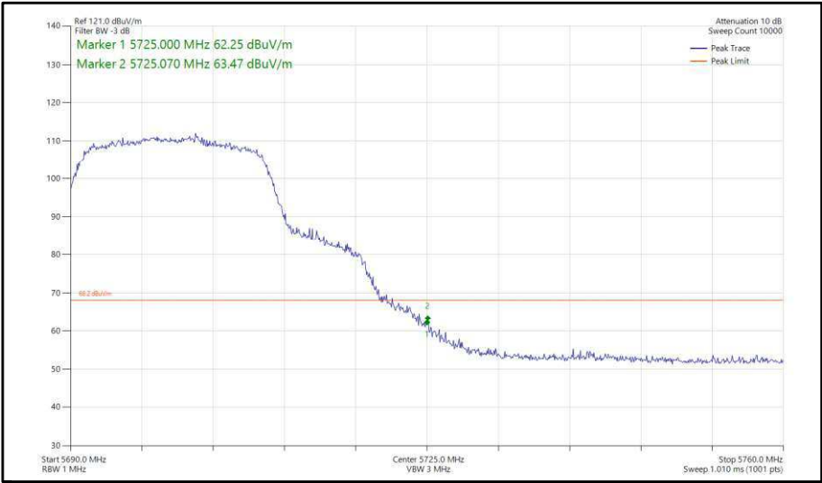
Figure 346 - 802.11n, HT20, TxBF, Core 0-1 - 5700 MHz, Band Edge Frequency 5725 MHz
