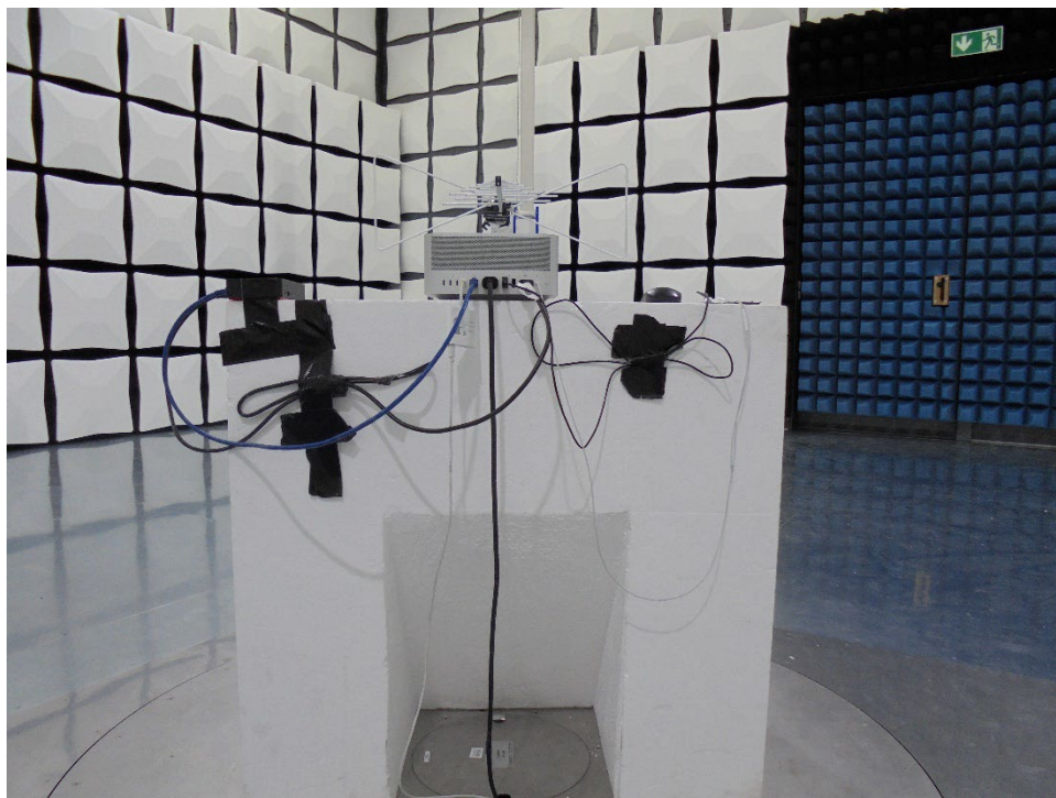
Figure 1 - Radiated Disturbance - Below 1 GHz
