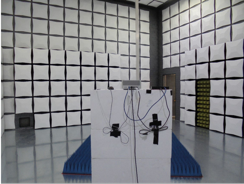
Figure 2 Radiated Disturbance - Above 1 GHz
