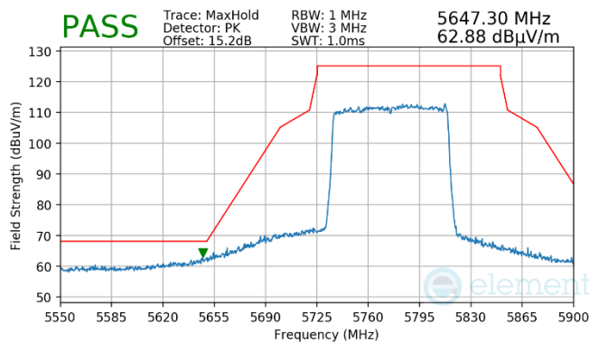
Plot 7-812. Antenna WF8 (Pk, Ch.155, 802.11ax(SU), MCS4)
