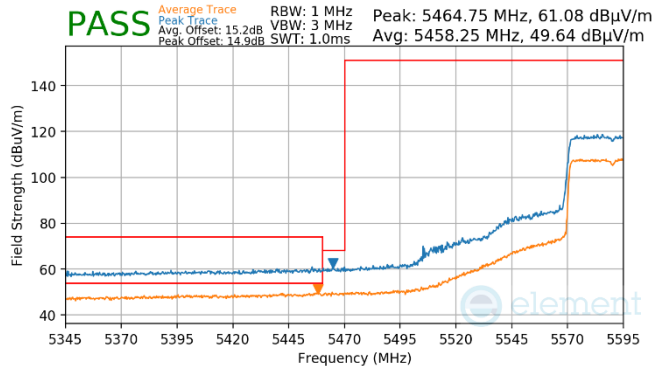
Plot 7-760. (FCC Only) Antenna WF8 (Pk & Avg, Ch.118, 80.11ax(SU), MCS2)
