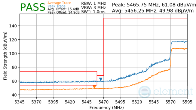
Plot 7-761. (FCC Only) Antenna WF8 (Pk & Avg, Ch.118, 80.11ax(SU), MCS4)
