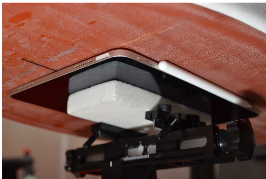
Wireless Power Transfer Test Setup Photo 12 – Back Side at 0mm
