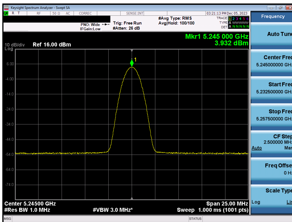
Plot 7-39. FCC/ISED PSD Antenna 3a (BDR, iPA– 5245MHz)
