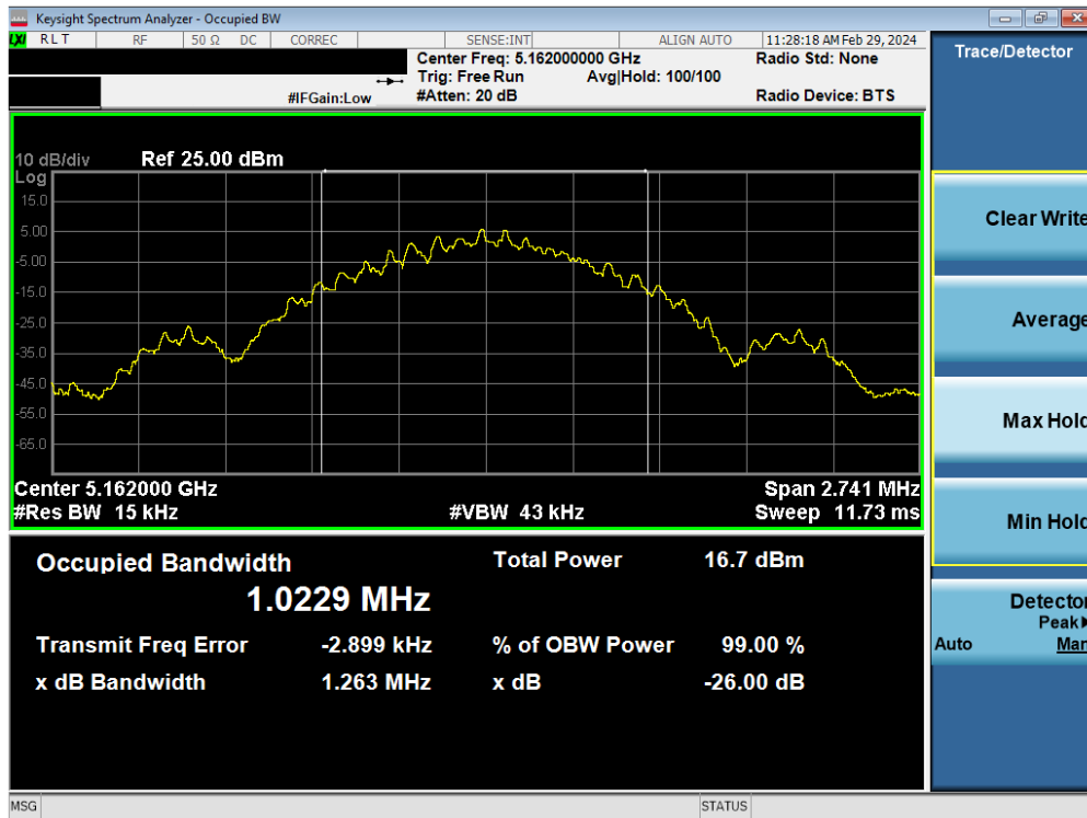
Plot 7-7. 26dB BW & 99% OBW Antenna 3a (BDR GFSK, ePA– 5162MHz)
