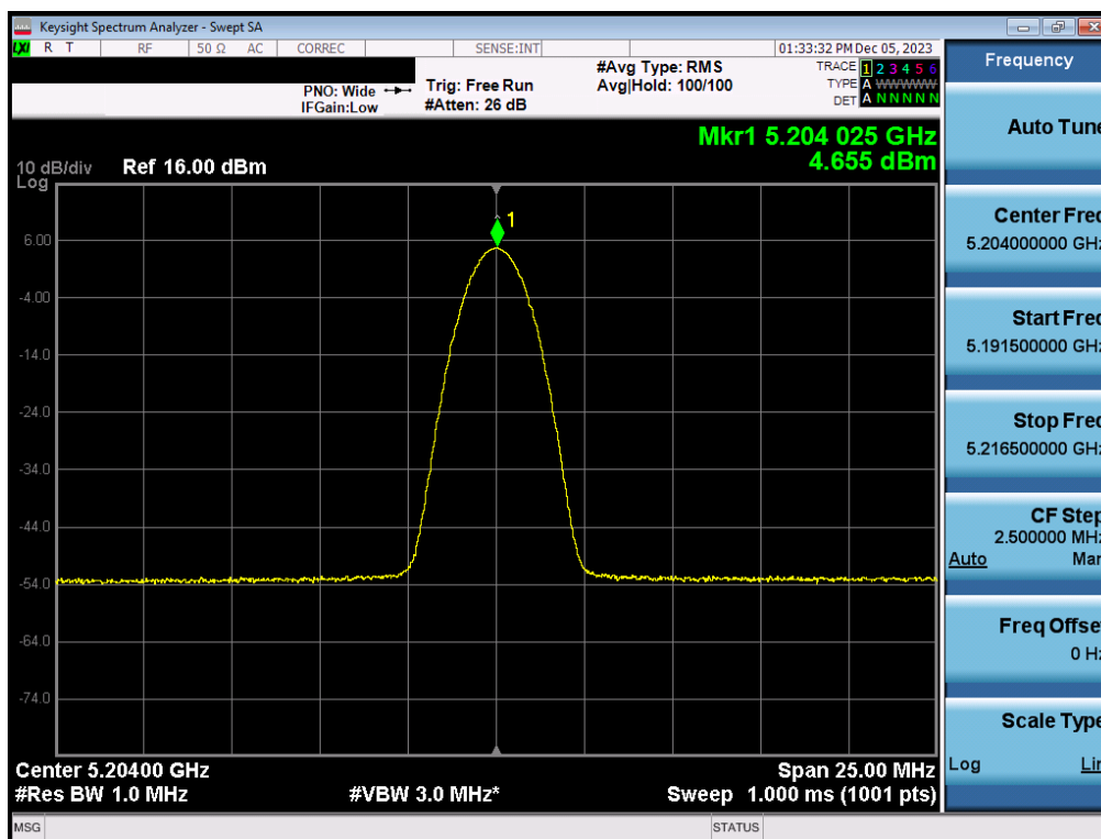
Plot 7-23. FCC/ISED PSD Antenna 3c (BDR, iPA – 5204MHz)
