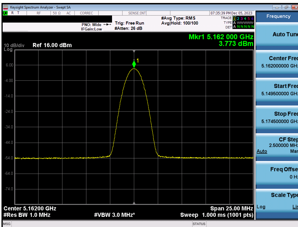
Plot 7-49. FCC/ISED PSD Antenna 1b (BDR, iPA - 5162MHz)
