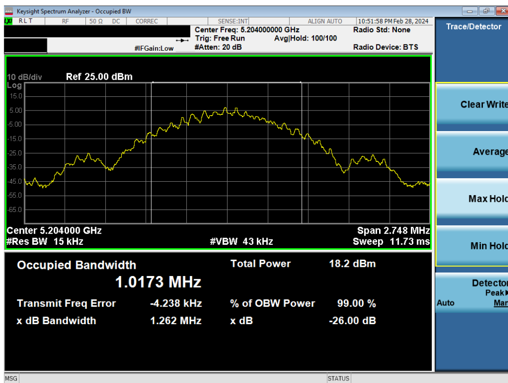
Plot 7-2. 26dB BW & 99% OBW Antenna 3c (BDR GFSK, ePA- 5204MHz)
