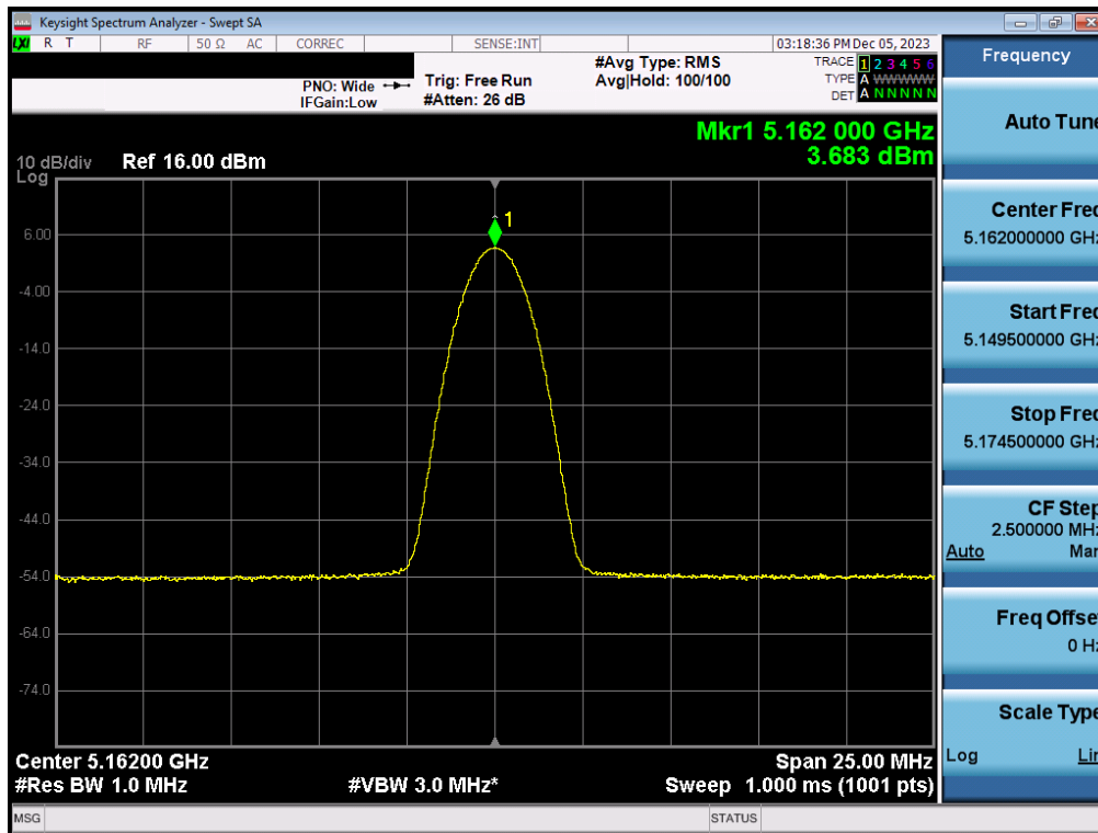
Plot 7-37. FCC/ISED PSD Antenna 3a (BDR, iPA - 5162MHz)
