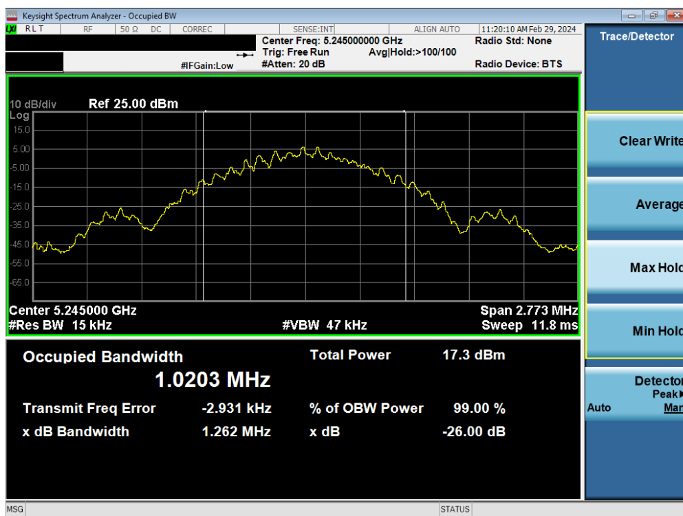
Plot 7-6. 26dB BW & 99% OBW Antenna 3a (BDR GFSK, ePA – 5245MHz)
