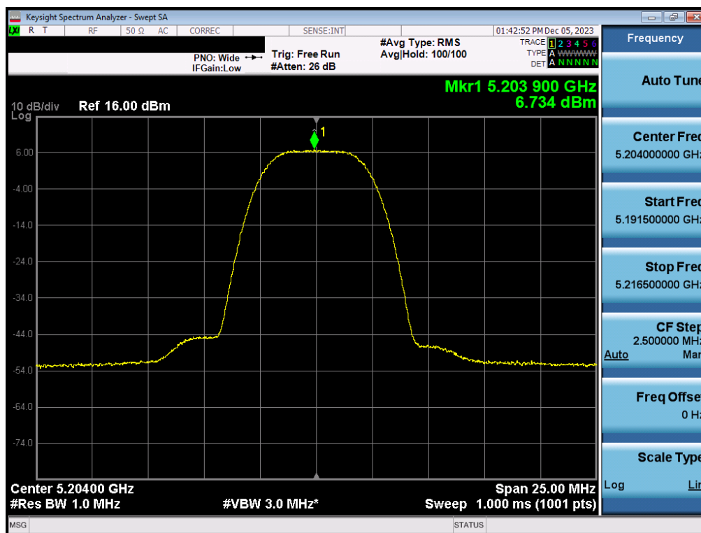
Plot 7-44. FCC PSD Antenna 3c (HDR8, ePA – 5204MHz)
