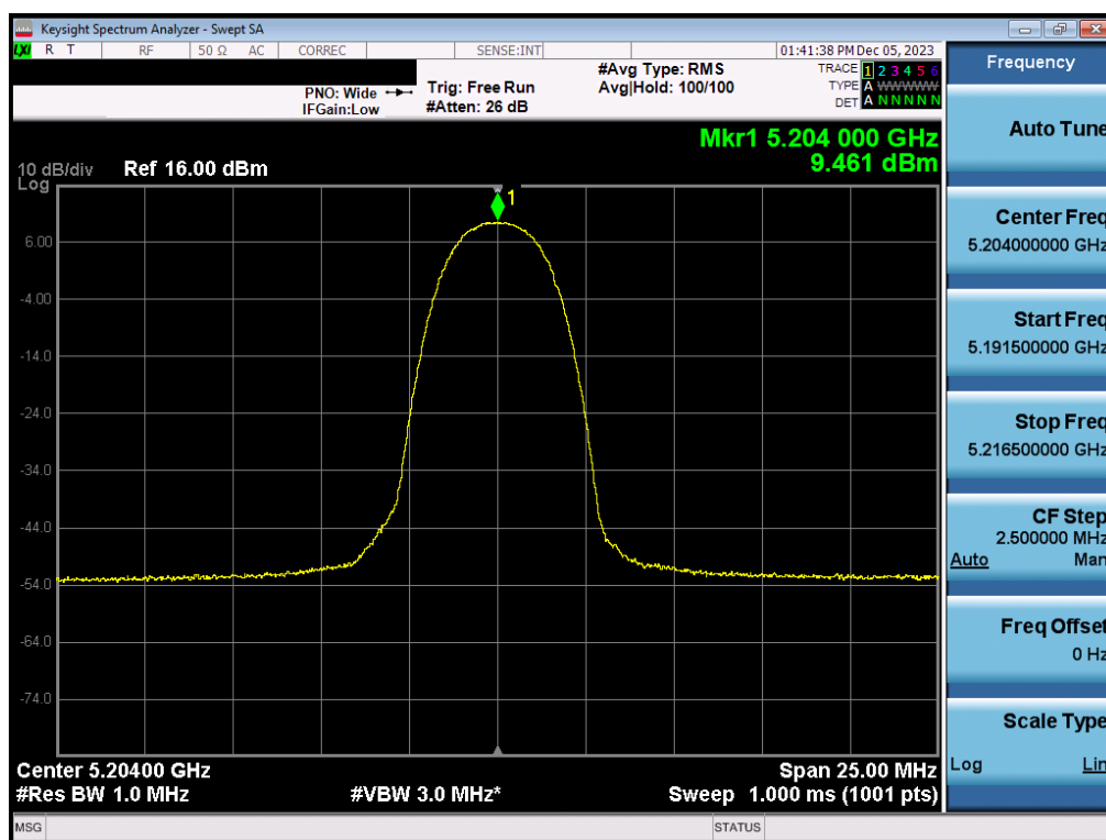
Plot 7-38. FCC PSD Antenna 3c (HDR4, ePA – 5204MHz)
