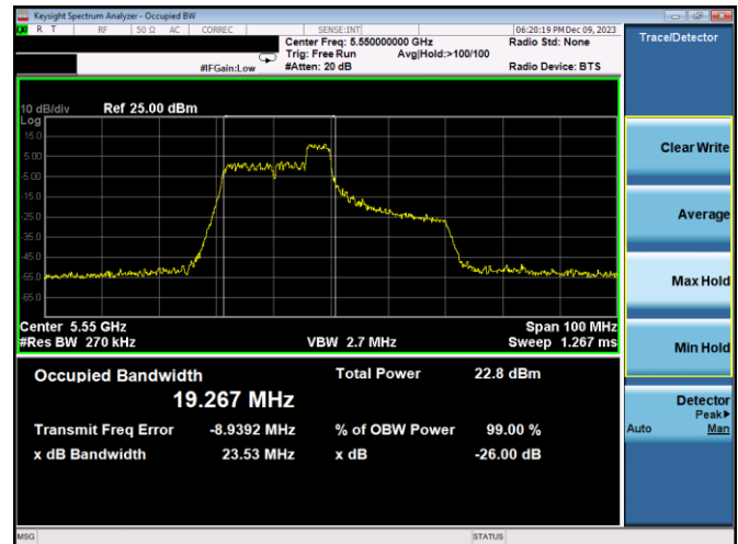
Plot 7-34. 26dB BW & 99% OBW Antenna 3c (40MHz BW 11ax Index 40 - RU52 - Ch.110)
