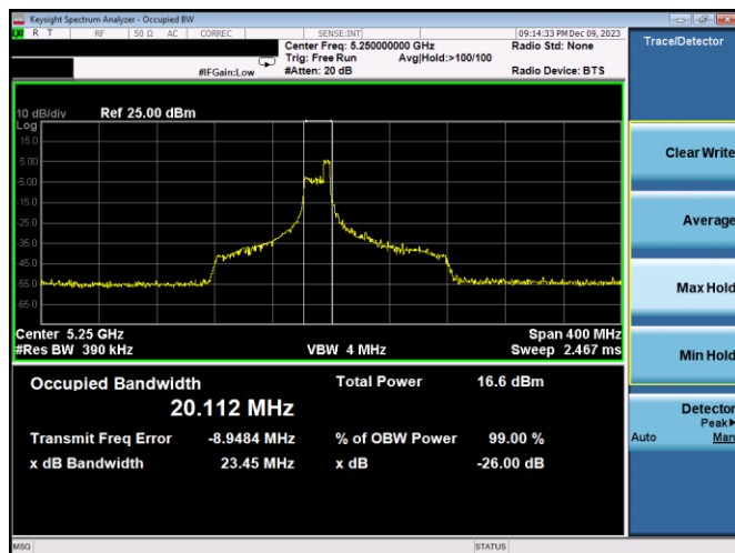
Plot 7-58. 26dB BW & 99% OBW Antenna 3a (160MHz BW 11ax Index 44 – RU52 – Ch.50)
