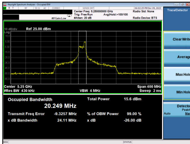
Plot 7-14. 26dB BW & 99% OBW Antenna 3c (160MHz BW 11ax Index 44 - RU52 - Ch.50)
