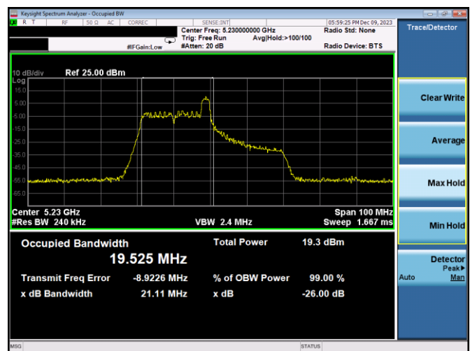
Plot 7-6. 26dB BW & 99% OBW Antenna 3c (40MHz BW 11ax Index 8 – RU26 – Ch.46)
