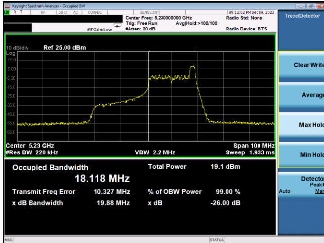
Plot 7-51. 26dB BW & 99% OBW Antenna 3a (40MHz BW 11ax Index 17 – RU26 – Ch.46)
