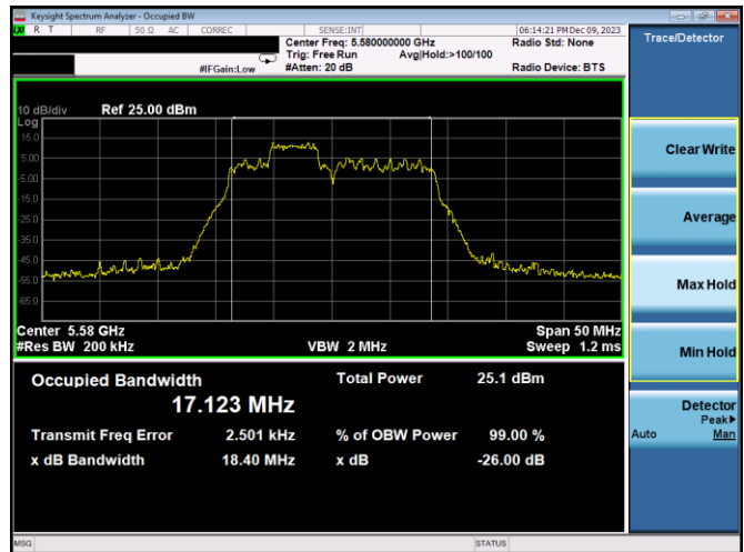
Plot 7-30. 26dB BW & 99% OBW Antenna 3c (20MHz BW 11ax Index 38 – RU52 – Ch.116)
