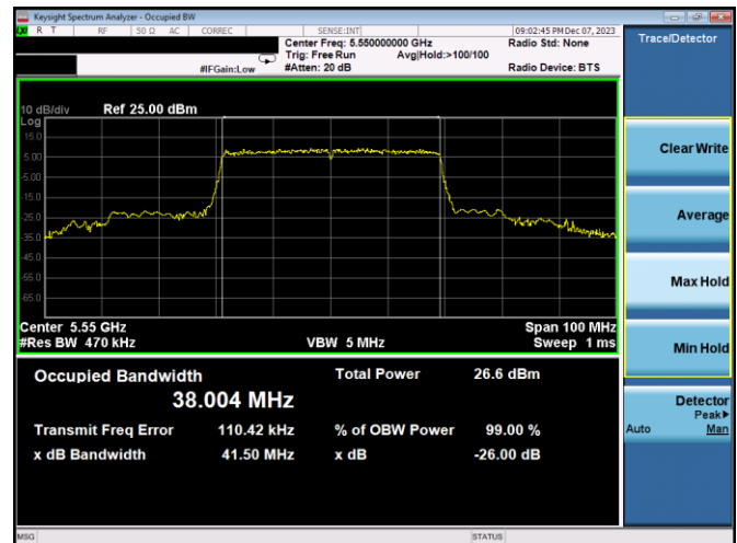
Plot 7-36. 26dB BW & 99% OBW Antenna 3c (40MHz BW 11ax - RU484 - Ch.110)
