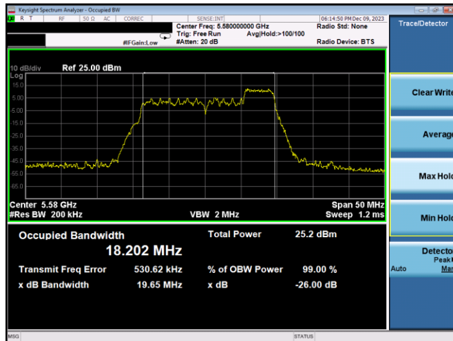
Plot 7-31. 26dB BW & 99% OBW Antenna 3c (20MHz BW 11ax Index 40 - RU52 - Ch.116)
