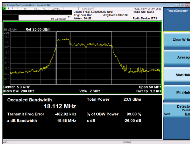
Plot 7-61. 26dB BW & 99% OBW Antenna 3a (20MHz BW 11ax Index 37 – RU52 – Ch.60)
