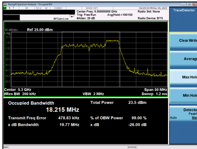
Plot 7-19. 26dB BW & 99% OBW Antenna 3c (20MHz BW 11ax Index 40 – RU52 – Ch.60)
