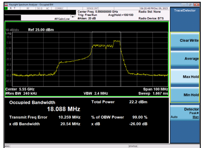
Plot 7-35. 26dB BW & 99% OBW Antenna 3c (40MHz BW 11ax Index 44 - RU52 - Ch.110)
