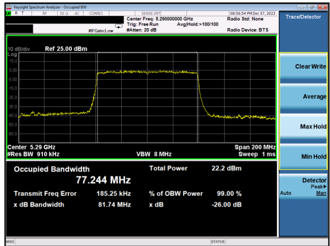
Plot 7-28. 26dB BW & 99% OBW Antenna 3c (80MHz BW 11ax – RU996 – Ch.58)
