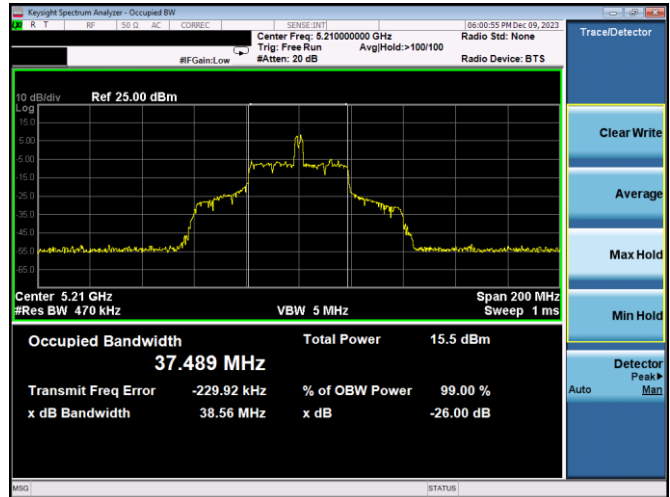
Plot 7-10. 26dB BW & 99% OBW Antenna 3c (80MHz BW 11ax Index 18 – RU26 – Ch.42)
