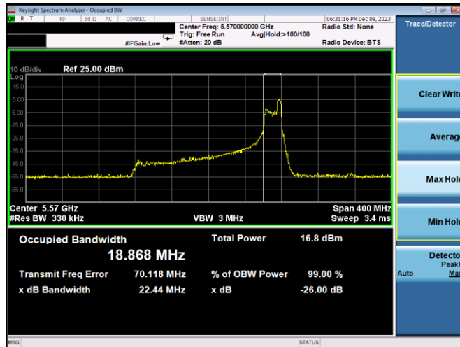
Plot 7-43. 26dB BW & 99% OBW Antenna 3c (160MHz BW 11ax Index 52 – RU52 – Ch.114)
