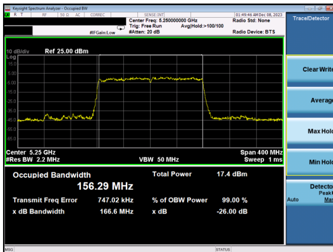
Plot 7-60. 26dB BW & 99% OBW Antenna 3a (160MHz BW 11ax – RU996x2 – Ch.50)
