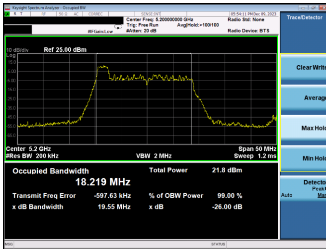
Plot 7-1. 26dB BW & 99% OBW Antenna 3c (20MHz BW 11ax Index 0 – RU26 – Ch.40)
