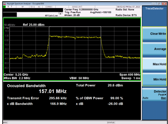
Plot 7-16. 26dB BW & 99% OBW Antenna 3c (160MHz BW 11ax - RU996x2 - Ch.50)
