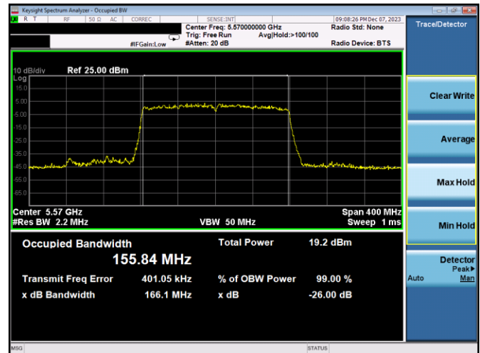
Plot 7-44. 26dB BW & 99% OBW Antenna 3c (160MHz BW 11ax – RU996x2 – Ch.114)
