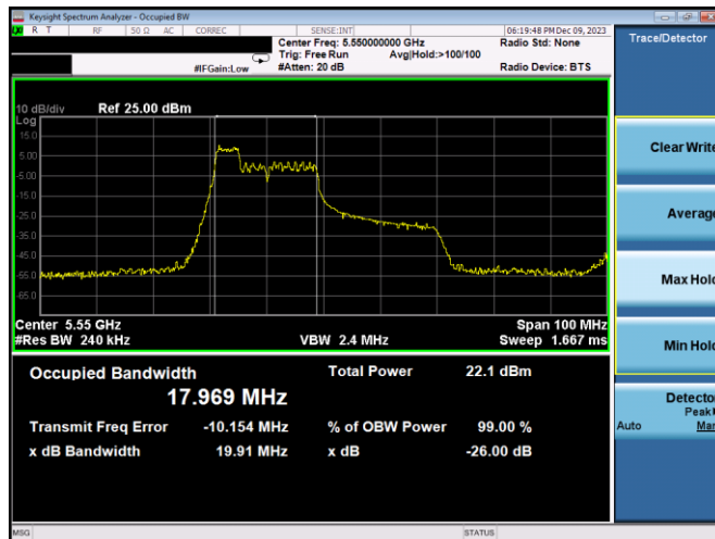
Plot 7-33. 26dB BW & 99% OBW Antenna 3c (40MHz BW 11ax Index 37 - RU52 - Ch.110)
