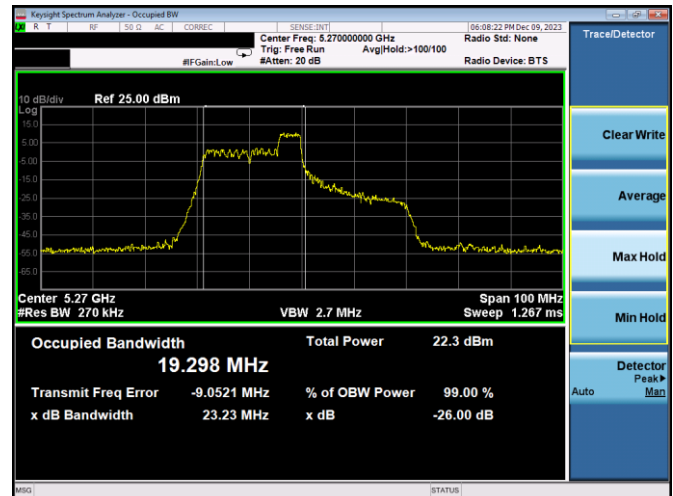
Plot 7-22. 26dB BW & 99% OBW Antenna 3c (40MHz BW 11ax Index 40 – RU52 – Ch.54)
