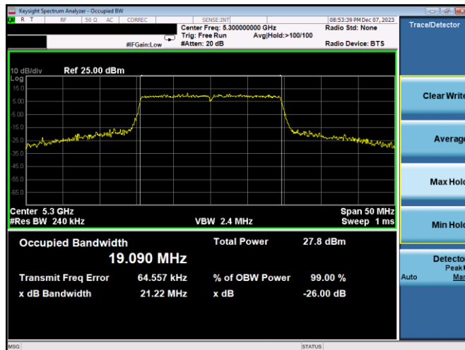
Plot 7-20. 26dB BW & 99% OBW Antenna 3c (20MHz BW 11ax – RU242 – Ch.60)
