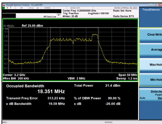
Plot 7-3. 26dB BW & 99% OBW Antenna 3c (20MHz BW 11ax Index 8– RU26 – Ch.40)
