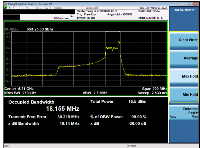
Plot 7-11. 26dB BW & 99% OBW Antenna 3c (80MHz BW 11ax Index 36 – RU26 – Ch.42)
