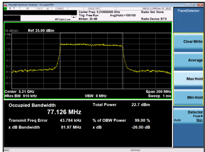
Plot 7-12. 26dB BW & 99% OBW Antenna 3c (80MHz BW 11ax – RU996 – Ch.42)
