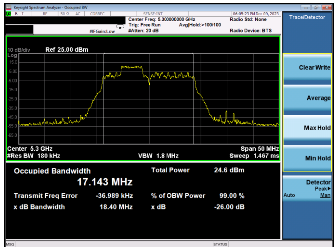
Plot 7-18. 26dB BW & 99% OBW Antenna 3c (20MHz BW 11ax Index 38 - RU52 - Ch.60)
