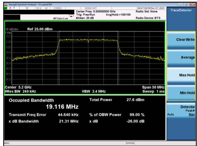
Plot 7-4. 26dB BW & 99% OBW Antenna 3c (20MHz BW 11ax– RU242 – Ch.40)
