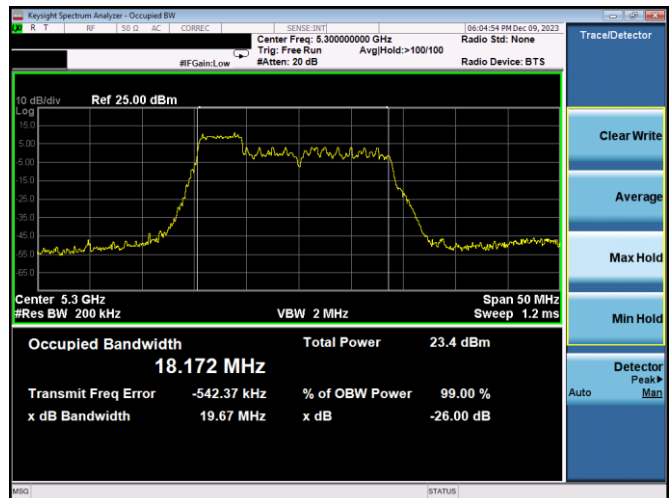
Plot 7-17. 26dB BW & 99% OBW Antenna 3c (20MHz BW 11ax Index 37 - RU52 - Ch.60)
