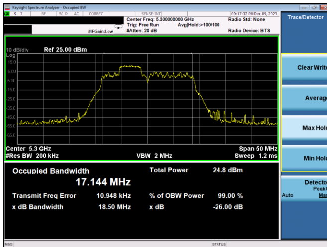
Plot 7-62. 26dB BW & 99% OBW Antenna 3a (20MHz BW 11ax Index 38 – RU52 – Ch.60)
