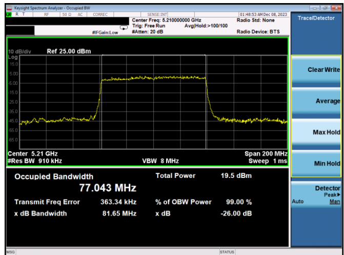
Plot 7-56. 26dB BW & 99% OBW Antenna 3a (80MHz BW 11ax – RU996 – Ch.42)
