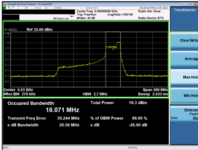
Plot 7-39. 26dB BW & 99% OBW Antenna 3c (80MHz BW 11ax Index 52 – RU52 – Ch.106)
