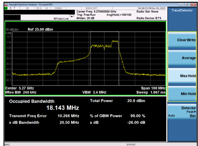
Plot 7-23. 26dB BW & 99% OBW Antenna 3c (40MHz BW 11ax Index 44 – RU52 – Ch.54)
