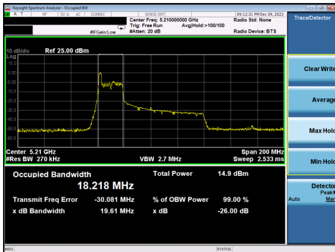
Plot 7-53. 26dB BW & 99% OBW Antenna 3a (80MHz BW 11ax Index 0 – RU26 – Ch.42)
