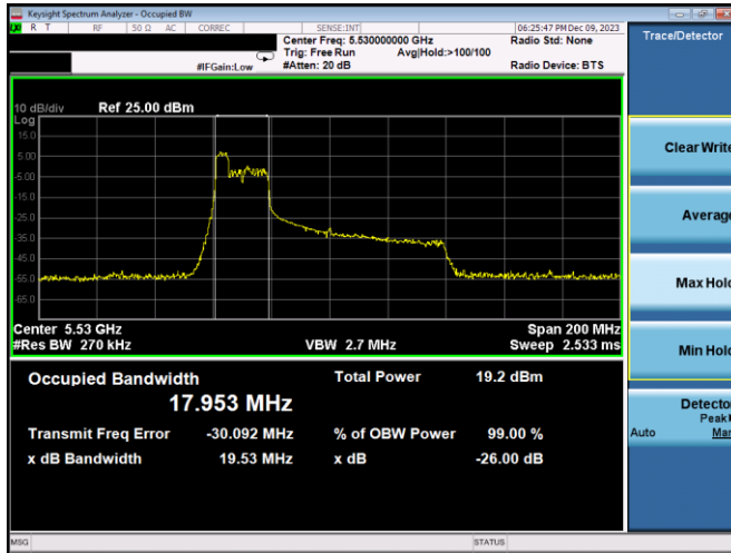
Plot 7-37. 26dB BW & 99% OBW Antenna 3c (80MHz BW 11ax Index 37 – RU52 – Ch.106)
