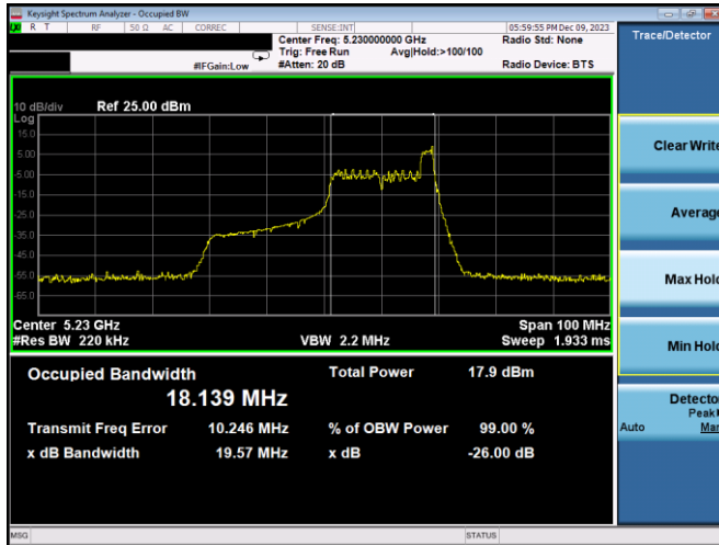
Plot 7-7. 26dB BW & 99% OBW Antenna 3c (40MHz BW 11ax Index 17 – RU26 – Ch.46)
