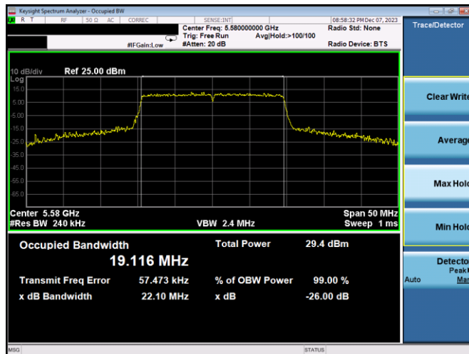
Plot 7-32. 26dB BW & 99% OBW Antenna 3c (20MHz BW 11ax - RU242 - Ch.116)
