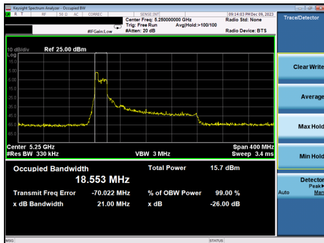
Plot 7-57. 26dB BW & 99% OBW Antenna 3a (160MHz BW 11ax Index 37 – RU52 – Ch.50)
