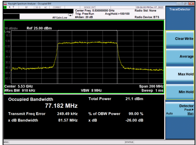
Plot 7-40. 26dB BW & 99% OBW Antenna 3c (80MHz BW 11ax – RU996 – Ch.106)
