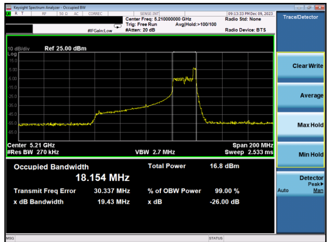
Plot 7-55. 26dB BW & 99% OBW Antenna 3a (80MHz BW 11ax Index 36 – RU26 – Ch.42)
