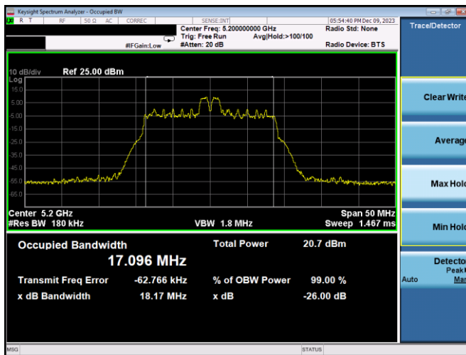
Plot 7-2. 26dB BW & 99% OBW Antenna 3c (20MHz BW 11ax Index 4 – RU26 – Ch.40)
