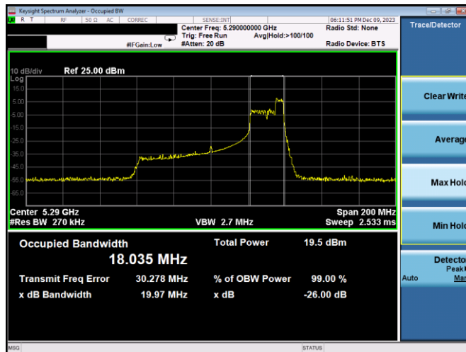
Plot 7-27. 26dB BW & 99% OBW Antenna 3c (80MHz BW 11ax Index 52 – RU52 – Ch.58)
