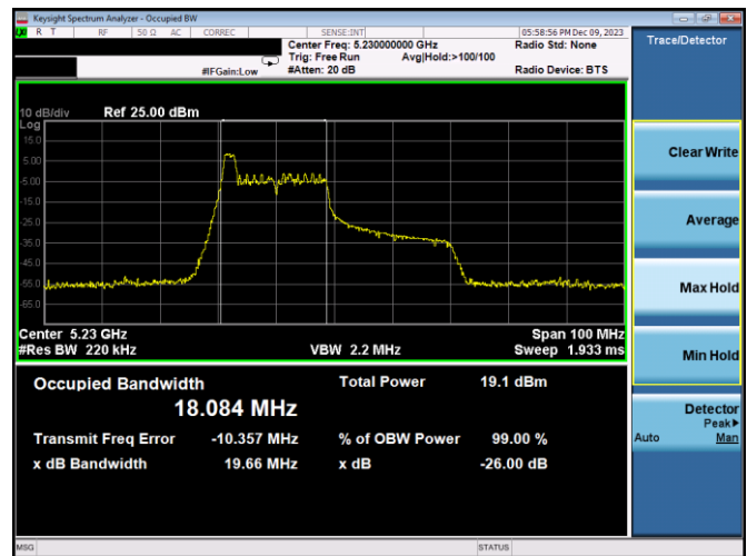
Plot 7-5. 26dB BW & 99% OBW Antenna 3c (40MHz BW 11ax Index 0 – RU26 – Ch.46)
