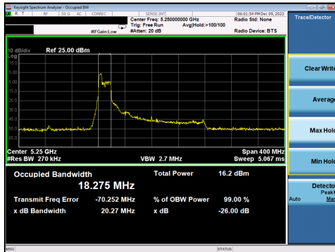
Plot 7-13. 26dB BW & 99% OBW Antenna 3c (160MHz BW 11ax Index 37 - RU52 - Ch.50)
