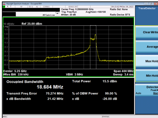
Plot 7-59. 26dB BW & 99% OBW Antenna 3a (160MHz BW 11ax Index 52 – RU52 – Ch.50)
