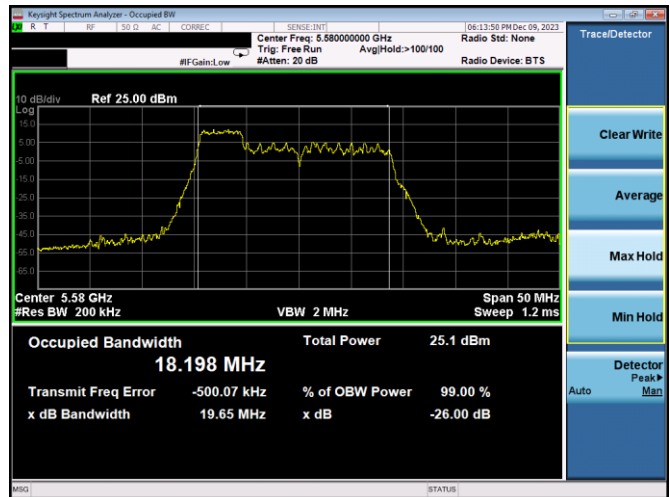
Plot 7-29. 26dB BW & 99% OBW Antenna 3c (20MHz BW 11ax Index 37 – RU52 – Ch.116)
