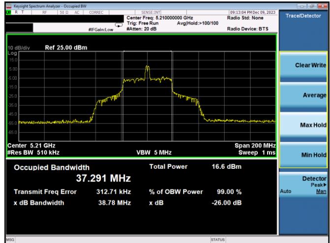
Plot 7-54. 26dB BW & 99% OBW Antenna 3a (80MHz BW 11ax Index 18 – RU26 – Ch.42)
