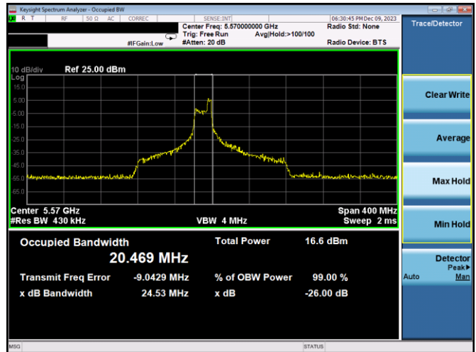
Plot 7-42. 26dB BW & 99% OBW Antenna 3c (160MHz BW 11ax Index 44 – RU52 – Ch.114)
