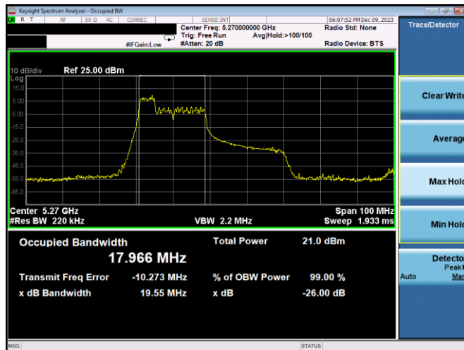
Plot 7-21. 26dB BW & 99% OBW Antenna 3c (40MHz BW 11ax Index 37 – RU52 – Ch.54)
