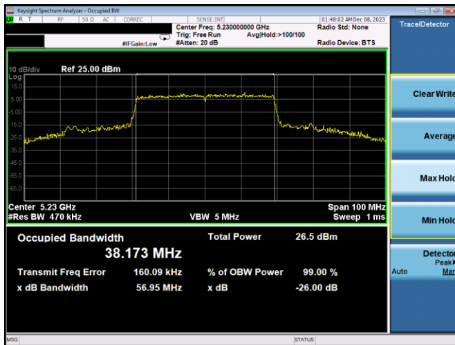
Plot 7-52. 26dB BW & 99% OBW Antenna 3a (40MHz BW 11ax – RU484 – Ch.46)
