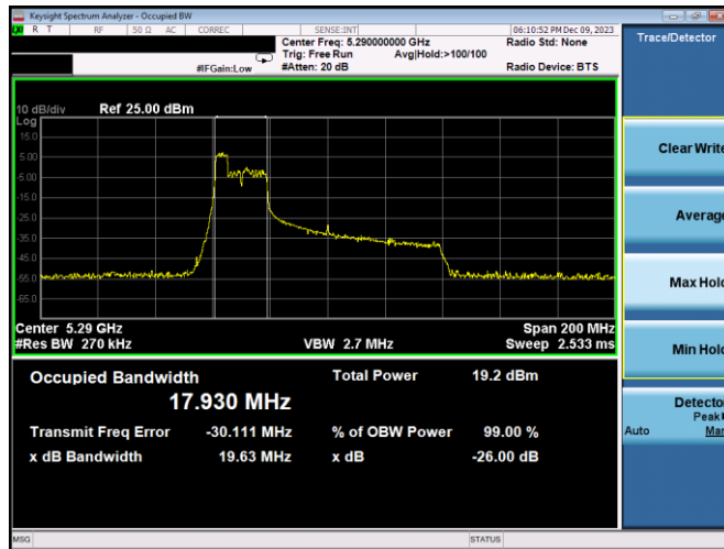
Plot 7-25. 26dB BW & 99% OBW Antenna 3c (80MHz BW 11ax Index 37 – RU52 – Ch.58)
