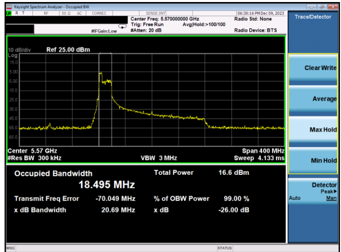
Plot 7-41. 26dB BW & 99% OBW Antenna 3c (160MHz BW 11ax Index 37 – RU52 – Ch.114)
