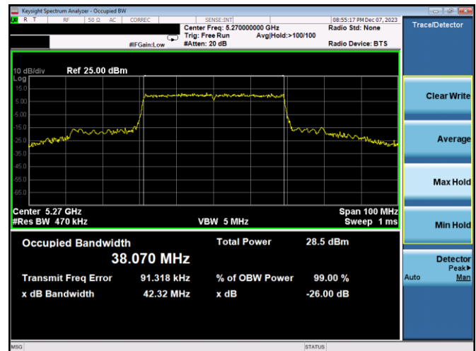
Plot 7-24. 26dB BW & 99% OBW Antenna 3c (40MHz BW 11ax – RU484 – Ch.54)
