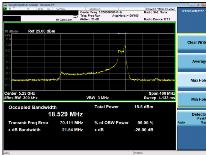
Plot 7-15. 26dB BW & 99% OBW Antenna 3c (160MHz BW 11ax Index 52 - RU52 - Ch.50)
