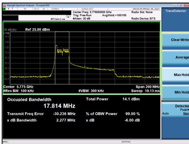
Plot 7-153. 6dB BW & 99% OBW Antenna 3a (80MHz BW 11ax Index 0 – RU26 – Ch.155)
