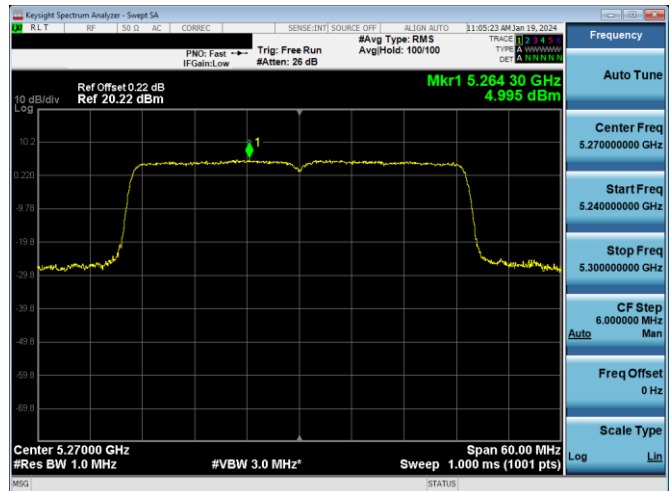
Plot 7-263. PSD Antenna 3a (40MHz BW 11ax - RU484 - Ch.54)
