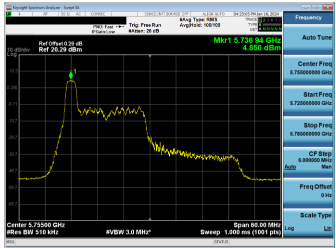
Plot 7-217. PSD Antenna 3c (40MHz BW 11ax Index 0 - RU26 - Ch.151)
