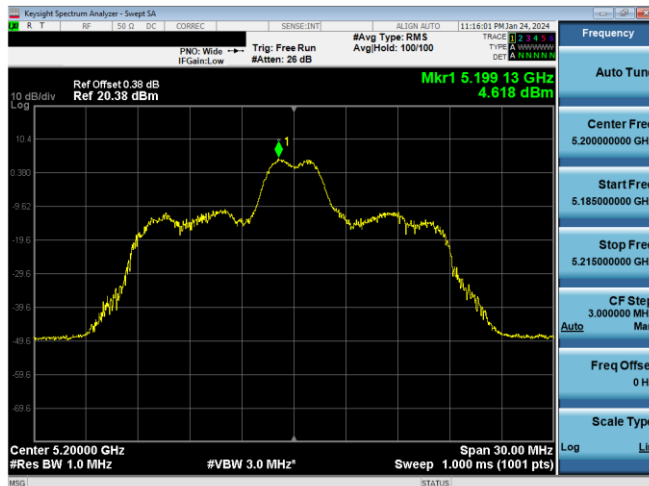
Plot 7-226. ISED PSD Antenna 3c (20MHz BW 11ax Index 4 - RU26 - Ch.40)
