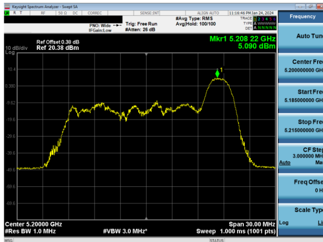
Plot 7-227. ISED PSD Antenna 3c (20MHz BW 11ax Index 8- RU26 - Ch.40)
