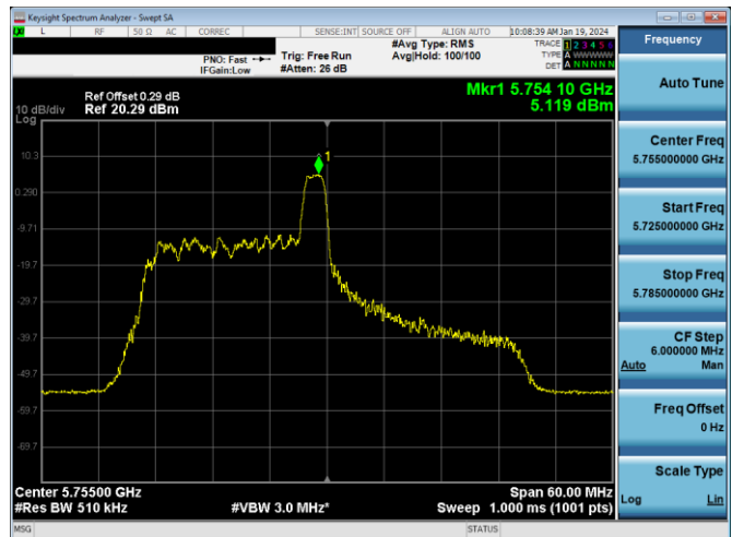
Plot 7-289. PSD Antenna 3a (40MHz BW 11ax Index 8 - RU26 - Ch.151)
