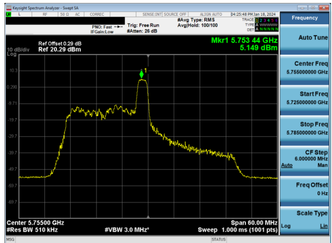
Plot 7-218. PSD Antenna 3c (40MHz BW 11ax Index 8 - RU26 - Ch.151)
