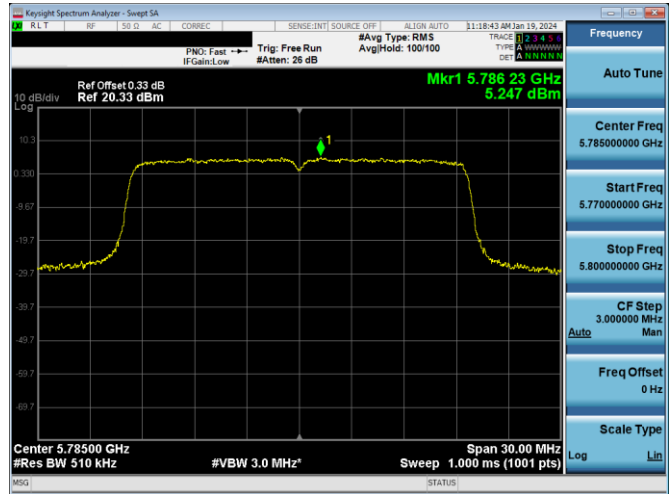
Plot 7-287. PSD Antenna 3a (20MHz BW 11ax - RU242 - Ch.157)
