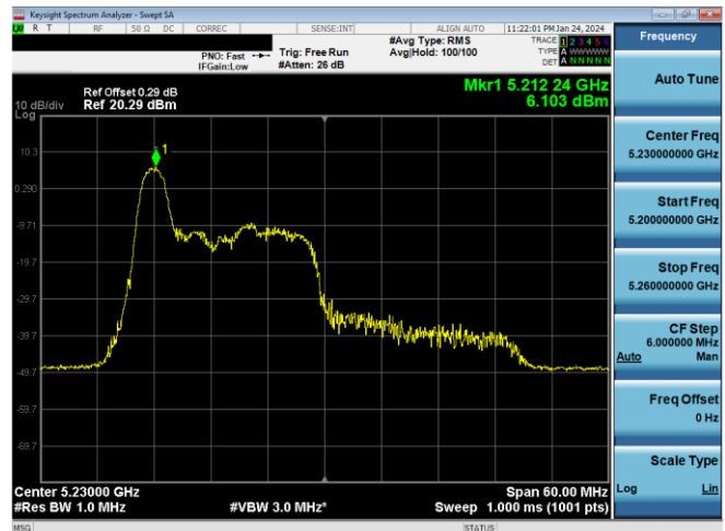
Plot 7-229. ISED PSD Antenna 3c (40MHz BW 11ax Index 0 - RU26 - Ch.46)
