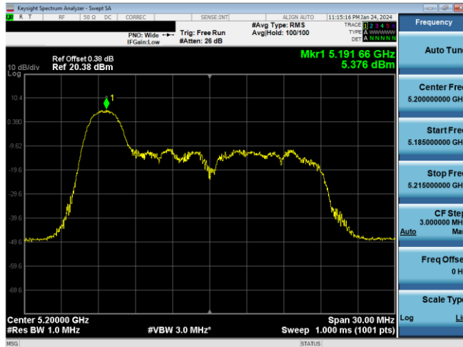
Plot 7-225. ISED PSD Antenna 3c (20MHz BW 11ax Index 0 - RU26 - Ch.40)
