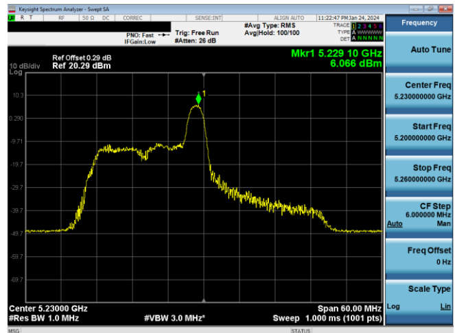
Plot 7-230. ISED PSD Antenna 3c (40MHz BW 11ax Index 8 - RU26 - Ch.46)
