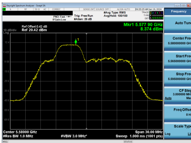
Plot 7-269. PSD Antenna 3a (20MHz BW 11ax Index 38 – RU52 – Ch.116)
