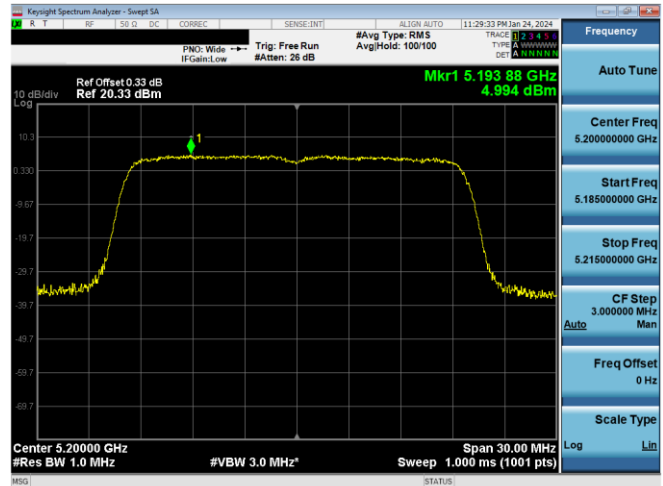
Plot 7-228. ISED PSD Antenna 3c (20MHz BW 11ax- RU242 - Ch.40)
