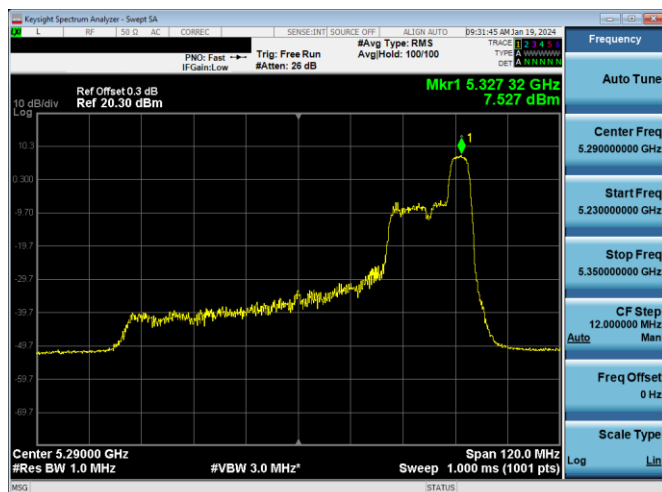
Plot 7-266. PSD Antenna 3a (80MHz BW 11ax Index 52 – RU52 – Ch.58)
