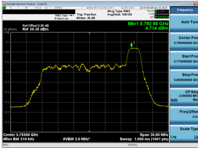
Plot 7-286. PSD Antenna 3a (20MHz BW 11ax Index 8 - RU26 - Ch.157)
