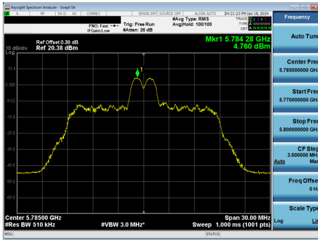
Plot 7-214. PSD Antenna 3c (20MHz BW 11ax Index 4 - RU26 - Ch.157)
