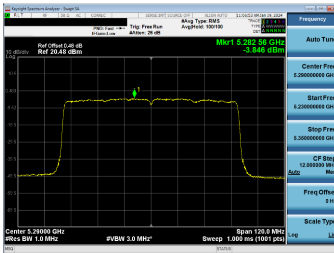
Plot 7-267. PSD Antenna 3a (80MHz BW 11ax – RU96 – Ch.58)
