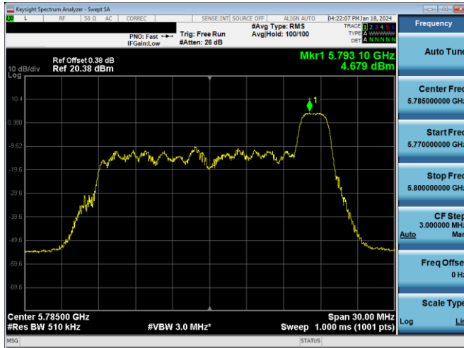
Plot 7-215. PSD Antenna 3c (20MHz BW 11ax Index 8 - RU26 - Ch.157)
