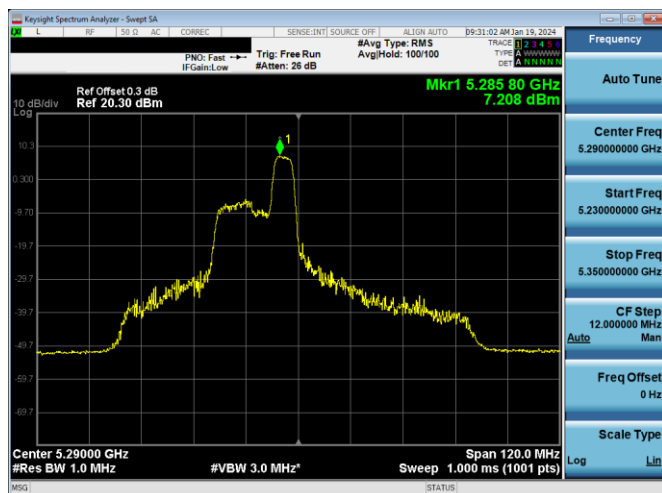
Plot 7-265. PSD Antenna 3a (80MHz BW 11ax Index 44 – RU52 – Ch.58)
