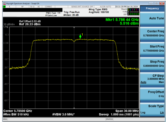
Plot 7-216. PSD Antenna 3c (20MHz BW 11ax - RU242 - Ch.157)
