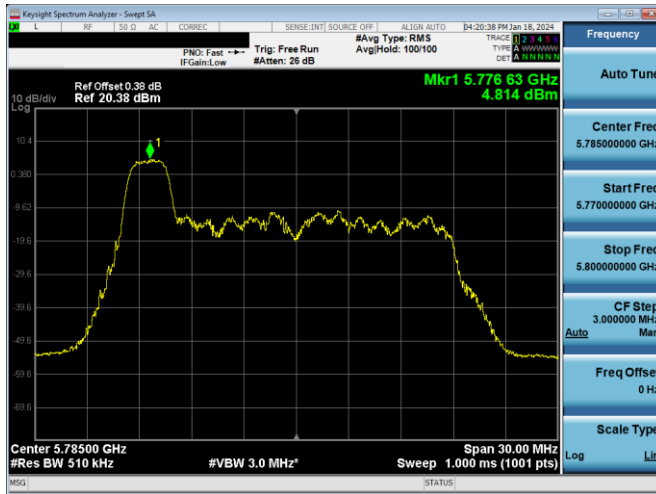
Plot 7-213. PSD Antenna 3c (20MHz BW 11ax Index 0 - RU26 - Ch.157)
