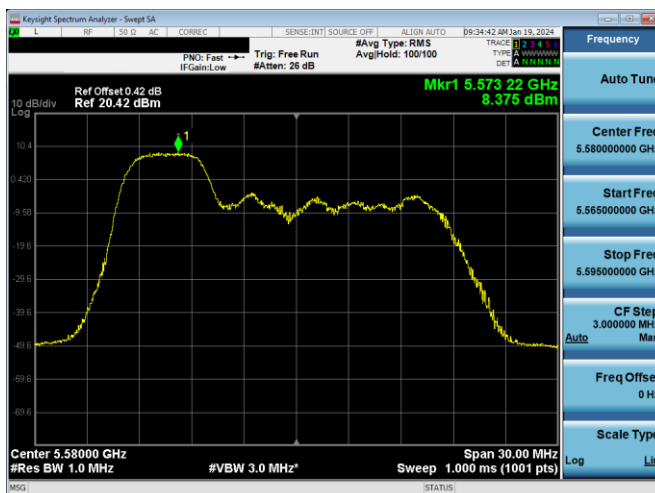
Plot 7-268. PSD Antenna 3a (20MHz BW 11ax Index 37 – RU52 – Ch.116)
