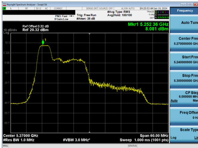
Plot 7-260. PSD Antenna 3a (40MHz BW 11ax Index 37 - RU52 - Ch.54)
