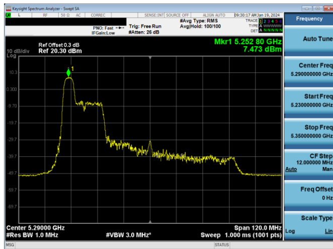
Plot 7-264. PSD Antenna 3a (80MHz BW 11ax Index 37 – RU52 – Ch.58)
