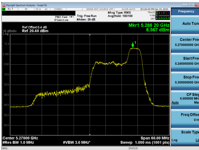
Plot 7-427. PSD CDD Antenna 3a (40MHz BW 11ax Index 44 - RU52 - Ch.54)
