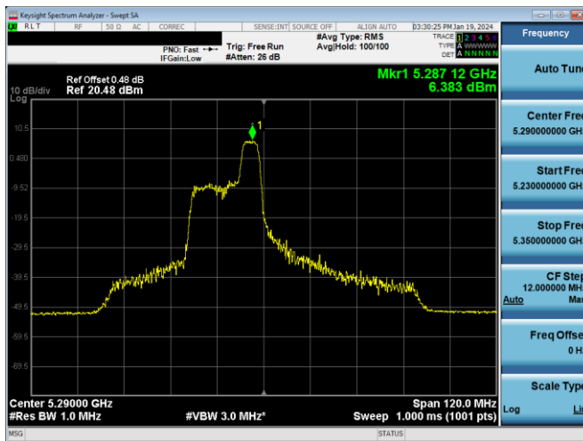
Plot 7-433. PSD CDD Antenna 3a (80MHz BW 11ax Index 44 - RU52 - Ch.58)
