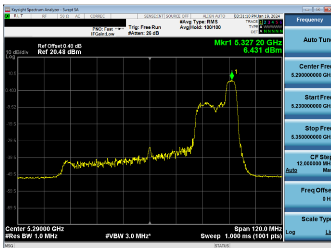
Plot 7-435. PSD CDD Antenna 3a (80MHz BW 11ax Index 52 - RU52 - Ch.58)
