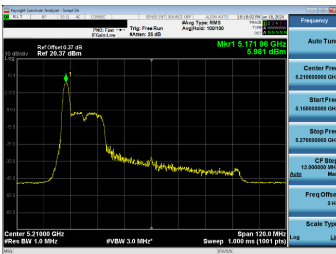
Plot 7-398. PSD CDD Antenna 3c (80MHz BW 11ax Index 0 - RU26 - Ch.42)
