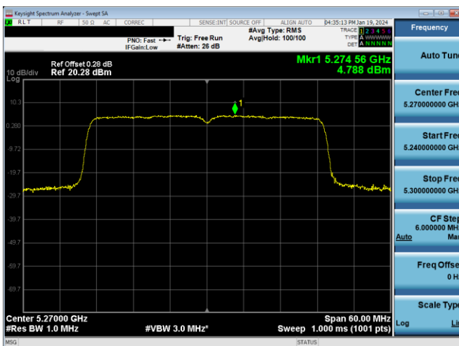
Plot 7-429. PSD CDD Antenna 3a (40MHz BW 11ax - RU484 - Ch.54)
