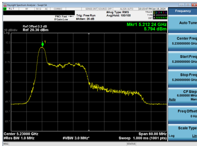
Plot 7-390. PSD CDD Antenna 3c (40MHz BW 11ax Index 0 - RU26 - Ch.46)
