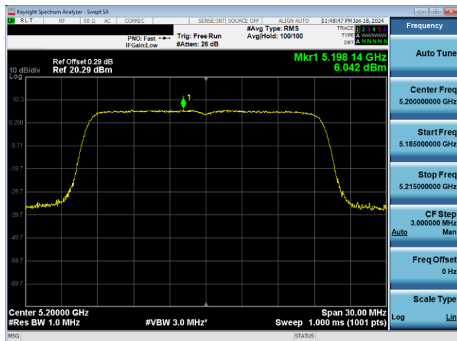
Plot 7-388. PSD CDD Antenna 3c (20MHz BW 11ax - RU242 - Ch.40)
