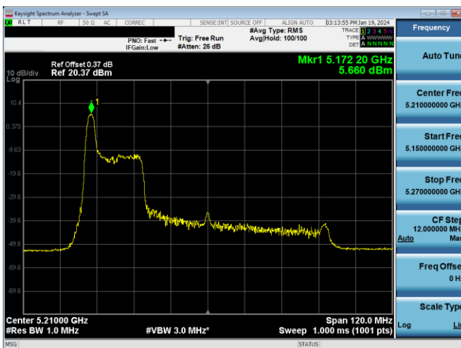
Plot 7-399. PSD CDD Antenna 3a (80MHz BW 11ax Index 0 - RU26 - Ch.42)
