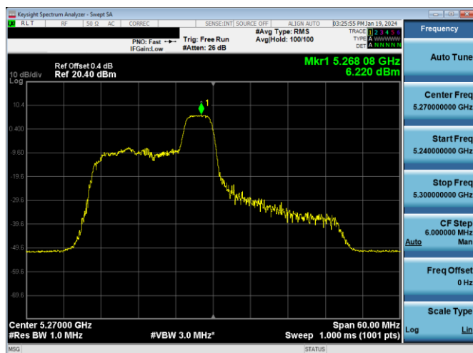
Plot 7-425. PSD CDD Antenna 3a (40MHz BW 11ax Index 40 - RU52 - Ch.54)
