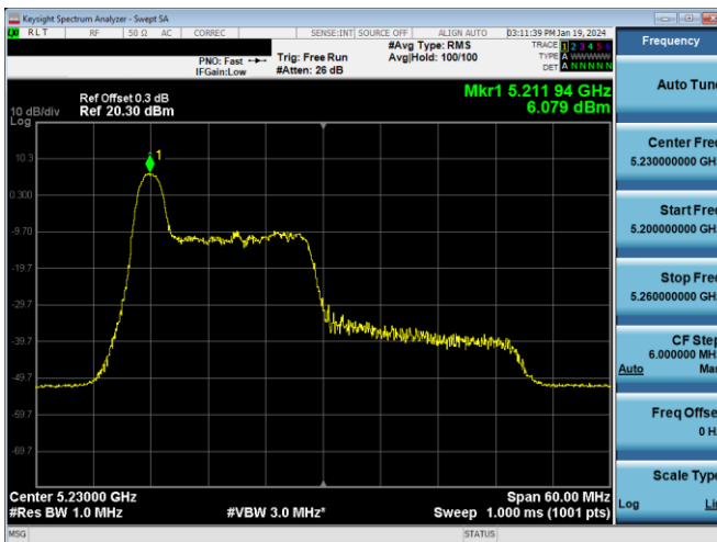
Plot 7-391. PSD CDD Antenna 3a (40MHz BW 11ax Index 0 - RU26 - Ch.46)
