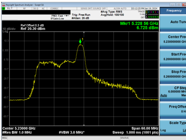
Plot 7-393. PSD CDD Antenna 3a (40MHz BW 11ax Index 8 - RU26 - Ch.46)
