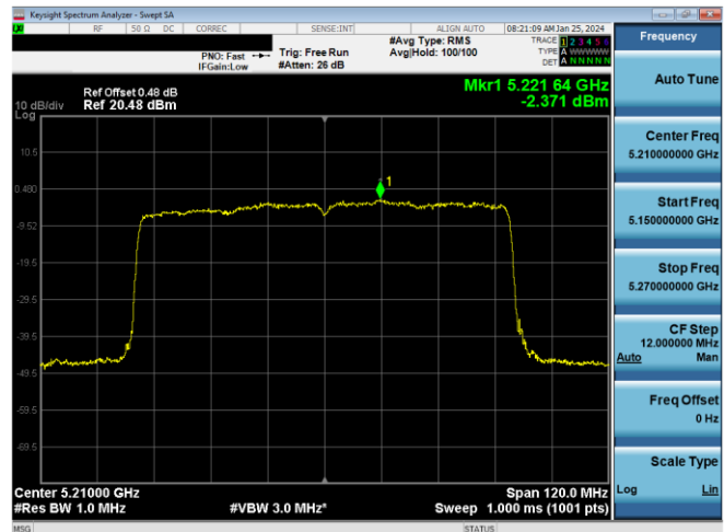
Plot 7-378. ISPD PSD Antenna 1b (80MHz BW 11ax - RU996 - Ch.42)
