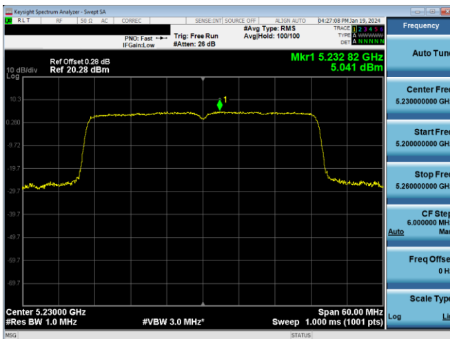
Plot 7-397. PSD CDD Antenna 3a (40MHz BW 11ax - RU484 - Ch.46)
