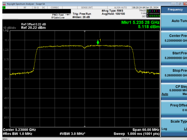
Plot 7-374. ISPD PSD Antenna 1b (40MHz BW 11ax - RU484 - Ch.46)
