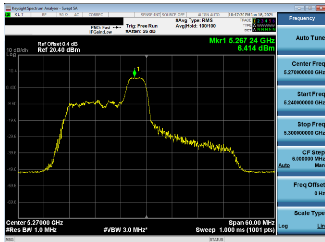
Plot 7-424. PSD CDD Antenna 3c (40MHz BW 11ax Index 40 - RU52 - Ch.54)
