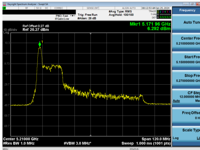
Plot 7-375. ISPD PSD Antenna 1b (80MHz BW 11ax Index 0 - RU26 - Ch.42)
