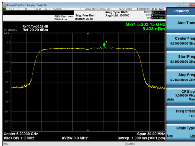
Plot 7-389. PSD CDD Antenna 3a (20MHz BW 11ax - RU242 - Ch.40)
