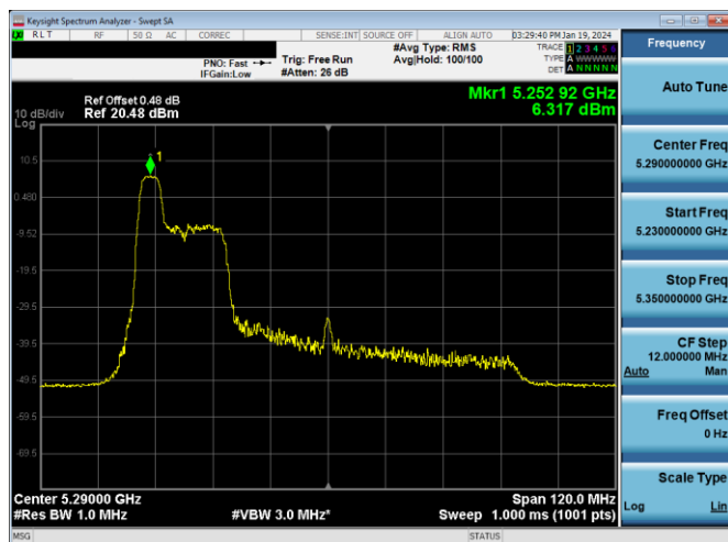
Plot 7-431. PSD CDD Antenna 3a (80MHz BW 11ax Index 37 - RU52 - Ch.58)
