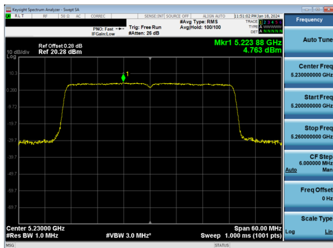
Plot 7-396. PSD CDD Antenna 3c (40MHz BW 11ax - RU484 - Ch.46)
