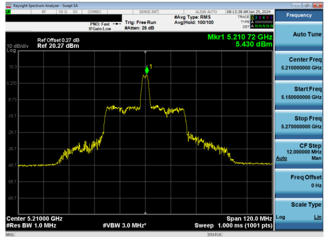
Plot 7-376. ISPD PSD Antenna 1b (80MHz BW 11ax Index 18 - RU26 - Ch.42)
