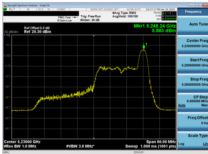
Plot 7-394. PSD CDD Antenna 3c (40MHz BW 11ax Index 17 - RU26 - Ch.46)
