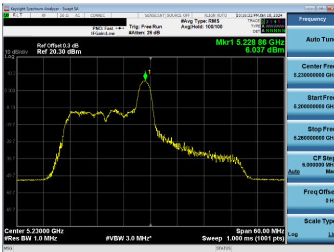
Plot 7-392. PSD CDD Antenna 3c (40MHz BW 11ax Index 8 - RU26 - Ch.46)
