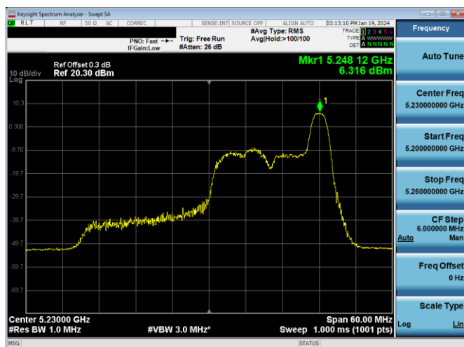
Plot 7-395. PSD CDD Antenna 3a (40MHz BW 11ax Index 17 - RU26 - Ch.46)
