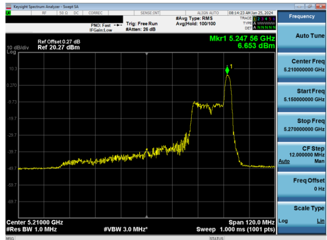
Plot 7-377. ISPD PSD Antenna 1b (80MHz BW 11ax Index 36 - RU26 - Ch.42)
