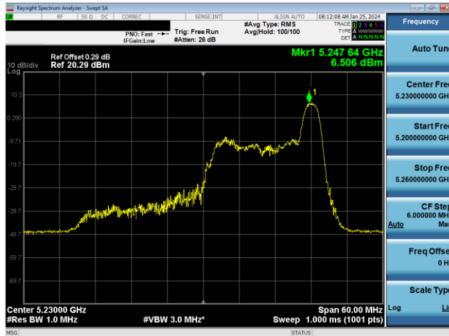
Plot 7-373. ISPD PSD Antenna 1b (40MHz BW 11ax Index 17 - RU26 - Ch.46)
