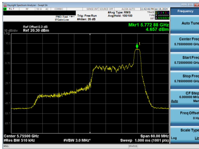
Plot 7-482. PSD CDD Antenna 3c (40MHz BW 11ax Index 17 - RU26 - Ch.151)
