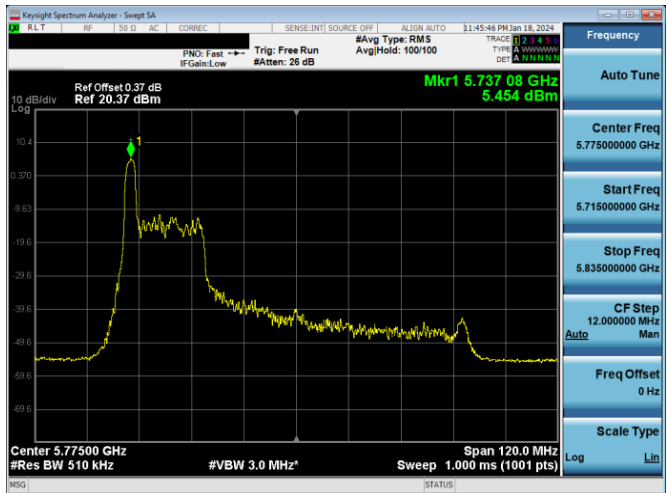
Plot 7-486. PSD CDD Antenna 3c (80MHz BW 11ax Index 0 - RU26 - Ch.155)
