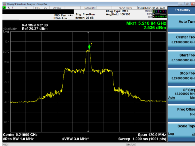
Plot 7-513. ISED PSD SDM Antenna 3a (80MHz BW 11ax Index 18 - RU26 - Ch.42)
