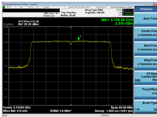
Plot 7-484. PSD CDD Antenna 3c (40MHz BW 11ax - RU484 - Ch.151)
