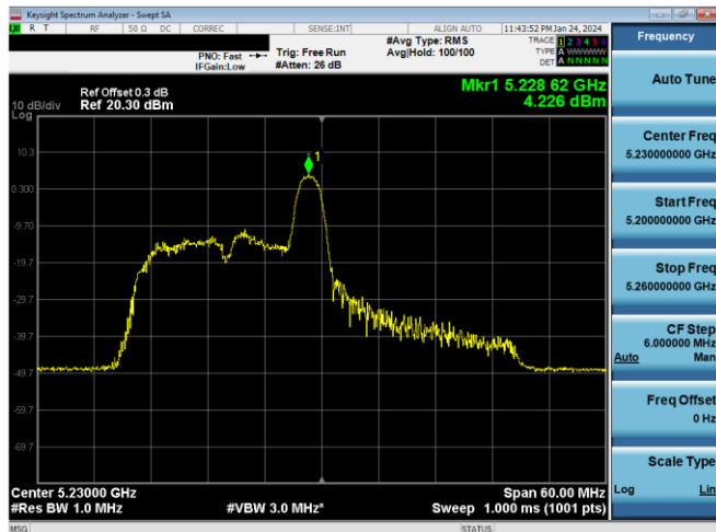
Plot 7-504. ISED PSD SDM Antenna 3c (40MHz BW 11ax Index 8 - RU26 - Ch.46)
