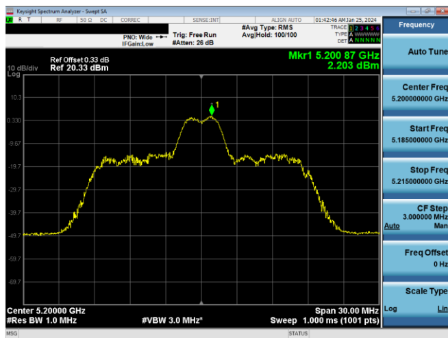
Plot 7497. ISED PSD SDM Antenna 3a (20MHz BW 11ax Index 4 - RU26 - Ch.40)
