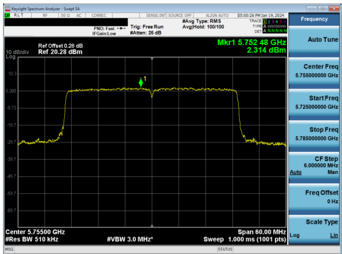
Plot 7-485. PSD CDD Antenna 3a (40MHz BW 11ax - RU484 - Ch.151)
