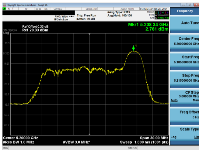
Plot 7499. ISED PSD SDM Antenna 3a (20MHz BW 11ax Index 8 - RU26 - Ch.40)
