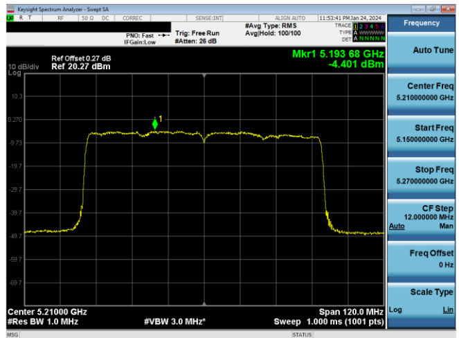
Plot 7-516. ISED PSD CDD Antenna 3c (80MHz BW 11ax - RU996 - Ch.42)
