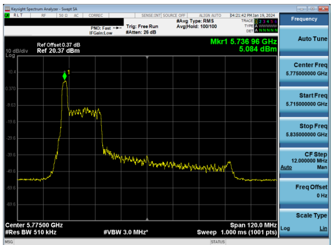
Plot 7-487. PSD CDD Antenna 3a (80MHz BW 11ax Index 0 - RU26 - Ch.155)
