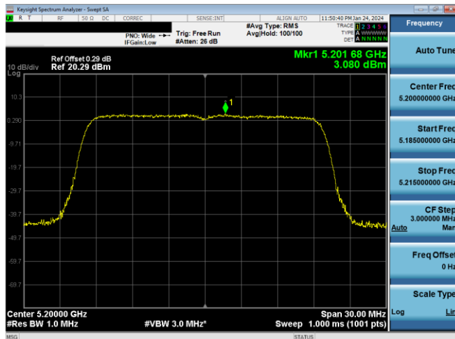
Plot 7-500. ISED PSD SDM Antenna 3c (20MHz BW 11ax- RU242 - Ch.40)
