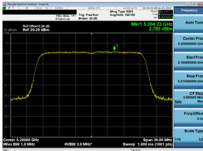
Plot 7-501. ISED PSD SDM Antenna 3a (20MHz BW 11ax- RU242 - Ch.40)
