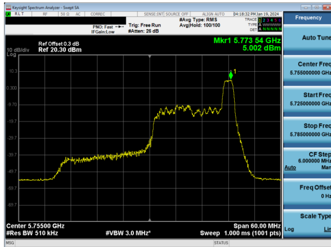
Plot 7-483. PSD CDD Antenna 3a (40MHz BW 11ax Index 17 - RU26 - Ch.151)
