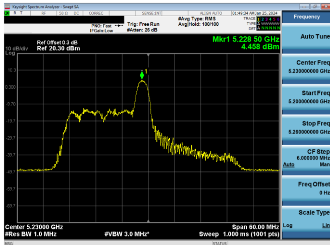
Plot 7-505. ISED PSD SDM Antenna 3a (40MHz BW 11ax Index 8 - RU26 - Ch.46)
