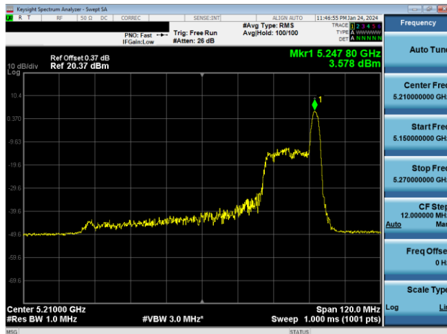
Plot 7-514. ISED PSD SDM Antenna 3c (80MHz BW 11ax Index 36 - RU26 - Ch.42)
