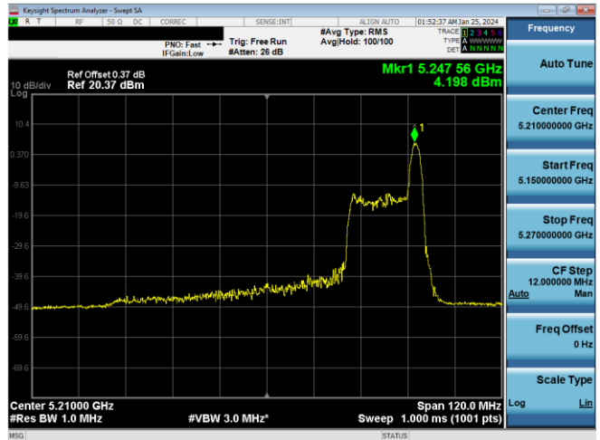
Plot 7-515. ISED PSD SDM Antenna 3a (80MHz BW 11ax Index 36 - RU26 - Ch.42)
