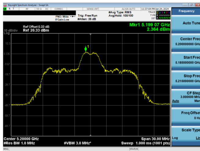
Plot 7496. ISED PSD SDM Antenna 3c (20MHz BW 11ax Index 4 - RU26 - Ch.40)
