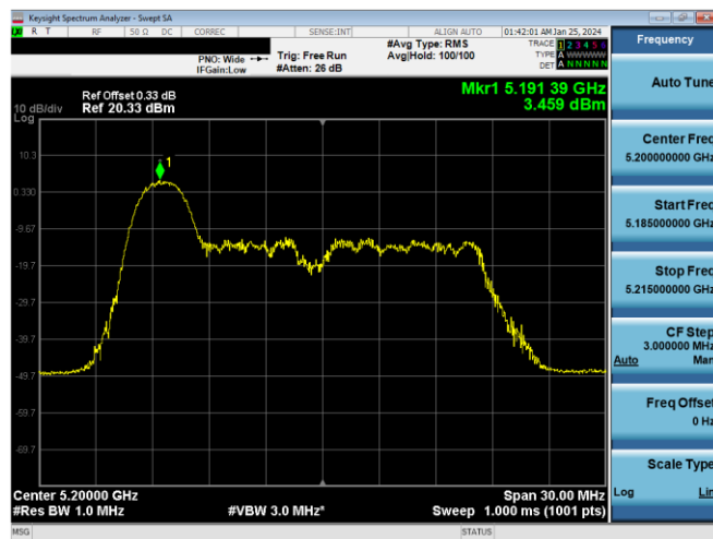
Plot 7495. ISED PSD SDM Antenna 3a (20MHz BW 11ax Index 0 - RU26 - Ch.40)
