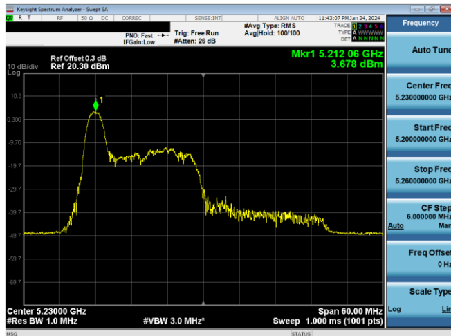
Plot 7-502. ISED PSD SDM Antenna 3c (40MHz BW 11ax Index 0 - RU26 - Ch.46)
