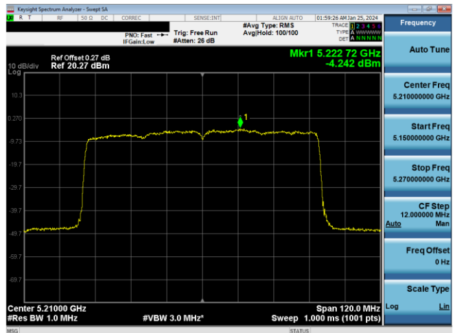
Plot 7-517. ISED PSD CDD Antenna 3a (80MHz BW 11ax - RU996 - Ch.42)
