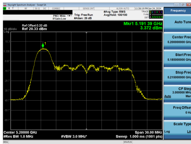
Plot 7494. ISED PSD SDM Antenna 3c (20MHz BW 11ax Index 0 - RU26 - Ch.40)
