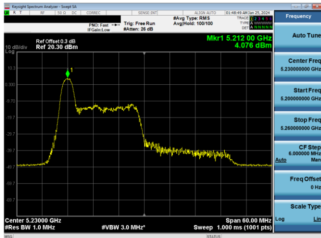
Plot 7-503. ISED PSD SDM Antenna 3a (40MHz BW 11ax Index 0 - RU26 - Ch.46)
