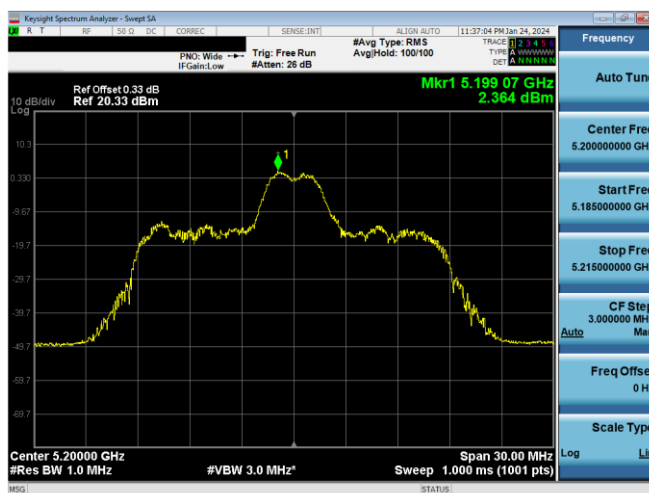
Plot 7-638. ISED PSD SDM Antenna 3c (20MHz BW 11ax Index 4 – RU26 – Ch.40)
