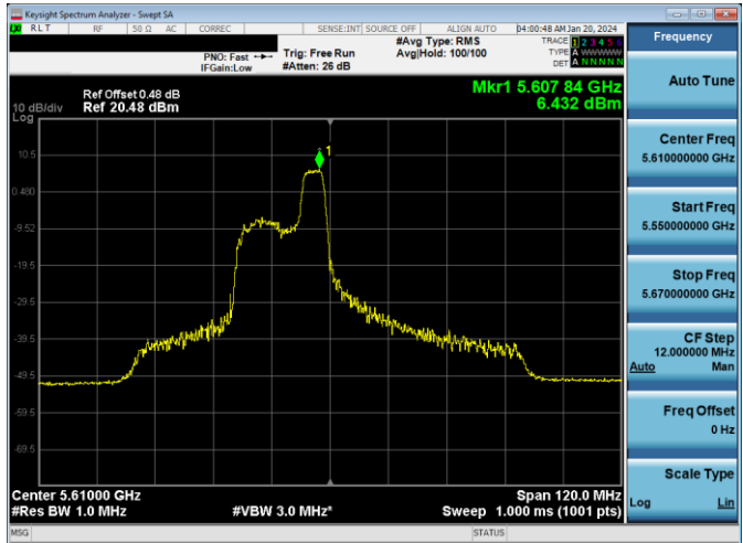
Plot 7-599. PSD CDD Antenna 1b (80MHz BW 11ax Index 44 - RU52 - Ch.122)
