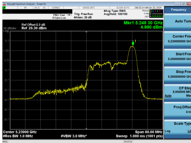
Plot 7-649. ISED PSD SDM Antenna 1b (40MHz BW 11ax Index 17 - RU26 - Ch.46)
