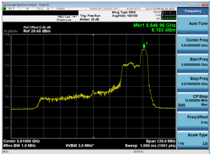
Plot 7-600. PSD CDD Antenna 3c (80MHz BW 11ax Index 52 - RU52 - Ch.122)
