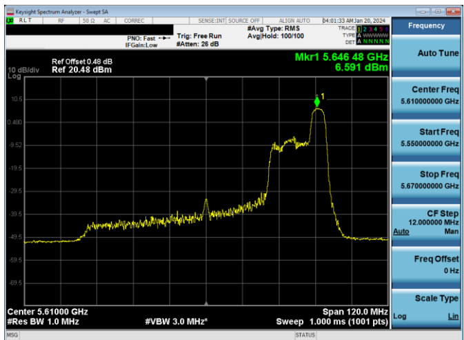
Plot 7-601. PSD CDD Antenna 1b (80MHz BW 11ax Index 52 - RU52 - Ch.122)
