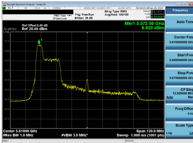
Plot 7-597. PSD CDD Antenna 1b (80MHz BW 11ax Index 37 - RU52 - Ch.122)
