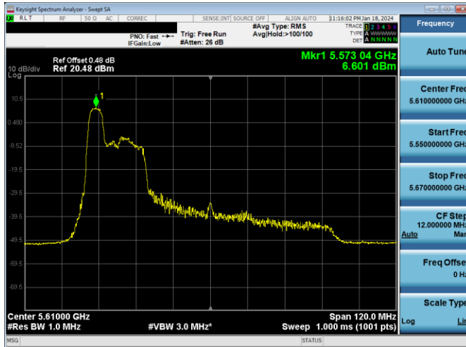
Plot 7-596. PSD CDD Antenna 3c (80MHz BW 11ax Index 37 - RU52 - Ch.122)
