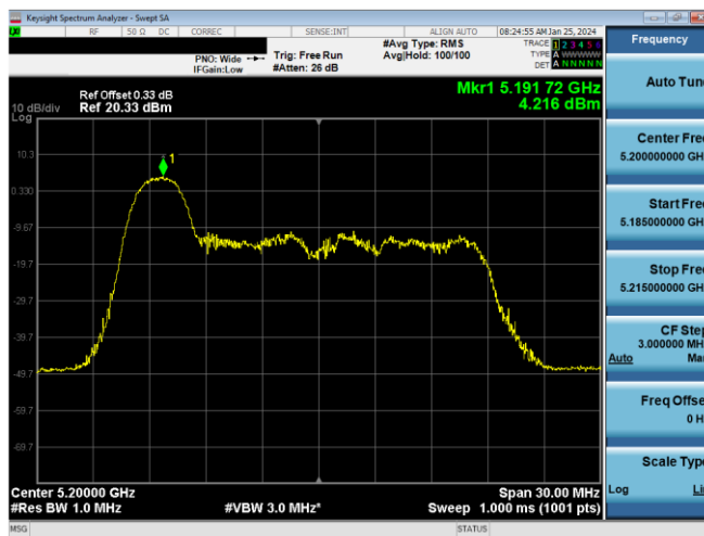
Plot 7-637. ISED PSD SDM Antenna 1b (20MHz BW 11ax Index 0 – RU26 – Ch.40)
