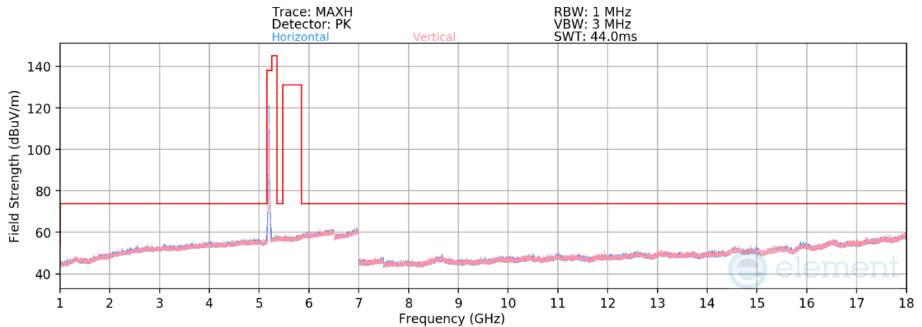
Plot 7-667. RSE above 1GHz Antenna 3c (11ax – Ch.40 – RU26)
