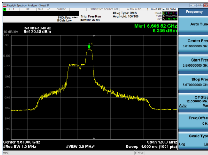
Plot 7-598. PSD CDD Antenna 3c (80MHz BW 11ax Index 44 - RU52 - Ch.122)
