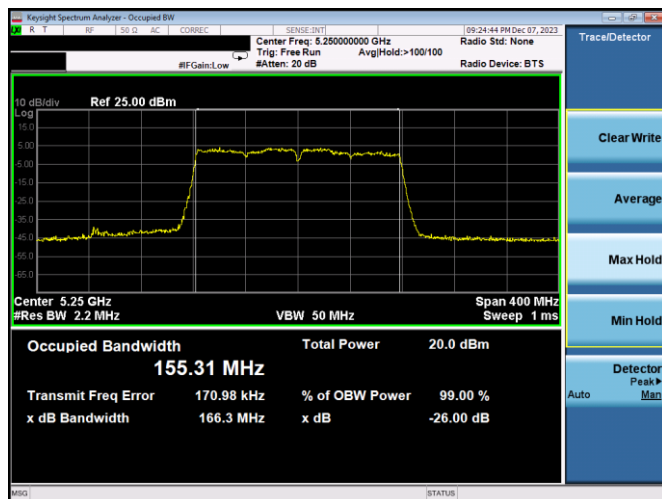
Plot 7-7. 26dB BW & 99% OBW Antenna 3c (160MHz BW 802.11ac – Ch. 50, MCS2)
