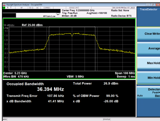
Plot 7-3. 26dB BW & 99% OBW Antenna 3c (40MHz BW 802.11n – Ch. 46, MCS2)
