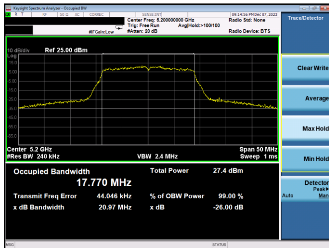
Plot 7-1. 26dB BW & 99% OBW Antenna 3c (20MHz BW 802.11n – Ch. 40, MCS2)
