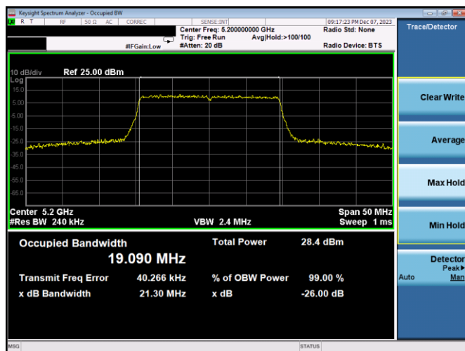
Plot 7-2. 26dB BW & 99% OBW Antenna 3c (20MHz BW 802.11ax(SU) – Ch. 40, MCS2)
