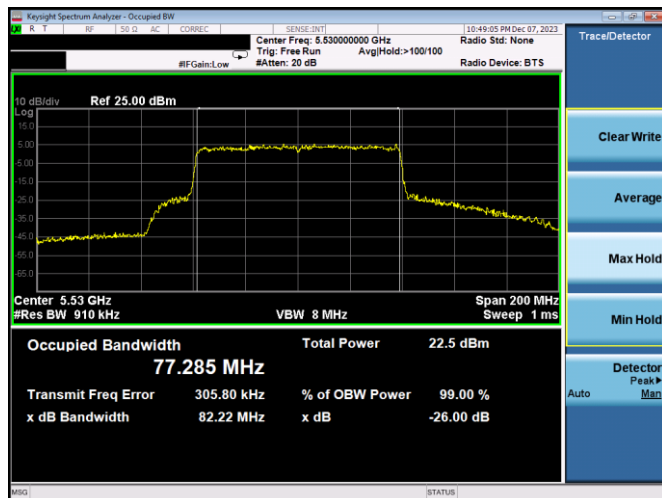
Plot 7-42. 26dB BW & 99% OBW Antenna 3c (80MHz BW 802.11ax(SU) – Ch. 106, MCS4)
