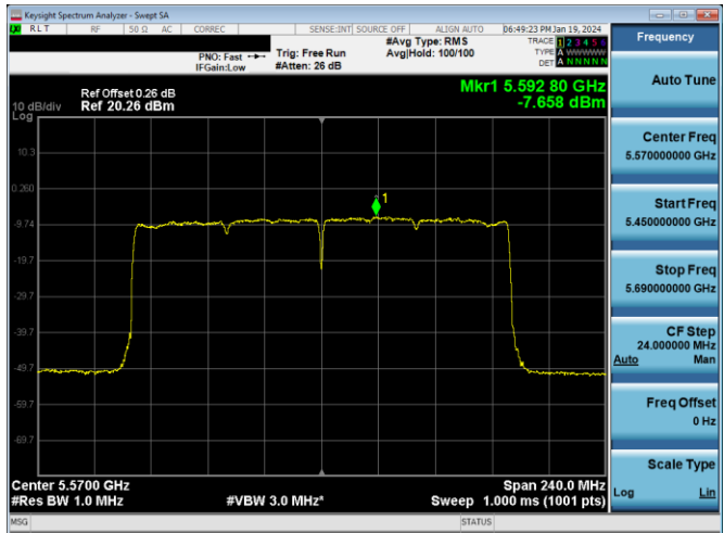
Plot 7-664. PSD CDD PRIMARY Antenna 3a (160MHz BW 802.11ac(SU) - Ch. 114, MCS4)
