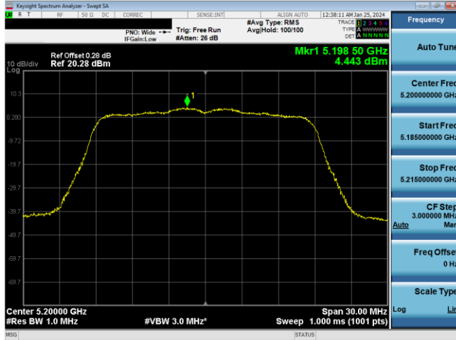
Plot 7-757. ISED PSD SDM Primary Antenna 3c (20MHz BW 11n - Ch.40, MCS12)
