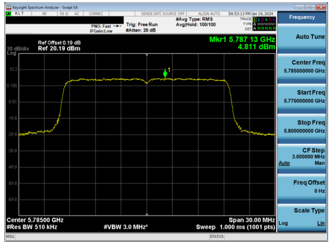
Plot 7-724. PSD CDD PRIMARY Antenna 3a (20MHz BW 802.11ax(SU) – Ch. 157, MCS4)
