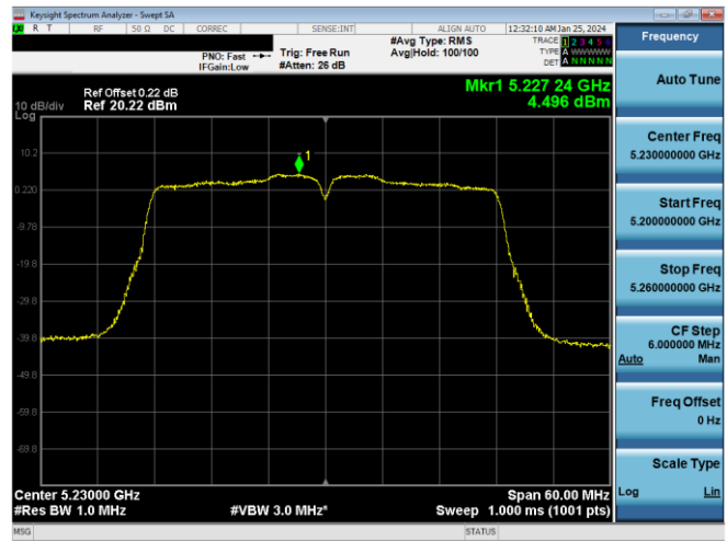
Plot 7-749. ISED PSD SDM Primary Antenna 3c (40MHz BW 11n – Ch.46, MCS10)
