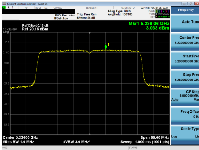
Plot 7-764. ISED SDM Primary PSD Antenna 3a (40MHz BW 11ax(SU) – Ch.46, MCS4)
