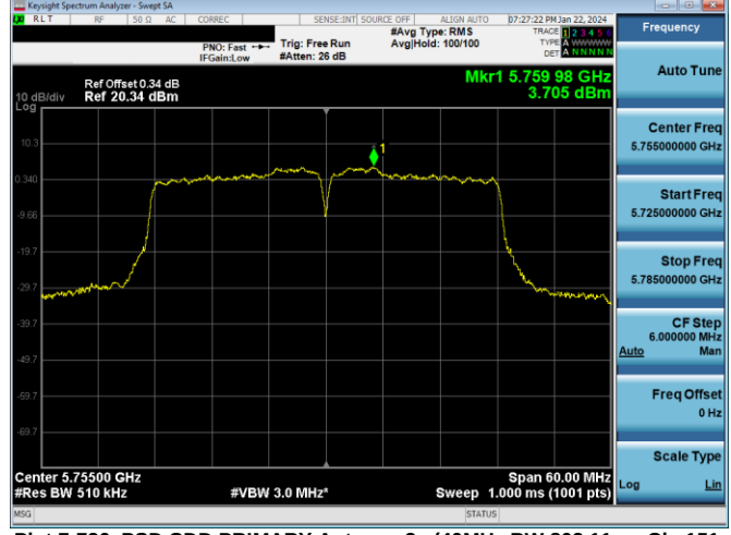
Plot 7-726. PSD CDD PRIMARY Antenna 3a (40MHz BW 802.11n – Ch. 151, MCS12)
