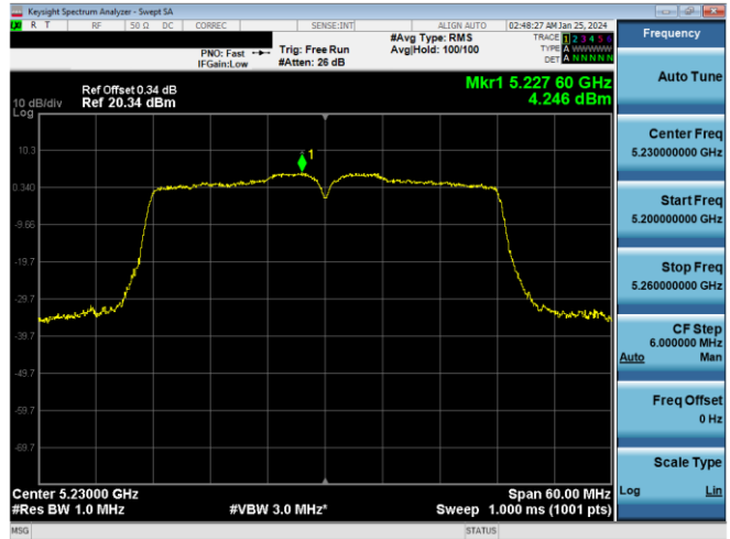
Plot 7-762. ISED PSD SDM Primary Antenna 3a (40MHz BW 11n - Ch.46, MCS12)
