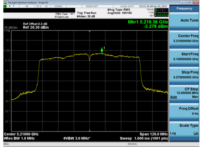
Plot 7-766. ISED PSD CDD Primary Antenna 3a (80MHz BW 11ac – Ch.42, MCS4)
