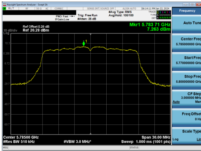
Plot 7-721. PSD CDD PRIMARY Antenna 3c (20MHz BW 802.11n – Ch. 157, MCS12)
