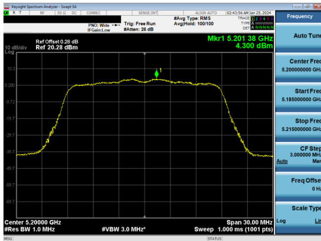
Plot 7-758. ISED PSD SDM Primary Antenna 3a (20MHz BW 11n - Ch.40, MCS12)
