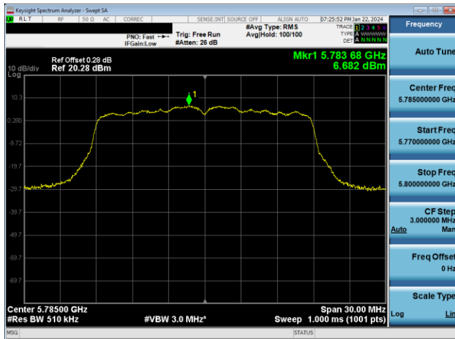
Plot 7-722. PSD CDD PRIMARY Antenna 3a (20MHz BW 802.11n – Ch. 157, MCS12)
