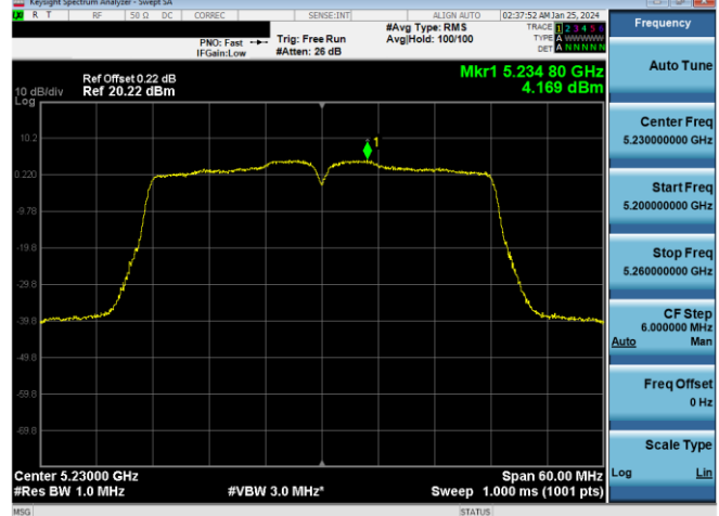
Plot 7-750. ISED PSD SDM Primary Antenna 3a (40MHz BW 11n – Ch.46, MCS10)
