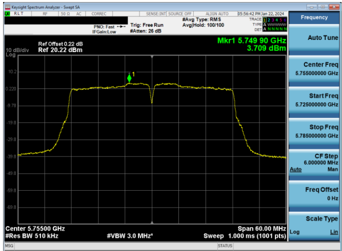
Plot 7-713. PSD CDD PRIMARY Antenna 3c (40MHz BW 802.11n – Ch. 151, MCS10)
