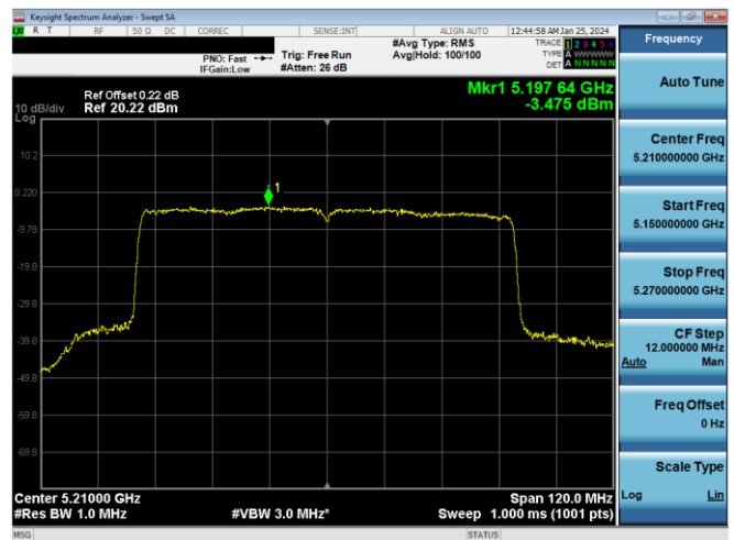
Plot 7-767. ISED PSD CDD Antenna 3c Primary (80MHz BW 11ax (SU) – Ch.42, MCS4)
