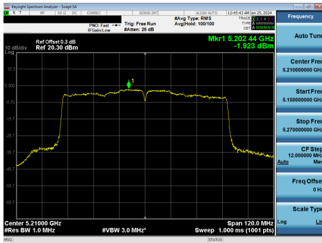
Plot 7-765. ISED PSD CDD Primary Antenna 3c (80MHz BW 11ac – Ch.42, MCS4)
