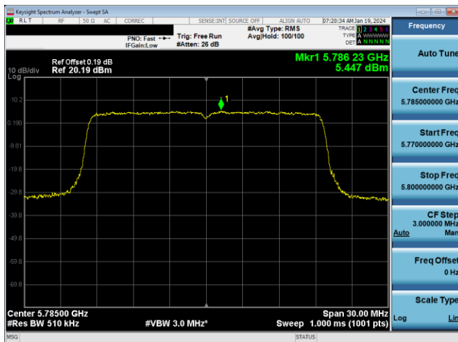
Plot 7-723. PSD CDD PRIMARY Antenna 3c (20MHz BW 802.11ax(SU) – Ch. 157, MCS4)
