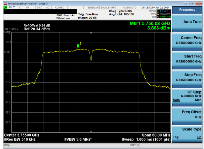
Plot 7-725. PSD CDD PRIMARY Antenna 3c (40MHz BW 802.11n – Ch. 151, MCS12)
