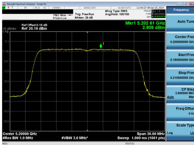
Plot 7-759. ISED PSD SDM Primary Antenna 3c (20MHz BW 11ax(SU) - Ch.40, MCS4)
