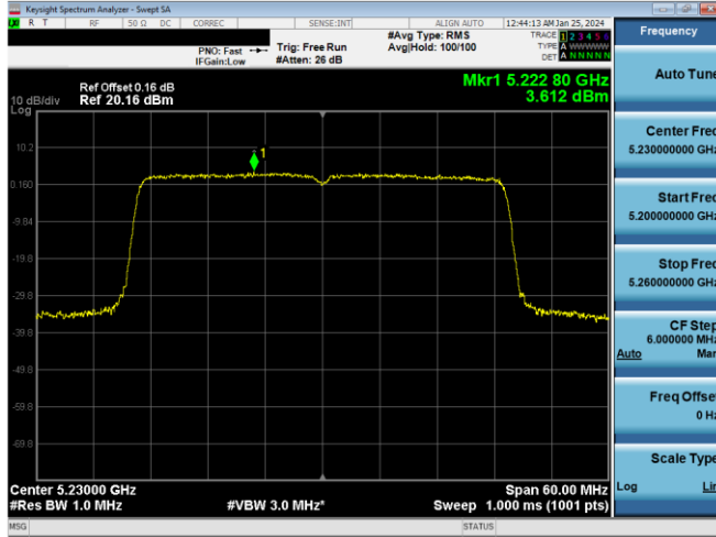
Plot 7-763. ISED PSD SDM Primary Antenna 3c (40MHz BW 11ax(SU) – Ch.46, MCS4)
