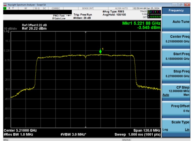
Plot 7-768. ISED PSD CDD Primary Antenna 3a (80MHz BW 11ax (SU) – Ch.42, MCS4)
