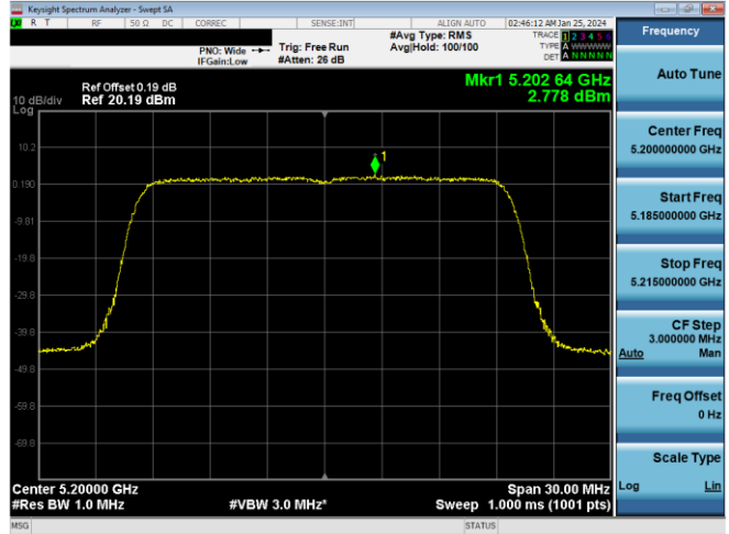
Plot 7-760. ISED PSD SDM Primary Antenna 3a (20MHz BW 11ax(SU) - Ch.40, MCS4)
