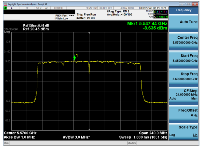
Plot 7-707. PSD CDD PRIMARY Antenna 3c (160MHz BW 802.11ax(SU) – Ch. 114, MCS11)
