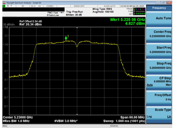
Plot 7-761. ISED PSD SDM Primary Antenna 3c (40MHz BW 11n - Ch.46, MCS12)
