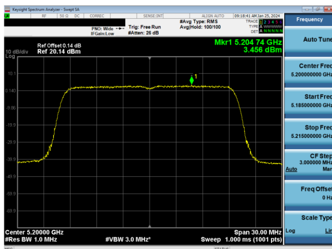
Plot 7-884. ISCED PSD CDD DIVERSITY Antenna 1b (20MHz BW 11ax(SU) - Ch.40, MCS2)
