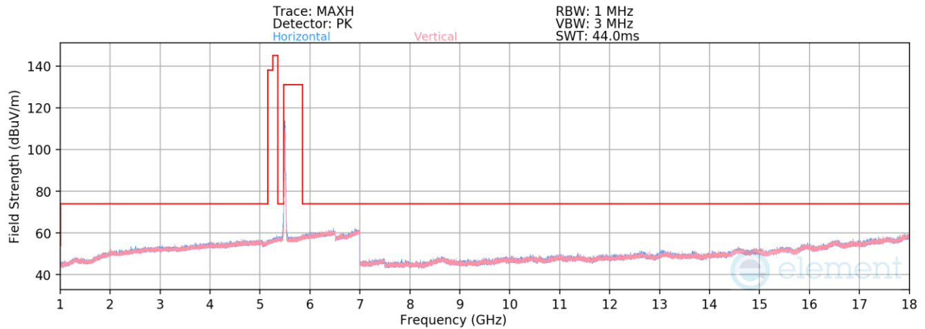
Plot 7-913. Radiated Spurious Emissions above 1GHz Antenna 3c (802.11n – Ch. 100)
