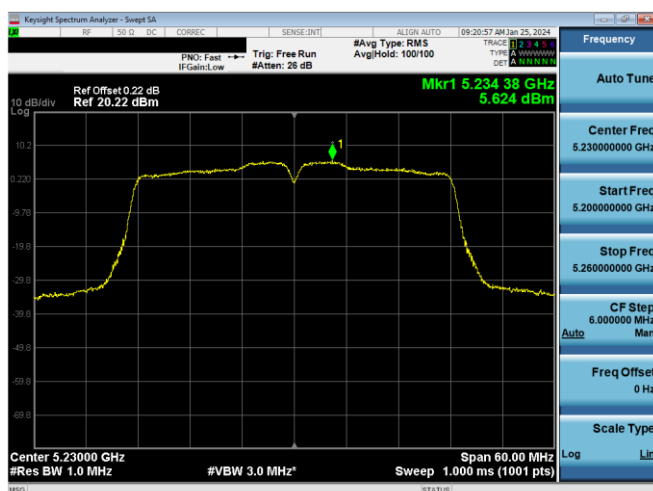
Plot 7-885. ISCED PSD CDD DIVERSITY Antenna 1b (40MHz BW 11n - Ch.46, MCS10)
