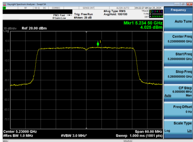
Plot 7-886. ISCED CDD DIVERSITY PSD Antenna 1b (40MHz BW 11ax(SU) - Ch.46, MCS2)
