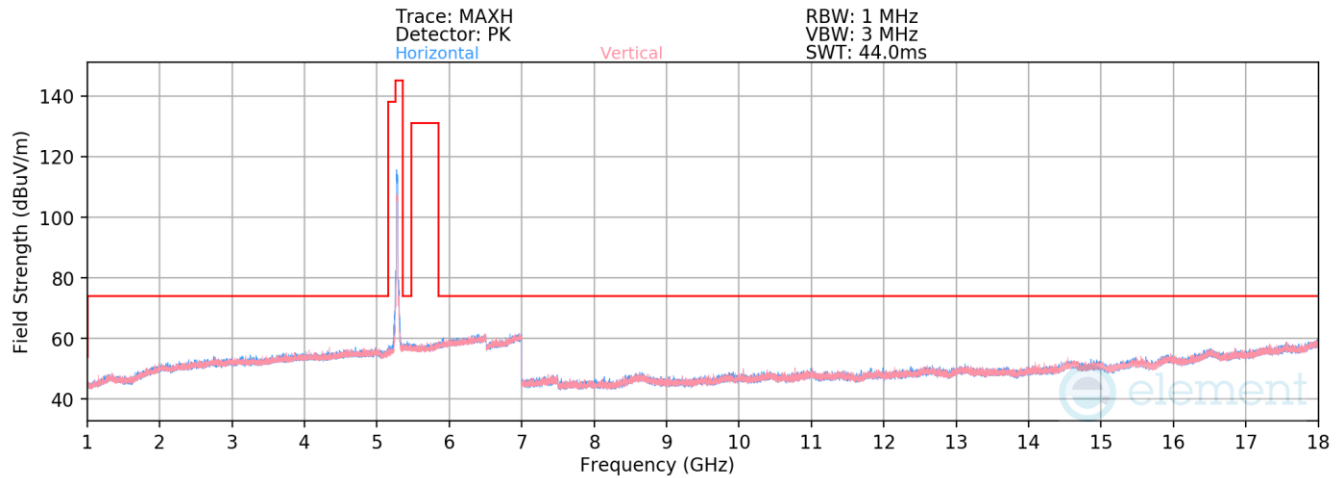
Plot 7-923. Radiated Spurious Emissions above 1GHz Antenna 3c (802.11ax(SU) – Ch. 56)
