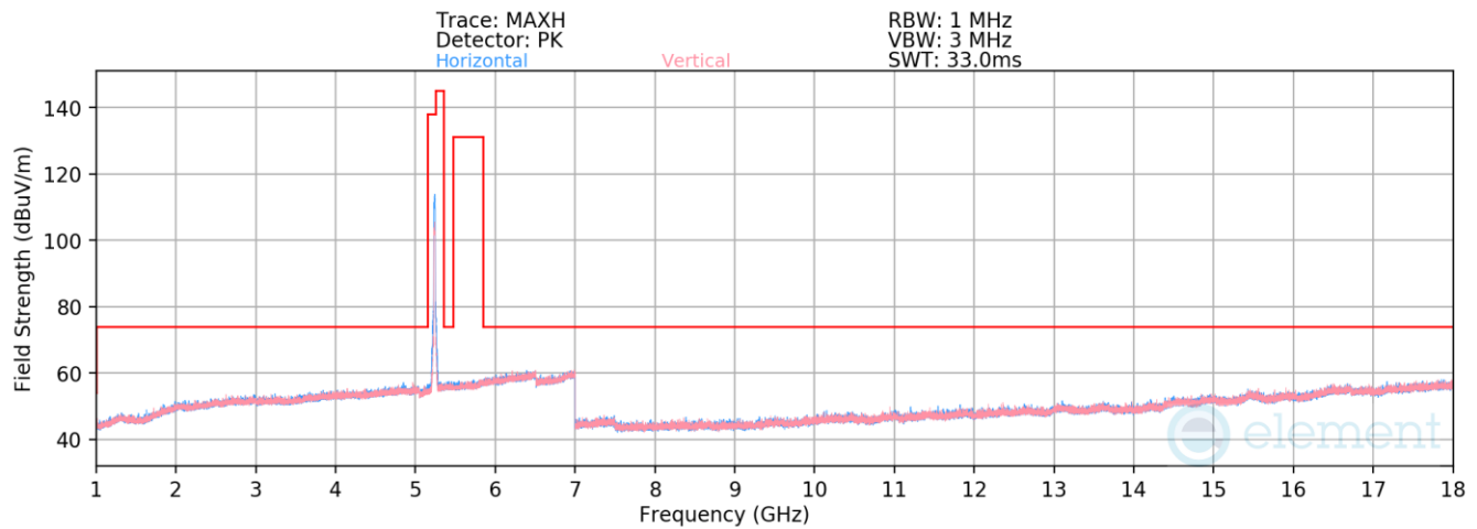
Plot 7-909. Radiated Spurious Emissions above 1GHz Antenna 3c (802.11n – Ch. 48)
