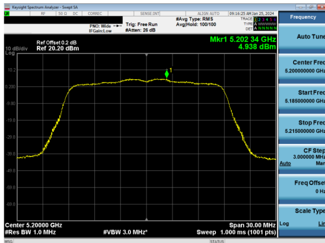
Plot 7-883. ISCED PSD CDD DIVERSITY Antenna 1b (20MHz BW 11n - Ch.40, MCS10)
