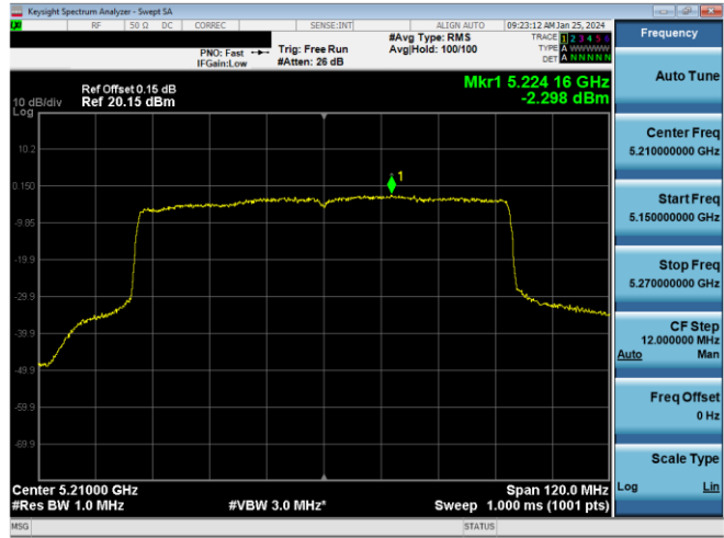
Plot 7-888. ISCED PSD CDD DIVERSITY Antenna 1b (80MHz BW 11ax (SU) - Ch.42, MCS2)
