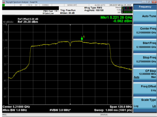
Plot 7-887. ISCED PSD CDD DIVERSITY Antenna 1b (80MHz BW 11ac - Ch.42, MCS2)
