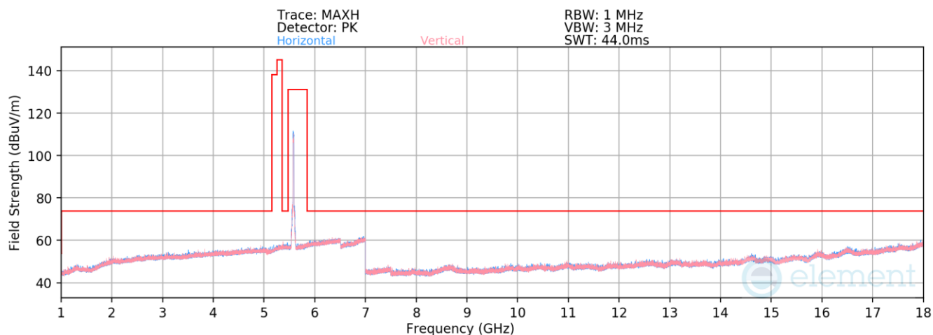
Plot 7-974. Radiated Spurious Emissions above 1GHz Antenna 1b (802.11ax(SU) – Ch. 116)
