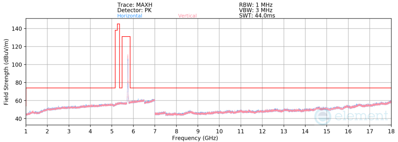
Plot 7-940. Radiated Spurious Emissions above 1GHz Antenna 3a (802.11n – Ch. 149)
