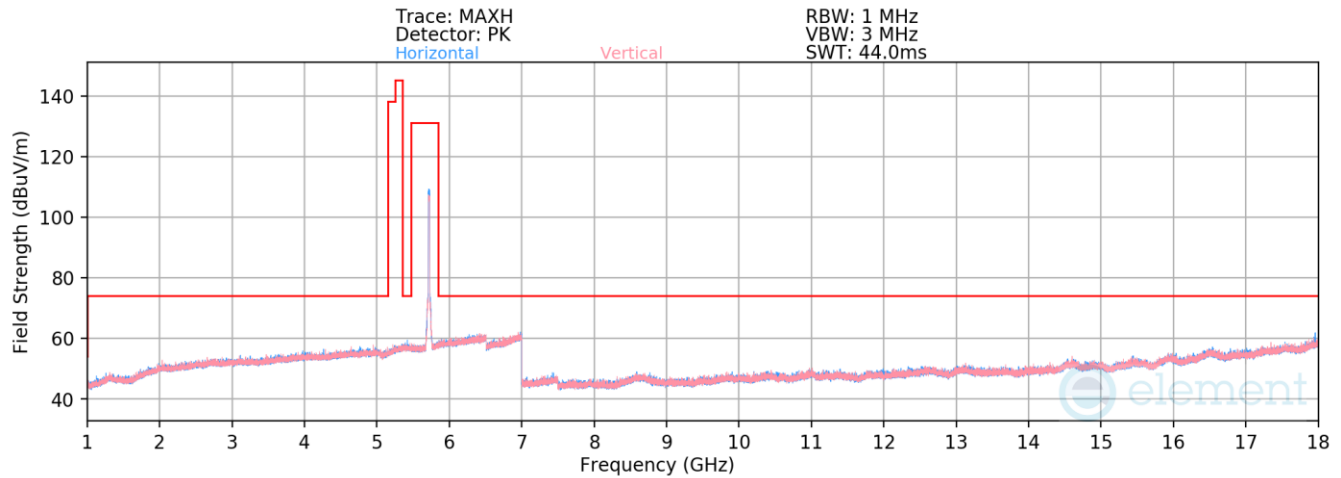
Plot 7-975. Radiated Spurious Emissions above 1GHz Antenna 1b (802.11ax(SU) – Ch. 144)
