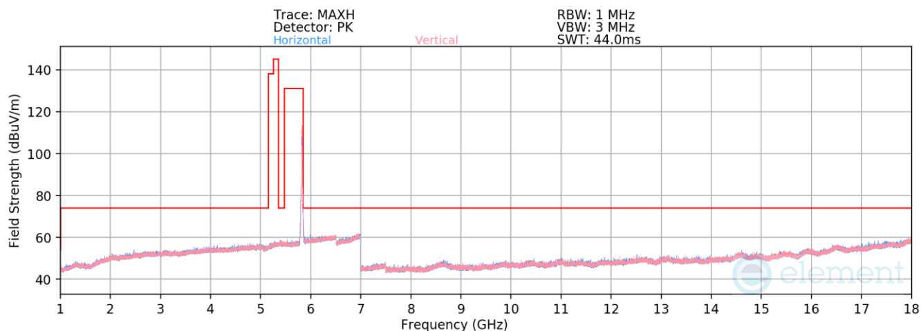
Plot 7-942. Radiated Spurious Emissions above 1GHz Antenna 3a (802.11n – Ch. 165)
