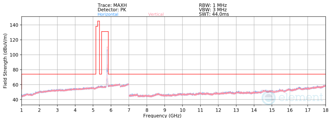
Plot 7-953. Radiated Spurious Emissions above 1GHz Antenna 3a (802.11ax(SU) – Ch. 157)
