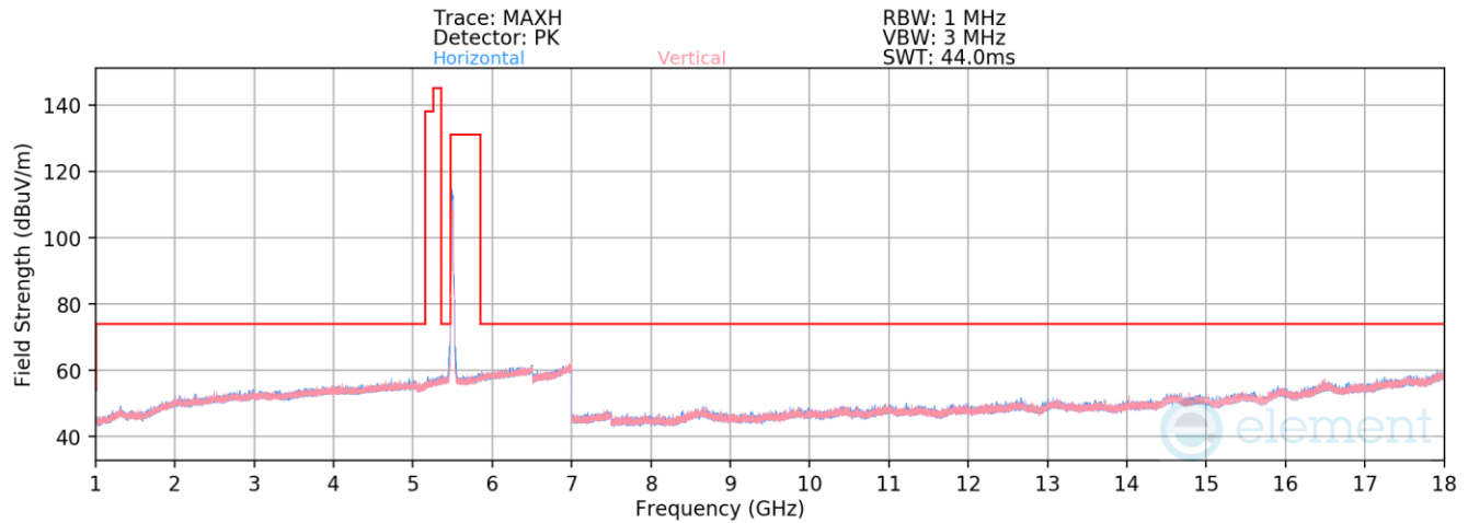
Plot 7-925. Radiated Spurious Emissions above 1GHz Antenna 3c (802.11ax(SU) – Ch. 100)
