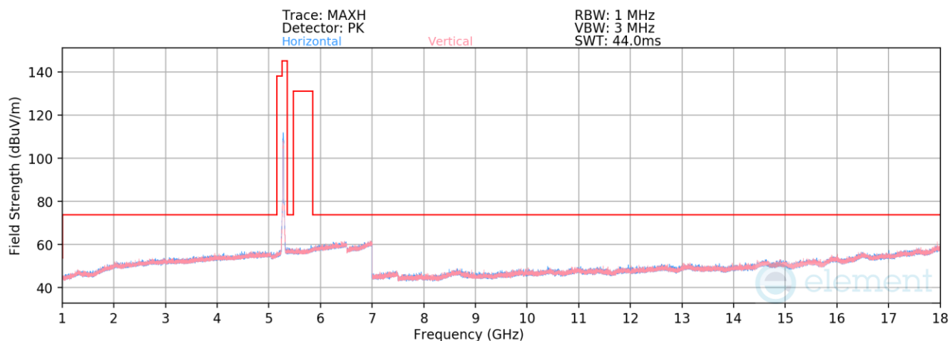
Plot 7-959. Radiated Spurious Emissions above 1GHz Antenna 1b (802.11n – Ch. 56)
