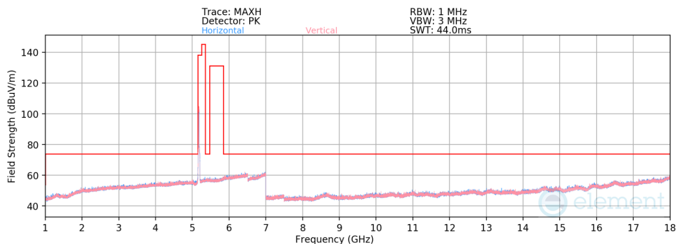
Plot 7-943. Radiated Spurious Emissions above 1GHz Antenna 3a (802.11ax(SU) – Ch. 36)
