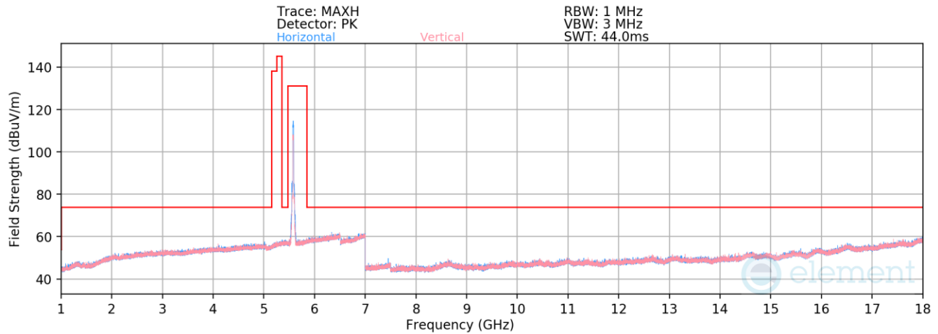
Plot 7-926. Radiated Spurious Emissions above 1GHz Antenna 3c (802.11ax(SU) – Ch. 116)
