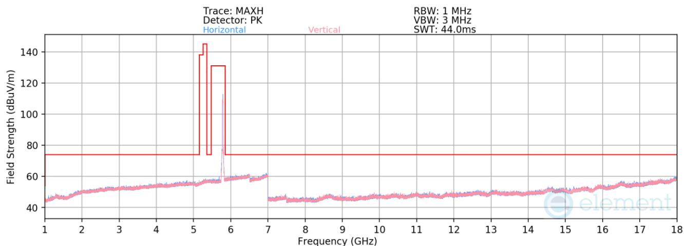
Plot 7-977. Radiated Spurious Emissions above 1GHz Antenna 1b (802.11ax(SU) – Ch. 157)
