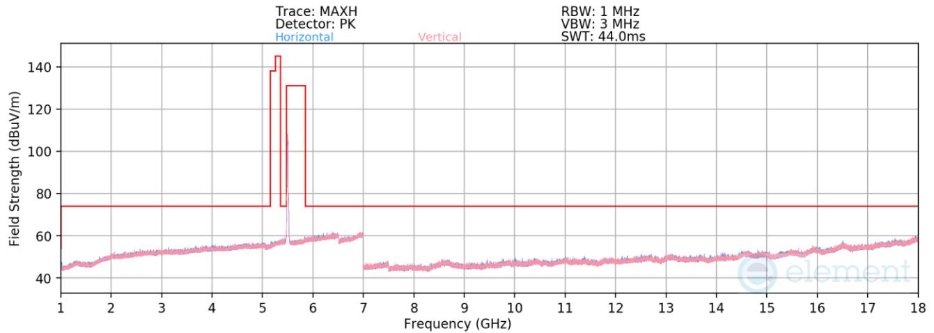
Plot 7-937. Radiated Spurious Emissions above 1GHz Antenna 3a (802.11n – Ch. 100)
