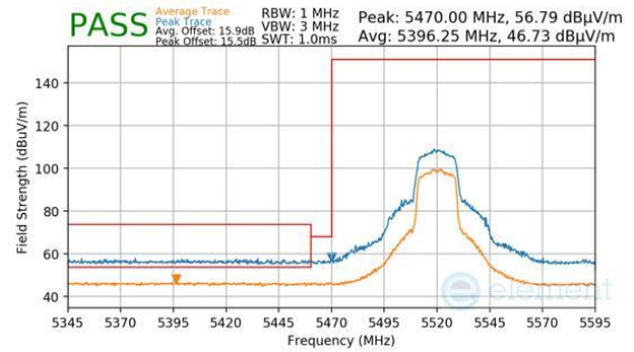
Plot 7-1472. Antenna 1b (Pk & Avg, Ch.104, 802.11n, MCS4)
