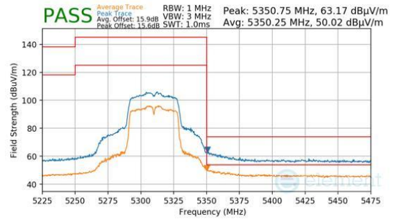
Plot 7-1538. Antenna 1b (Pk & Avg, Ch.62, 802.11n, MCS4)
