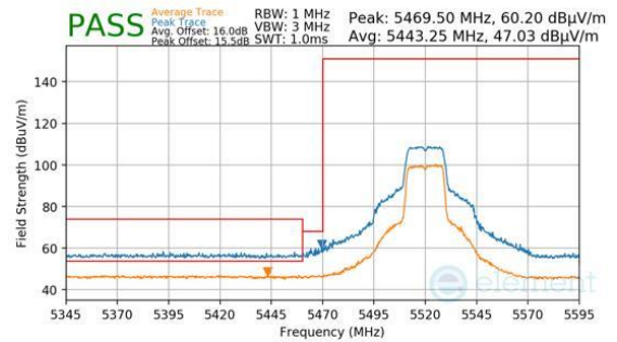
Plot 7-1473. Antenna 1b (Pk & Avg, Ch.104, 802.11n, MCS7)
