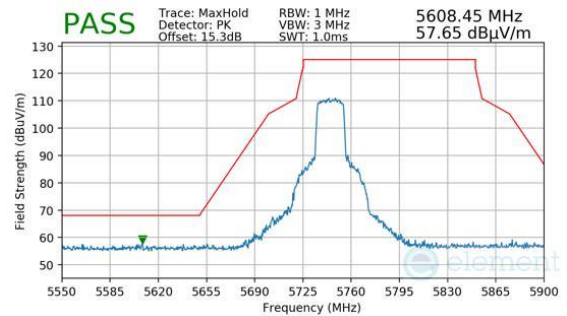
Plot 7-1521. Antenna 1b (Pk, Ch.149, 802.11ax(SU), MCS11)
