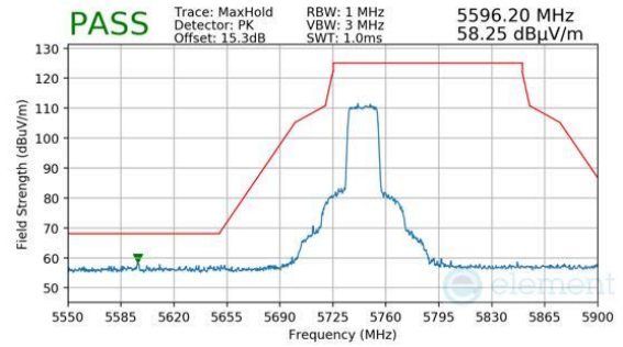
Plot 7-1519. Antenna 1b (Pk, Ch.149, 802.11ax(SU), MCS2)
