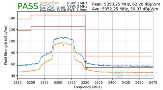
Plot 7-1537. Antenna 1b (Pk & Avg, Ch.62, 802.11n, MCS2)
