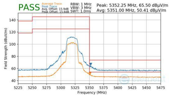
Plot 7-1466. Antenna 1b (Pk & Avg, Ch.64, 802.11n, MCS4)
