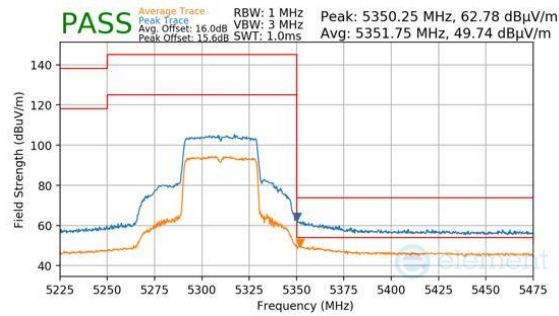
Plot 7-1571. Antenna 1b (Pk & Avg, Ch.62, 802.11ax(SU), MCS4)
