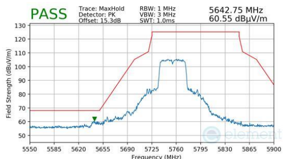
Plot 7-1557. Antenna 1b (Pk, Ch.151, 802.11n, MCS7)
