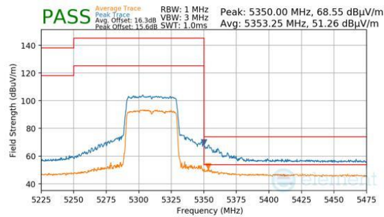
Plot 7-1572. Antenna 1b (Pk & Avg, Ch.62, 802.11ax(SU), MCS11)
