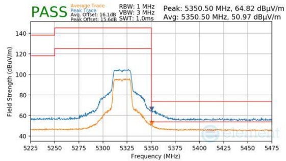
Plot 7-1467. Antenna 1b (Pk & Avg, Ch.64, 802.11n, MCS7)
