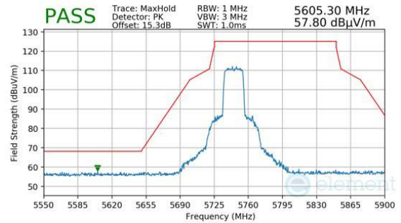
Plot 7-1520. Antenna 1b (Pk, Ch.149, 802.11ax(SU), MCS4)
