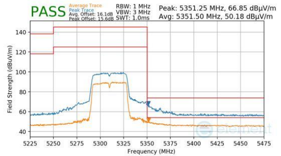
Plot 7-1539. Antenna 1b (Pk & Avg, Ch.62, 802.11n, MCS7)
