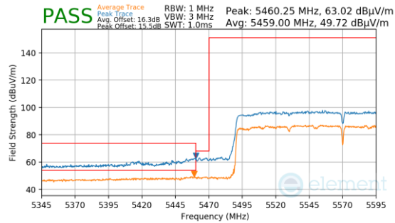
Plot 7-1655. Antenna 1b (Pk & Avg, Ch.114, 802.11ax(SU), MCS11)
