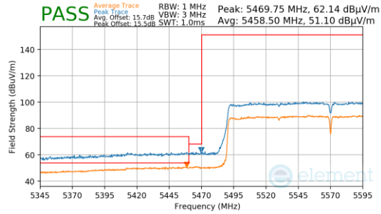
Plot 7-1653. Antenna 1b (Pk & Avg, Ch.114, 802.11ax(SU), MCS2)
