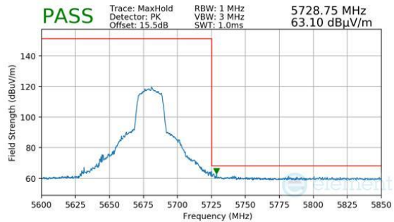
Plot 7-1674. CDD/SDM Primary (Pk, Ch.136, 802.11n, MCS10)
