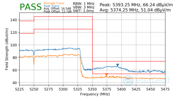
Plot 7-1652. Antenna 1b (Pk & Avg, Ch.50, 802.11ax(SU), MCS11)
