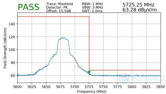
Plot 7-1675. CDD/SDM Primary (Pk, Ch.136, 802.11n, MCS12)
