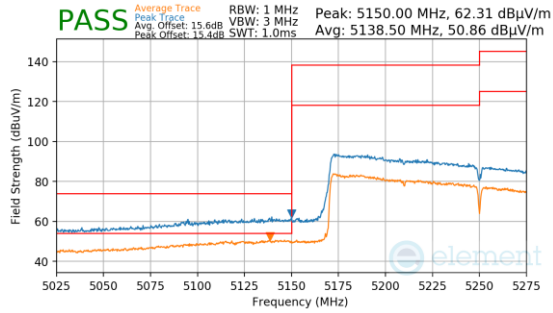
Plot 7-1647. Antenna 1b (Pk & Avg, Ch.50, 802.11ax(SU), MCS2)
