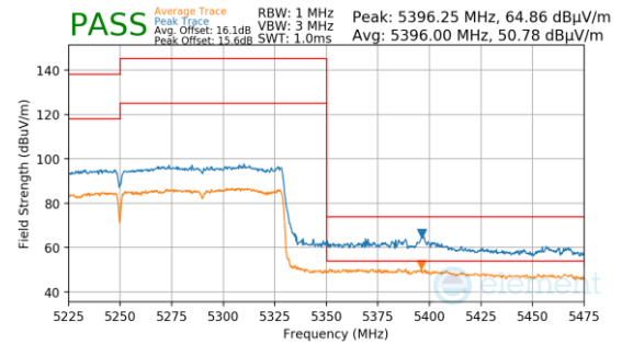
Plot 7-1651. Antenna 1b (Pk & Avg, Ch.50, 802.11ax(SU), MCS4)
