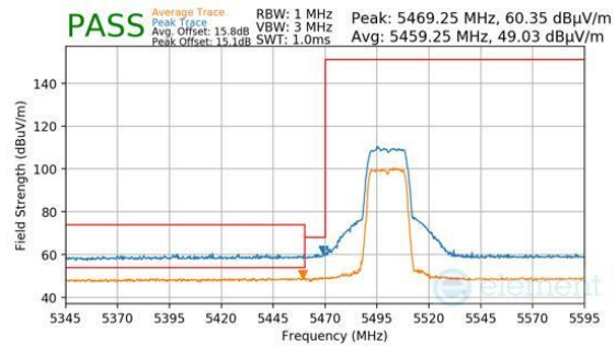
Plot 7-1670. CDD/SDM Primary (Pk & Avg, Ch.100, 802.11n, MCS15)
