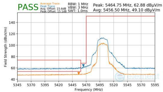
Plot 7-1669. CDD/SDM Primary (Pk & Avg, Ch.100, 802.11n, MCS12)
