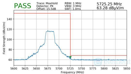
Plot 7-1676. CDD/SDM Primary (Pk, Ch.136, 802.11n, MCS15)
