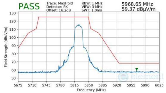
Plot 7-1889. CDD/SDM Diversity (Pk, Ch.165, 802.11n, MCS10)
