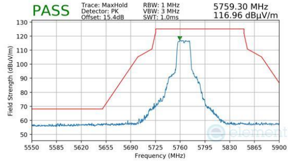
Plot 7-1888. CDD/SDM Diversity (Pk, Ch.153, 802.11n, MCS15)
