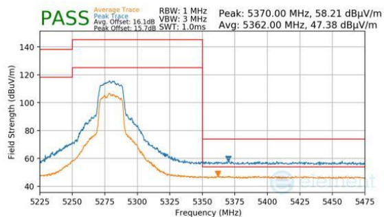
Plot 7-1859. CDD/SDM Diversity (Pk & Avg, Ch.56, 802.11n, MCS12)
