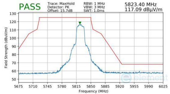
Plot 7-1890. CDD/SDM Diversity (Pk, Ch.165, 802.11n, MCS12)
