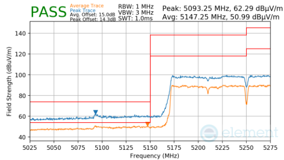
Plot 7-1826. CDD/SDM Primary (Pk & Avg, Ch.50, 802.11ac, MCS4)
