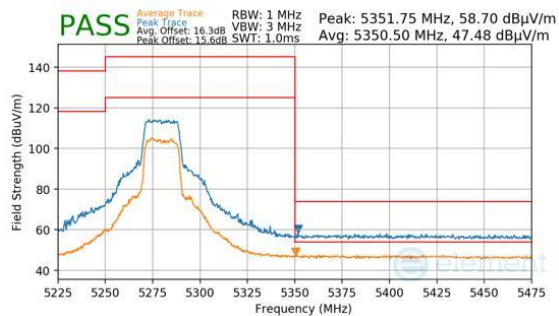
Plot 7-1860. CDD/SDM Diversity (Pk & Avg, Ch.56, 802.11n, MCS15)
