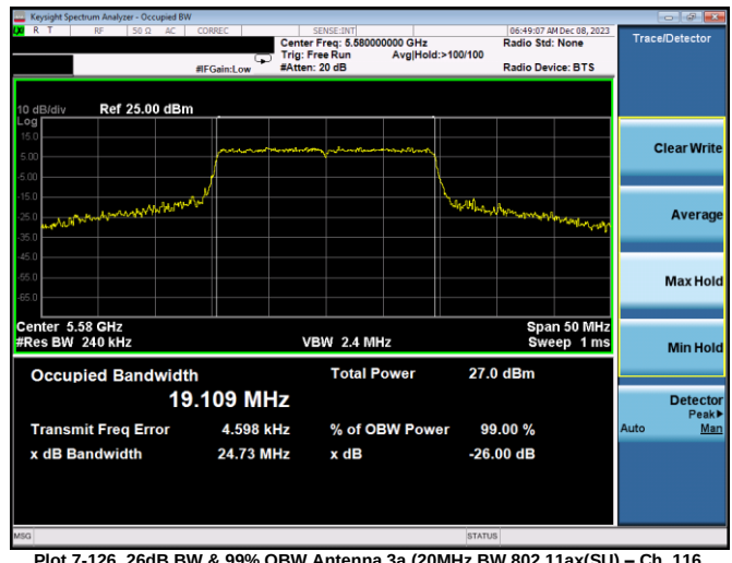
Plot 7-126. 26dB BW & 99% OBW Antenna 3a (20MHz BW 802.11ax(SU) – Ch. 116, MCS11)
