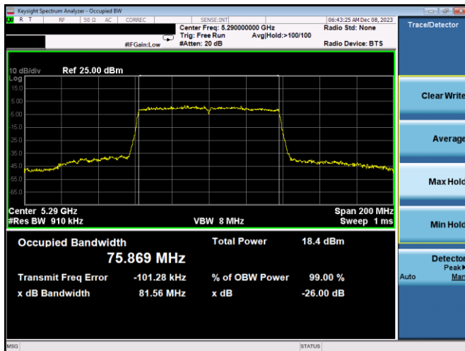
Plot 7-123. 26dB BW & 99% OBW Antenna 3a (80MHz BW 802.11ac – Ch. 58, MCS9)
