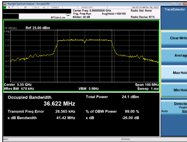
Plot 7-127. 26dB BW & 99% OBW Antenna 3a (40MHz BW 802.11n – Ch. 110), MCS7)
