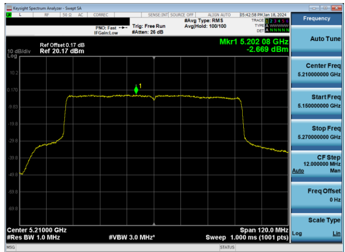
Plot 7-258. PSD Antenna 3c (80MHz BW 802.11ax(SU) – Ch. 42, MCS2)
