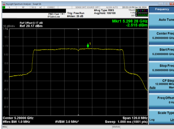
Plot 7-266. PSD Antenna 3c (80MHz BW 802.11ax(SU) – Ch. 58, MCS2)
