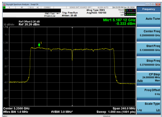
Plot 7-282. PSD Antenna 3c (160MHz BW 802.11ax(SU) – Ch. 50, MCS4)
