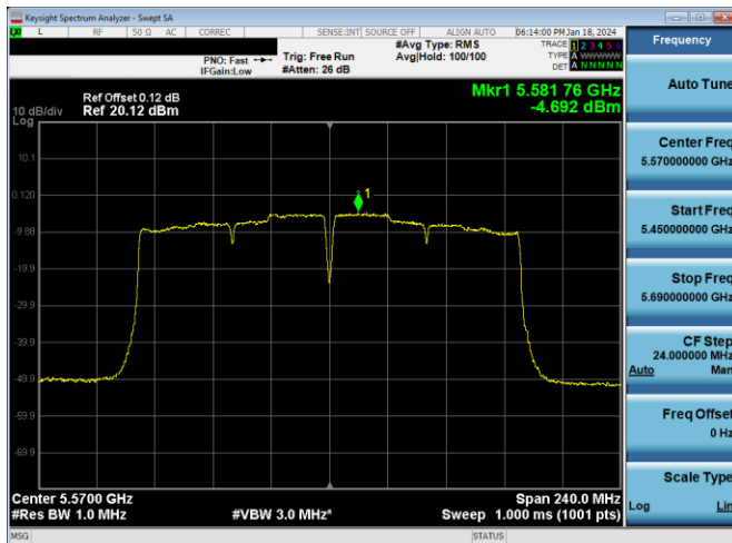
Plot 7-273. PSD Antenna 3c (160MHz BW 802.11ac - Ch. 114, MCS2)
