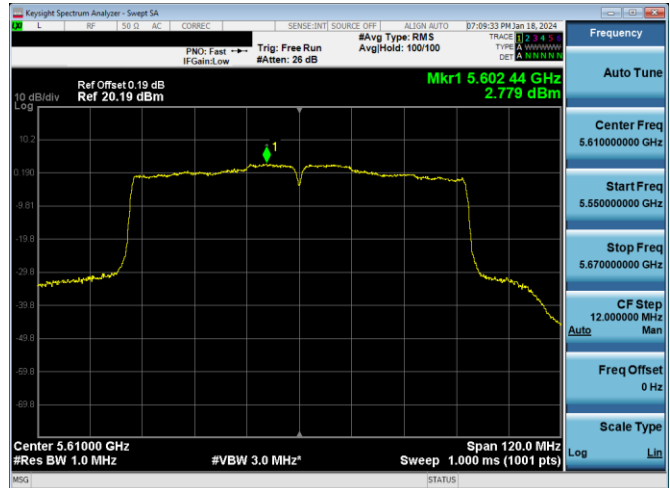
Plot 7-293. PSD Antenna 3c (80MHz BW 802.11ac – Ch. 122, MCS4)
