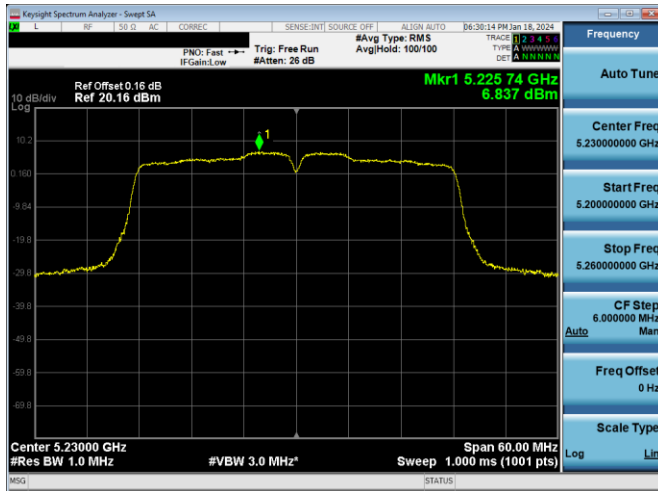
Plot 7-277. PSD Antenna 3c (40MHz BW 802.11n – Ch. 46, MCS4)
