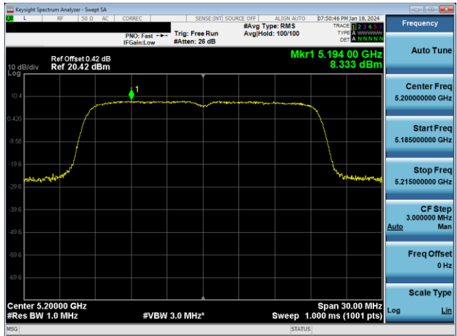
Plot 7-298. PSD Antenna 3c (20MHz BW 802.11ax(SU) – Ch. 40, MCS11)
