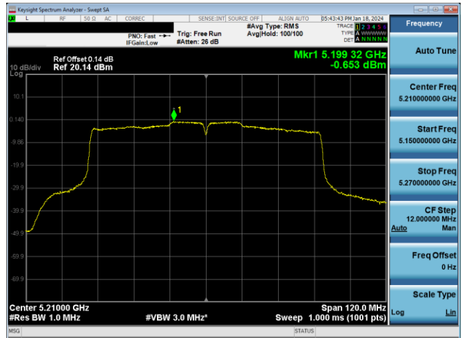
Plot 7-257. PSD Antenna 3c (80MHz BW 802.11ac – Ch. 42, MCS2)
