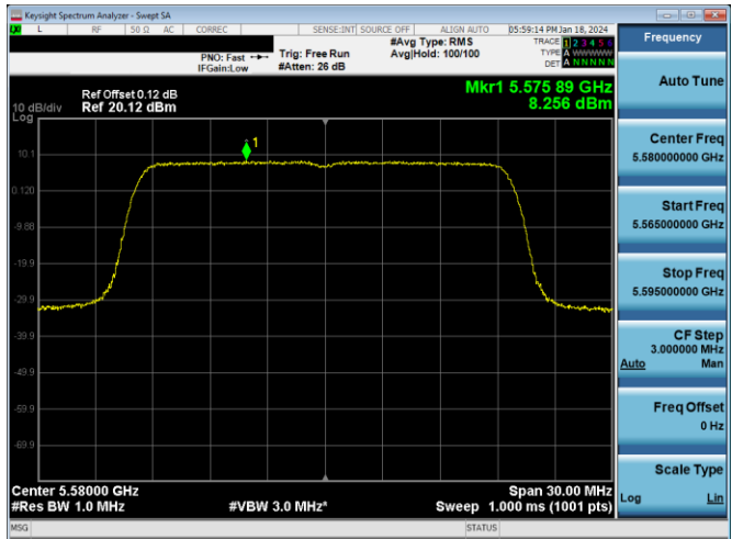
Plot 7-268. PSD Antenna 3c (20MHz BW 802.11ax(SU) – Ch. 116, MCS2)
