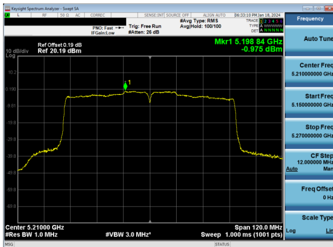
Plot 7-279. PSD Antenna 3c (80MHz BW 802.11ac – Ch. 42, MCS4)
