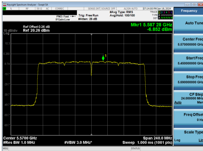
Plot 7-296. PSD Antenna 3c (160MHz BW 802.11ax(SU) – Ch. 114, MCS4)
