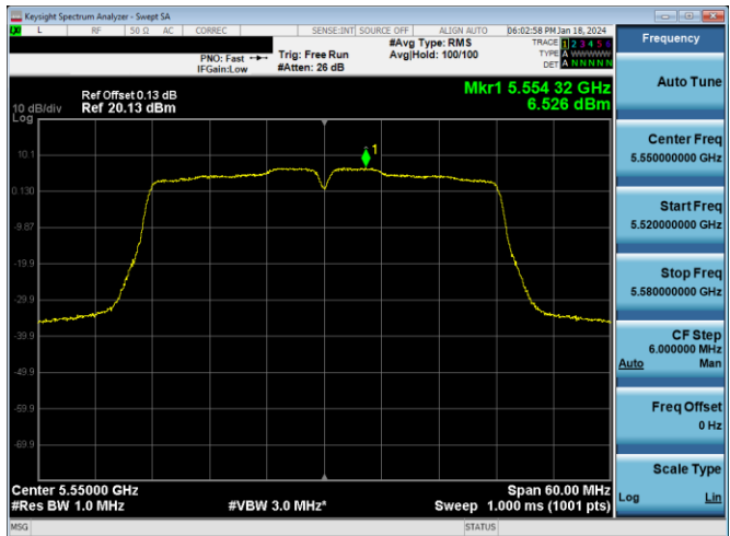
Plot 7-269. PSD Antenna 3c (40MHz BW 802.11n – Ch. 110, MCS2)
