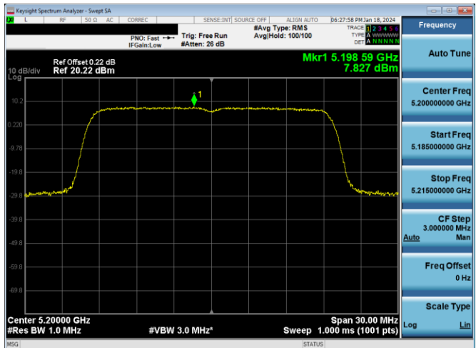
Plot 7-276. PSD Antenna 3c (20MHz BW 802.11ax(SU) - Ch. 40, MCS4)
