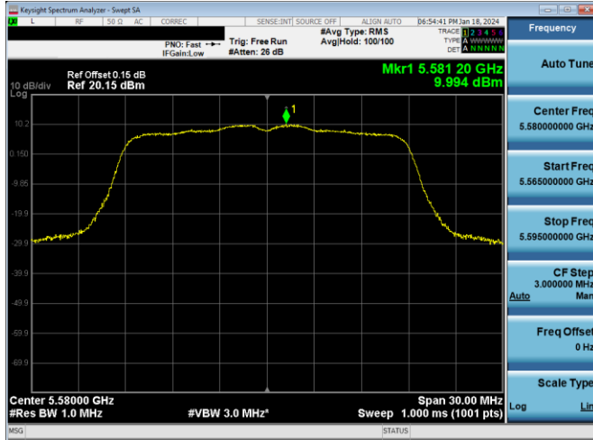
Plot 7-289. PSD Antenna 3c (20MHz BW 802.11n – Ch. 116, MCS4)
