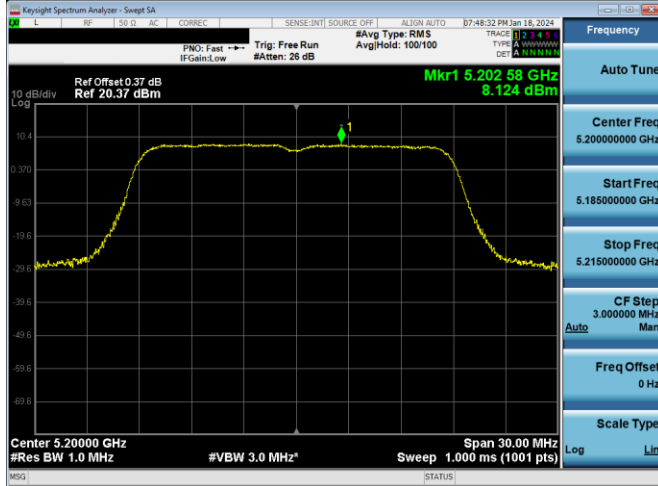
Plot 7-297. PSD Antenna 3c (20MHz BW 802.11n – Ch. 40, MCS7)
