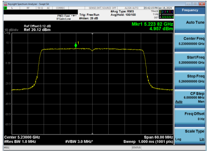
Plot 7-256. PSD Antenna 3c (40MHz BW 802.11ax(SU) – Ch. 46, MCS2)
