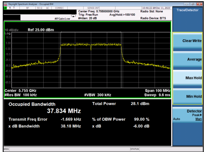
Plot 7-244. 6dB BW & 99% OBW Antenna 1b (40MHz BW 802.11ax(SU) – Ch. 151, MCS4)
