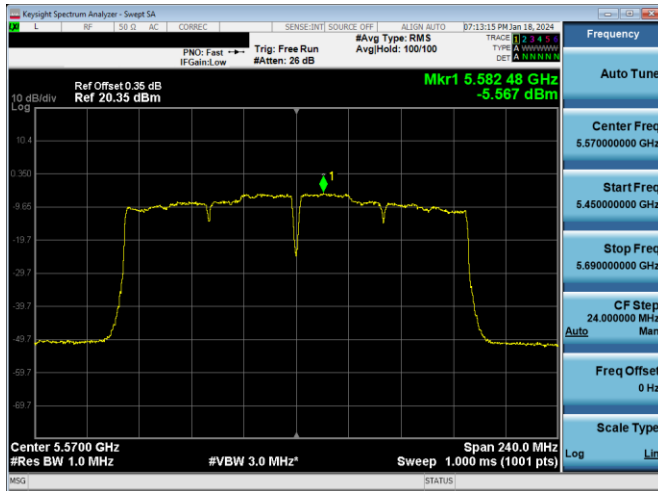
Plot 7-295. PSD Antenna 3c (160MHz BW 802.11ac – Ch. 114, MCS4)
