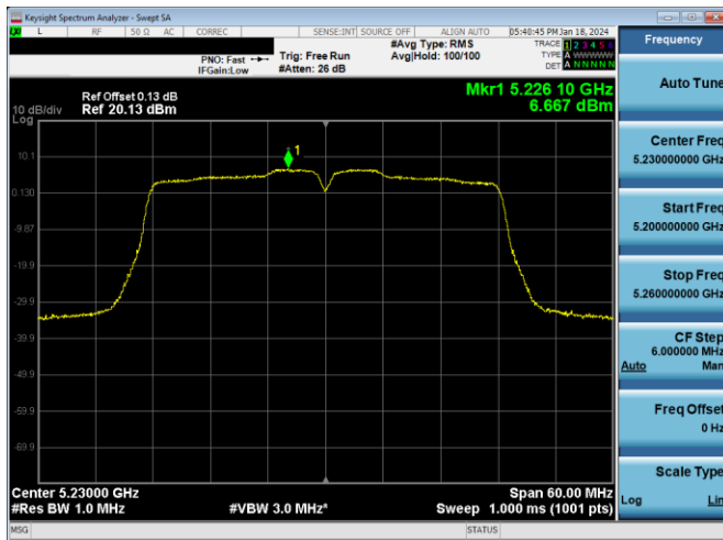
Plot 7-255. PSD Antenna 3c (40MHz BW 802.11n – Ch. 46, MCS2)
