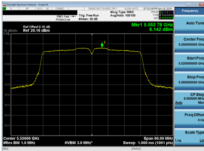
Plot 7-291. PSD Antenna 3c (40MHz BW 802.11n – Ch. 110, MCS4)
