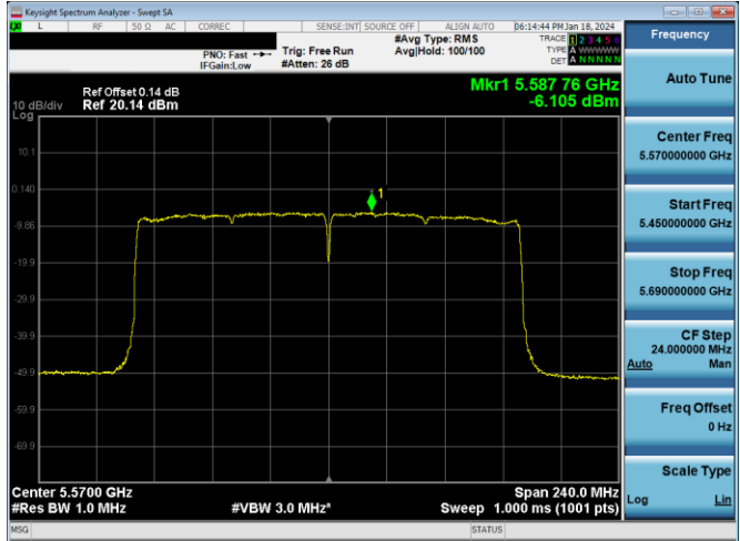
Plot 7-274. PSD Antenna 3c (160MHz BW 802.11ax(SU) - Ch. 114, MCS2)
