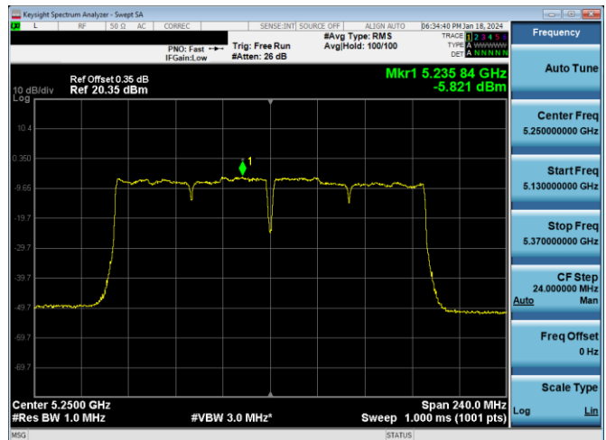
Plot 7-281. PSD Antenna 3c (160MHz BW 802.11ac – Ch. 50, MCS4)
