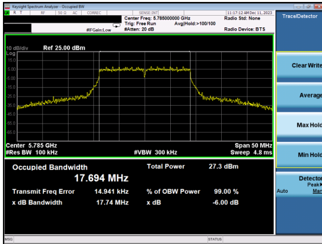
Plot 7-247. 6dB BW & 99% OBW Antenna 1b (20MHz BW 802.11n – Ch. 157, MCS7)
