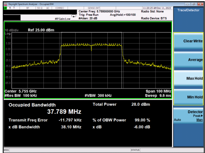
Plot 7-250. 6dB BW & 99% OBW Antenna 1b (40MHz BW 802.11ax(SU) – Ch. 151, MCS11)
