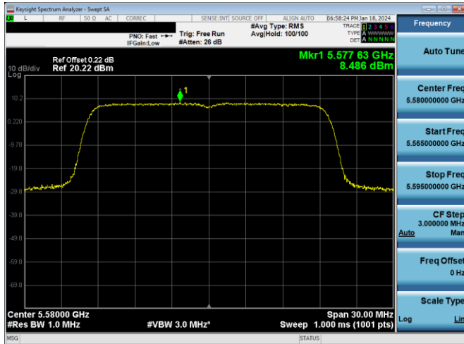
Plot 7-290. PSD Antenna 3c (20MHz BW 802.11ax(SU) – Ch. 116, MCS4)
