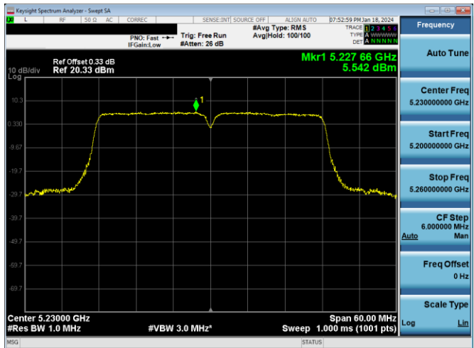
Plot 7-299. PSD Antenna 3c (40MHz BW 802.11n – Ch. 46, MCS7)
