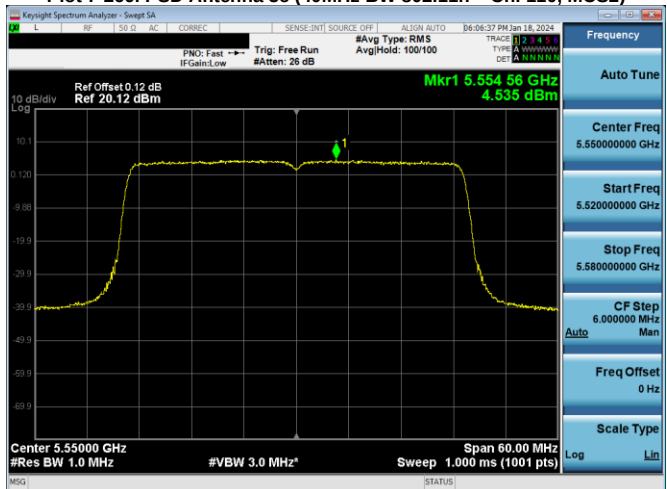
Plot 7-270. PSD Antenna 3c (40MHz BW 802.11ax(SU) – Ch. 110, MCS2)
