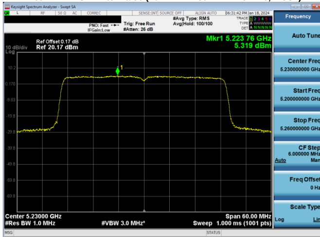
Plot 7-278. PSD Antenna 3c (40MHz BW 802.11ax(SU) – Ch. 46, MCS4)
