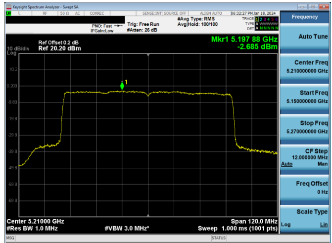
Plot 7-280. PSD Antenna 3c (80MHz BW 802.11ax(SU) – Ch. 42, MCS4)
