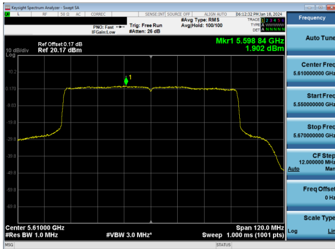
Plot 7-272. PSD Antenna 3c (80MHz BW 802.11ax(SU) - Ch. 122, MCS2)
