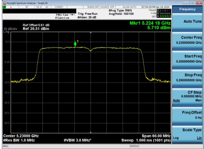
Plot 7-300. PSD Antenna 3c (40MHz BW 802.11ax(SU) – Ch. 46, MCS11)
