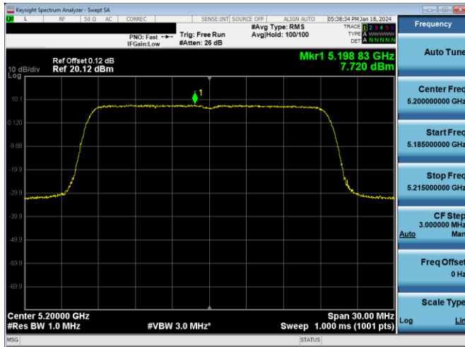
Plot 7-254. PSD Antenna 3c (20MHz BW 802.11ax(SU) – Ch. 40, MCS2)
