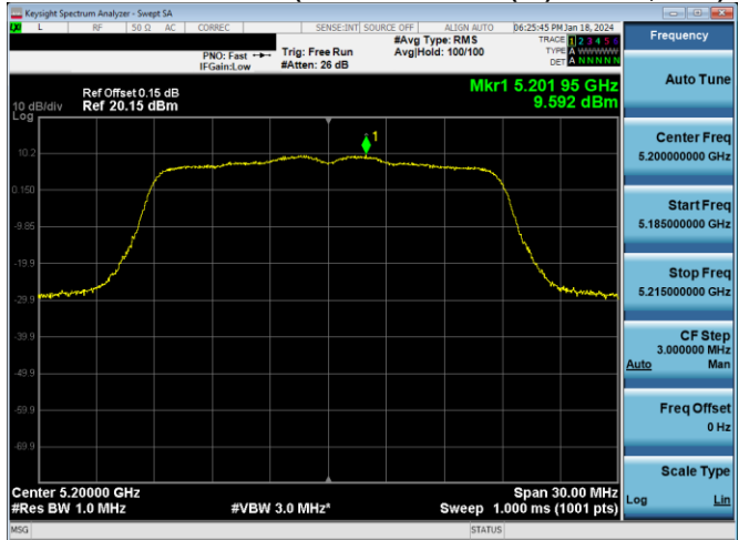
Plot 7-275. PSD Antenna 3c (20MHz BW 802.11n - Ch. 40, MCS4)
