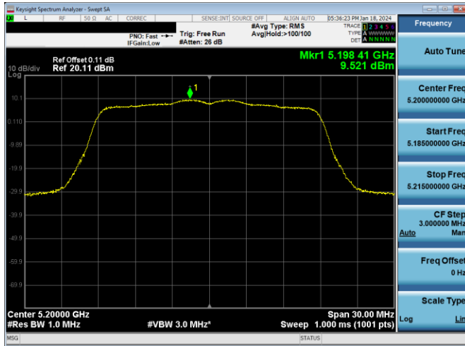
Plot 7-253. PSD Antenna 3c (20MHz BW 802.11n – Ch. 40, MCS2)
