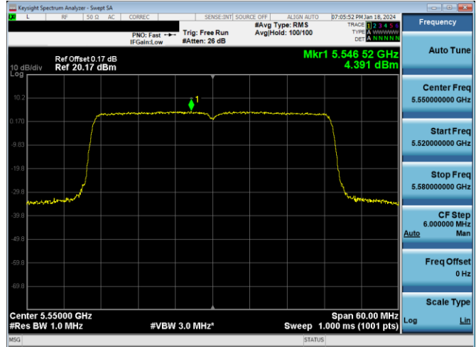
Plot 7-292. PSD Antenna 3c (40MHz BW 802.11ax(SU) – Ch. 110, MCS4)
