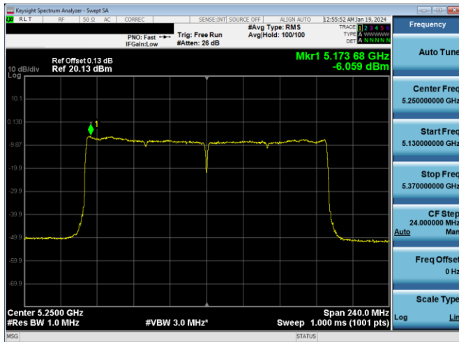
Plot 7-591. PSD CDD PRIMARY Antenna 3c (160MHz BW 802.11ax(SU) – Ch. 50, MCS2)
