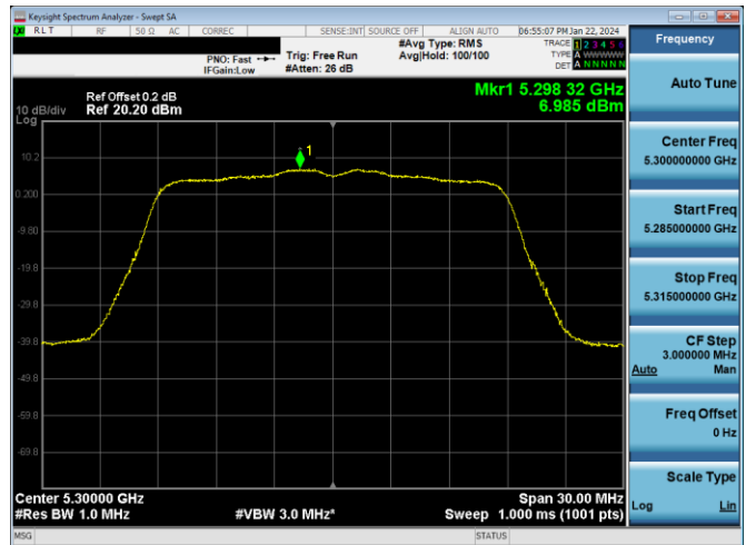
Plot 7-594. PSD CDD PRIMARY Antenna 3a (20MHz BW 802.11n – Ch. 60, MCS10)
