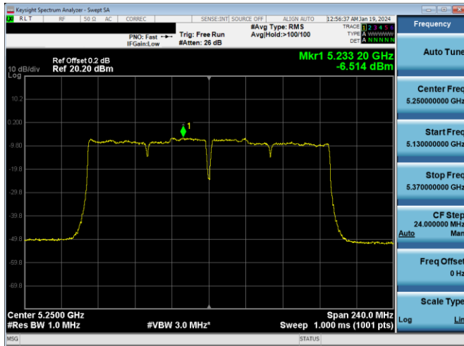
Plot 7-589. PSD CDD PRIMARY Antenna 3c (160MHz BW 802.11ac – Ch. 50, MCS2)
