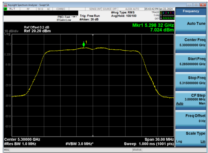
Plot 7-593. PSD CDD PRIMARY Antenna 3c (20MHz BW 802.11n – Ch. 60, MCS10)
