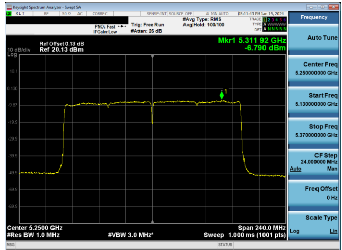
Plot 7-592. PSD CDD PRIMARY Antenna 3a (160MHz BW 802.11ax(SU) – Ch. 50, MCS2)
