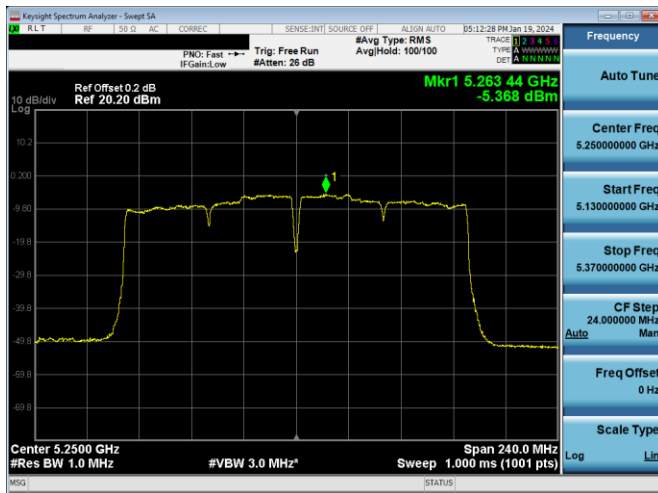
Plot 7-590. PSD CDD PRIMARY Antenna 3a (160MHz BW 802.11ac – Ch. 50, MCS2)
