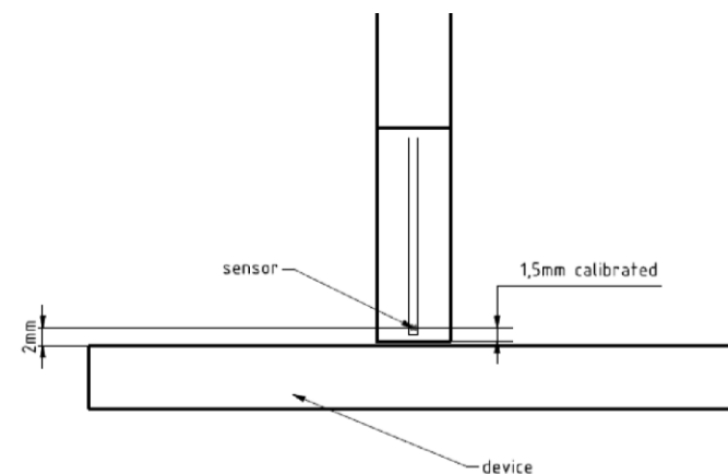
Figure I-2 EUMmWVx Probe
