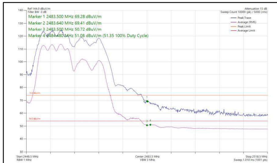
Figure 48 - 802.11ax, HE20, RU 106-53, CDD, Core 0-1 - 2462 MHz, Band Edge Frequency 2483.5 MHz
