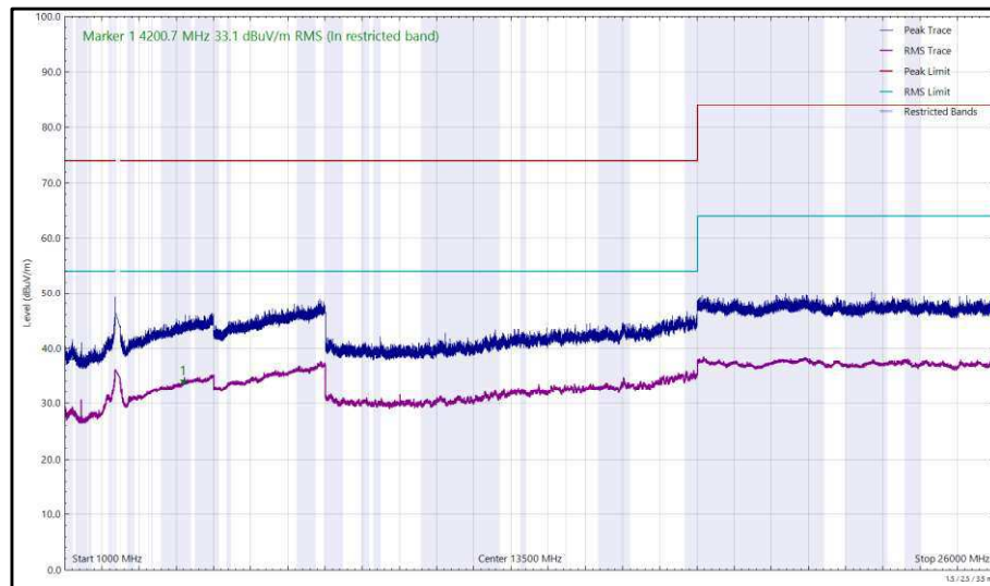
Figure 116 - 2412 MHz (CH1), 802.11g, Core 1, 1 GHz to 26 GHz, Vertical
