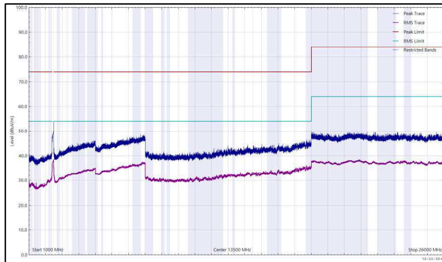
Figure 118 - 2442 MHz (CH7), 802.11g, Core 1, 1 GHz to 26 GHz, Horizontal
