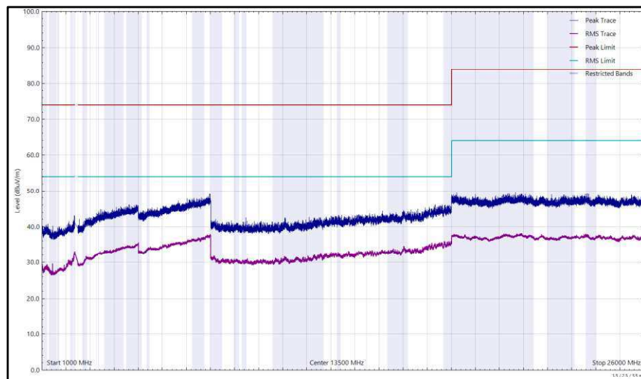
Figure 91 - 2412 MHz (CH1), 802.11b, Core 0, 1 GHz to 26 GHz, Horizontal
